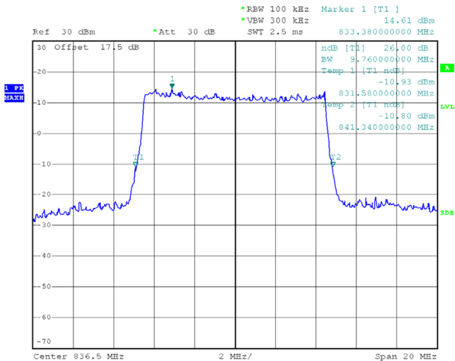
(Plot P4: 26dB Bandwidth LTE Band 5/10MHz/16QAM)
