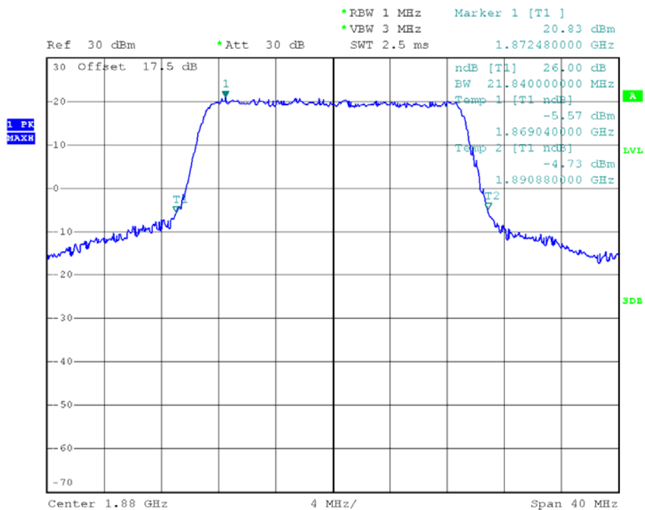
(Plot F4: 26dB Bandwidth LTE Band 2/20MHz/16QAM)
