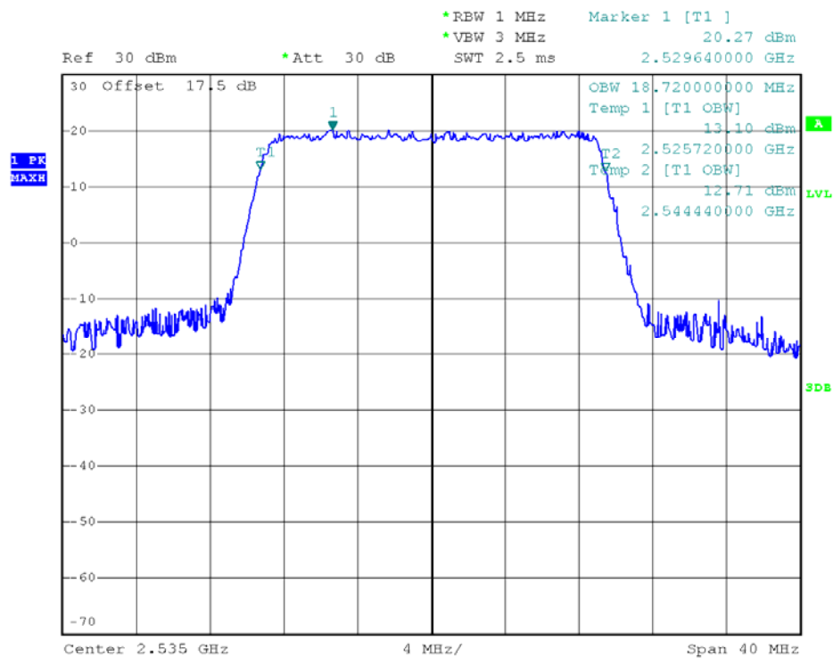
(Plot T3: 99% Occupied Bandwidth LTE Band 7/20MHz/16QAM)
