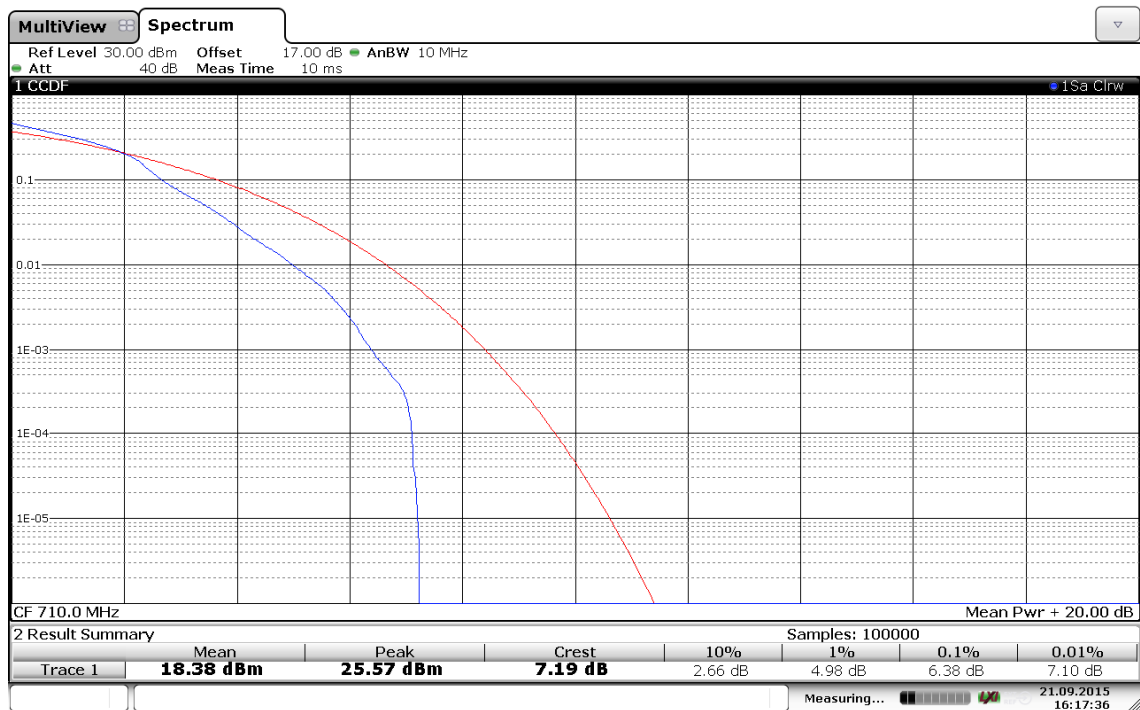
(Plot E4: Band 17/10MHz/16QAM in Ch.23790 100RB Size)
