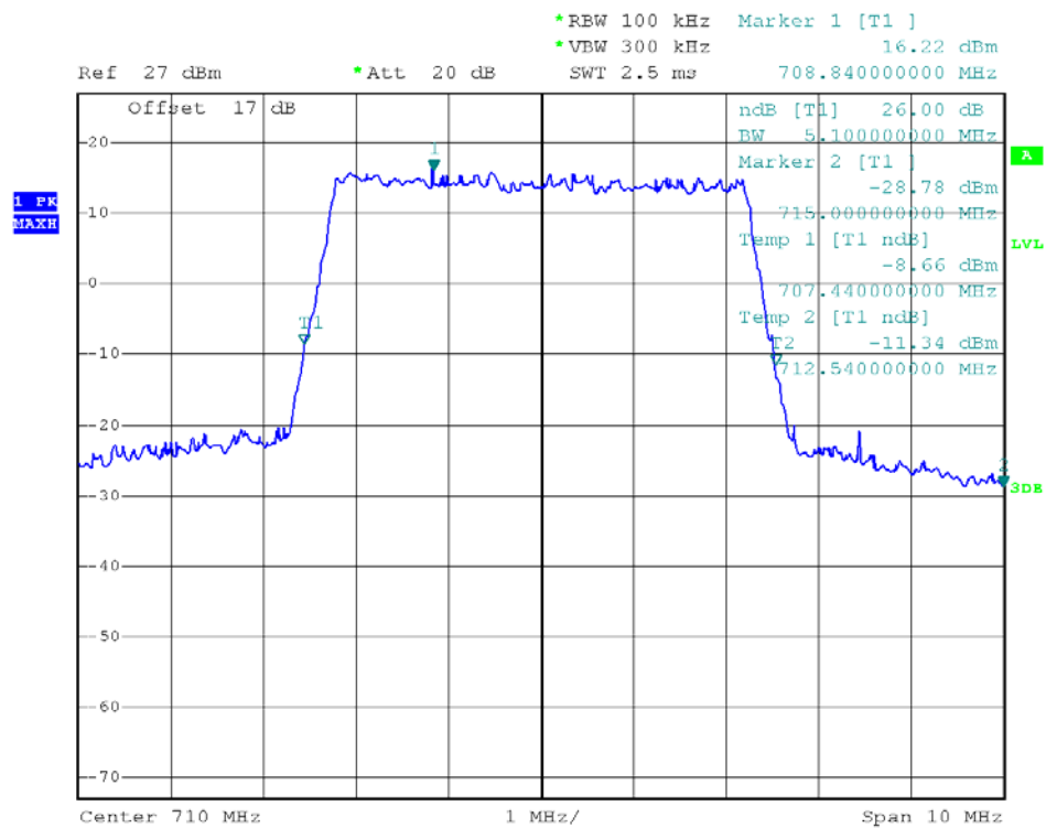
(Plot U2: 26dB Bandwidth LTE Band 17/5MHz/QPSK)
