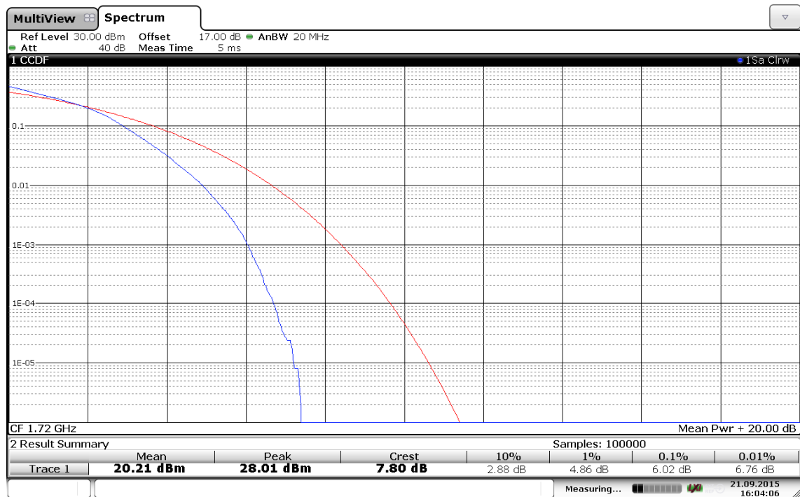
(Plot B2: Band 4/20MHz/16QAM in Ch.20050 100RB Size)
