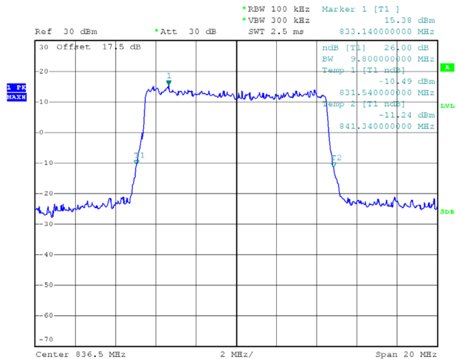
(Plot P2: 26dB Bandwidth LTE Band 5/10MHz/QPSK)
