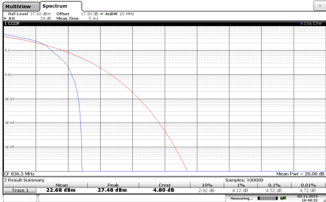
(Plot C3: Band 5/10MHz/16QAM in Ch.20525 1RB Size)
