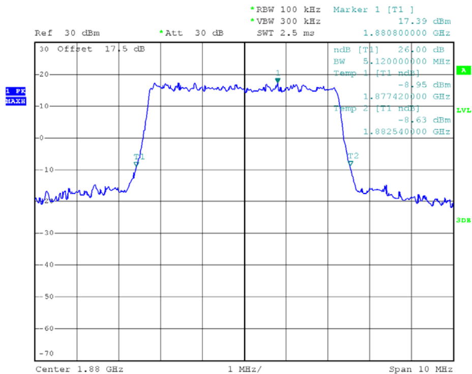
(Plot C2: 26dB Bandwidth LTE Band 2/5MHz/QPSK)
