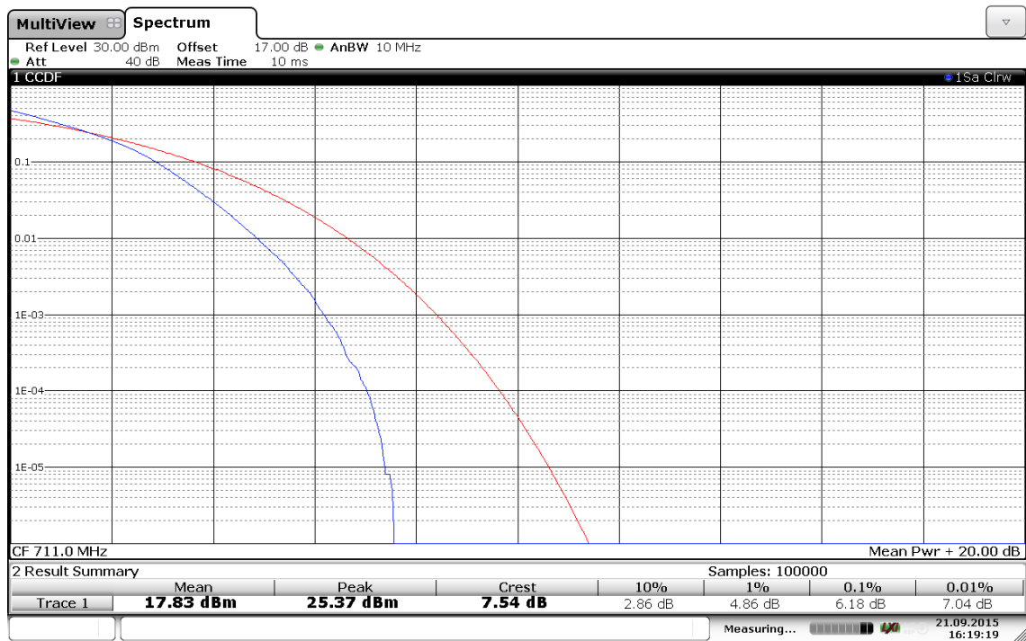
(Plot E6: Band 17/10MHz/16QAM in Ch.23800 100RB Size)
