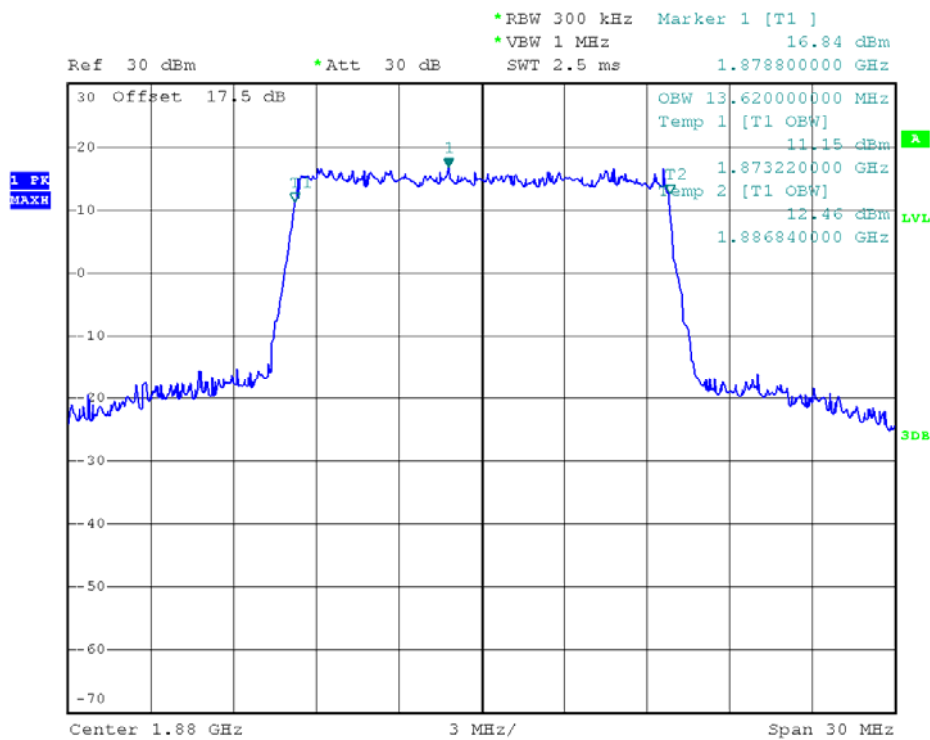
(Plot E3: 99% Occupied Bandwidth LTE Band 2/15MHz/16QAM)
