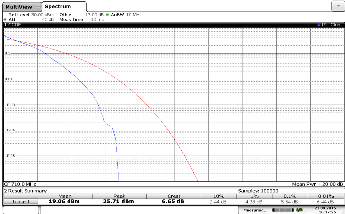
(Plot E3: Band 17/10MHz/16QAM in Ch.23790 1RB Size)
