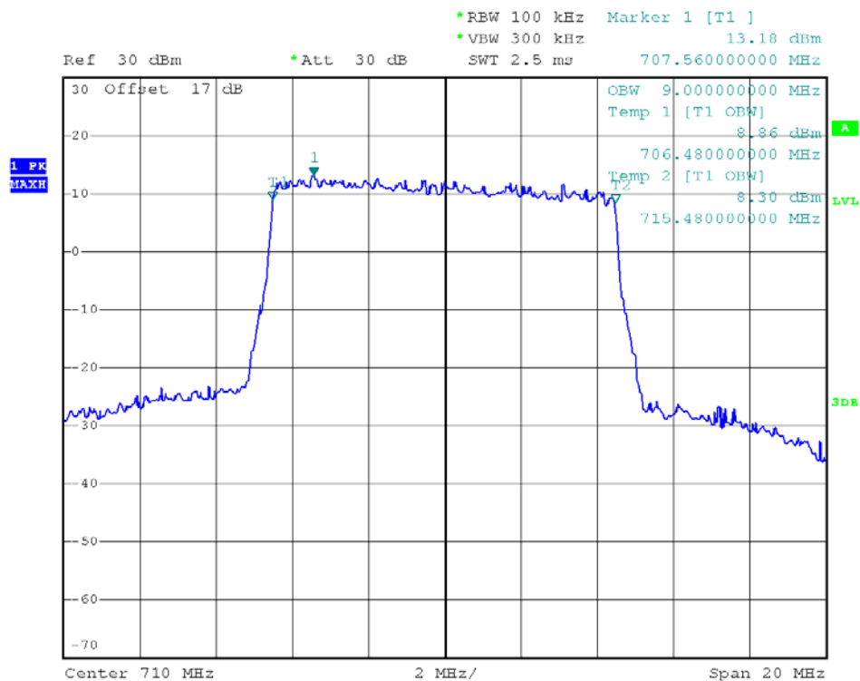
(Plot V1: 99% Occupied Bandwidth 10MHz/QPSK Channel = 23790)
