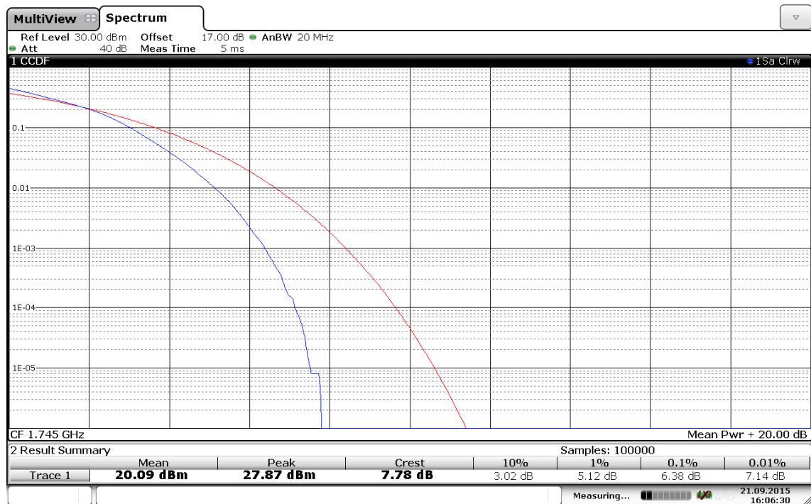
(Plot B6: Band 4/20MHz/16QAM in Ch.20300 100RB Size)
