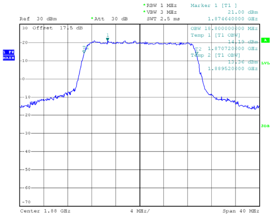
(Plot F3: 99% Occupied Bandwidth LTE Band 2/20MHz/16QAM)
