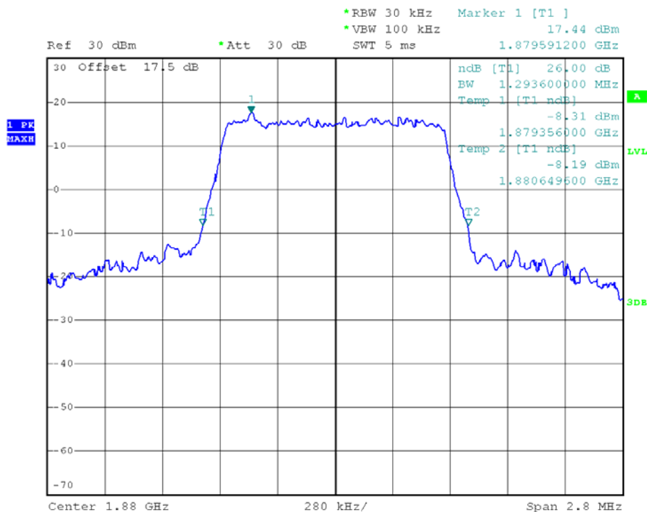
(Plot A4: 26dB Bandwidth LTE Band 2 1.4MHz/16QAM)
