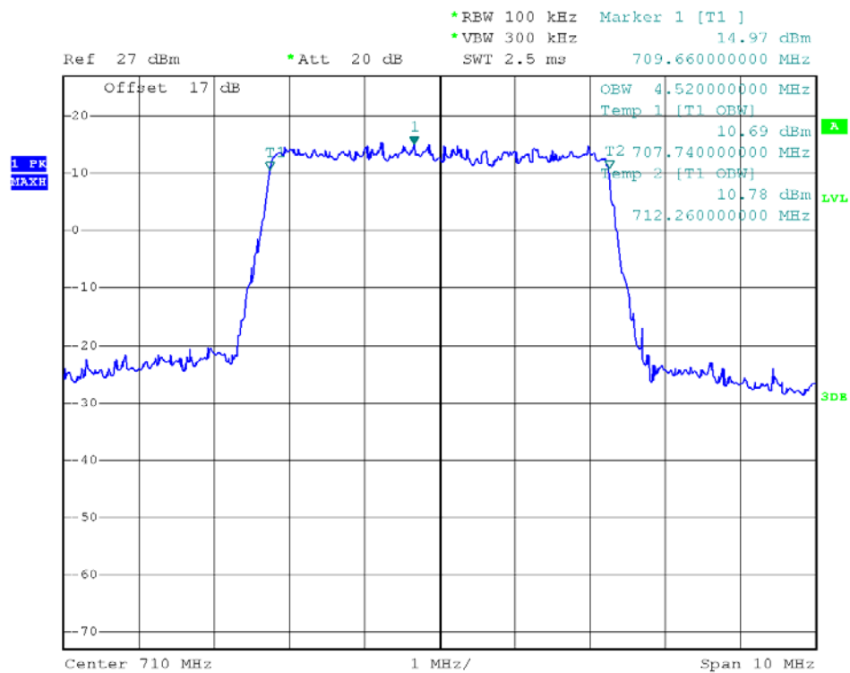
(Plot U1: 99% Occupied Bandwidth LTE Band 17/5MHz/QPSK)
