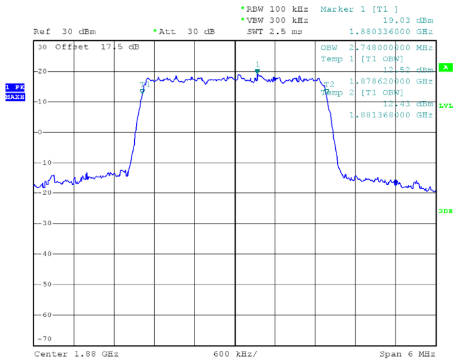
(Plot B1: 99% Occupied Bandwidth LTE Band 2/3MHz/QPSK)
