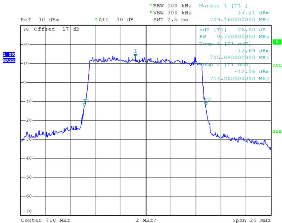
(Plot V4: 26dB Bandwidth 10MHz/16QAM Channel = 23790)
