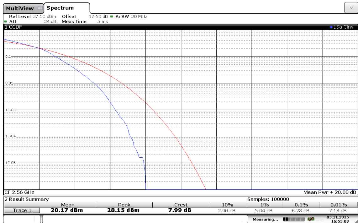
(Plot D6: Band 7/20MHz/16QAM in Ch.21350 100RB Size)
