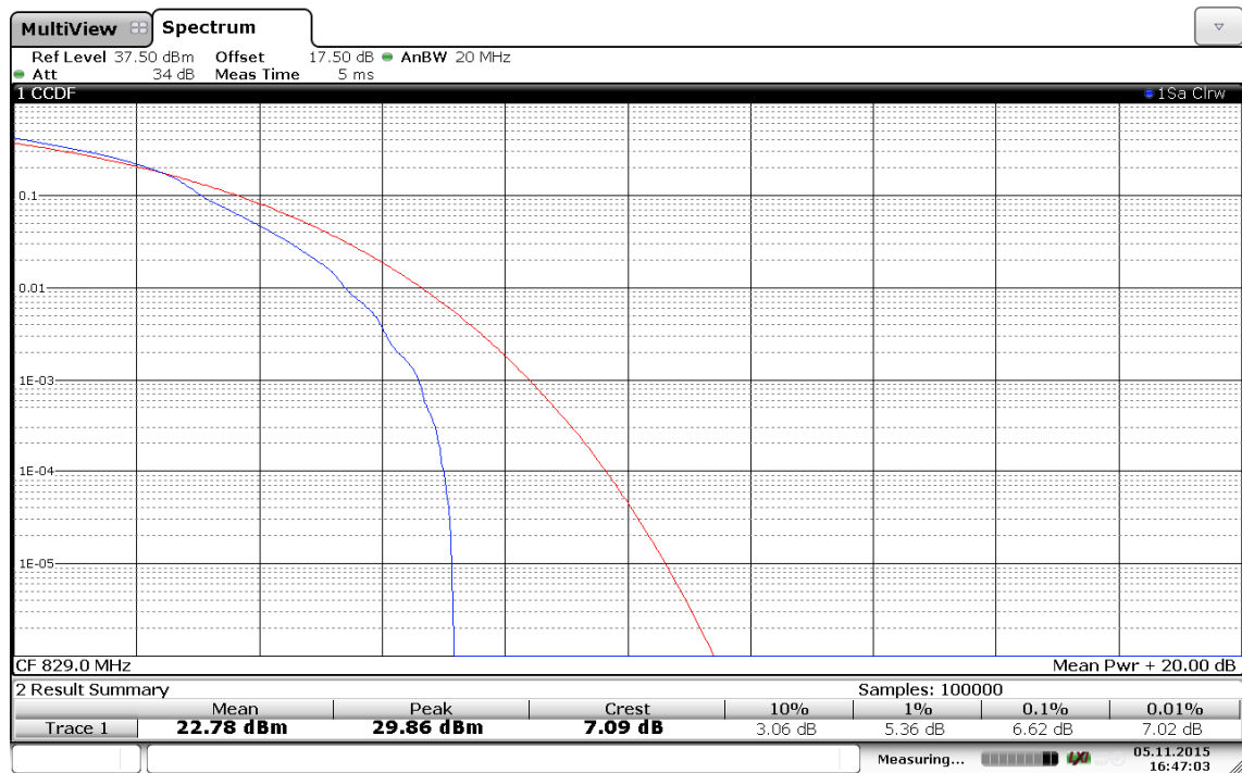
(Plot C2: Band 5/10MHz/16QAM in Ch.20450 50RB Size)
