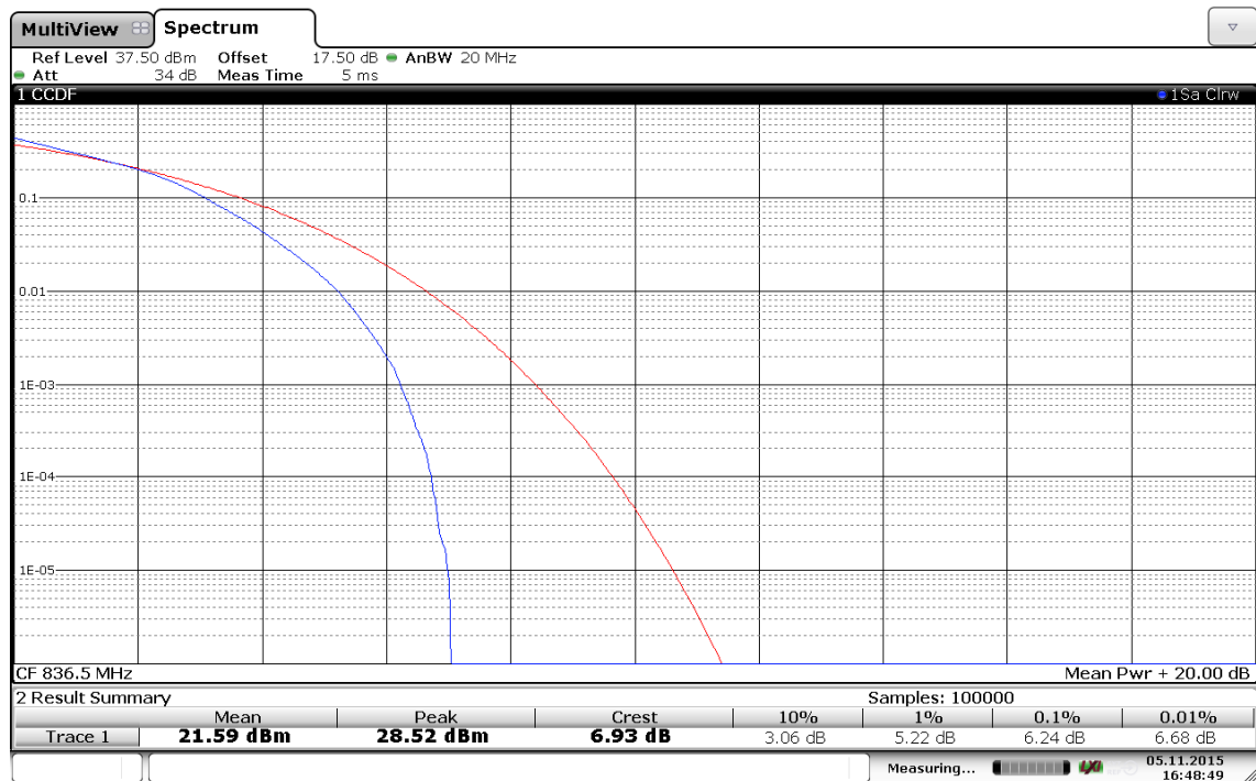
(Plot C4: Band 5/10MHz/16QAM in Ch.20525 50RB Size)
