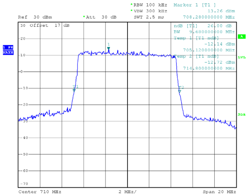
(Plot V2: 26dB Bandwidth 10MHz/QPSK Channel = 23790)
