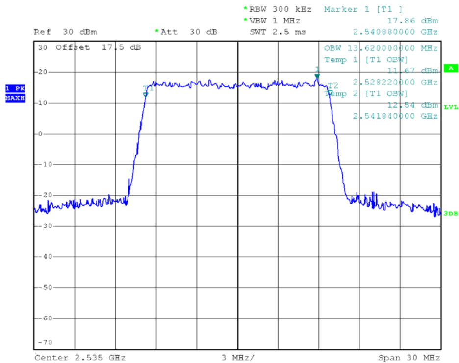
(Plot S1: 99% Occupied Bandwidth LTE Band 7/15MHz/QPSK)
