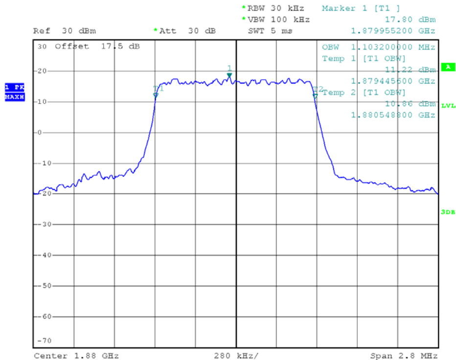
(Plot A1: 99% Occupied Bandwidth LTE Band 2 1.4MHz/QPSK)
