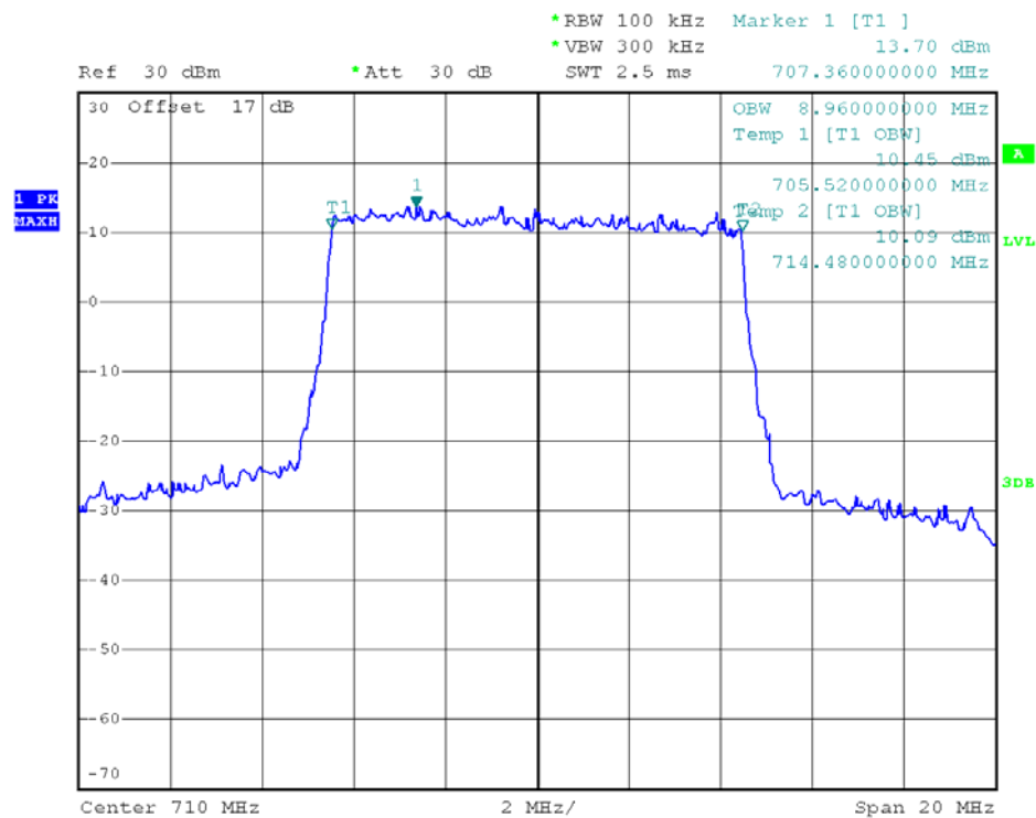
(Plot V3: 99% Occupied Bandwidth 10MHz/16QAM Channel = 23790)
