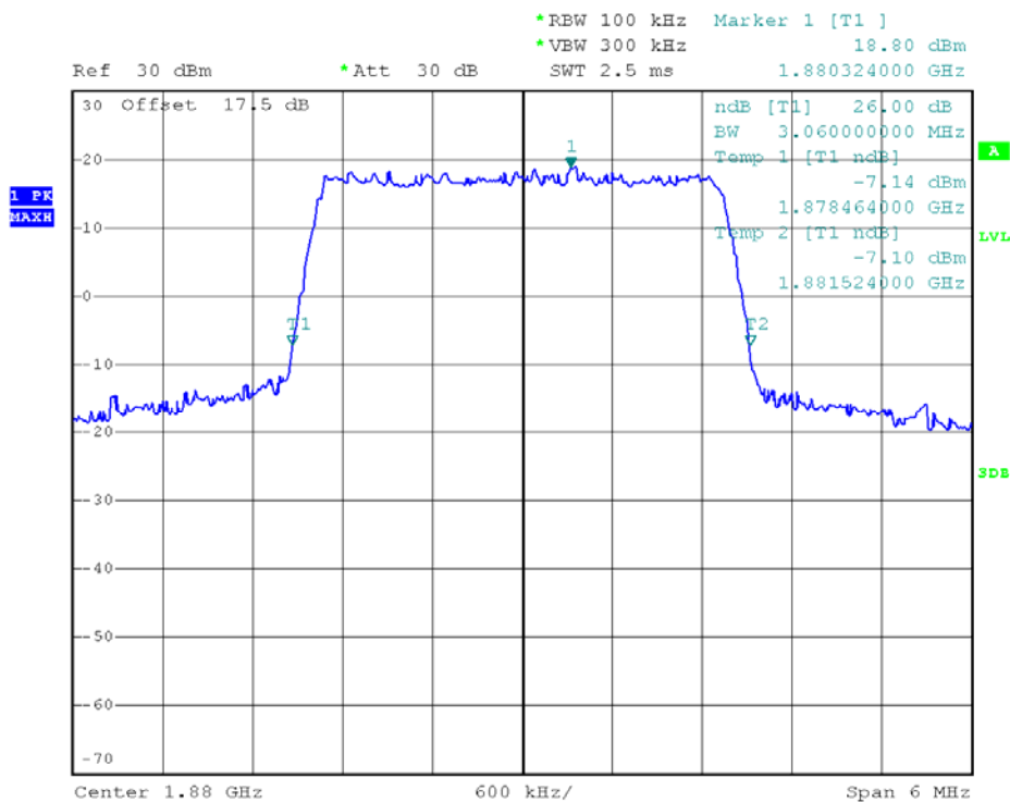
(Plot B2: 26dB Bandwidth LTE Band 2/3MHz/QPSK)
