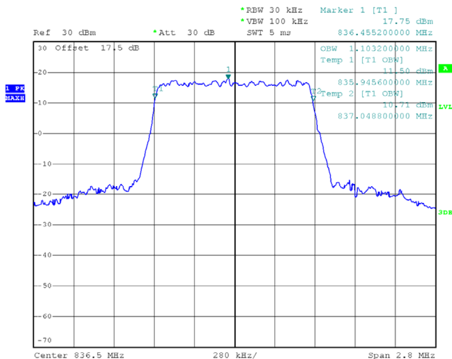
(Plot M1: 99% Occupied Bandwidth LTE Band 5/1.4MHz/QPSK)
