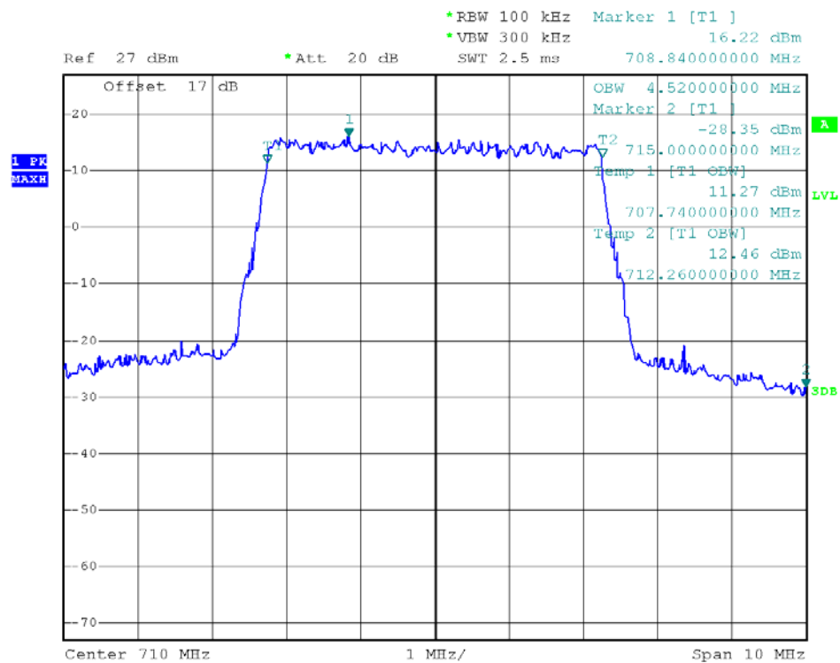
(Plot U3: 99% Occupied Bandwidth 5MHz/16QAM Channel = 23790)
