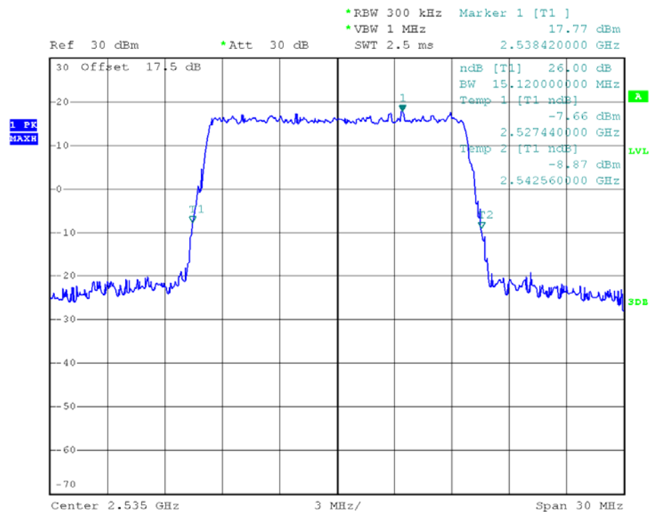
(Plot S2: 26dB Bandwidth LTE Band 7/15MHz/QPSK)
