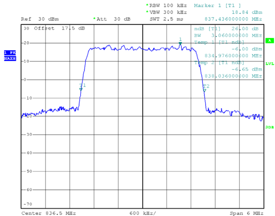
(Plot N4: 26dB Bandwidth LTE Band 5/3MHz/16QAM)
