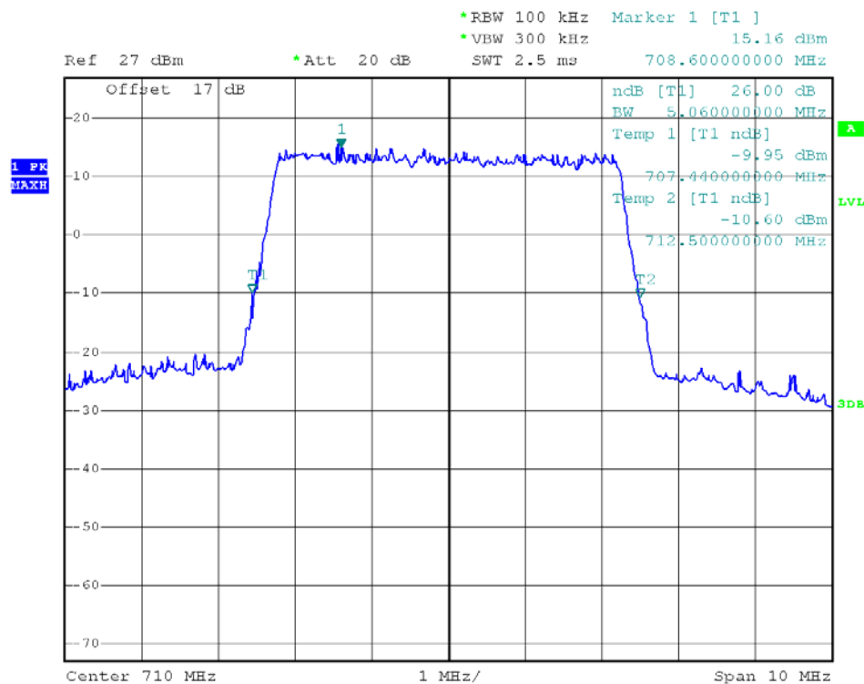
(Plot U4: 26dB Bandwidth 5MHz/16QAM Channel = 23790)
