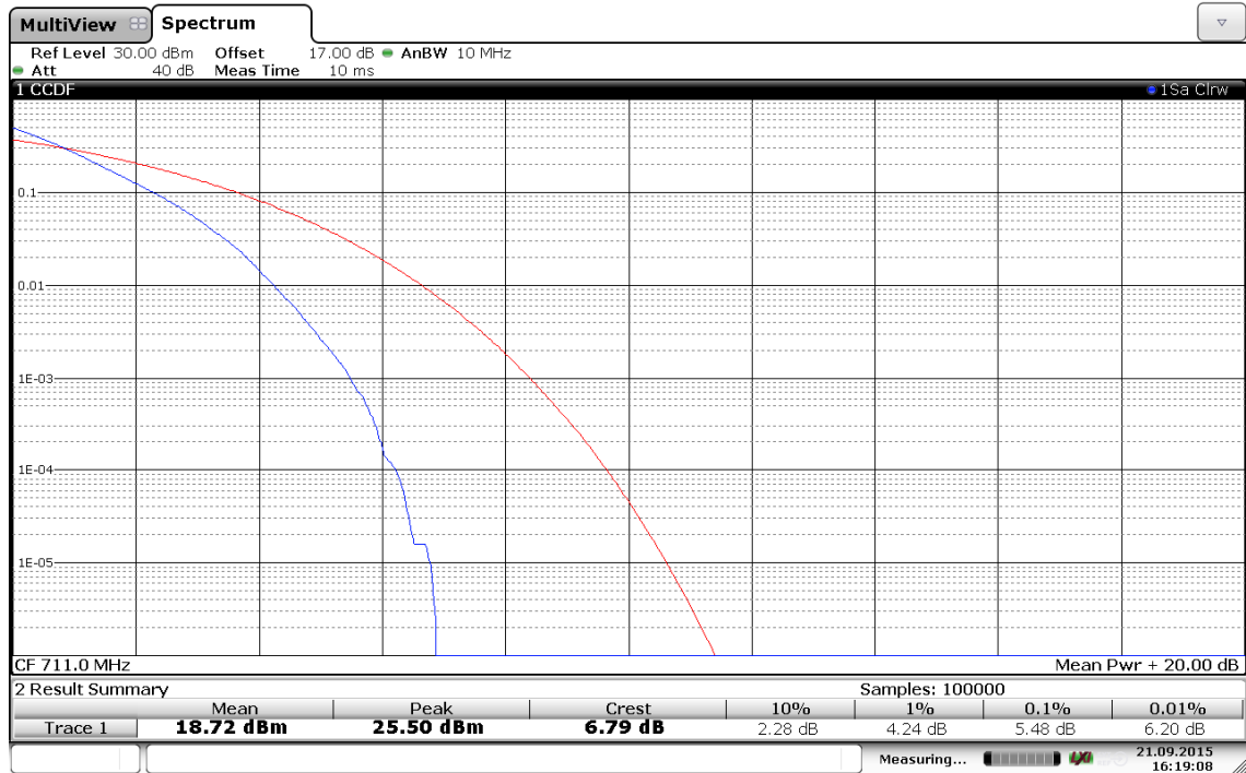
(Plot E5: Band 17/10MHz/16QAM in Ch.23800 1RB Size)
