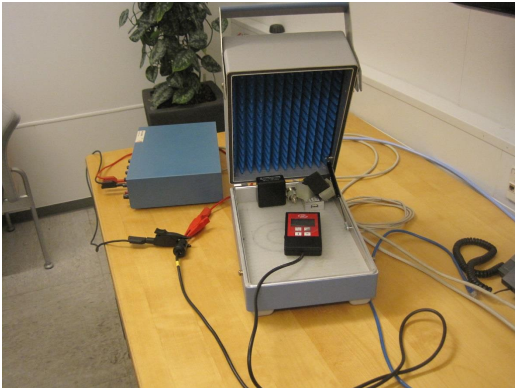
Photo 4.4.1 Test setup regarding measurement of 20 dB bandwidth.
