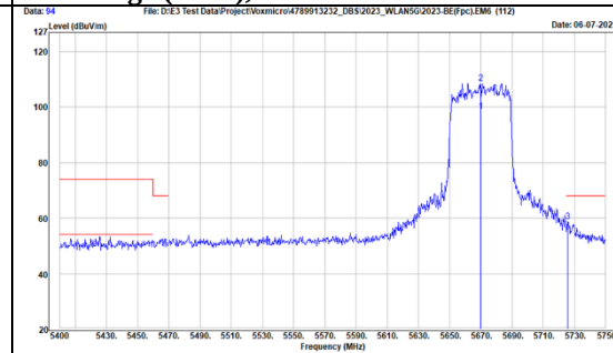
TX, 802.11ax(HE40) (Ch 134) Band Edge (Peak), Vertical
