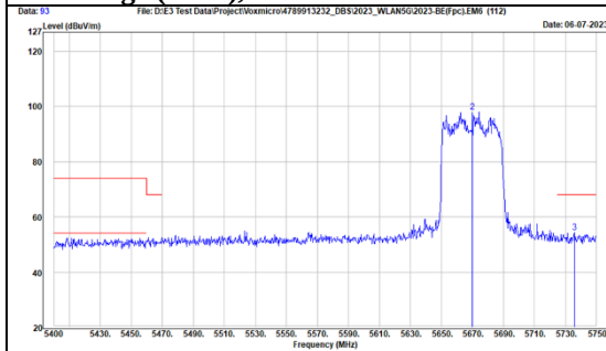
TX, 802.11ax(HE40) (Ch 134) Band Edge (Peak), Horizontal
