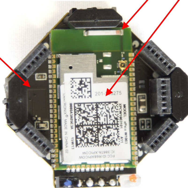
RF (Top) Board, Bottom view
