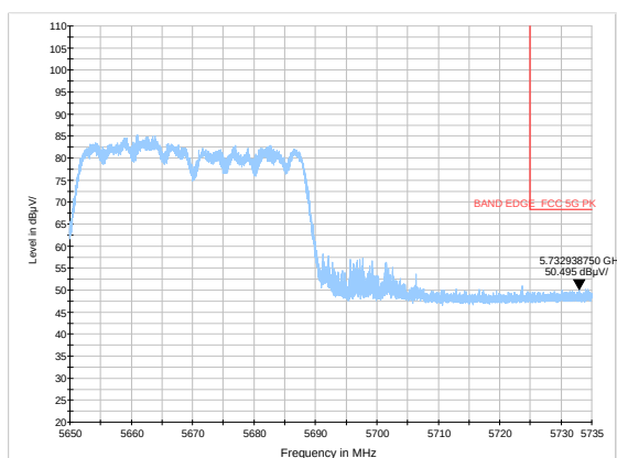
802.11ac HT40-Channel 134: Peak
