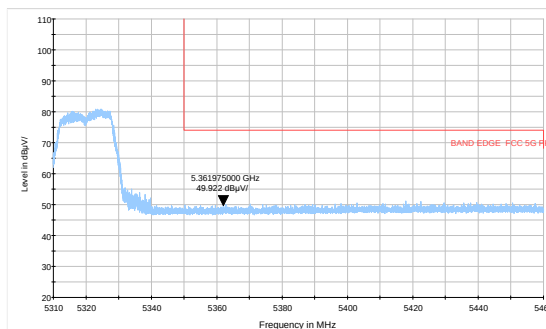
802.11a-Channel 64: Average
