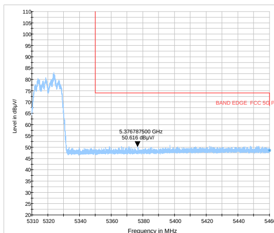
802.11n HT20-Channel 64: Peak
