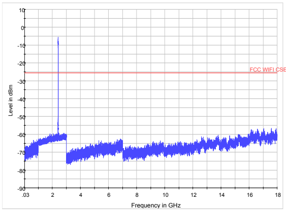
802.11g CH1 30MHz to 18GHz
