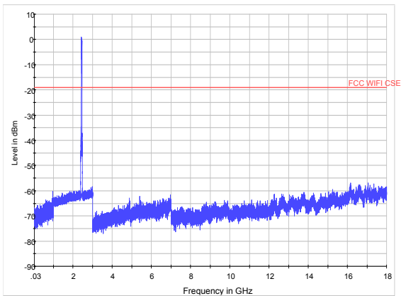
802.11n (HT40) CH6 30MHz to 18GHz
