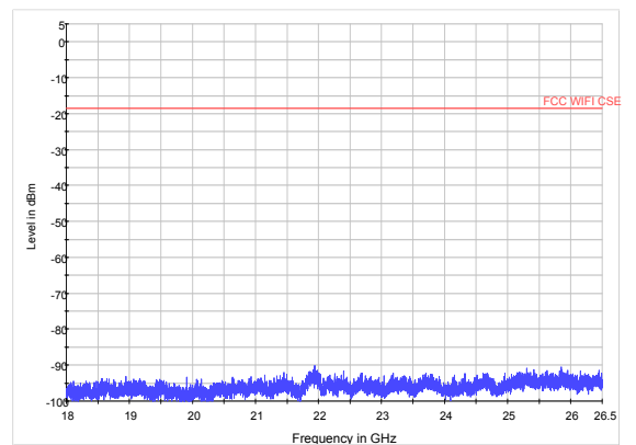
802.11n (HT40) CH9 18GHz to 26.5GHz
