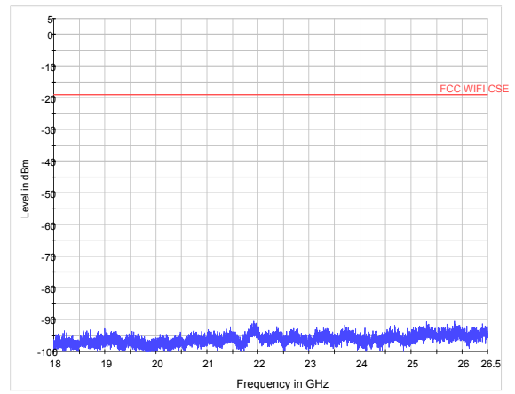
802.11n (HT40) CH3 18GHz to 26.5GHz
