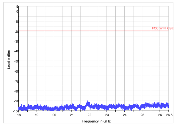
802.11n (HT40) CH6 18GHz to 26.5GHz
