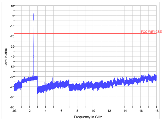
802.11n (HT20) CH11 30MHz to 18GHz
