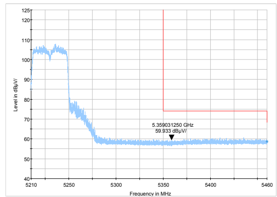
802.11ac HT40-Channel 46: Peak
