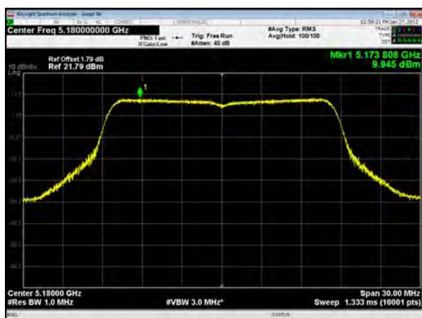
U-NII-1, 802.11a, Channel No.: 36
