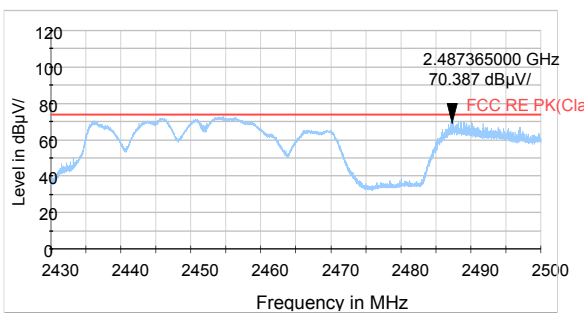
802.11n HT40 -Channel 9 Peak
