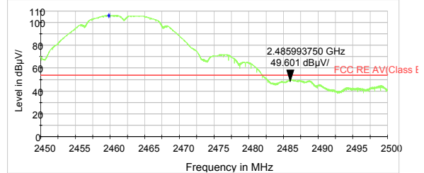
802.11b-Channel 11 Average
