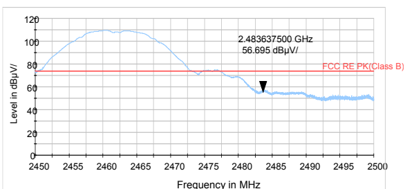
802.11b-Channel 11 Peak
