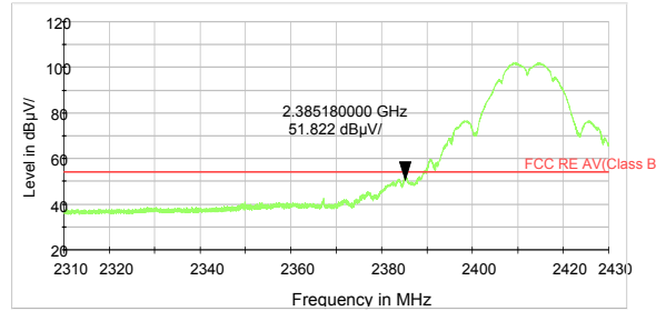
802.11b-Channel 1 Average
