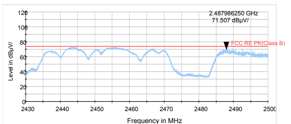
802.11n HT40 -Channel 9 Peak
