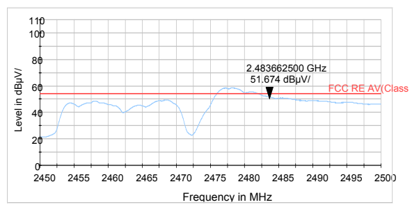
802.11g-Channel 11 Average
