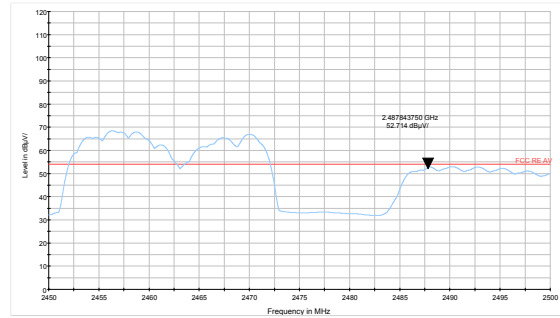
802.11ax HE20 -Channel 11 Average
