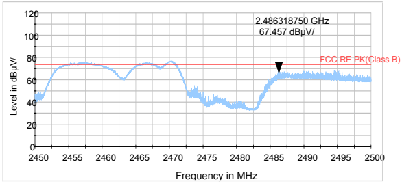
802.11n HT20 -Channel 11 Peak
