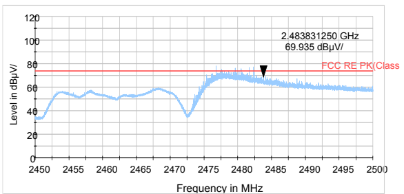
802.11n HT20 -Channel 11 Peak
