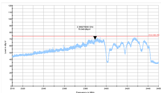
802.11ax HE40 -Channel 3 Peak
