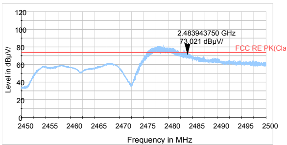
802.11g-Channel 11 Peak
