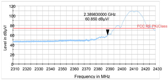
802.11b-Channel 1 Peak
