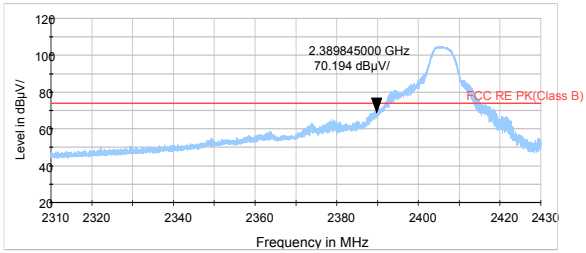
802.11g-Channel 1 Peak
