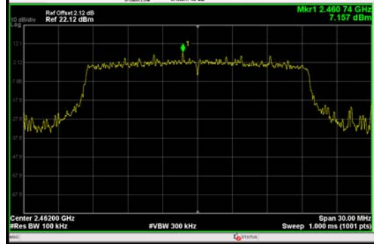
802.11ax(HE20), Channel No.: 11
