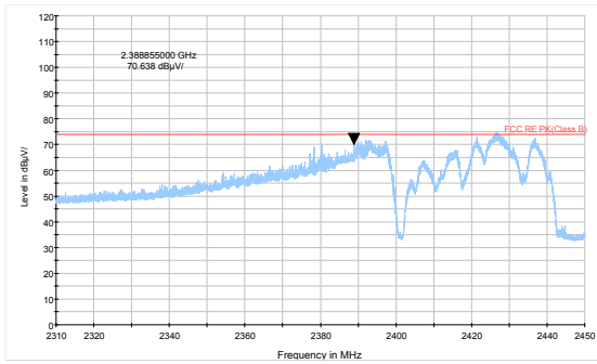
802.11ax HE40 -Channel 3 Peak
