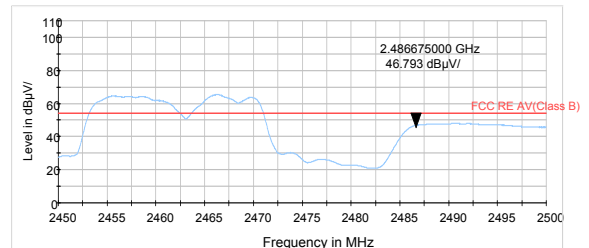
802.11g-Channel 11 Average
