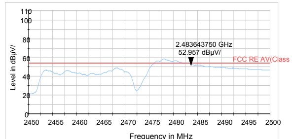
802.11n HT20 -Channel 11 Average
