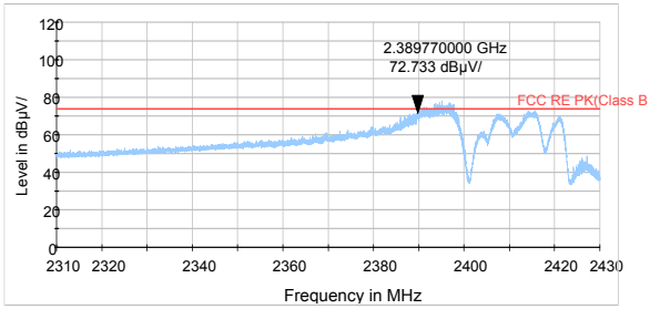
802.11ax HE20 -Channel 1 Peak
