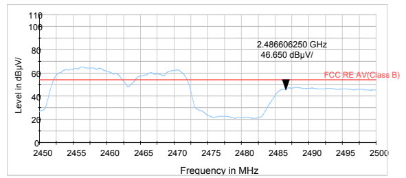
802.11ax HE20 -Channel 11 Average
