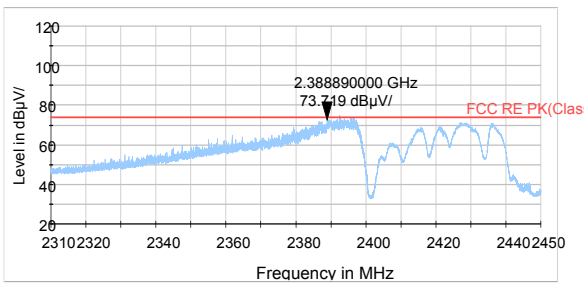
802.11n HT40 -Channel 3 Peak
