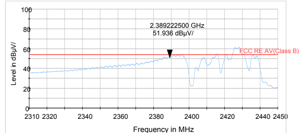
802.11n HT40 -Channel 3 Average
