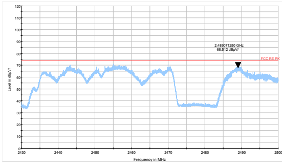
802.11ax HE40-Channel 9 Peak
