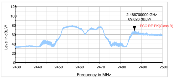
802.11ax HE20 -Channel 11 Peak
