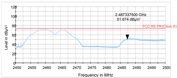
802.11b-Channel 11 Peak
