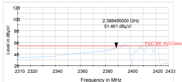
802.11ax HE20 -Channel 1 Average
