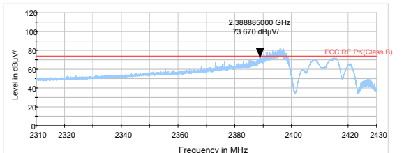
802.11n HT20 -Channel 1 Peak
