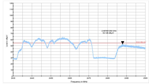
802.11ax HE40-Channel 9 Average
