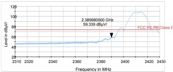
802.11b-Channel 1 Peak
