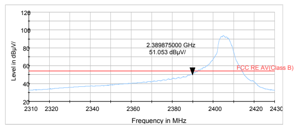
802.11n HT20 -Channel 1 Average
