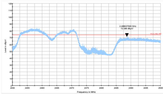
802.11ax HE20 -Channel 11 Peak
