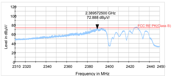
802.11n HT40 -Channel 3 Peak
