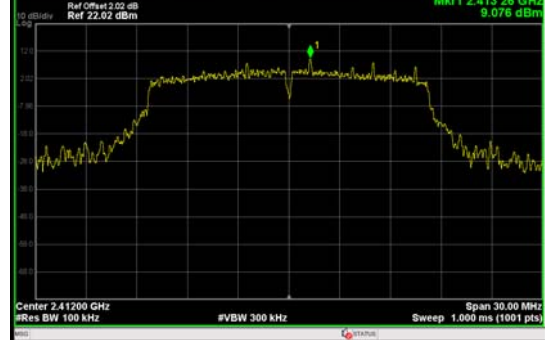
802.11g, Channel No.: 1
