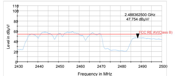
802.11n HT40 -Channel 9 Average
