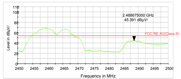
802.11b-Channel 11 Average
