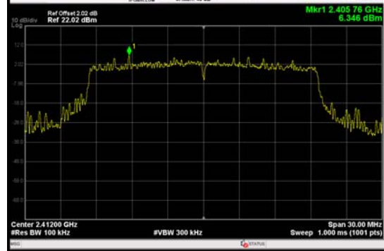
802.11ax(HE20), Channel No.: 1
