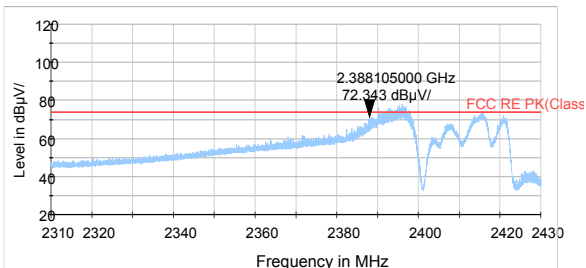
802.11ax HE20 -Channel 1 Peak
