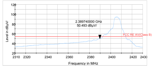
802.11g-Channel 1 Average
