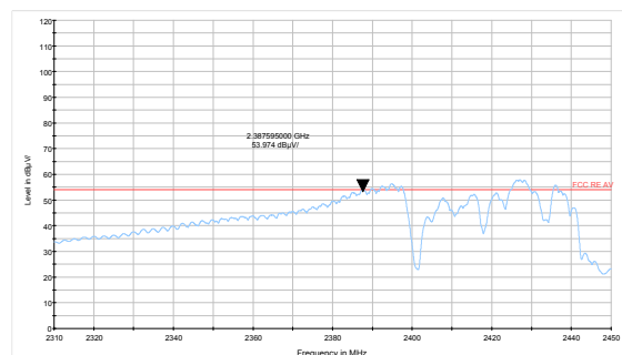
802.11ax HE40 -Channel 3 Average
