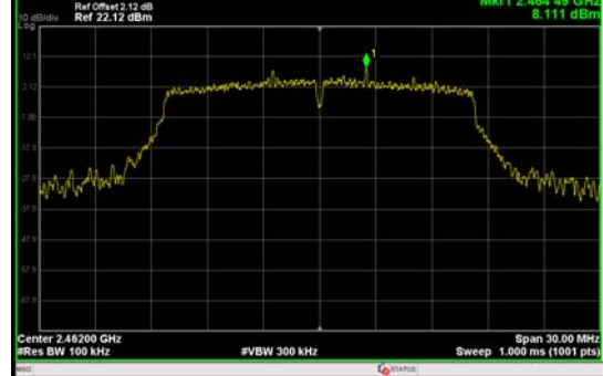
802.11g, Channel No.: 11
