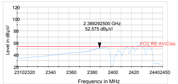
802.11n HT40 -Channel 3 Average
