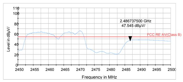
802.11n HT20 -Channel 11 Average
