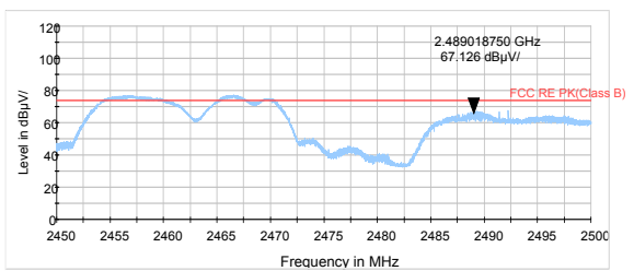
802.11g-Channel 11 Peak
