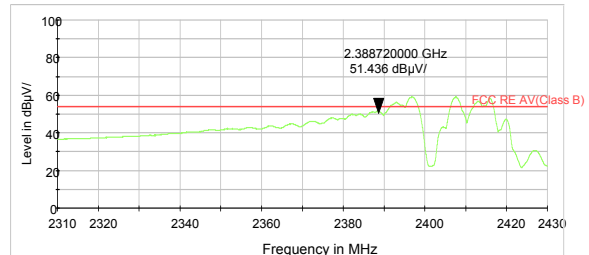
802.11g-Channel 1 Average
