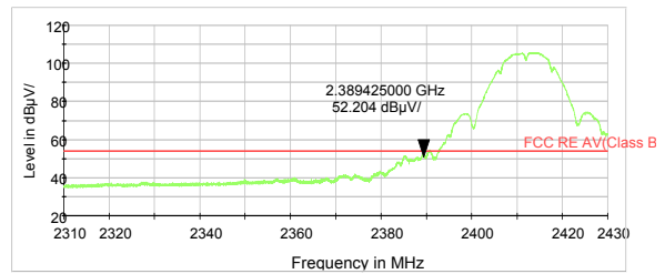
802.11b-Channel 1 Average
