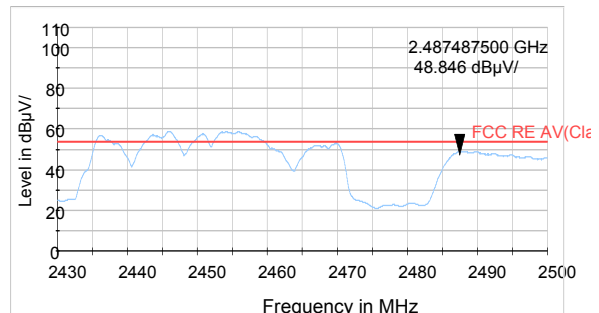
802.11n HT40 -Channel 9 Average
