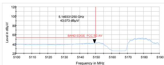
802.11ax HE20-Channel 36: Average
