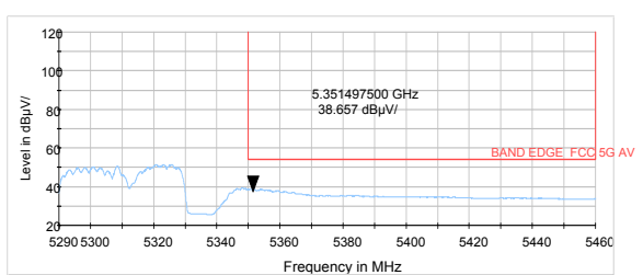
802.11ac VHT80- Channel 58: Average
