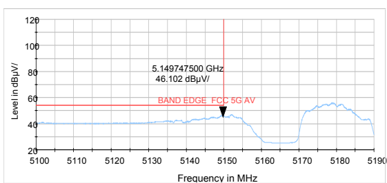
802.11n HT20-Channel 36: Average
