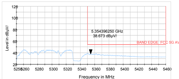
802.11ax HE80- Channel 58: Average
