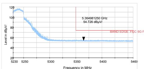
802.11ax HE20 -Channel 48: Peak
