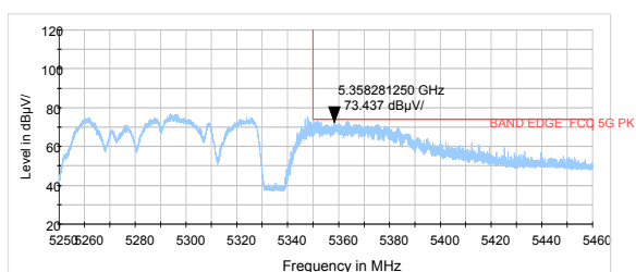
802.11ax HE80 -Channel 58: Peak
