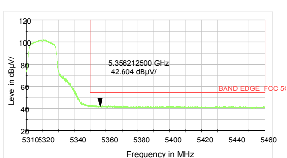
802.11n HT20-Channel 64: Peak
