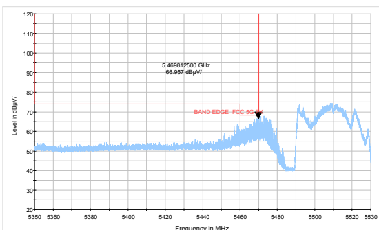
802.11ax HE40-Channel 102: Peak
