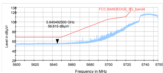
802.11ax HE20-Channel 149: Peak
