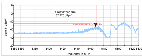
802.11ax HE40-Channel 102: Peak
