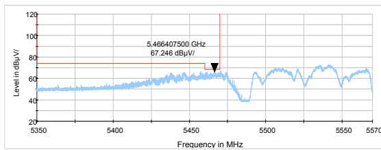
802.11ac VHT80 -Channel 106: Peak
