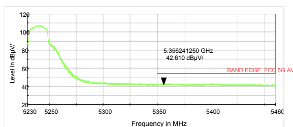
802.11a-Channel 48: Average
