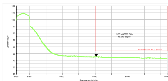
802.11ax HE20 -Channel 48: Average
