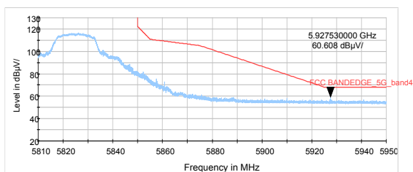
802.11n HT20-Channel 165: Peak
