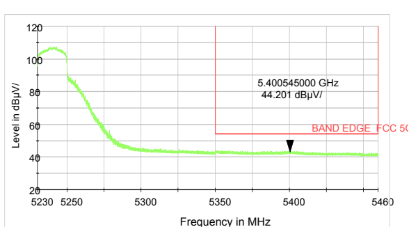
802.11ax HE20 -Channel 48: Average
