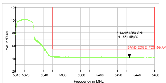
802.11n HT20-Channel 64: Average
