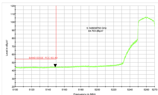
802.11ax HE20-Channel 52: Average
