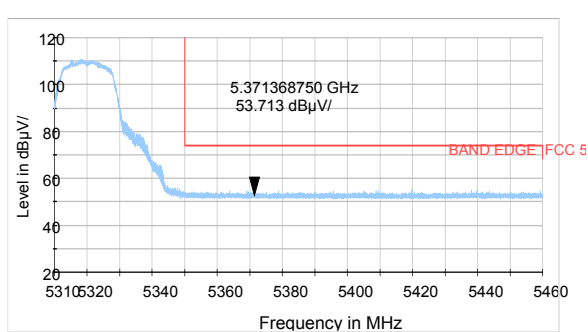
802.11a-Channel 64: Average
