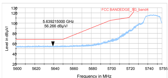
802.11n HT20-Channel 149: Peak
