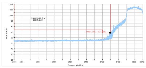
802.11ax HE20-Channel 100: Average
