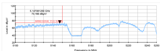
802.11ax HE80 -Channel 42: Peak
