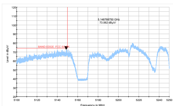
802.11ax HE80 -Channel 42: Peak
