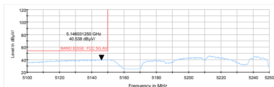
802.11ax HE80- Channel 42: Average
