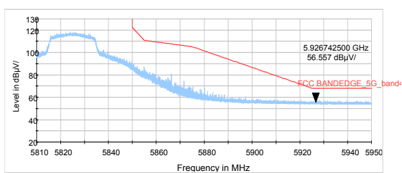
802.11ax HE20-Channel 165: Peak
