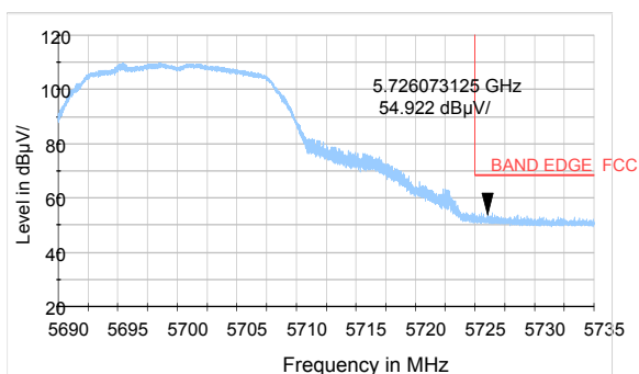
802.11a-Channel 140: Peak
