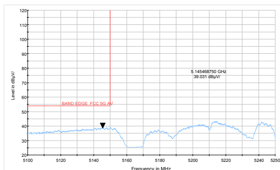
802.11ax HE80- Channel 42: Average
