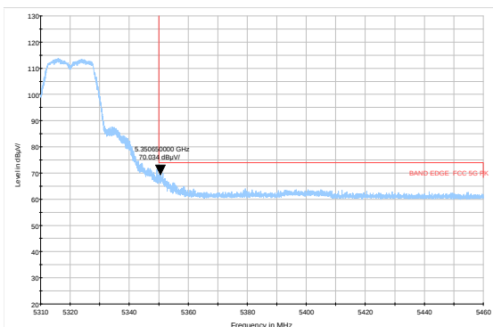
802.11a-Channel 64: Average
