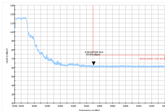
802.11a-Channel 48: Average
