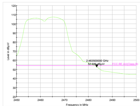
802.11g-Channel 11 Average
