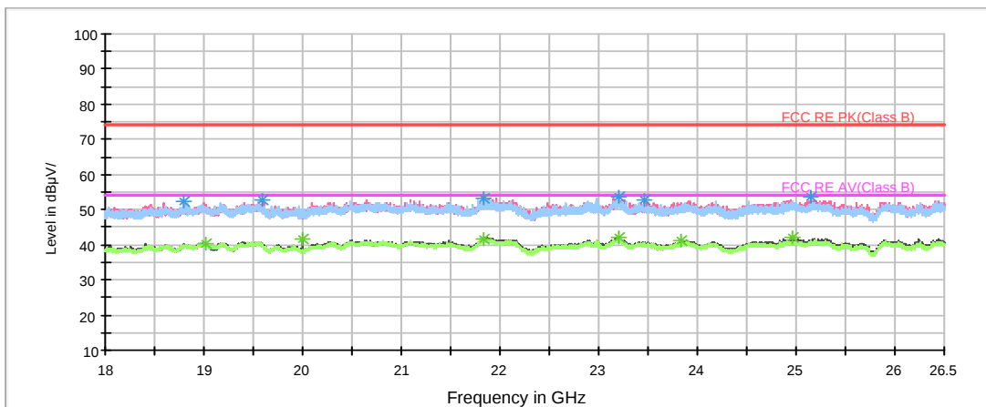
BELL_RE 18-26.5GHz PK+AV
