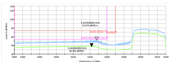
802.11ac VHT80-Channel 106: Peak+Average
