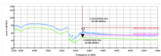
802.11ax HE80-Channel 58: Peak+ Average
