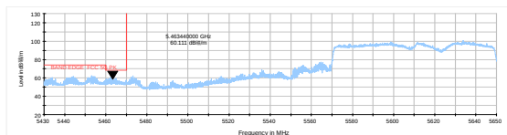
802.11ax HE80-Channel 122: Peak
