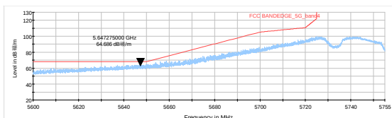
802.11n HT40-Channel 151: Peak
