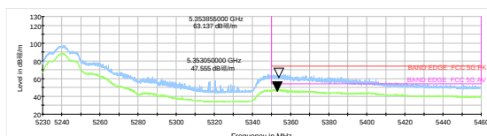
802.11n HT40-Channel 46: Peak+ Average
