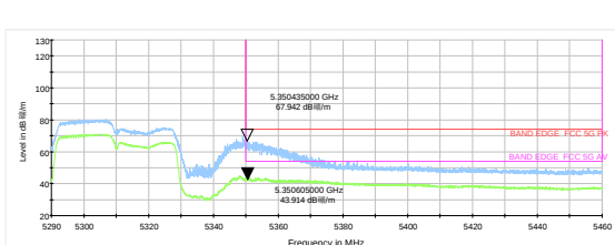
802.11ax HE20-Channel 52: Peak+ Average
