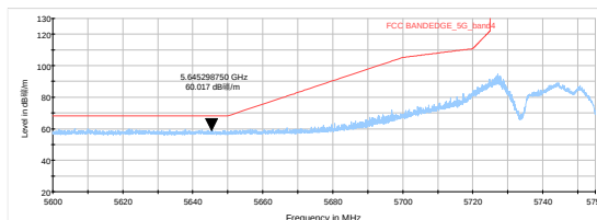
802.11ax HE20-Channel 149: Peak
