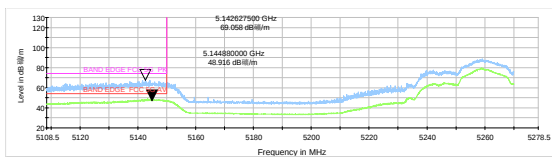
802.11n HT20-Channel 52: Peak+ Average
