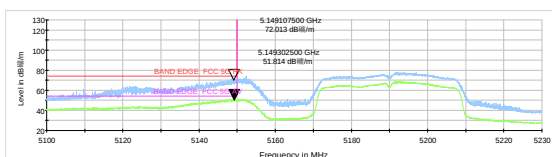
802.11ac VHT80 -Channel 42: Peak
