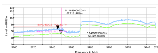
802.11ax HE80-Channel 42: Peak+ Average
