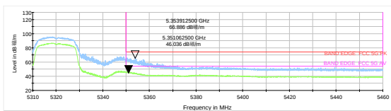
802.11n HT20-Channel 64: Peak+ Average
