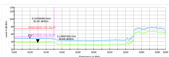
802.11ax HE80-Channel 58: Peak+ Average
