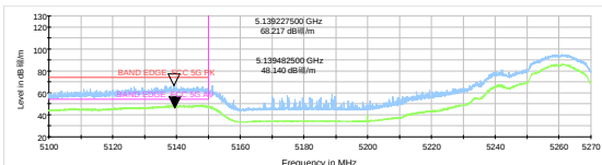
802.11n HT40-Channel 54: Peak+ Average
