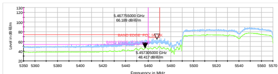
802.11ax HE80-Channel 106: Peak+Average
