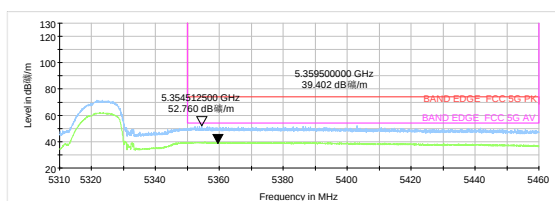
802.11n HT40-Channel 62: Peak+ Average
