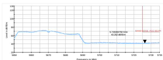
802.11ac VHT80-Channel 122: Peak
