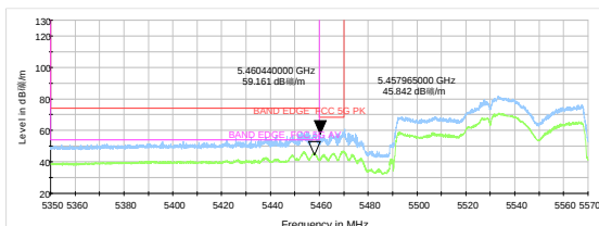
802.11ax HE20-Channel 100: Peak+ Average
