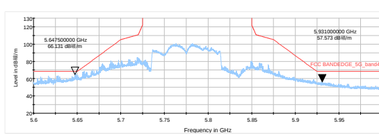
802.11ax HE80-Channel 155: Peak
