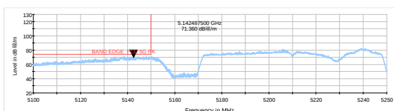
802.11ax HE20-Channel 36: Peak+ Average
