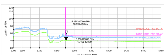
802.11ax HE40-Channel 62: Peak+ Average
