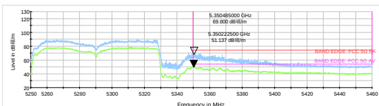
802.11ax HE20-Channel 64: Peak+ Average
