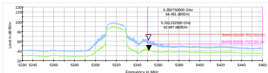
802.11n HT40-Channel 62: Peak+ Average
