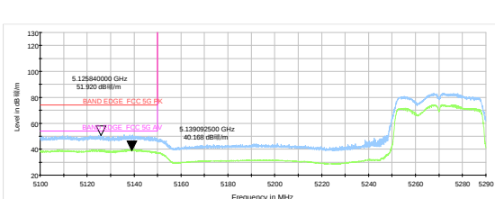
802.11ac VHT80 -Channel 58: Peak+ Average
