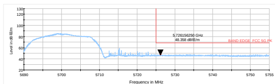
802.11n HT20-Channel 140: Peak
