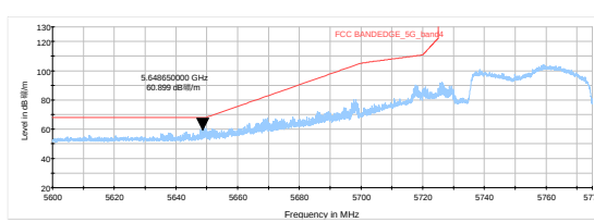
802.11ax HE40-Channel 151: Peak
