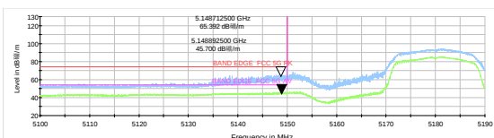
802.11n HT20-Channel 36: Peak+ Average
