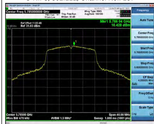
U-NII-3, 802.11a, Channel No.: 157
