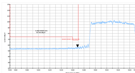
802.11ac VHT80 -Channel 106: Peak
