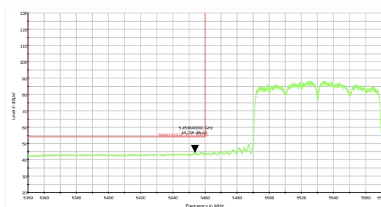
802.11ac VHT80- Channel 106: Average
