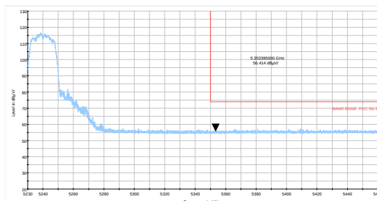
802.11a-Channel 48: Average
