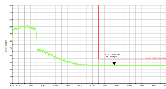
802.11ax HE40-Channel 46: Average
