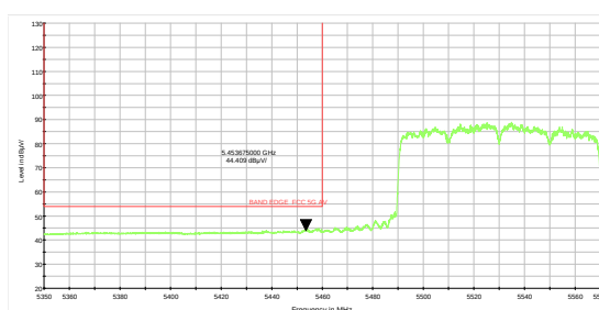
802.11ax HE80- Channel 106: Average
