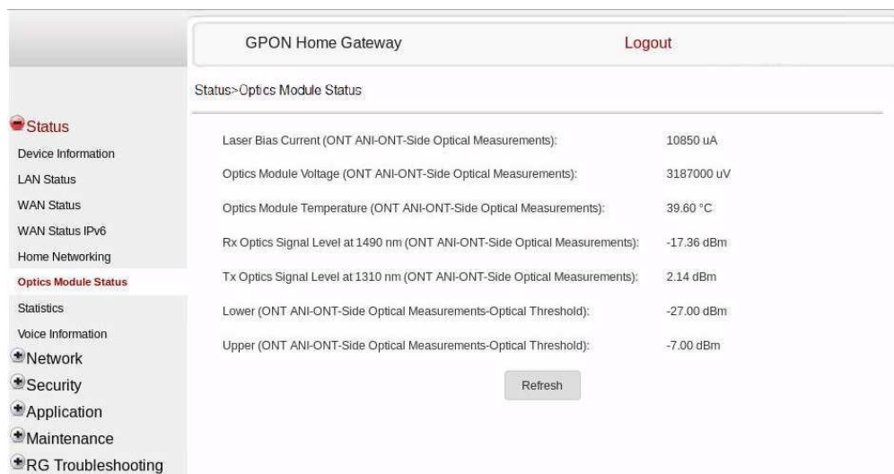
Figure 7-7 Optics module status window
