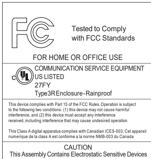
Figure 3-1 Sample safety label on the ONT equipment
