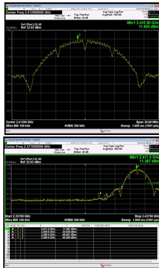
802.11g, Channel No.: 1
