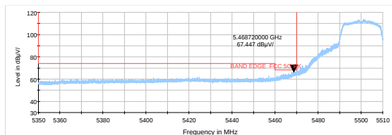
802.11ac VHT20-Channel 100: Average
