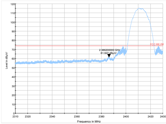
802.11b-Channel 1 Peak
