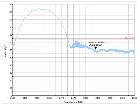
802.11b-Channel 11 Peak
