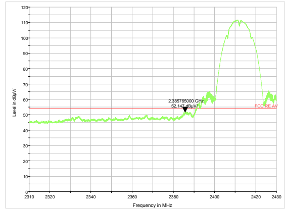
802.11g-Channel 1 Average
