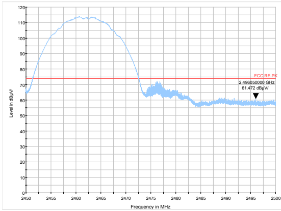
802.11g-Channel 11 Peak
