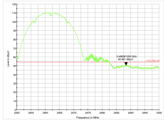
802.11g-Channel 11 Average
