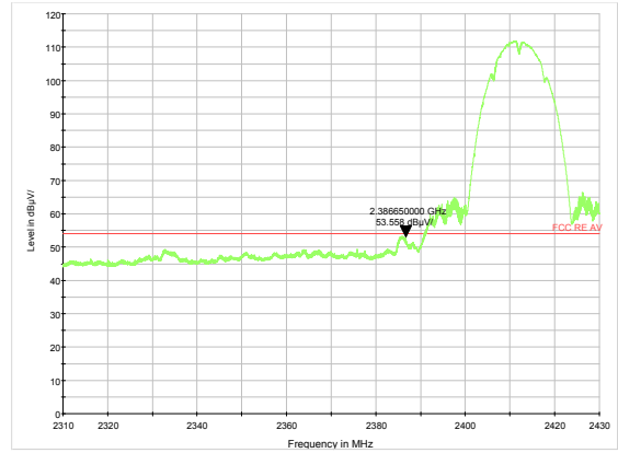
802.11b-Channel 1 Average
