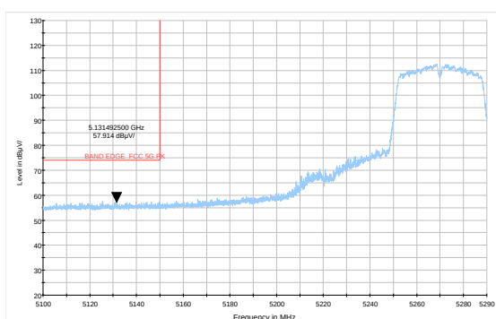
802.11n HT40-Channel 54: Peak
