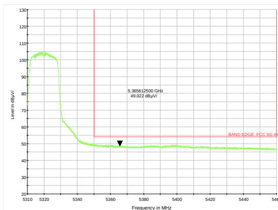
802.11a-Channel 64: Average
