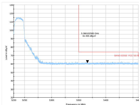
802.11a-Channel 48: Average
