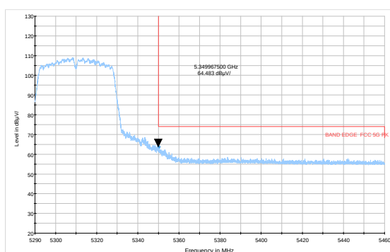
802.11n HT40-Channel 62: Peak
