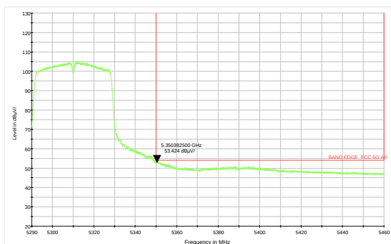
802.11ac VHT20 -Channel 64: Peak
