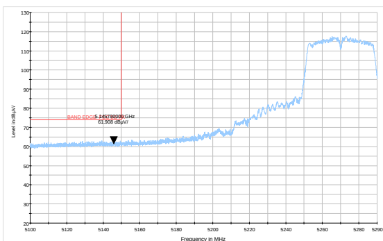
802.11ac VHT40-Channel 54: Average
