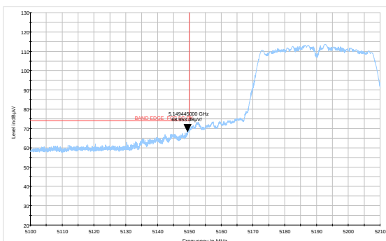
802.11ac VHT40-Channel 38: Average
