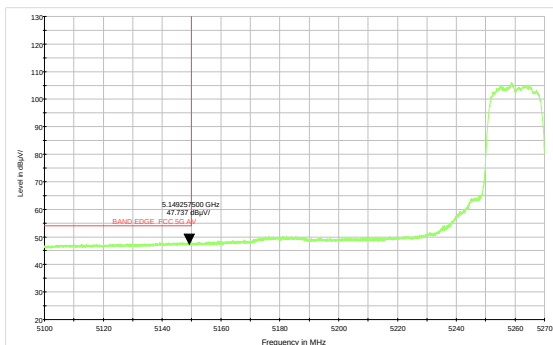
802.11ac VHT20-Channel 52: Average
