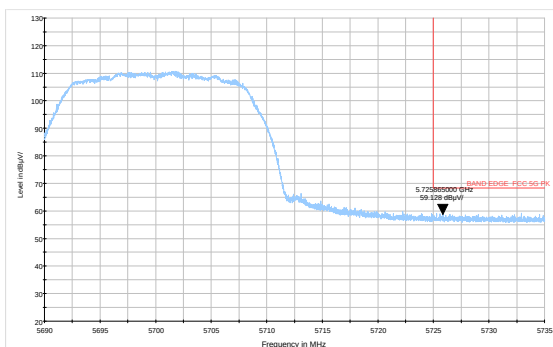
802.11a-Channel 140: Peak
