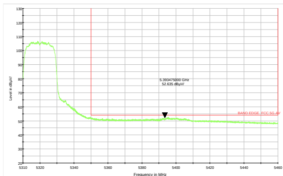
802.11ac VHT20 -Channel 64: Average
