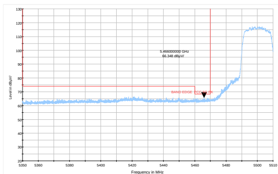
802.11ac VHT20-Channel 100: Average
