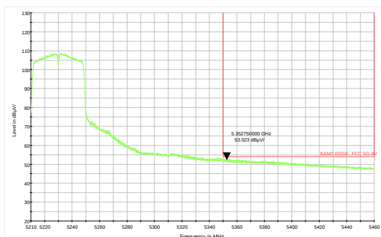
802.11ac VHT20 -Channel 48: Peak
