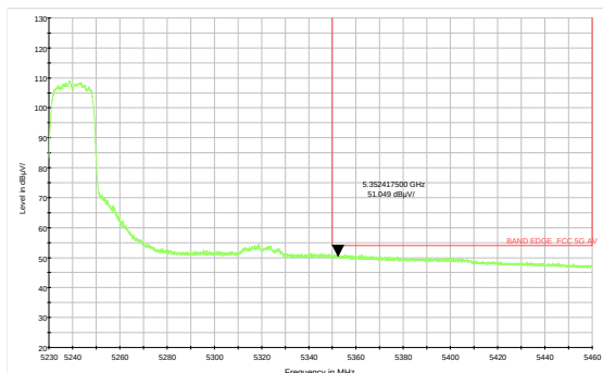
802.11ac VHT20 -Channel 48: Average
