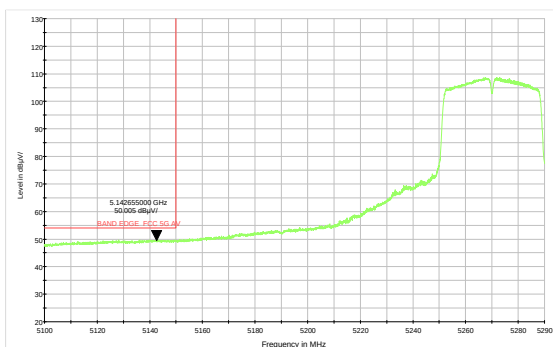
802.11ac VHT20 -Channel 52: Peak
