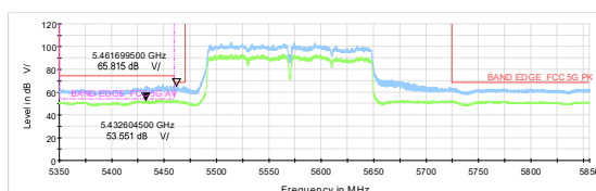
802.11ac VHT160- Channel 114: Peak
