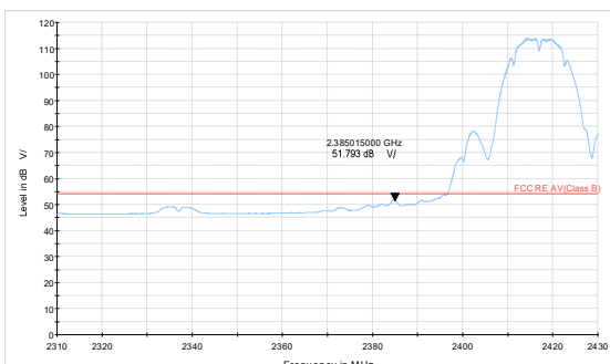
802.11b-Channel 2 Average
