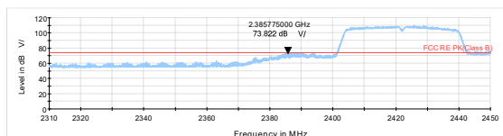
802.11n HT40-Channel 3 Peak
