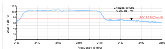
802.11n HT40-Channel 9 Peak
