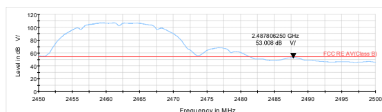
802.11n HT20-Channel 11 Average
