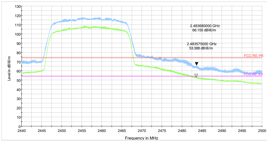
802.11ax HE 20 CH10
