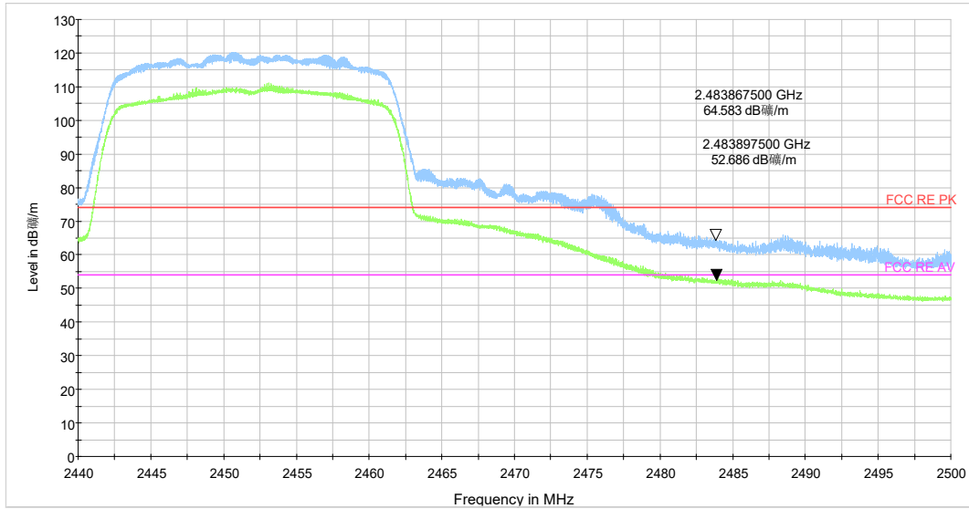
802.11ax HE 20 CH9
