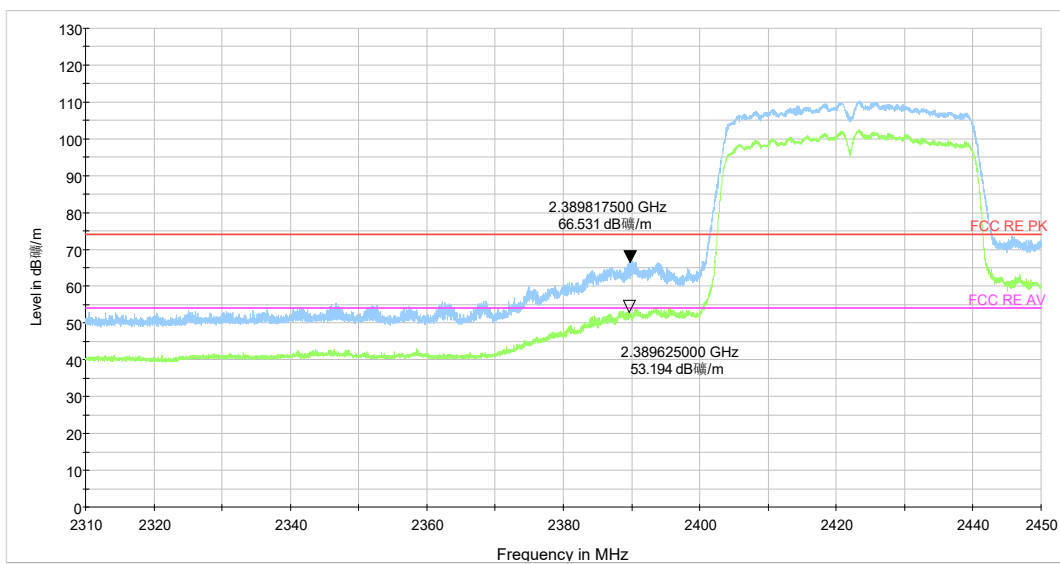
802.11n (HT40) CH3
