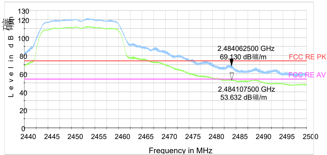
802.11g CH9
