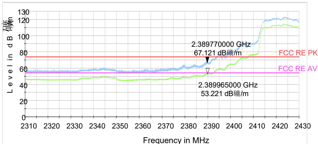
802.11g CH3
