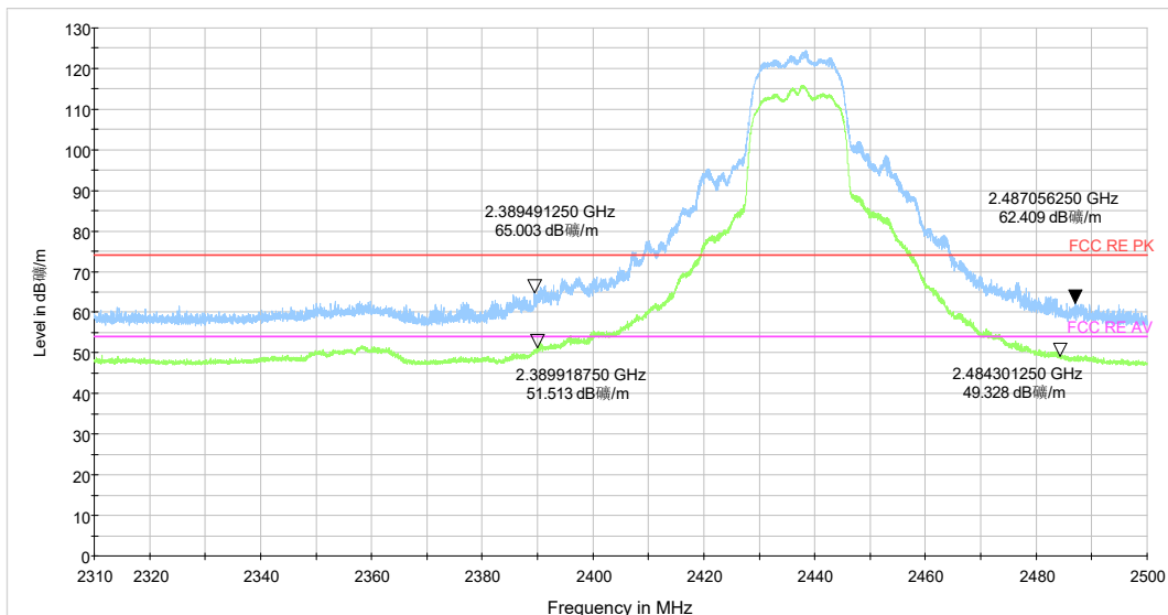
802.11g CH6
