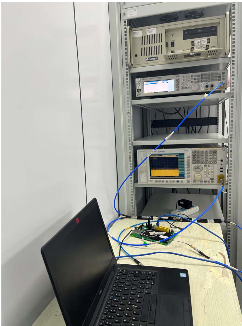
Picture 1 DFS Test Setup
