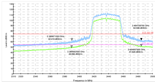
802.11n HT40-Channel 6 Peak+ Average
