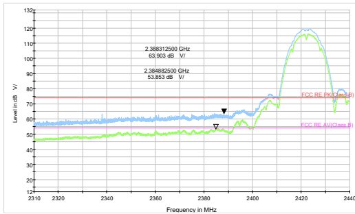
802.11b-Channel 3 Peak+ Average
