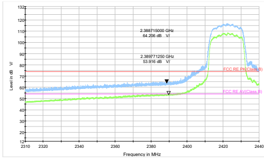
802.11n HT20-Channel 3 Peak+ Average
