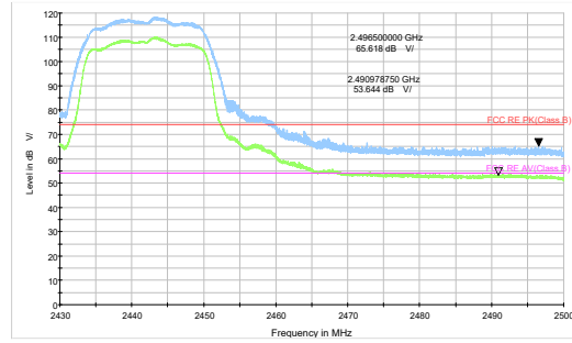
802.11g-Channel 7 Peak+ Average
