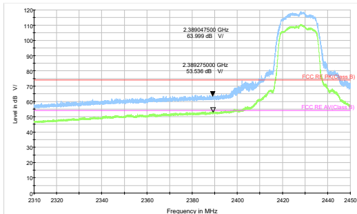
802.11g-Channel 4 Peak+ Average
