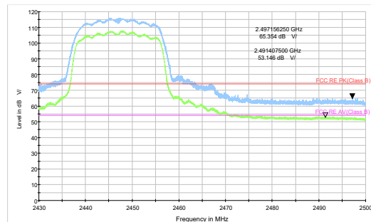
802.11n HT20-Channel 8 Peak+ Average
