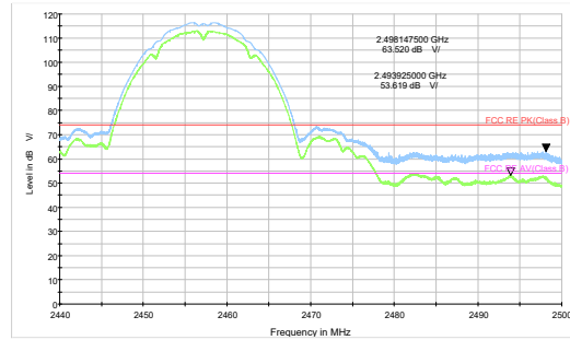
802.11b-Channel 10 Peak+ Average
