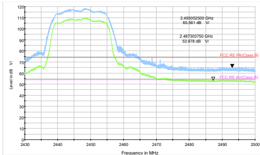
802.11g-Channel 8 Peak+ Average
