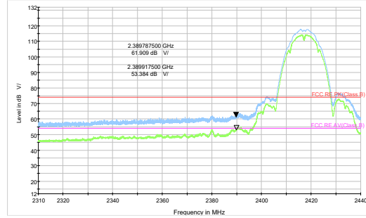
802.11b-Channel 2 Peak+ Average
