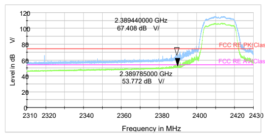
802.11g-Channel 1 Peak+ Average
