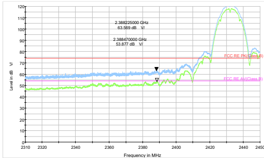
802.11b-Channel 5 Peak+ Average
