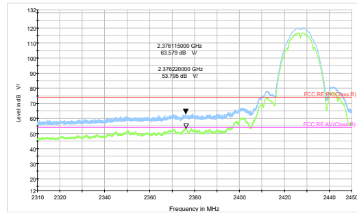
802.11b-Channel 4 Peak+ Average
