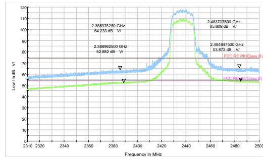
802.11n HT20-Channel 6 Peak+ Average
