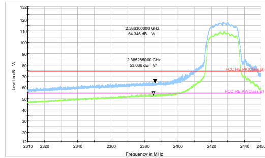
802.11n HT20-Channel 4 Peak+ Average
