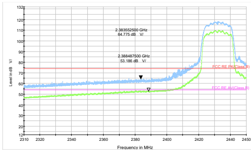
802.11n HT20-Channel 5 Peak+ Average
