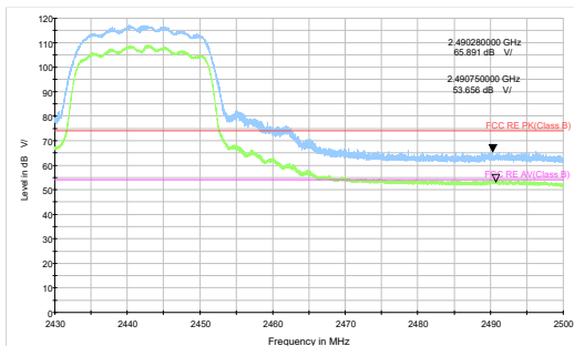
802.11n HT20-Channel 7 Peak+ Average
