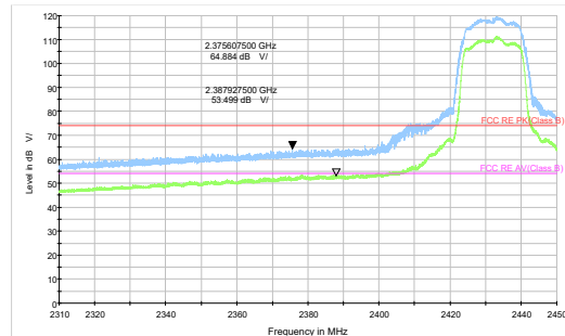
802.11g-Channel 5 Peak+ Average
