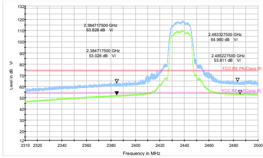
802.11g-Channel 6 Peak+ Average
