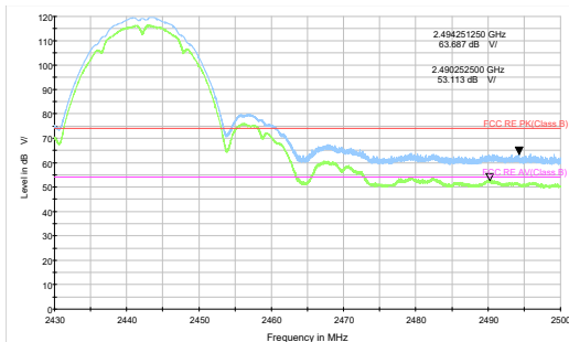
802.11b-Channel 7 Peak+ Average
