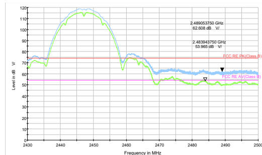
802.11b-Channel 8 Peak+ Average
