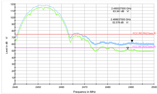
802.11b-Channel 9 Peak+ Average
