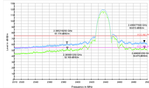
802.11b-Channel 6 Peak+ Average
