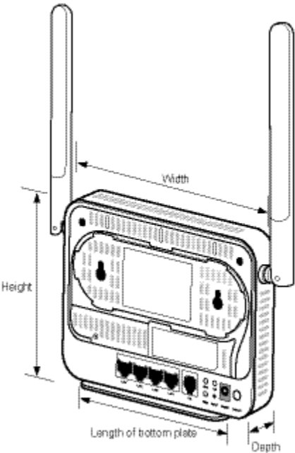
Figure 5-5 ONT physical specifications
