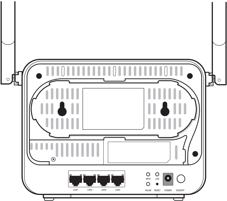
Figure 5-2 G-0425G-C indoor ONT physical connections (back)
