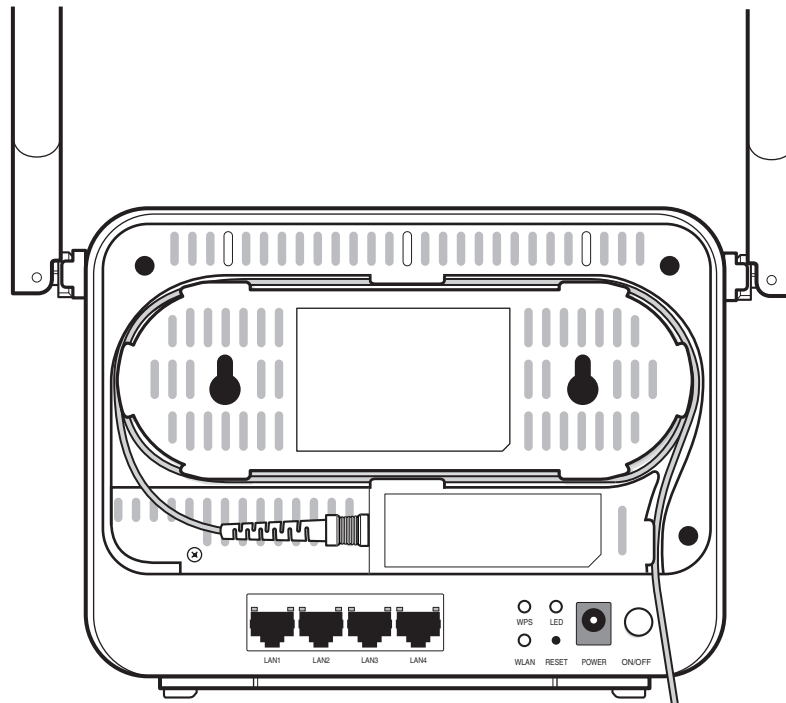
Figure 5-3 G-0425G-C indoor ONT with fiber optic connector
