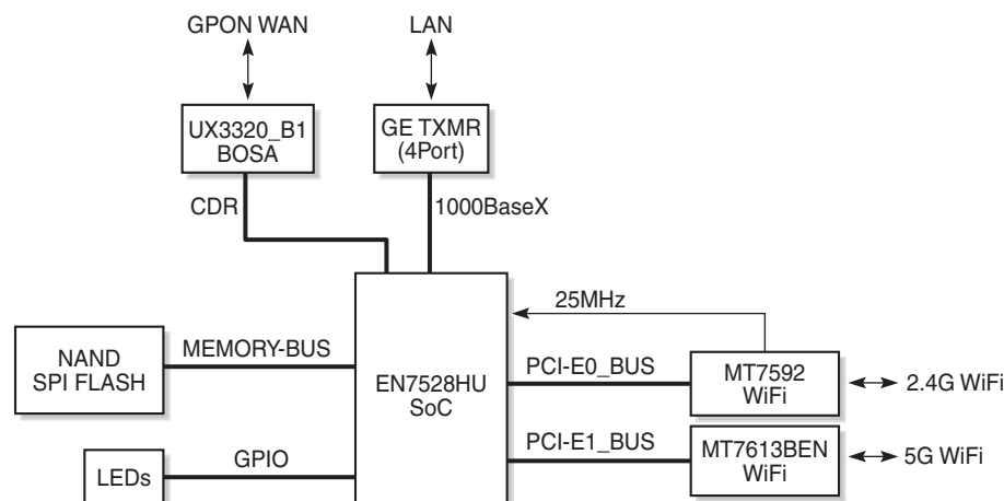
Figure 5-6 G-0425G-C ONT functional block
