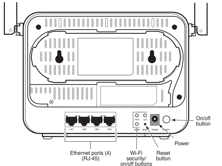
Figure 6-1 G-0425G-C ONT connections
