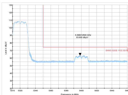
802.11a-Channel 64: Peak
