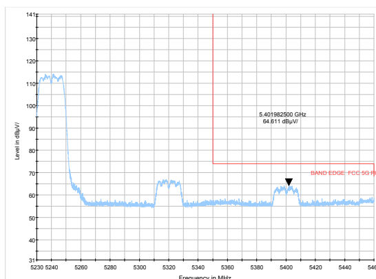
802.11a-Channel 48: Average
