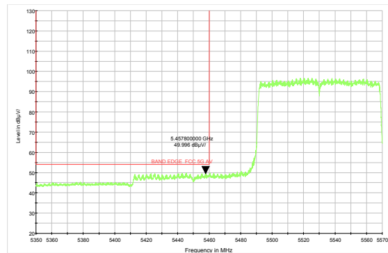
802.11ac VHT80- Channel 106: Average
