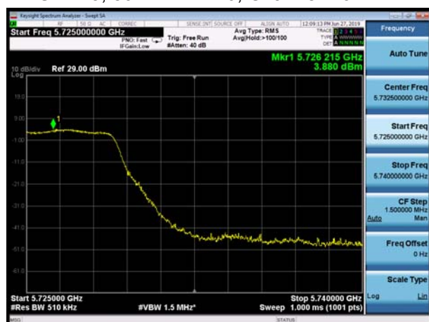
U-NII-3, 802.11ac VHT20, Channel No.: 144
