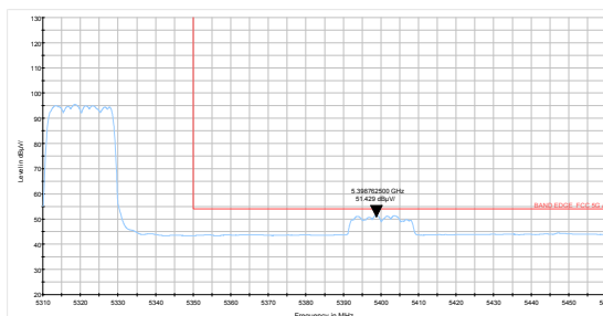
802.11a-Channel 64: Average
