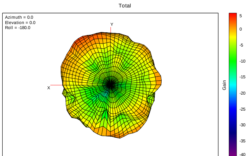
3D Free Space Router Gain Pattern 6G-6-6435MHz
