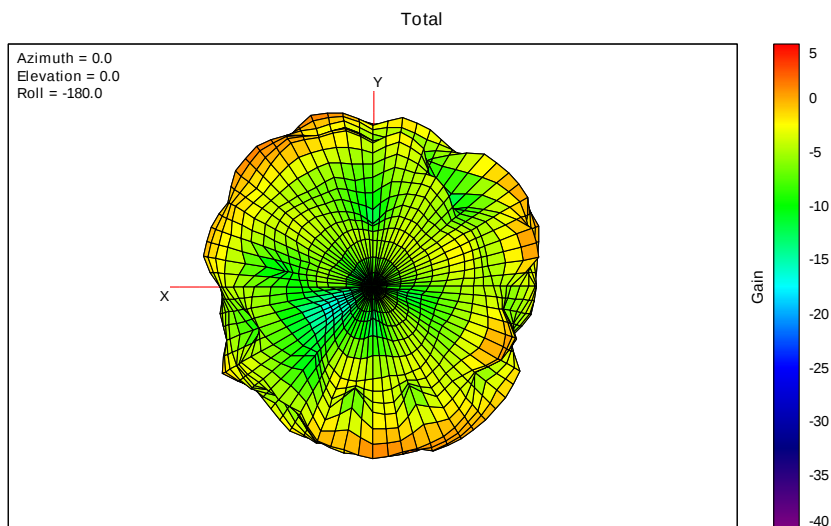
3D Free Space Router Gain Pattern 6G-6-5955MHz
