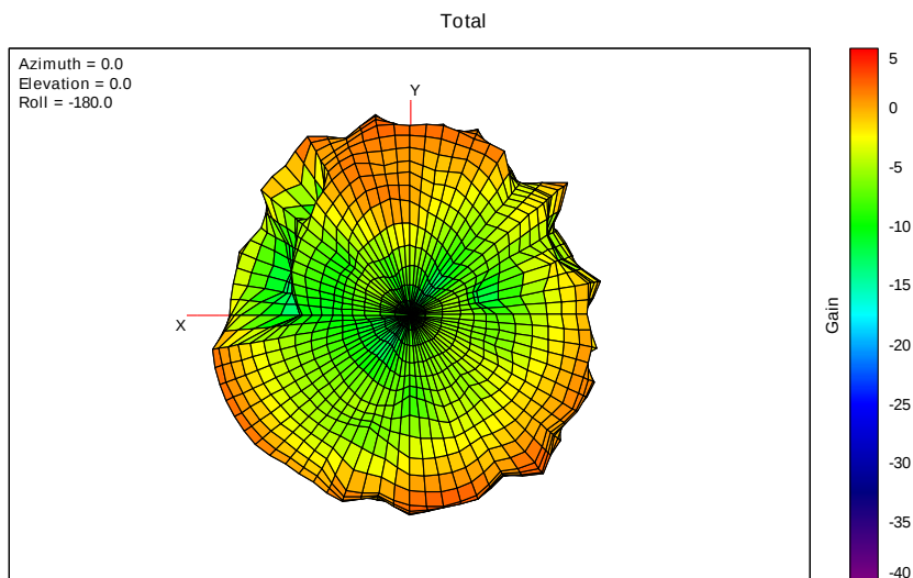
3D Free Space Router Gain Pattern 6G-7-6695MHz
