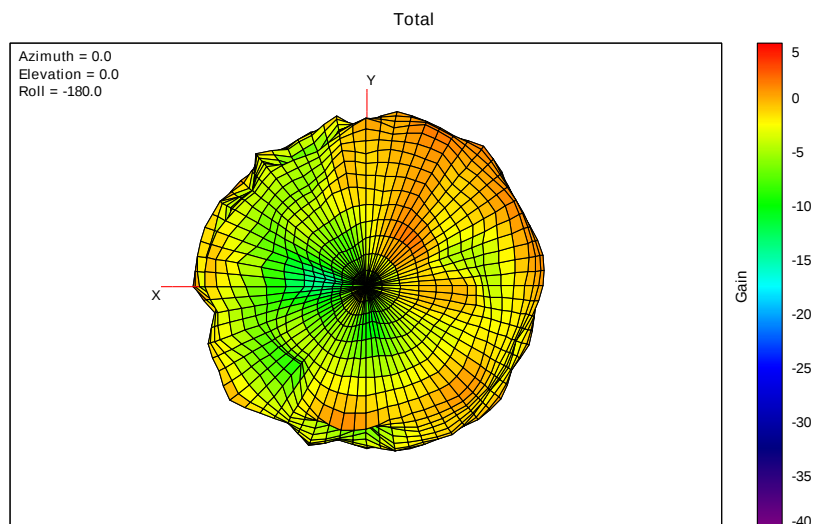
3D Free Space Router Gain Pattern 6G-8-6435MHz
