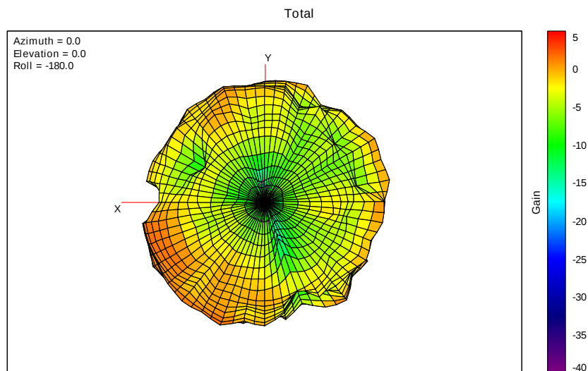
3D Free Space Router Gain Pattern 6G-5-7095MHz
