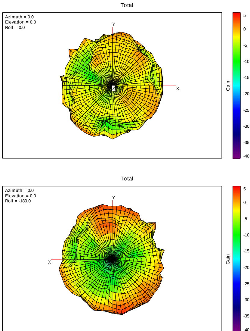
3D Free Space Router Gain Pattern 6G-7-6875MHz
