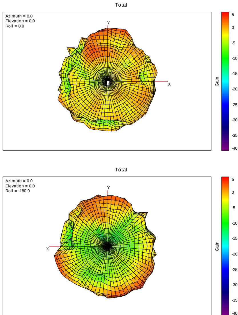
3D Free Space Router Gain Pattern 6G-7-6535MHz
