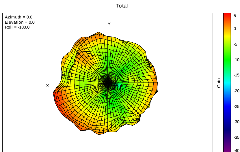
3D Free Space Router Gain Pattern 6G-5-6435MHz
