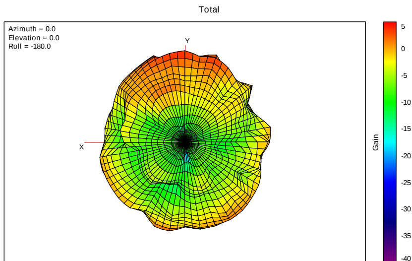
3D Free Space Router Gain Pattern 6G-7-5955MHz
