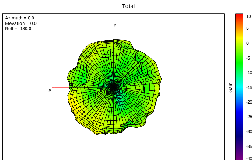
3D Free Space Router Gain Pattern 6G-5-6995MHz
