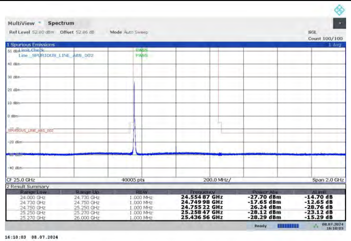
n258-b 200MHz-QPSK-Low -V-128RB0
