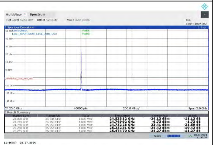
n258-b 50MHz-64QAM -Low -V-32RB0
