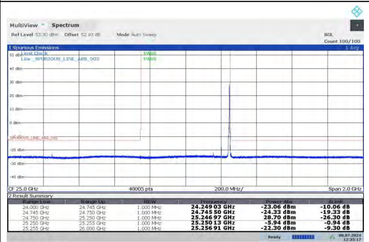
n258-b 50MHz-QPSK- High -V-1RB31
