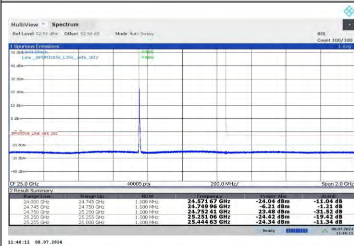
n258-b 50MHz-64QAM -Low -H-32RB0
