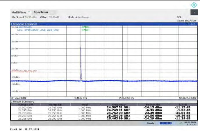
n258-b 50MHz-QPSK-Low -V-1RB0
