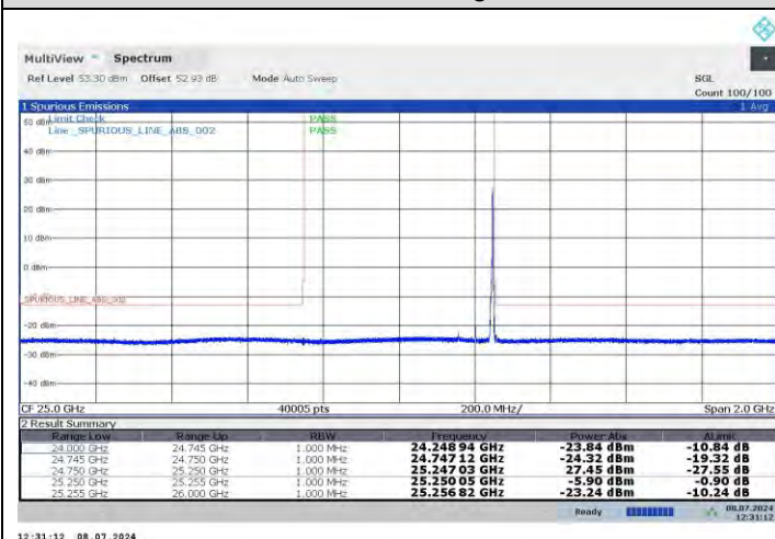
n258-b 50MHz-BPSK-High -H-1RB31
