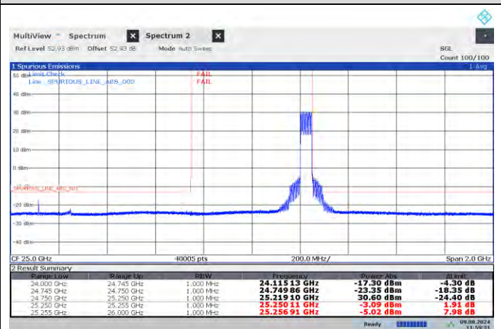
n258-b 50MHz-QPSK- High -V-32RB0
