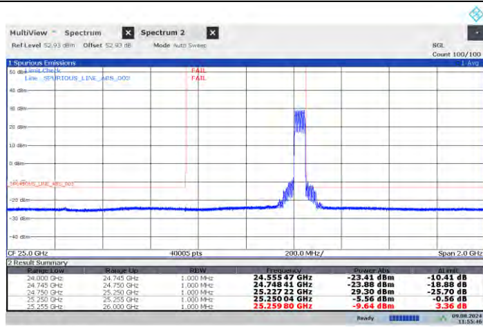
n258-b 50MHz-BPSK- High -H-32RB0
