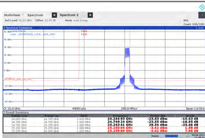
n258-b 50MHz-QPSK- High -H-32RB0
