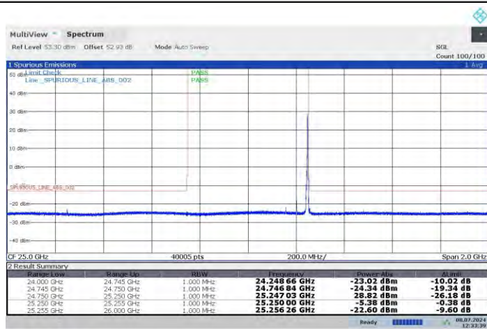
n258-b 50MHz-QPSK- High -H-1RB31
