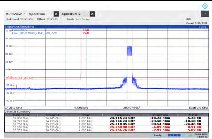
n258-b 50MHz-BPSK- High -V-32RB0
