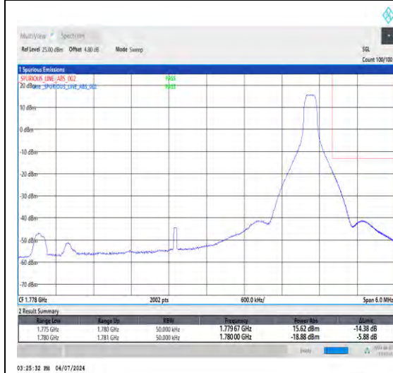
1-N66-15-5-H-5-CP-QPSK-Edge_1RB_Right-1@24-Ant1-1-seegraph-PASS-see graph
