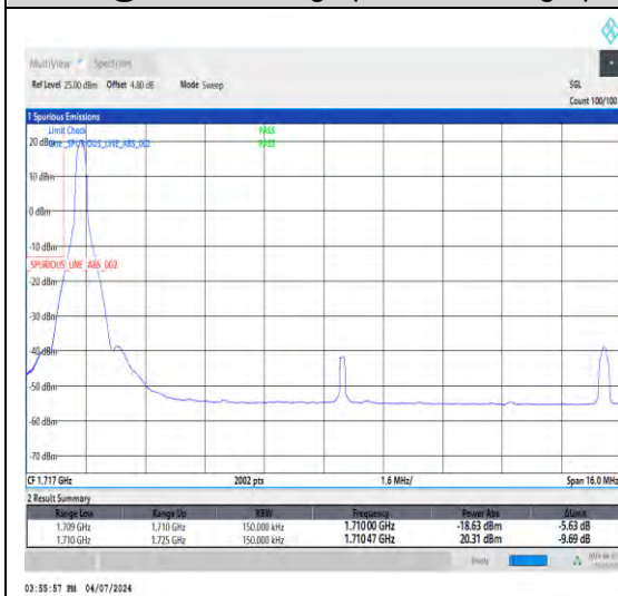
1-N66-15-15-L-4-CP-QPSK-Edge_1RB_Left-1@0-Ant1-1-seegraph-PASS-see graph
