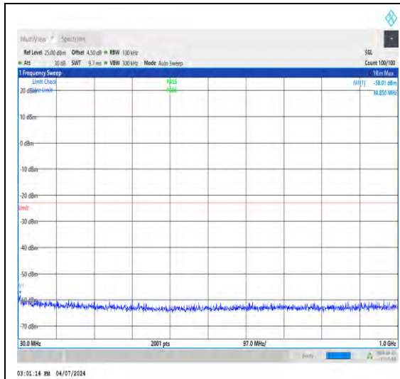
1-N66-15-40-H-1-DFT-PI2BPSK-Inner_1RB_ Left-1@1-30-1000-Ant1-34.85--58.01--23-PA SS
