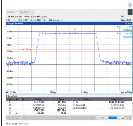
1-N66-15-15-M-1-DFT-QPSK-Outer_Full-75 @0-Ant1-13.486-14.700≤15-PASS
