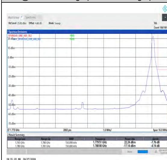
1-N66-15-15-H-2-DFT-PI2BPSK-Edge_1RB
