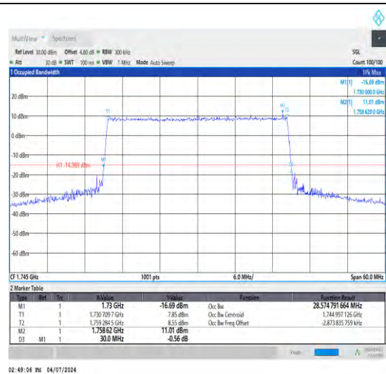
1-N66-15-30-M-9-CP-256QAM-Outer_Full-16 0@0-Ant1-28.575-30.000-≤30-PASS
