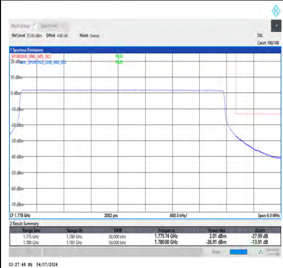
1-N66-15-5-H-6-CP-QPSK-Outer_Full-25@0-Ant1-1-seegraph-PASS-see graph
