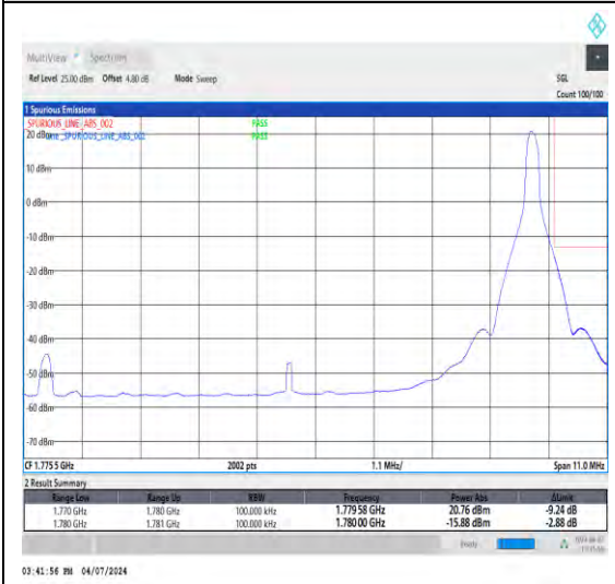
1-N66-15-10-H-2-DFT-PI2BPSK-Edge_1RB_Right-1@51-Ant1-1-seegraph-PASS-see graph
