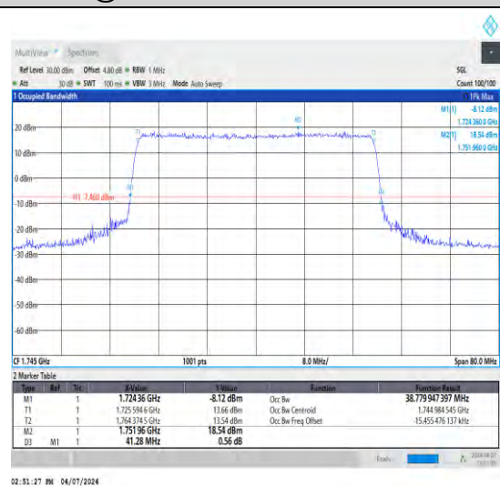
1-N66-15-40-M-4-DFT-64QAM-Outer_Full-21 6@0-Ant1-38.78-41.280-≤40-PASS
