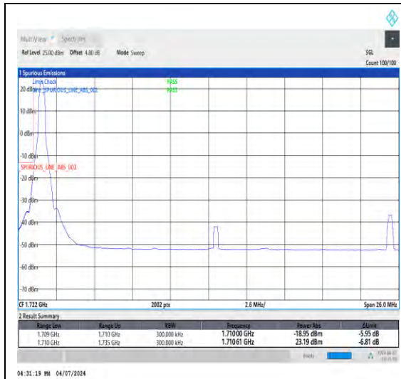
1-N66-15-25-L-1-DFT-PI2BPSK-Edge_1RB_Left-1@0-Ant1-1-seegraph-PASS-see graph
