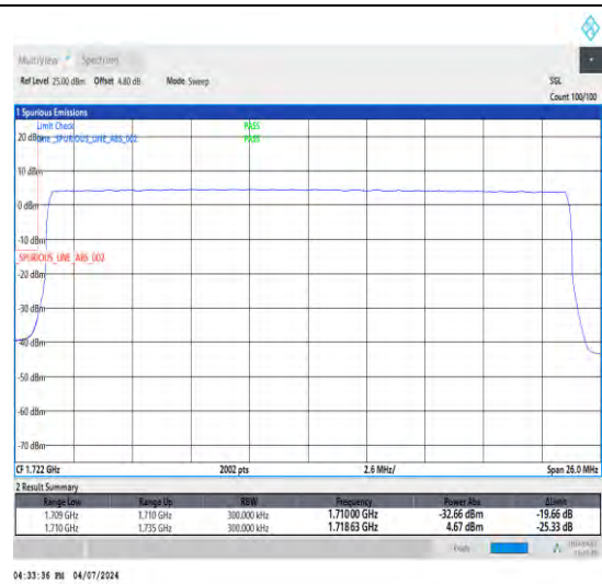
1-N66-15-25-L-3-DFT-PI2BPSK-Outer_Full-128@0-Ant1-1-seegraph-PASS-see graph
