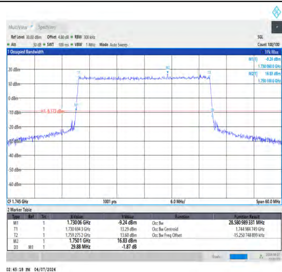
1-N66-15-30-M-1-DFT-QPSK-Outer_Full-160 @0-Ant1-28.581-29.880-≤30-PASS
