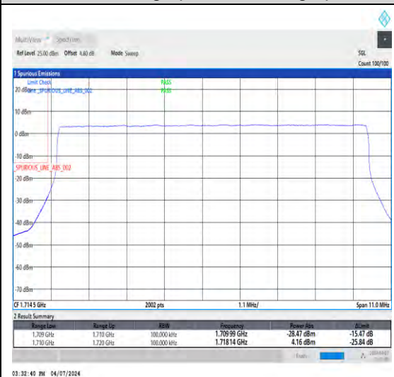
1-N66-15-10-L-3-DFT-PI2BPSK-Outer_Full-5@0-Ant1-1-seegraph-PASS-see graph
