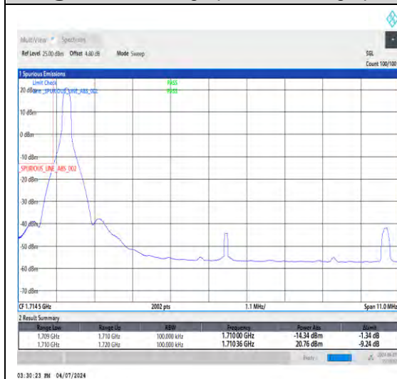
1-N66-15-10-L-1-DFT-PI2BPSK-Edge_1RB_Left-1@0-Ant1-1-seegraph-PASS-see graph
