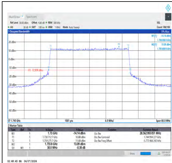
1-N66-15-30-M-8-CP-64QAM-Outer_Full-160 @0-Ant1-28.563-30.000-≤30-PASS
