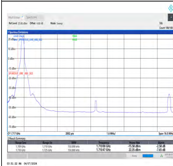
1-N66-15-15-L-1-DFT-PI2BPSK-Edge_1RB_Left-1@0-Ant1-1-seegraph-PASS-see graph
