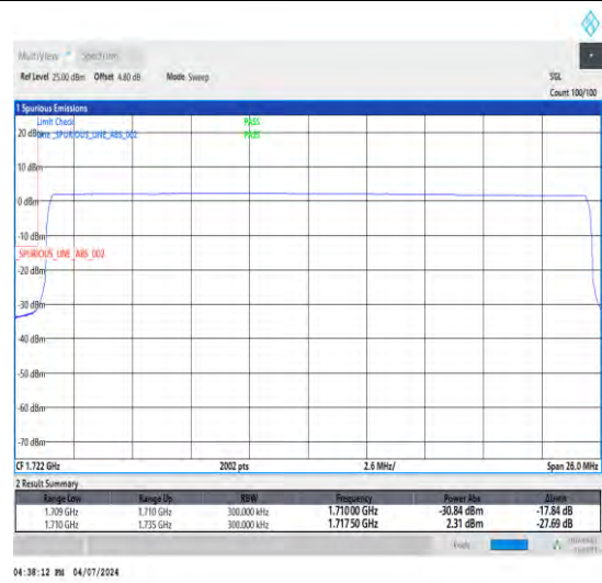
1-N66-15-25-L-6-CP-QPSK-Outer_Full-133@0-Ant1-1-seegraph-PASS-see graph
