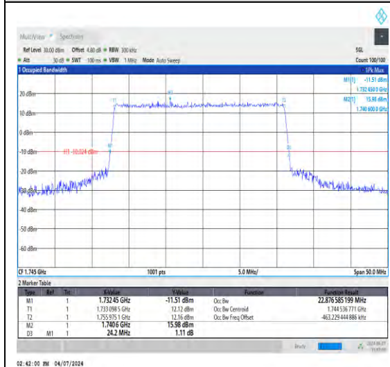
1-N66-15-25-M-3-DFT-16QAM-Outer_Full-12 8@0-Ant1-22.877-24.200-<25-PASS
