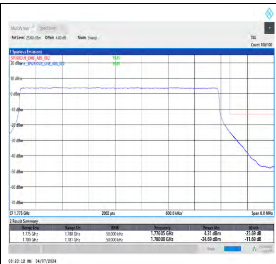
1-N66-15-5-H-3-DFT-PI2BPSK-Outer_Full-25@0-Ant1-1-seegraph-PASS-see graph
