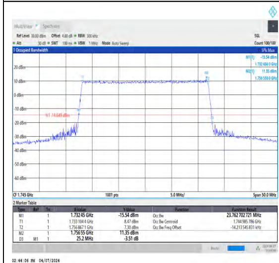
1-N66-15-25-M-9-CP-256QAM-Outer_Full-13 3@0-Ant1-23.763-25.200-≤25-PASS
