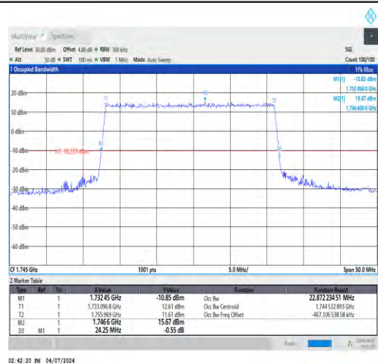
1-N66-15-25-M-4-DFT-64QAM-Outer_Full-12 8@0-Ant1-22.872-24.250-<25-PASS
