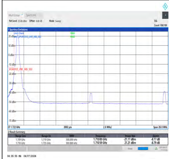
1-N66-15-25-L-4-CP-QPSK-Edge_1RB_Left-1@0-Ant1-1-seegraph-PASS-see graph
