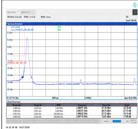
1-N41-30-50-L-4-CP-QPSK-Edge_1RB_Left- 1@0-Ant1-1--PASS-see graph
