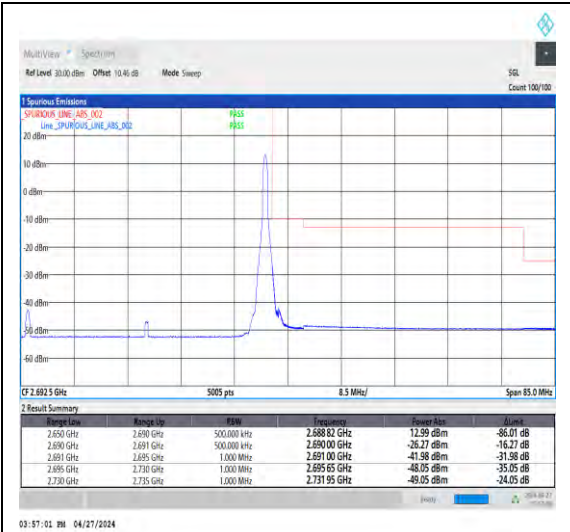
1-N41-30-40-H-2-DFT-PI2BPSK-Edge_1RB_Right-1@105-Ant1-1--PASS-see graph
