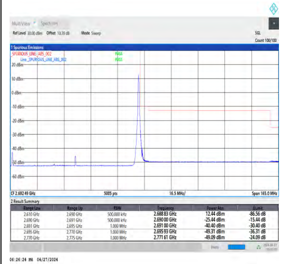
1-N41-30-80-H-5-CP-QPSK-Edge_1RB_Right-1@216-Ant1-1--PASS-see graph
