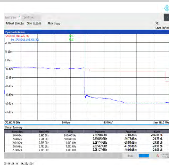
1-N41-30-90-H-6-CP-QPSK-Outer_Full-245@0-Ant1-1--PASS-see graph
