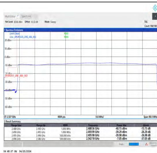
1-N41-30-90-L-6-CP-QPSK-Outer_Full-245@0-Ant1-1--PASS-see graph
