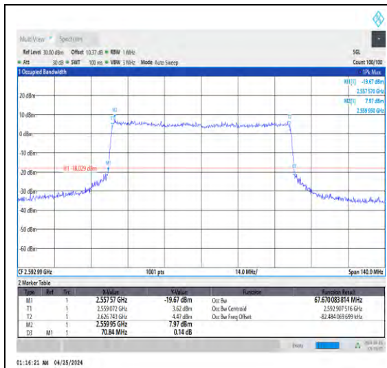
1-N41-30-70-M-8-CP-64QAM-Out_ Full-189 @0-Ant1-67.67-70.840-≤70-PASS
