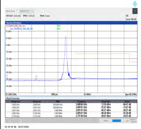
1-N41-30-40-H-5-CP-QPSK-Edge_1RB_Right-1@105-Ant1-1--PASS-see graph
