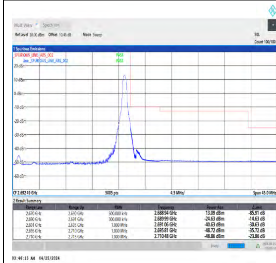
1-N41-30-20-H-5-CP-QPSK-Edge_1RB_Right-1@50-Ant1-1--PASS-see graph
