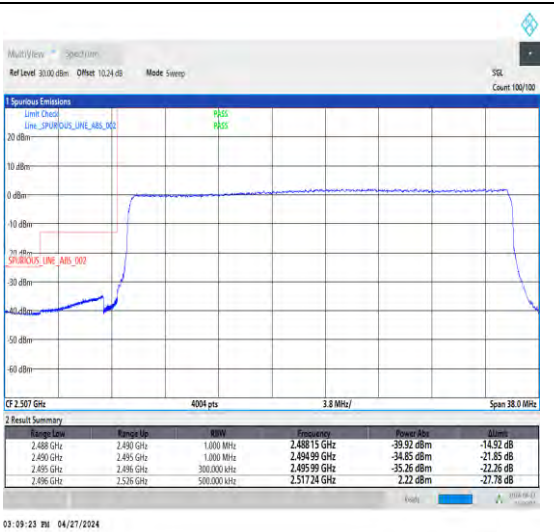
1-N41-30-30-L-3-DFT-PI2BPSK-Outer_Full-7 5@0-Ant1-1--PASS-see graph
