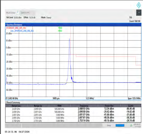
1-N41-30-60-H-5-CP-QPSK-Edge_1RB_Right-1@161-Ant1-1--PASS-see graph
