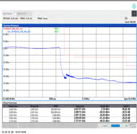
1-N41-30-30-H-3-DFT-PI2BPSK-Outer_Full-75@0-Ant1-1--PASS-see graph
