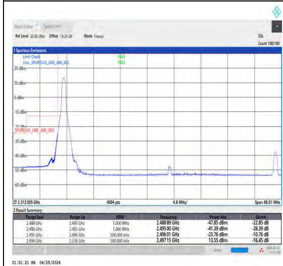
1-N41-30-40-L-4-CP-QPSK-Edge_1RB_Left- 1@0-Ant1-1--PASS-see graph
