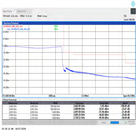
1-N41-30-30-H-6-CP-QPSK-Outer_Full-78@0-Ant1-1--PASS-see graph
