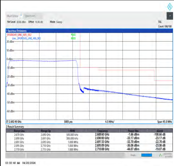
1-N41-30-20-H-6-CP-QPSK-Outer_Full-51@0-Ant1-1--PASS-see graph
