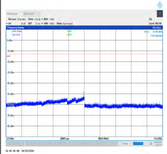
1-N2-15-40-H-1-DFT-PI2BPSK-Inner_1RB_L eft-1@1-3000-12000-Ant1-7471.65--51.95--1 3-PASS
