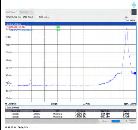
1-N2-15-20-H-5-CP-QPSK-Edge_1RB_Right -1@105-Ant1-1-seegraph-PASS-see graph
