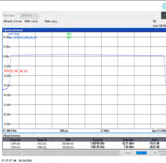
1-N2-15-30-L-6-CP-QPSK-Outer_Full-160@ 0-Ant1-1-seegraph-PASS-see graph
