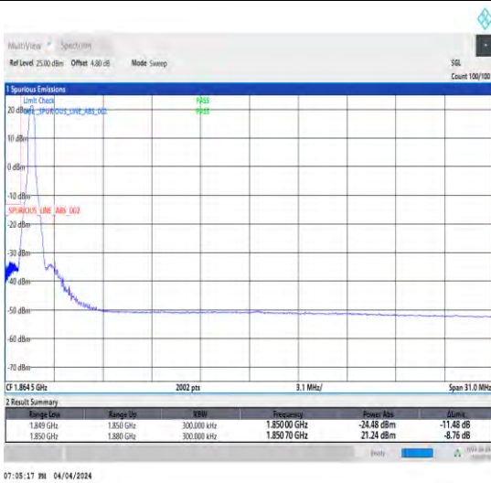
1-N2-15-30-L-4-CP-QPSK-Edge_1RB_Left-1 @0-Ant1-1-seegraph-PASS-see graph
