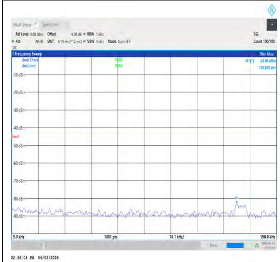
1-N2-15-40-M-1-DFT-PI2BPSK-Inner_1RB_L eft-1@1-0.009-0.15-Ant1-0.13--83.04--43-PA SS
