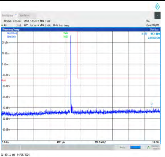
1-N2-15-40-H-1-DFT-PI2BPSK-Inner_1RB_L eft-1@1-1000-3000-Ant1-2894.50--39.76--13 -PASS
