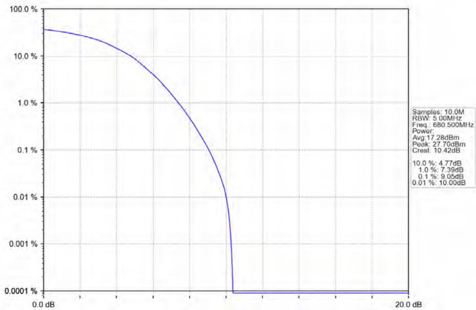
Band71_5MHz_64QAM_MCH_680.5MHz_RB_25_0_NTNV
