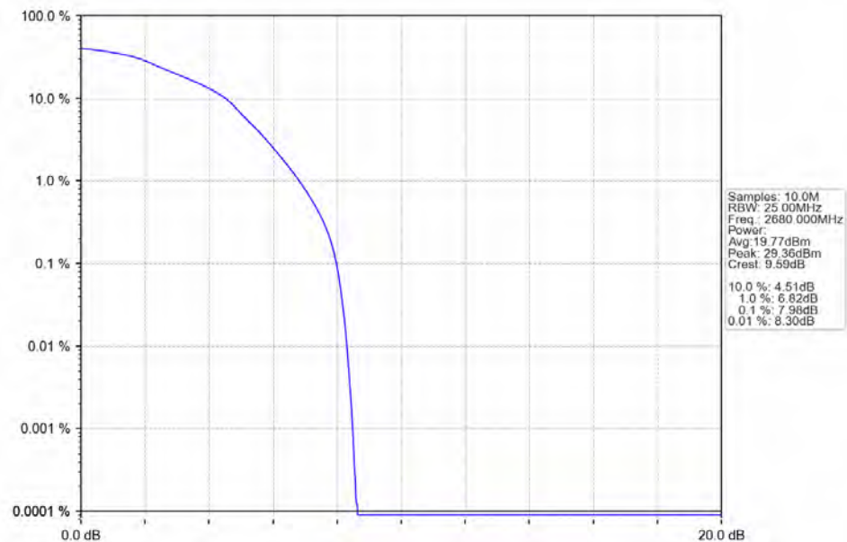
Band41_20MHz_16QAM_HCH_2680MHz_RB_100_0_NTNV
