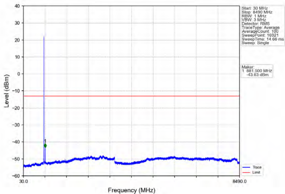
Band26b_10MHz_QPSK_MCH_836.5MHz_RB_1_0_NTNV
