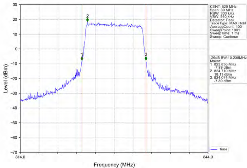
Band26b_10MHz_QPSK_LCH_829MHz_RB_50_0 NTN
