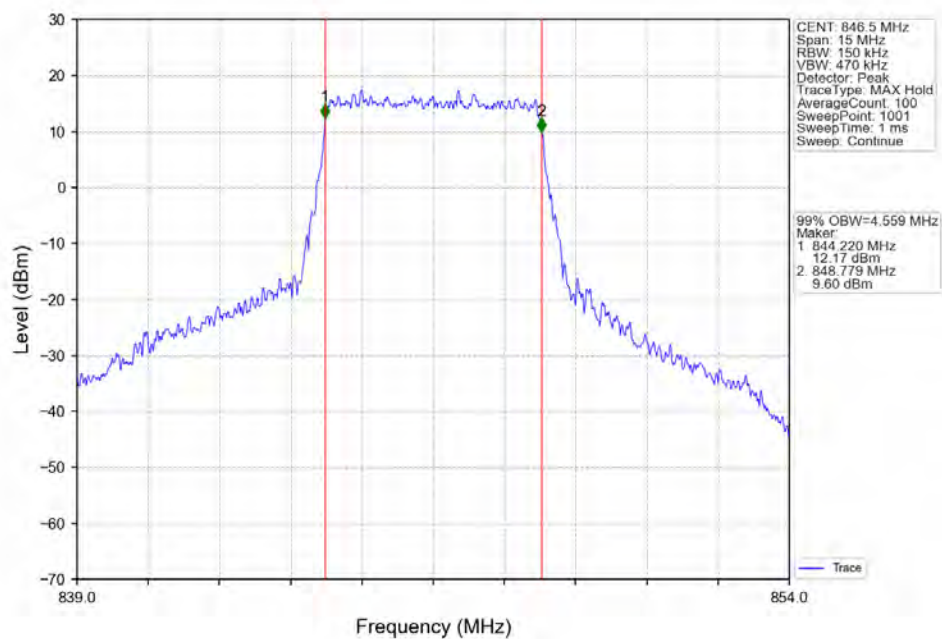
Band26b_5MHz_16QAM_HCH_846.5MHz_RB_25_0 NTN
