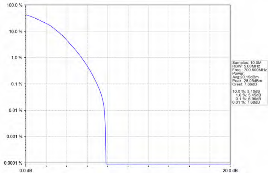
Band12_3MHz_64QAM_LCH_700.5MHz_RB_15_0_NTNV
