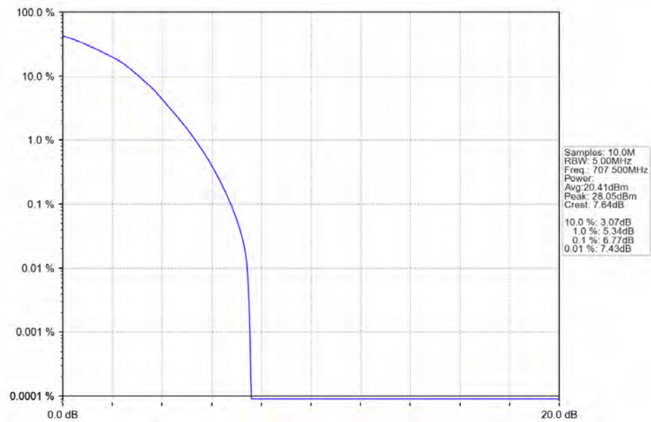
Band12_3MHz_64QAM_MCH_707.5MHz_RB_15_0_NTNV
