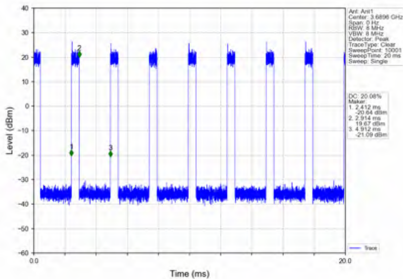
n78d_30kHz_SISO_NTNV_20MHz_CP-OFDM_16 QAM_3690MHz_Inner_Full
