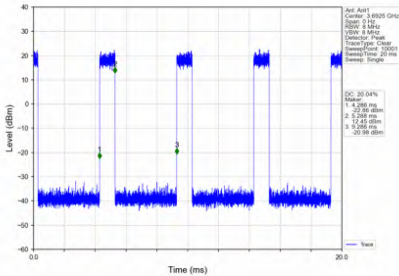
n78d_30kHz_SISO_NTV_15MHz_CP-OFDM 64 QAM_3692.49MHz_Inner_Full
