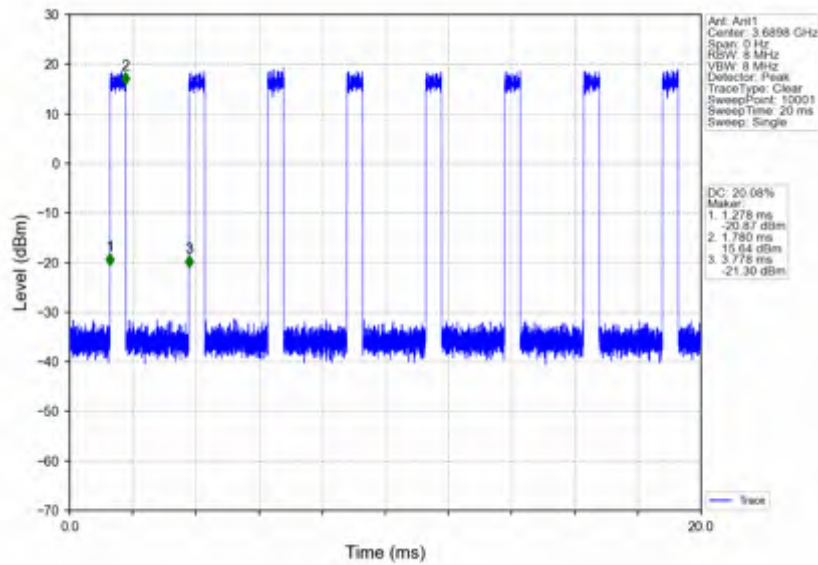
n78d_30kHz_SISO_NTV_20MHz_DFT-s-OFDM 64 QAM_3690MHz_Inner_Full
