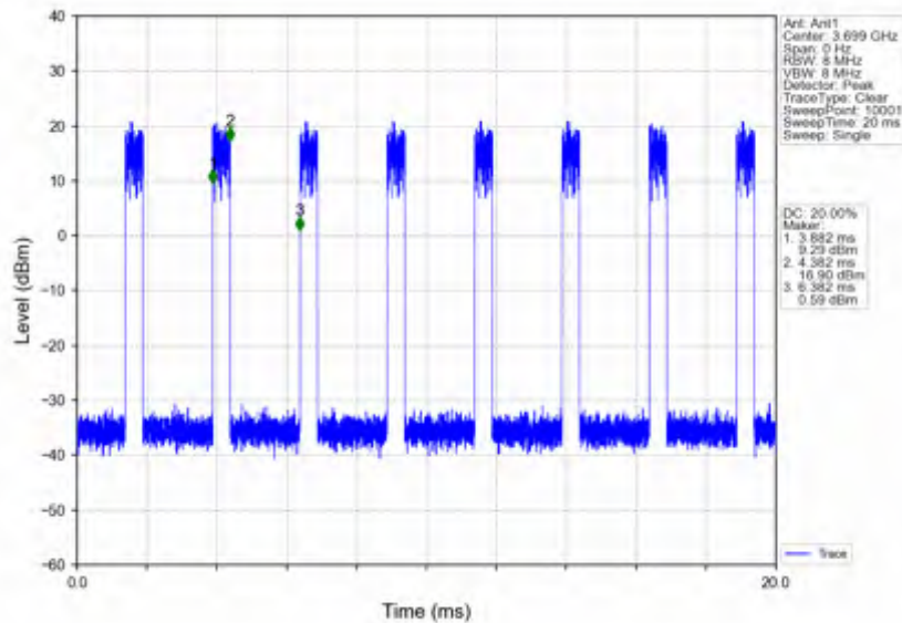
n78d_30kHz_SISO_NTNV_20MHz_DFT-s-OFDM 256 QAM_3690MHz_Edge_1RB_Right
