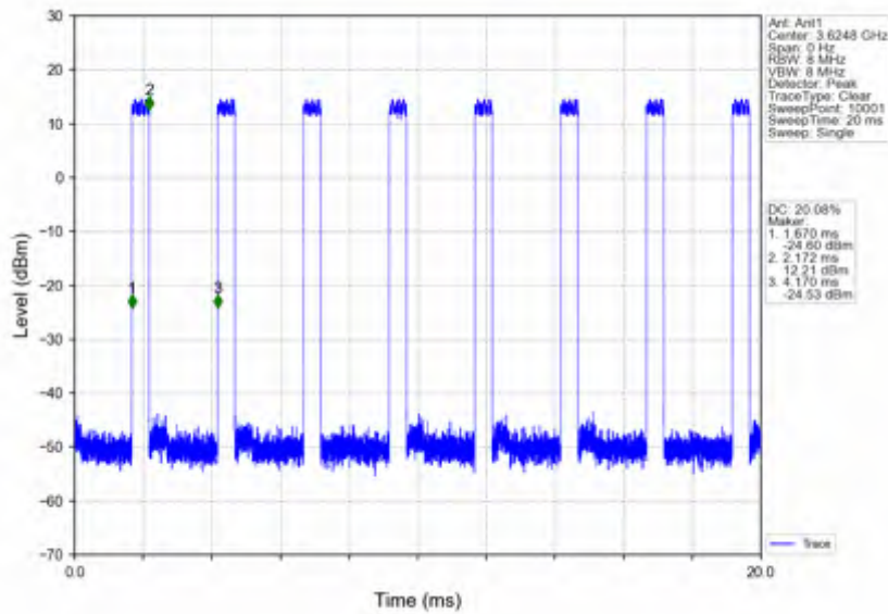
n78d_30kHz_SISO_NTNV_25MHz_DFT-s-OFDM PI/2 BPSK_3624.99MHz_Inner_Full
