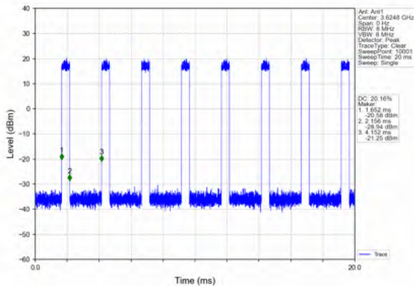
n78d_30kHz_SISO_NTNV_25MHz_DFT-s-OFDM_16 QAM_3624.99MHz_Inner_Full
