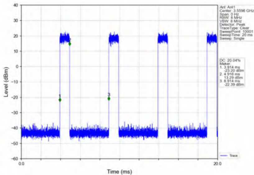
n78d_30kHz_SISO_NTV_20MHz_CP-OFDM 64 QAM_3560.01MHz_Inner_Full
