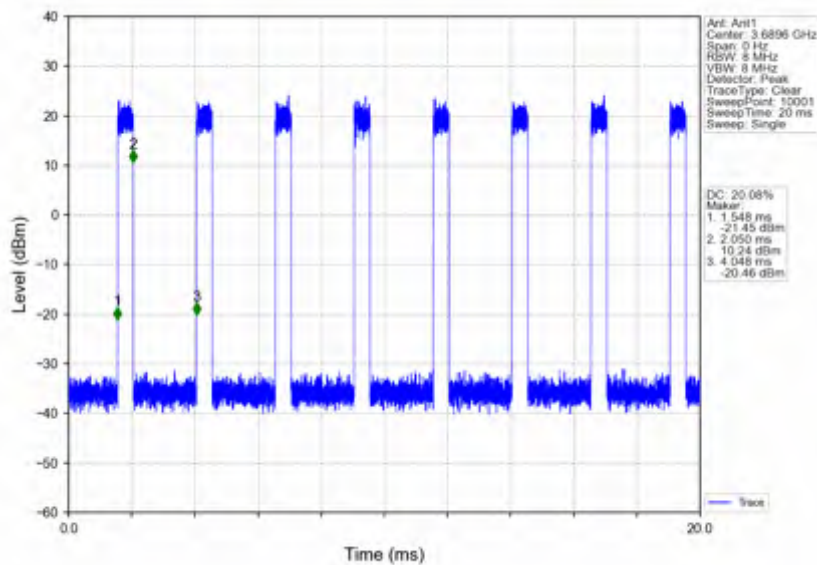
n78d_30kHz_SISO_NTNV_20MHz_CP-OFDM 64 QAM_3690MHz_Inner_Full
