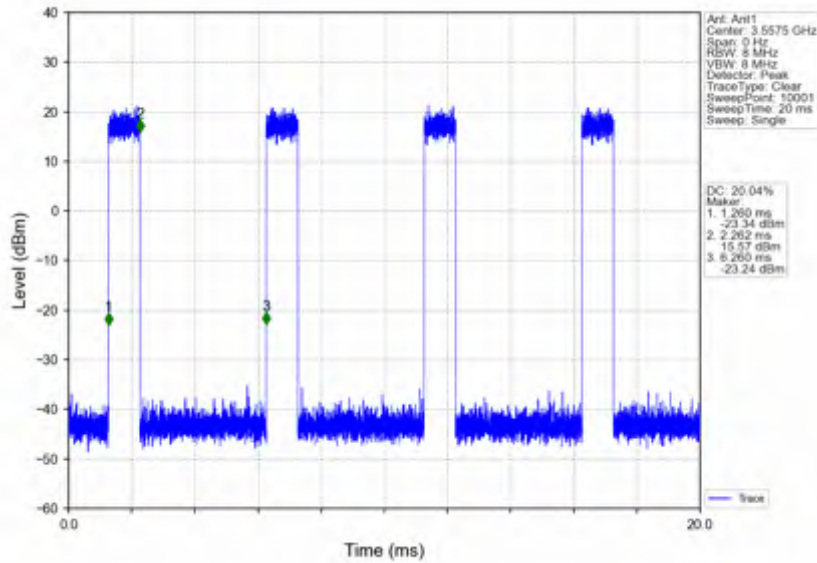
n78d_30kHz_SISO_NTNV_15MHz_CP-OFDM 256 QAM_3557.52MHz_Inner_Full
