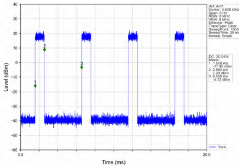
n78d_30kHz_SISO_NTNV_15MHz_CP-OFDM 256 QAM_3624.99MHz_Inner_Full
