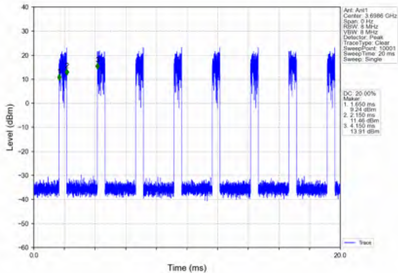
n78d_30kHz_SISO_NTV_20MHz_CP-OFDM 256 QAM_3690MHz_Inner_1RB_Right
