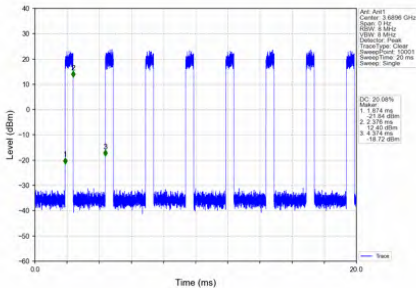
n78d_30kHz_SISO_NTNV_20MHz_CP-OFDM QPSK_3690MHz_Inner_Full
