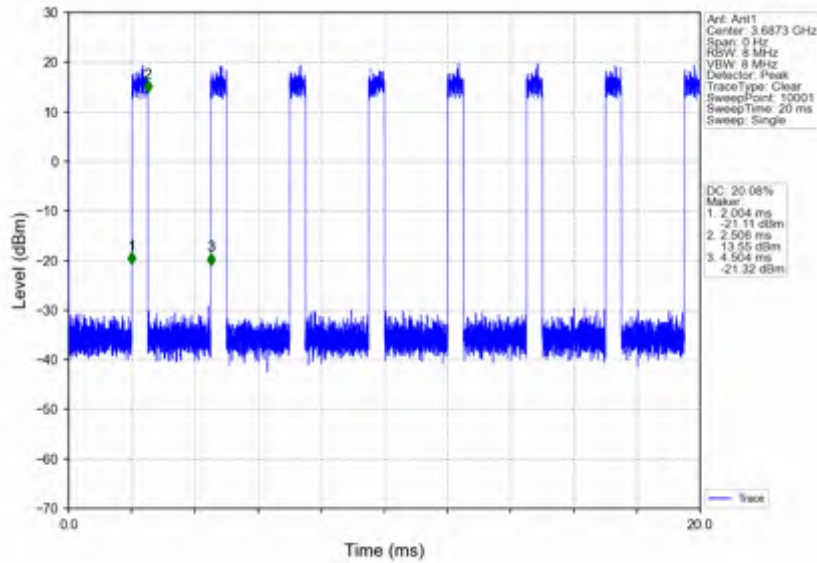
n78d_30kHz_SISO_NTNV_25MHz_DFT-s-OFDM QPSK_3687.48MHz_Inner_Full
