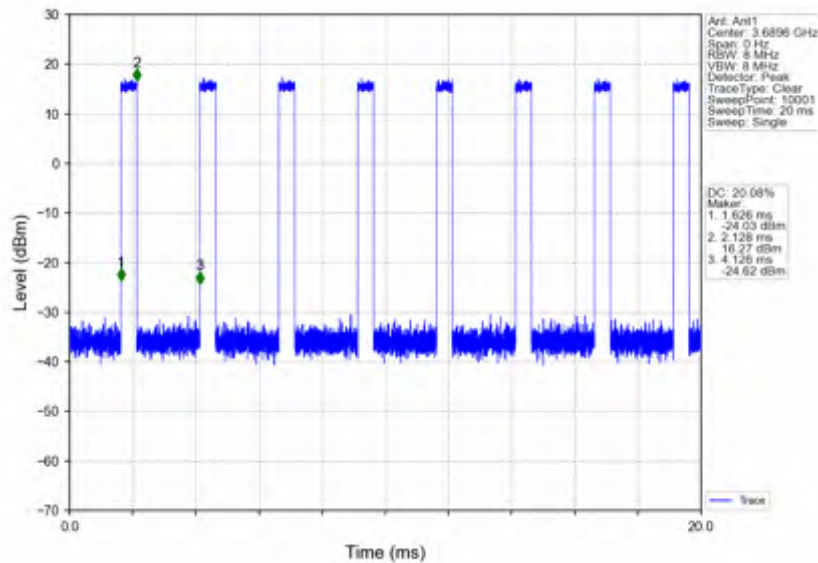
n78d_30kHz_SISO_NTNV_20MHz_DFT-s-OFDM PI/2 BPSK_3690MHz_Inner_Full
