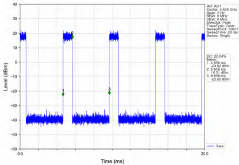
n78d_30kHz_SISO_NTV_15MHz_CP-OFDM 16 QAM_3624.99MHz_Inner_Full
