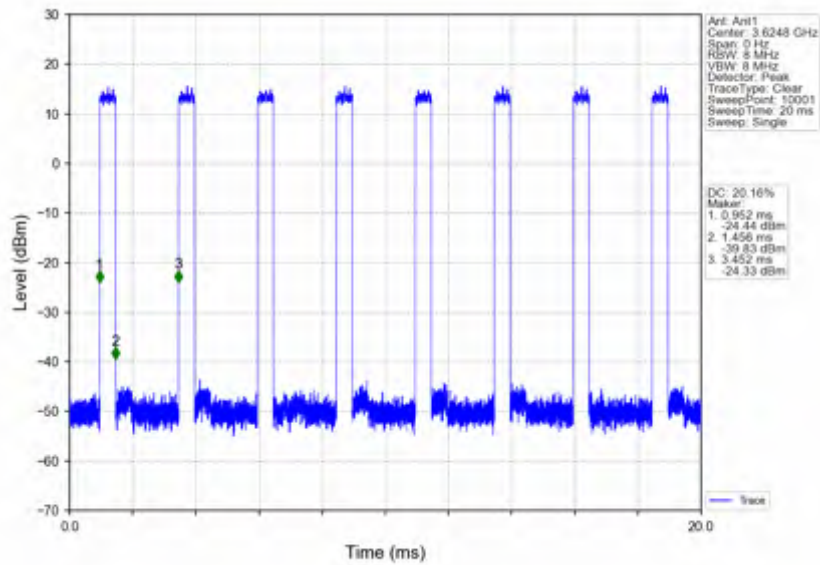
n78d_30kHz_SISO_NTNV_20MHz_DFT-s-OFDM PI/2 BPSK_3624.99MHz_Inner_Full
