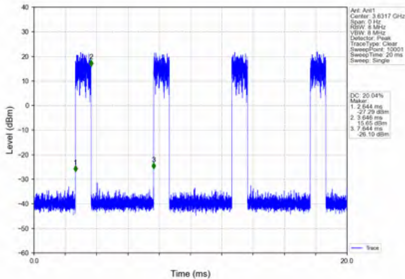
n78d_30kHz_SISO_NTNV_15MHz_CP-OFDM 256 QAM_3624.99MHz_Edge_1RB_Right
