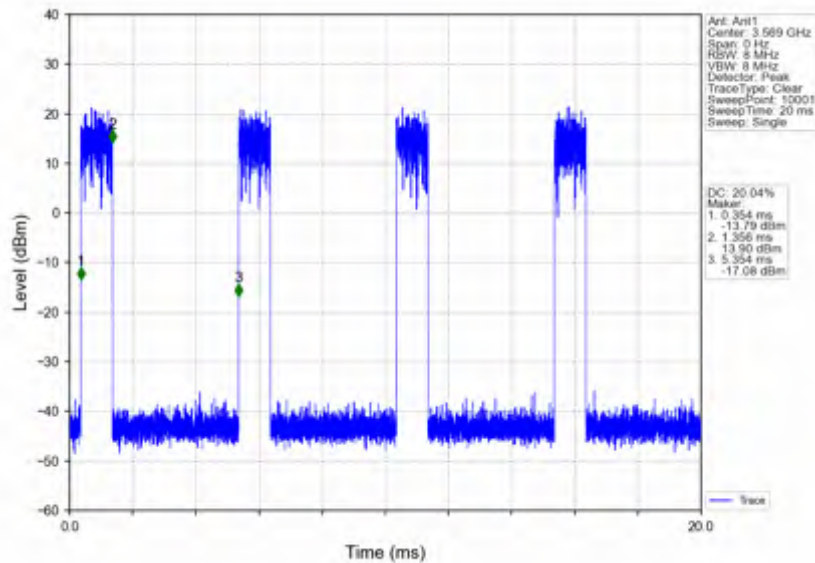
n78d_30kHz_SISO_NTNV_20MHz_CP-OFDM 256 QAM_3560.01MHz_Edge_1RB_Right
