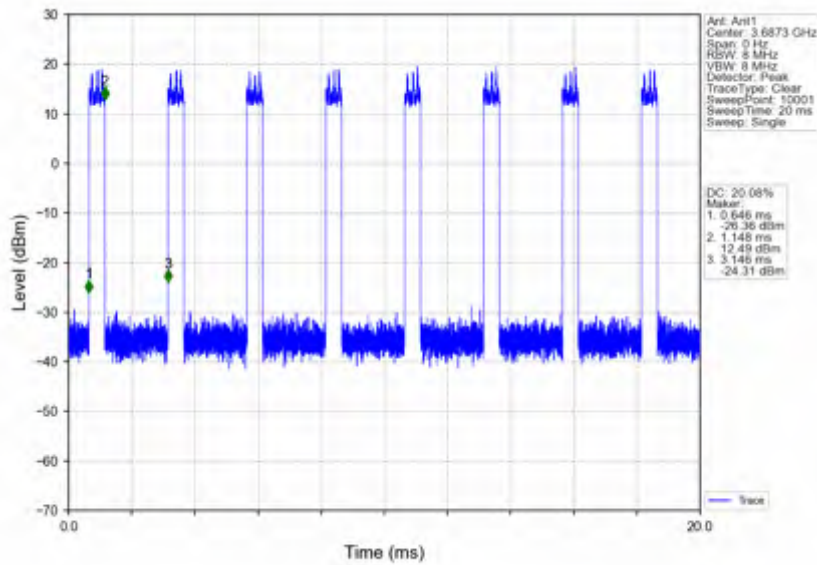
n78d_30kHz_SISO_NTNV_25MHz_DFT-s-OFDM PI/2 BPSK_3687.48MHz_Inner_Full
