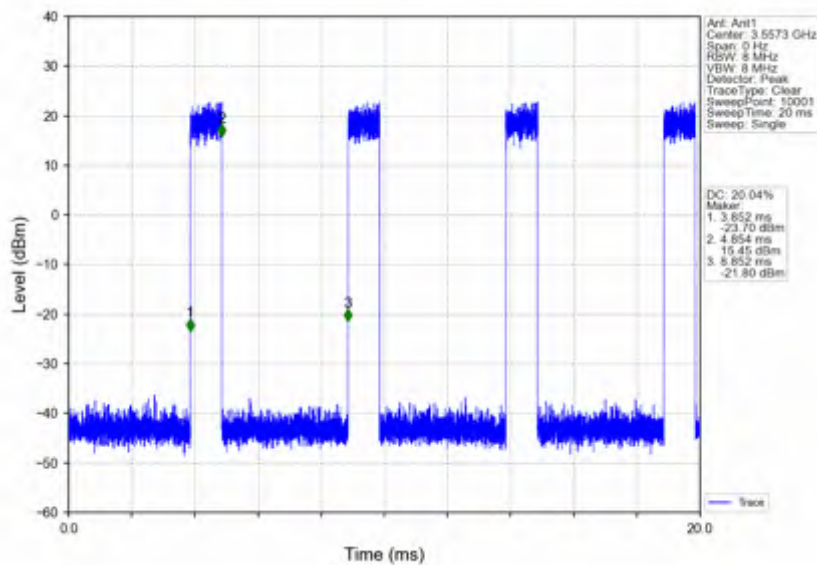
n78d_30kHz_SISO_NTV_15MHz_CP-OFDM 64 QAM_3557.52MHz_Inner_Full
