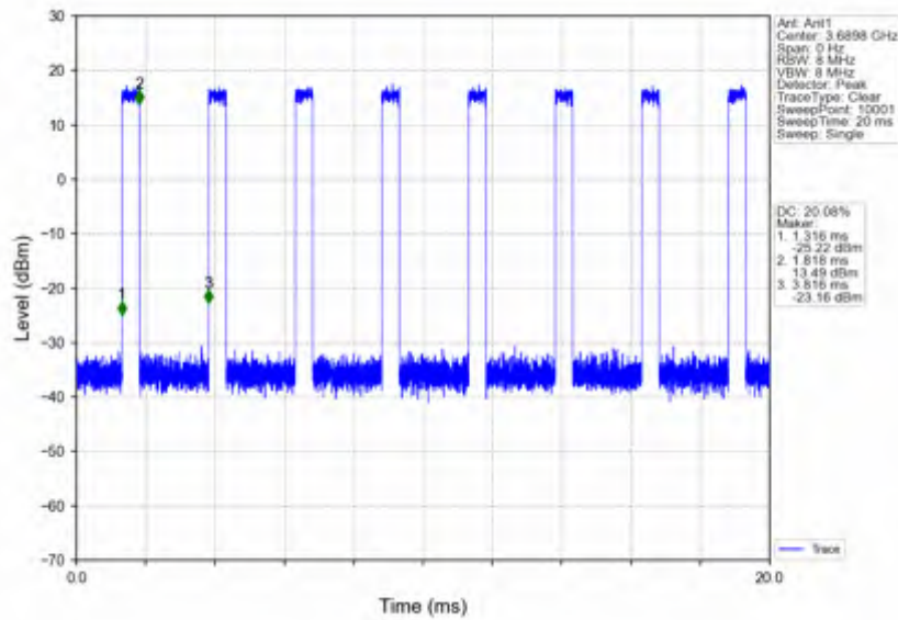
n78d_30kHz_SISO_NTNV_20MHz_DFT-s-OFDM_QPSK_3690MHz_Inner_Full
