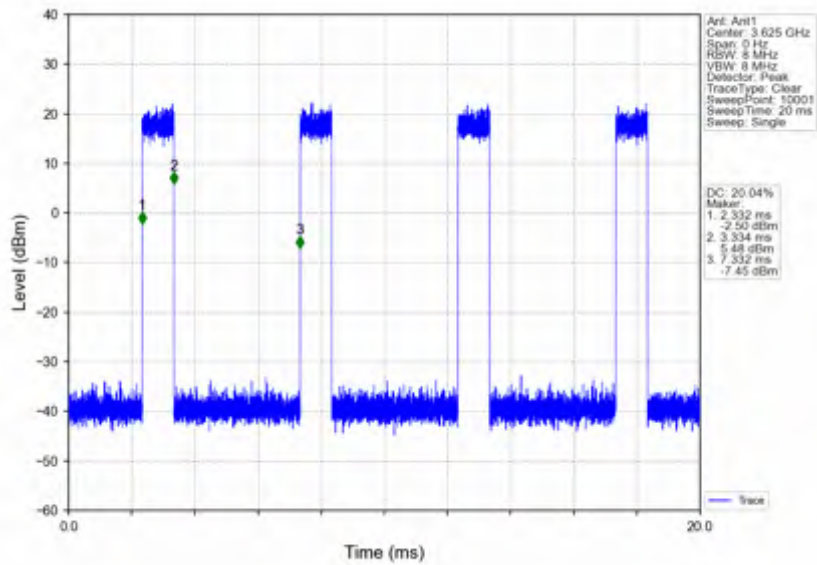
n78d_30kHz_SISO_NTV_15MHz_CP-OFDM 64 QAM_3624.99MHz_Inner_Full
