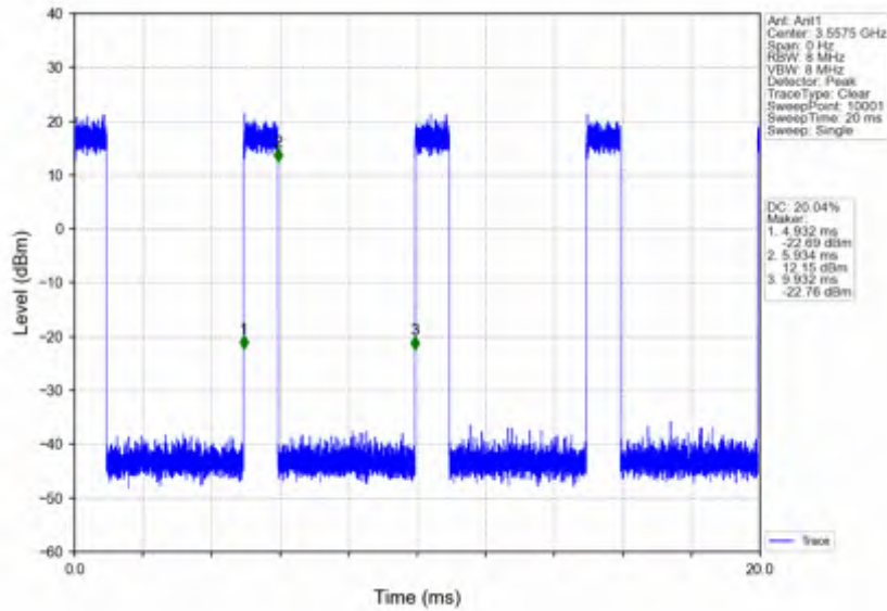
n78d_30kHz_SISO_NTNV_15MHz_CP-OFDM 16 QAM_3557.52MHz_Inner_Full
