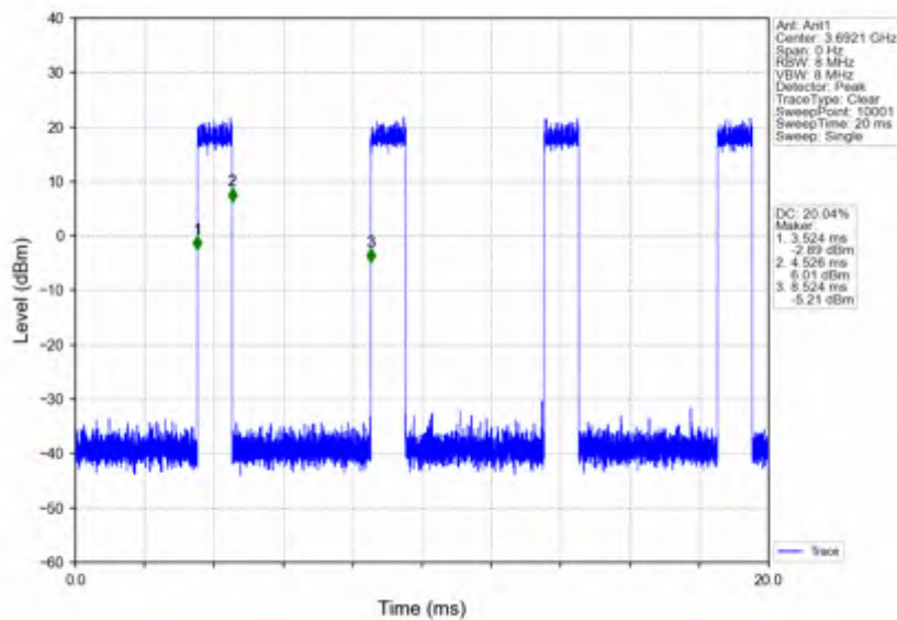
n78d_30kHz_SISO_NTNV_15MHz_DFT-s-OFDM 16 QAM_3692.49MHz_Inner_Full
