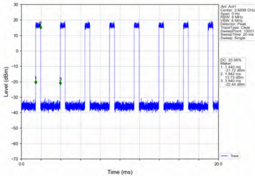
n78d_30kHz_SISO_NTNV_20MHz_DFT-s-OFDM_256_QAM_3690MHz_Inner_Full
