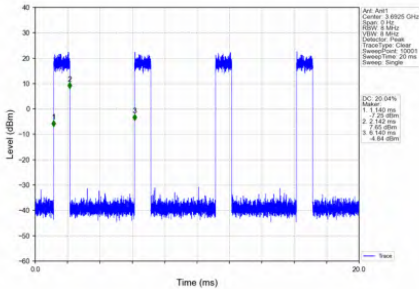
n78d_30kHz_SISO_NTV_15MHz_CP-OFDM_16_QAM_3692.49MHz_Inner_Full
