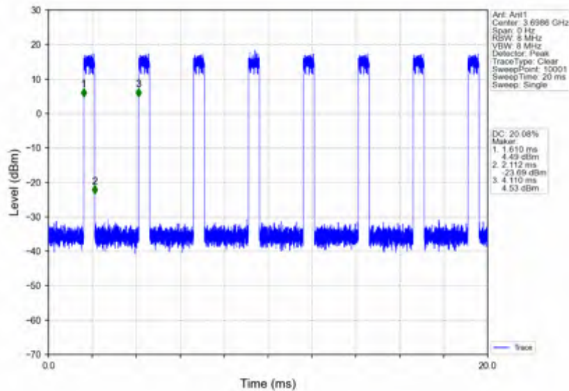
n78d_30kHz_SISO_NTNV_25MHz_DFT-s-OFDM PI/2 BPSK_3687.48MHz_Inner_1RB_Right
