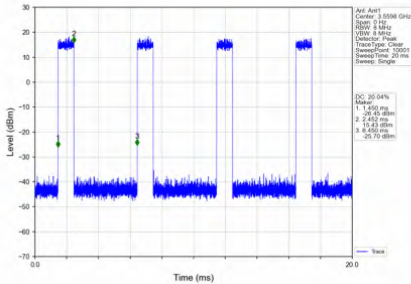
n78d_30kHz_SISO_NTNV_20MHz_DFT-s-OFDM 16 QAM_3560.01MHz_Inner_Full
