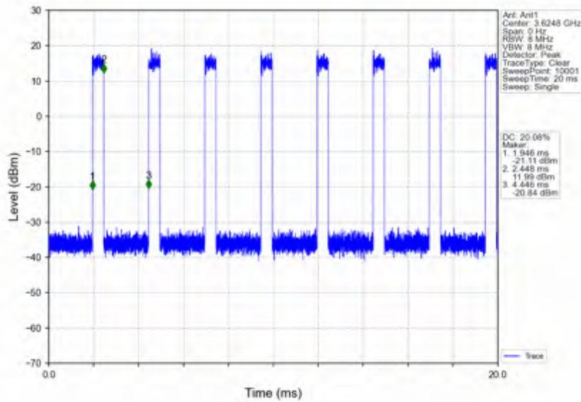
n78d_30kHz_SISO_NTNV_25MHz_DFT-s-OFDM 64 QAM_3624.99MHz_Inner_Full
