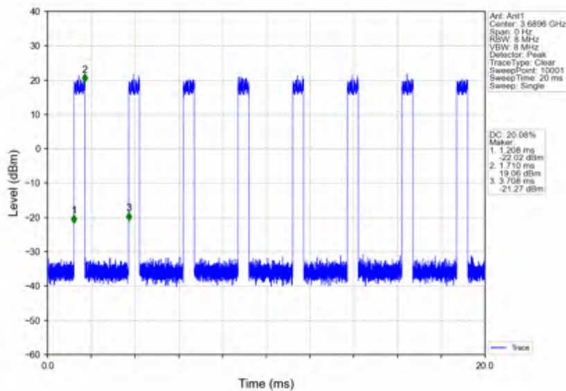
n78d_30kHz_SISO_NTV_20MHz_DFT-s-OFDM 16 QAM_3690MHz_Inner_Full
