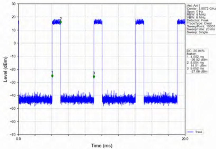
n78d_30kHz_SISO_NTNV_15MHz_DFT-s-OFDM_256_QAM_3557.52MHz_Inner_Full
