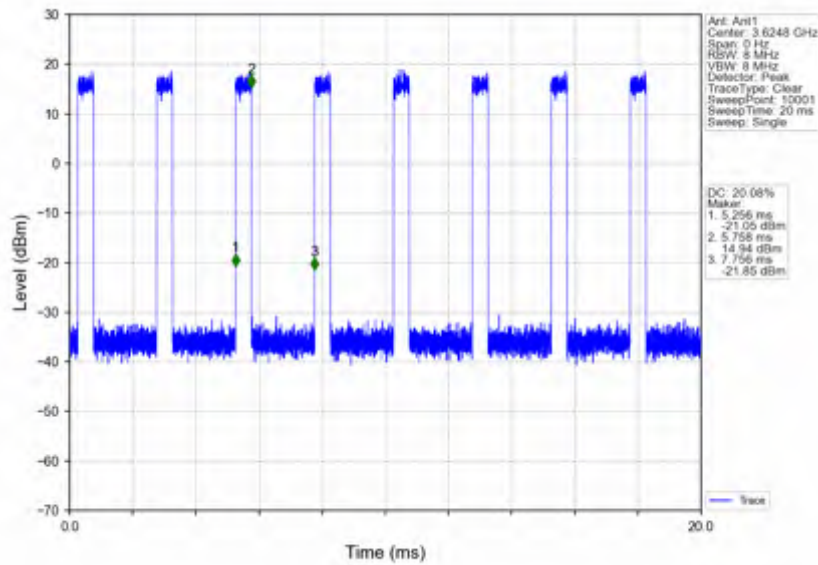
n78d_30kHz_SISO_NTNV_20MHz_DFT-s-OFDM_256_QAM_3624.99MHz_Inner_Full
