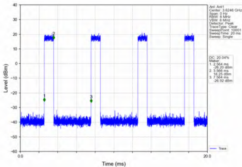
n78d_30kHz_SISO_NTNV_20MHz_DFT-s-OFDM 16 QAM_3624.99MHz_Inner_Full
