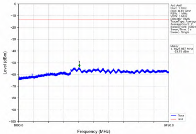
n5_30kHz_SISO_NTNV_15MHz_DFT-s-OFDM PI/2 BPSK_841.5MHz_Outer_Full
