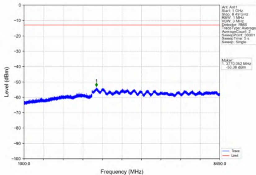
n5 30kHz SISO NTN 15MHz DFT-s-OFDM QPSK 841.5MHz Inner 1RB Right
