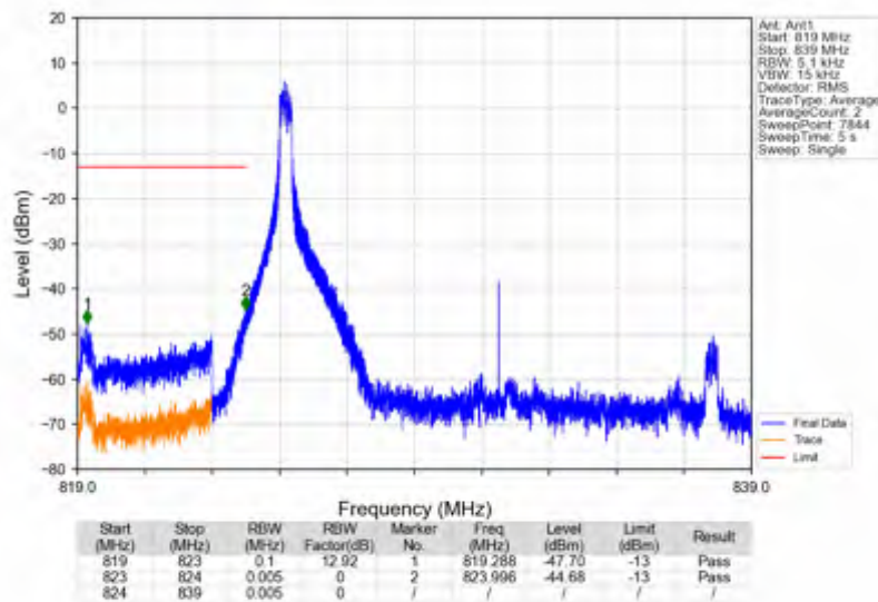
n5_30kHz_SISO_NTNV_15MHz_DFT-s-OFDM PI/2 BPSK 831.5MHz Inner_1RB_Left
