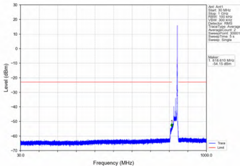
n5_30kHz_SISO_NTNV_20MHz_CP-OFDM QPSK_839MHz_Edge_1RB_Right
