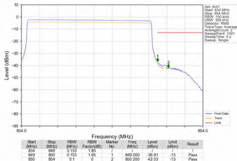
n5 30kHz SISO NTNV 15MHz CP-OFDM QPSK 841.5MHz Outer Full
