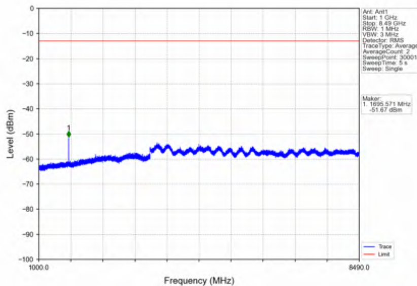
n5 30kHz SISO NTN 10MHz DFT-s-OFDM QPSK 844MHz Inner 1RB Right
