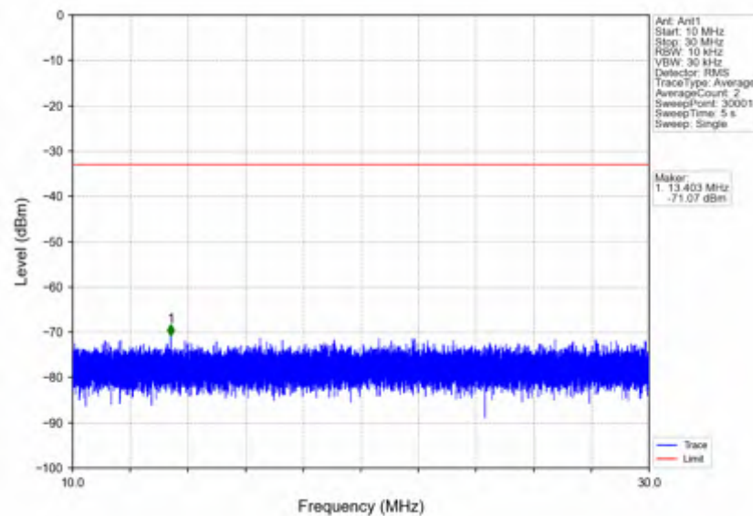
n5_30kHz_SISO_NTNV_10MHz_DFT-s-OFDM_QPSK_829MHz_Inner_1RB_Left
