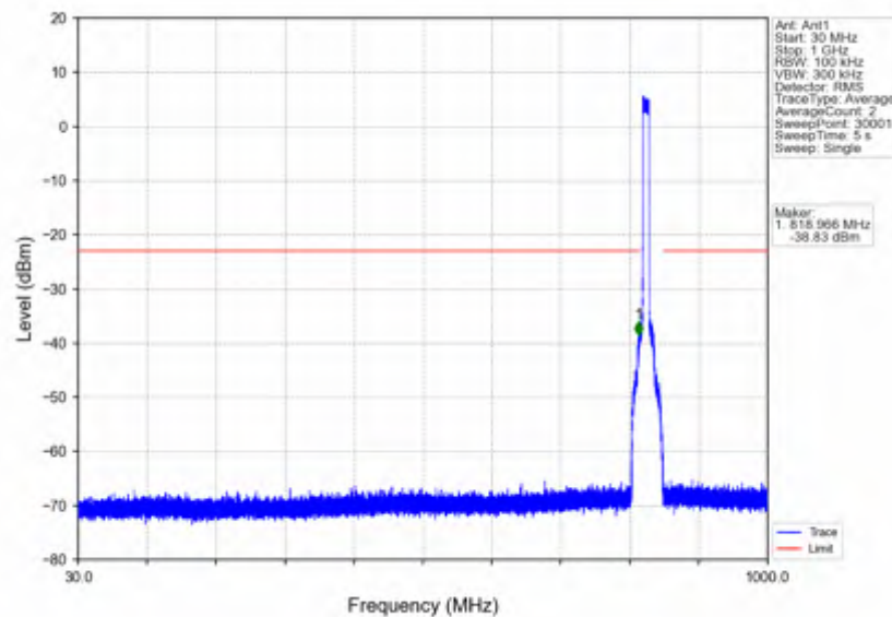
n5_30kHz_SISO_NTNV_10MHz_DFT-s-OFDM QPSK_829MHz_Outer_Full
