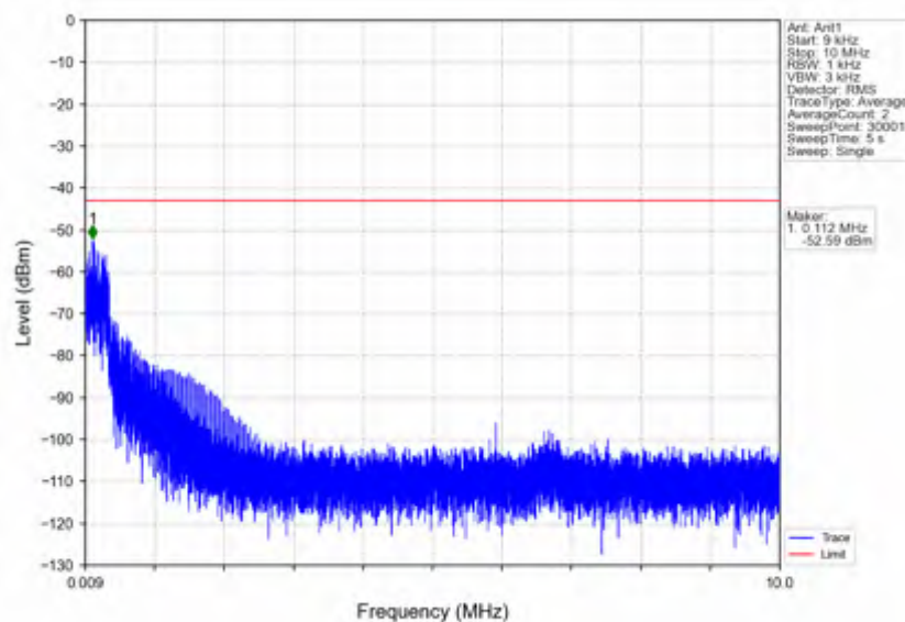
n5_30kHz_SISO_NTNV_15MHz_DFT-s-OFDM PI/2 BPSK 831.5MHz_Edge_1RB_Left
