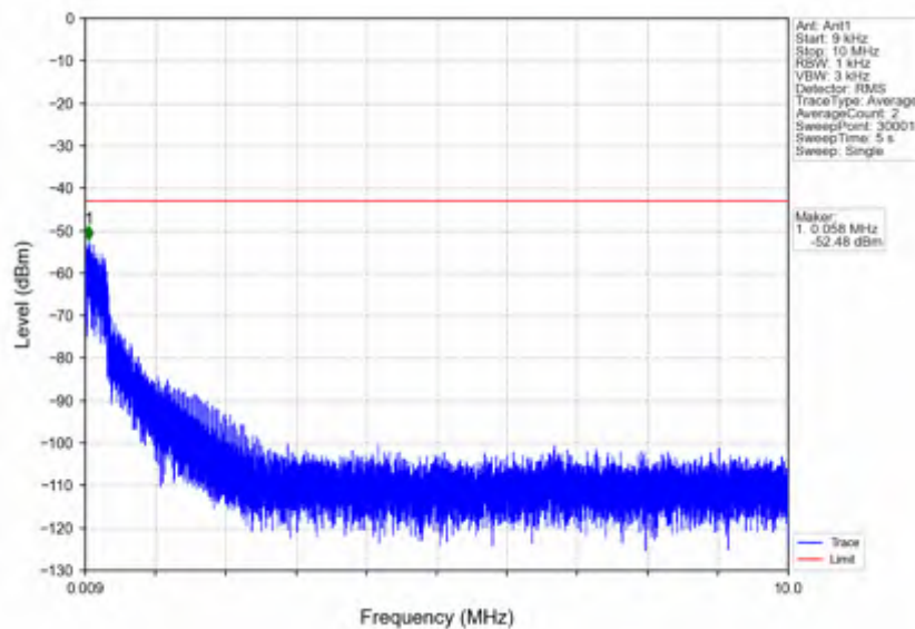
n5_30kHz_SISO_NTNV_15MHz_CP-OFDM QPSK_841.5MHz_Edge_1RB_Right
