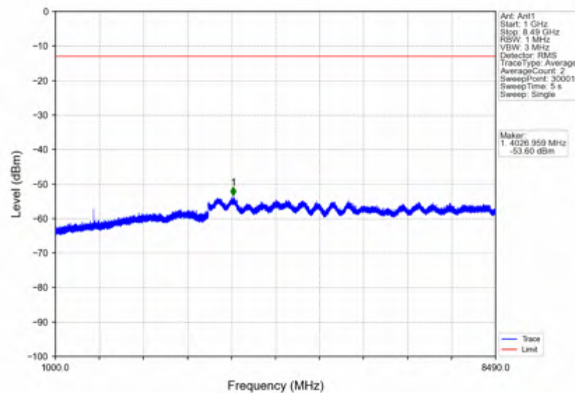
n5_30kHz_SISO_NTNV_15MHz_CP-OFDM QPSK_831.5MHz_Outer_Full
