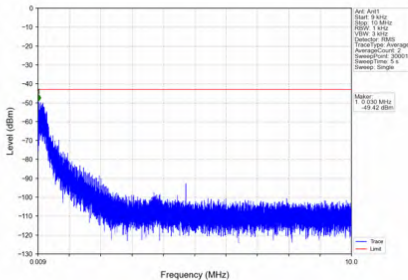
n5_30kHz_SISO_NTNV_10MHz_CP-OFDM_QPSK_844MHz_Inner_1RB_Right
