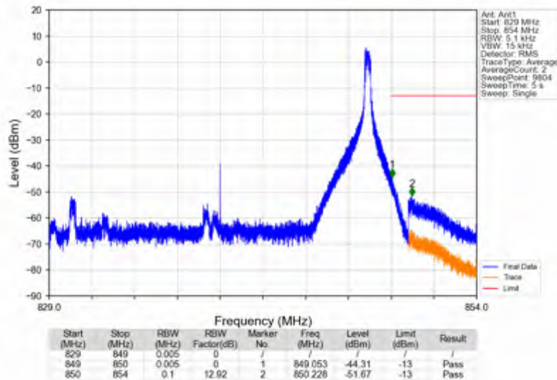
n5_30kHz_SISO_NTNV_20MHz_DFT-s-OFDM QPSK_839MHz_Inner_1RB_Right
