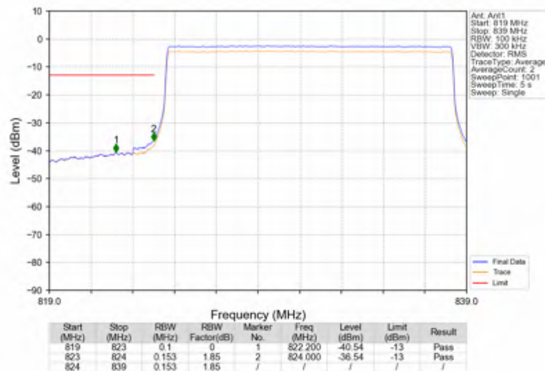
n5_30kHz_SISO_NTNV_15MHz_CP-OFDM QPSK_831.5MHz_Outer_Full
