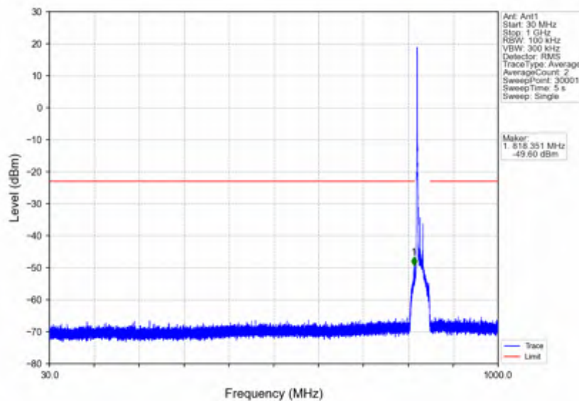
n5_30kHz_SISO_NTNV_15MHz_DFT-s-OFDM_QPSK_831.5MHz_Inner_1RB_Left
