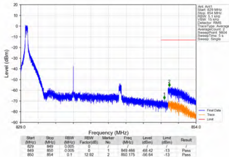
n5_30kHz_SISO_NTV_15MHz_CP-OFDM_QPSK_836.5MHz_Edge_1RB_Left
