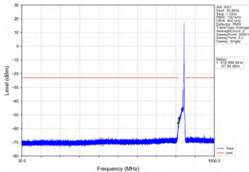
n5_30kHz_SISO_NTNV_15MHz_CP-OFDM QPSK_841.5MHz_Inner_1RB_Right
