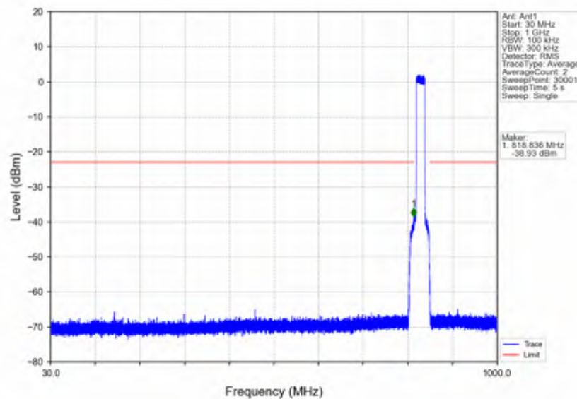
n5_30kHz_SISO_NTNV_20MHz_DFT-s-OFDM QPSK_834MHz_Outer_Full
