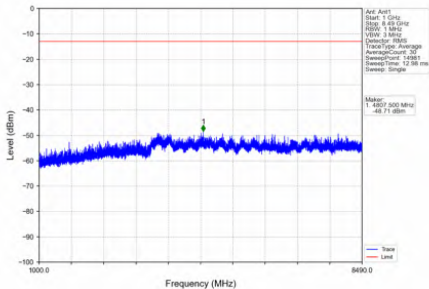
n5_15kHz_SISO_NTNV_20MHz_CP-OFDM QPSK_839MHz_Edge_1RB_Right
