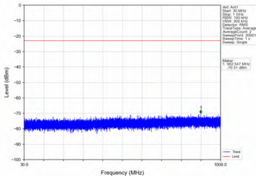
n7_15kHz_SISO_NTNV_5MHz_DFT-s-OFDM QPSK_2502.5MHz_Edge_1RB_Left
