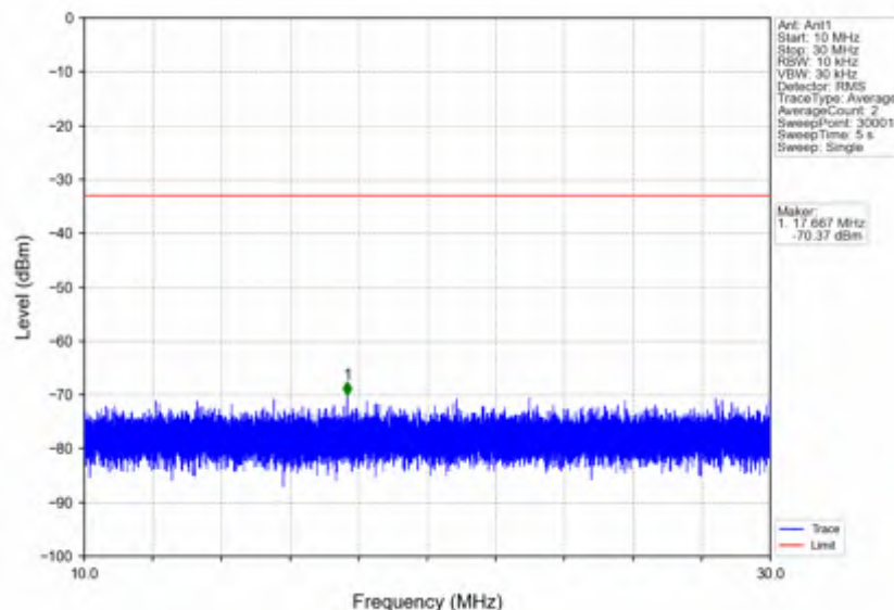
n5_30kHz_SISO_NTNV_10MHz_DFT-s-OFDM PI/2 BPSK 836.5MHz_Edge_1RB_Left
