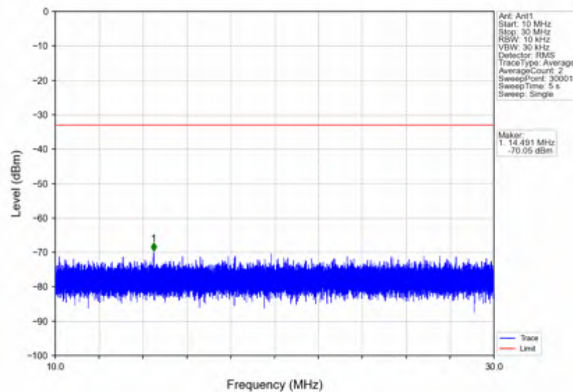
n5_30kHz_SISO_NTNV_15MHz_DFT-s-OFDM_QPSK_831.5MHz_Edge_1RB_Left
