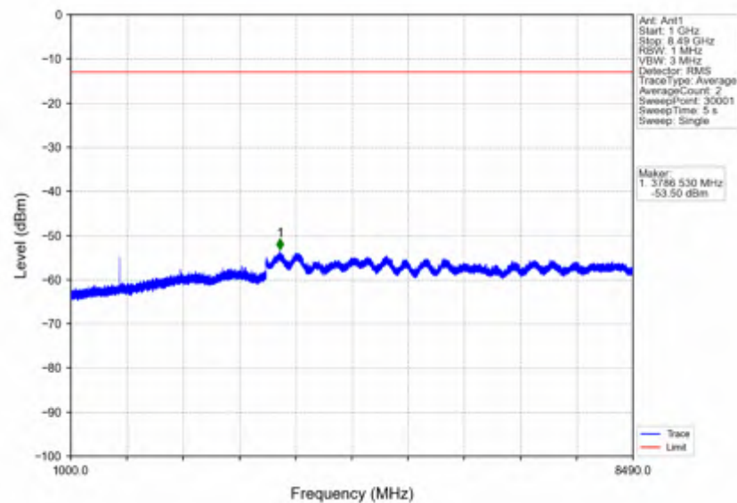
n5_30kHz_SISO_NTNV_20MHz_DFT-s-OFDM PI/2 BPSK_834MHz_Outer_Full
