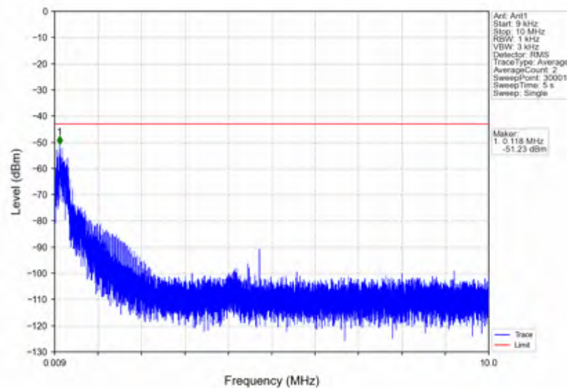
n5_30kHz_SISO_NTNV_10MHz_DFT-s-OFDM QPSK_844MHz_Edge_1RB_Right
