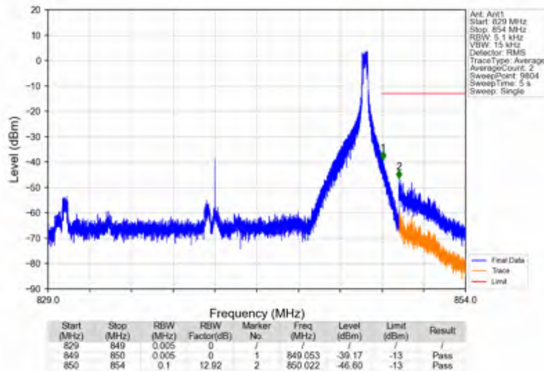
n5_30kHz_SISO_NTNV_20MHz_DFT-s-OFDM_QPSK_839MHz_Edge_1RB_Right
