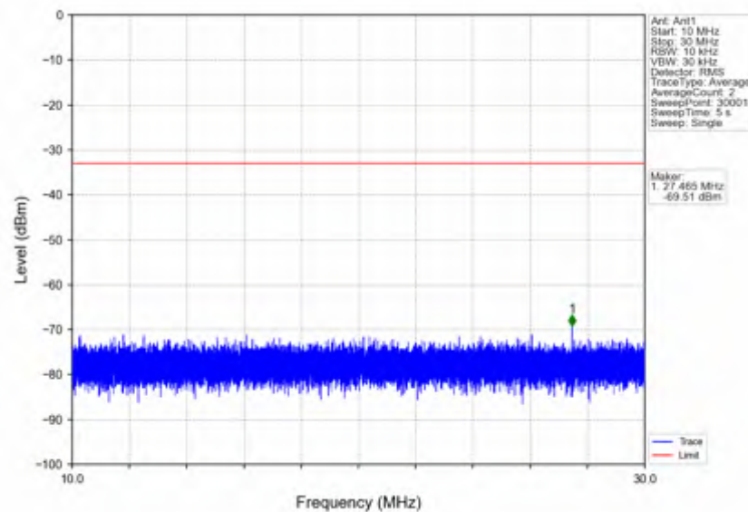
n5_30kHz_SISO_NTNV_10MHz_DFT-s-OFDM_QPSK_829MHz_Edge_1RB_Left
