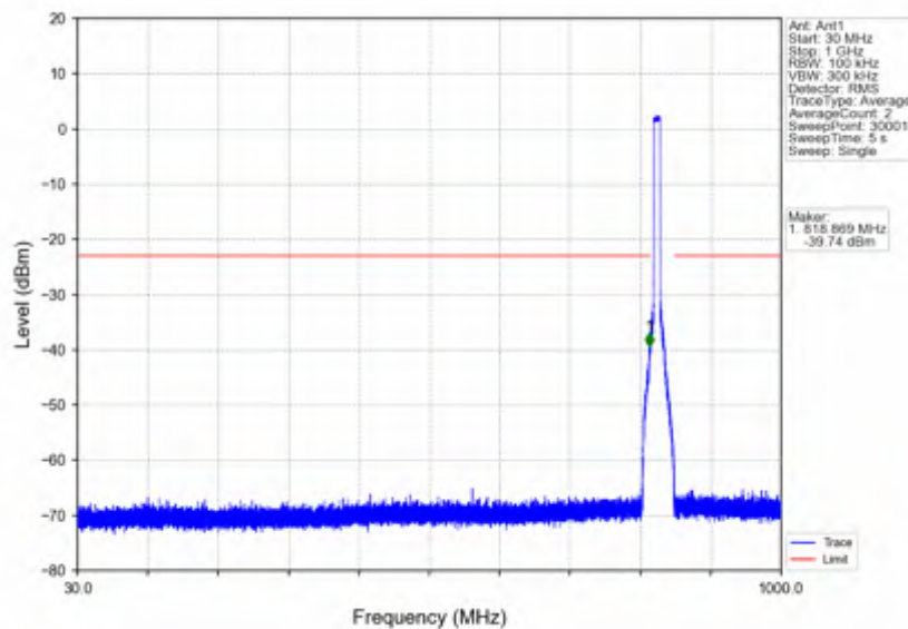
n5_30kHz_SISO_NTNV_10MHz_CP-OFDM QPSK_829MHz_Outer_Full
