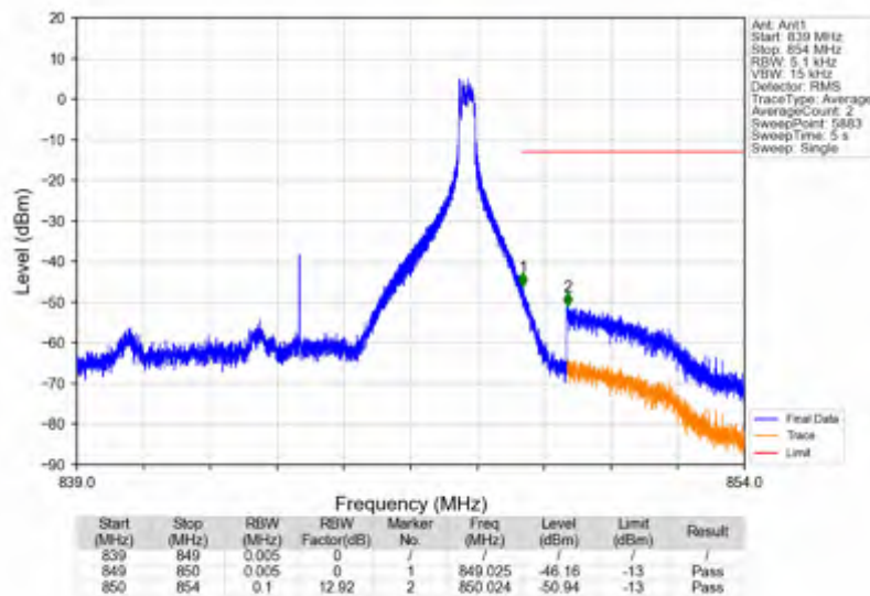
n5_30kHz_SISO_NTNV_10MHz_DFT-s-OFDM QPSK_844MHz_Inner_1RB_Right
