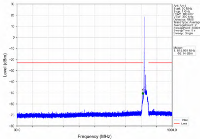
n5_30kHz_SISO_NTNV_20MHz_DFT-s-OFDM QPSK_834MHz_Edge_1RB_Left
