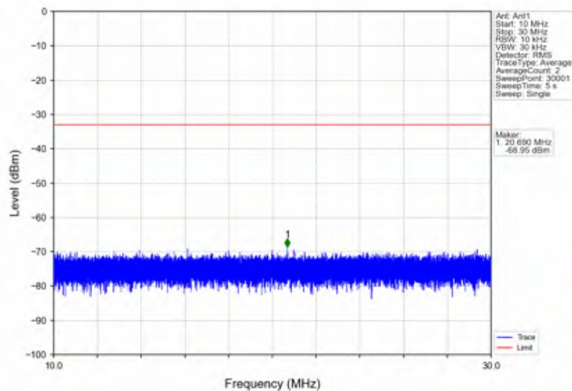
n5_30kHz_SISO_NTNV_20MHz_DFT-s-OFDM QPSK_839MHz_Outer_Full
