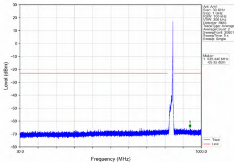
n5_30kHz_SISO_NTNV_10MHz_CP-OFDM_QPSK_844MHz_Inner_1RB_Right
