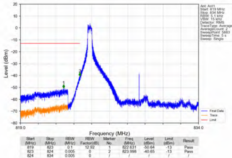
n5_30kHz_SISO_NTNV_10MHz_DFT-s-OFDM QPSK_829MHz_Edge_1RB_Left
