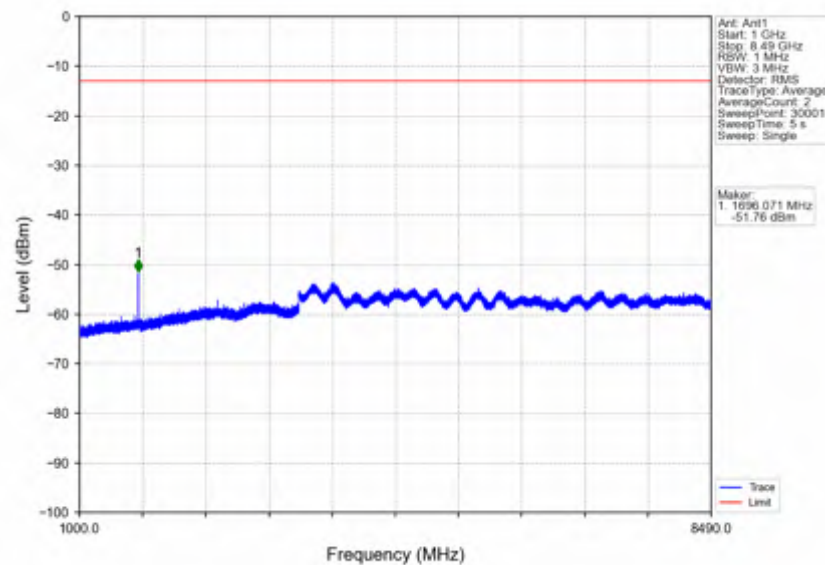
n5 30kHz SISO NTNv 10MHz DFT-s-OFDM PI/2 BPSK 844MHz Outer Full
