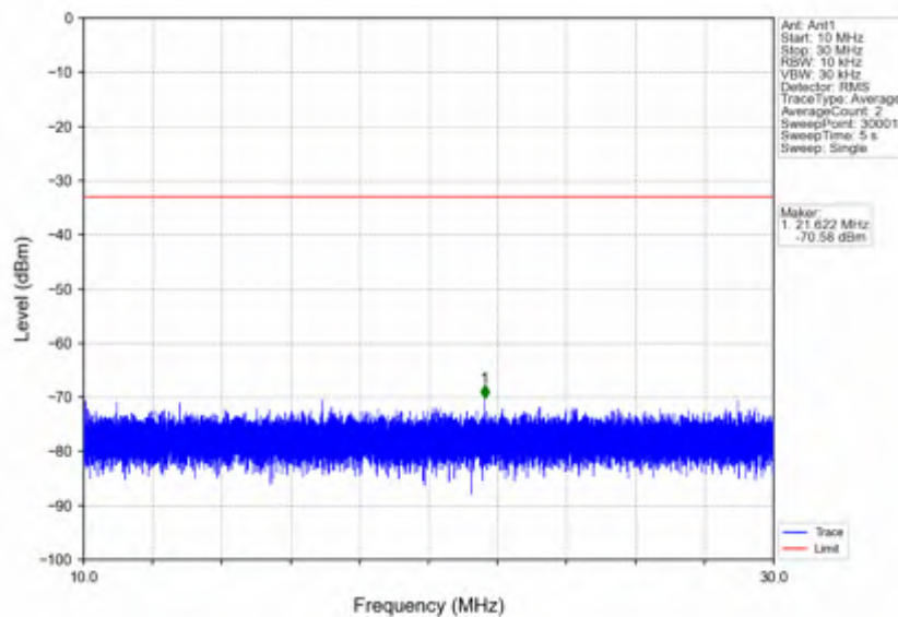
n5_30kHz_SISO_NTNV_15MHz_DFT-s-OFDM_QPSK_841.5MHz_Outer_Full
