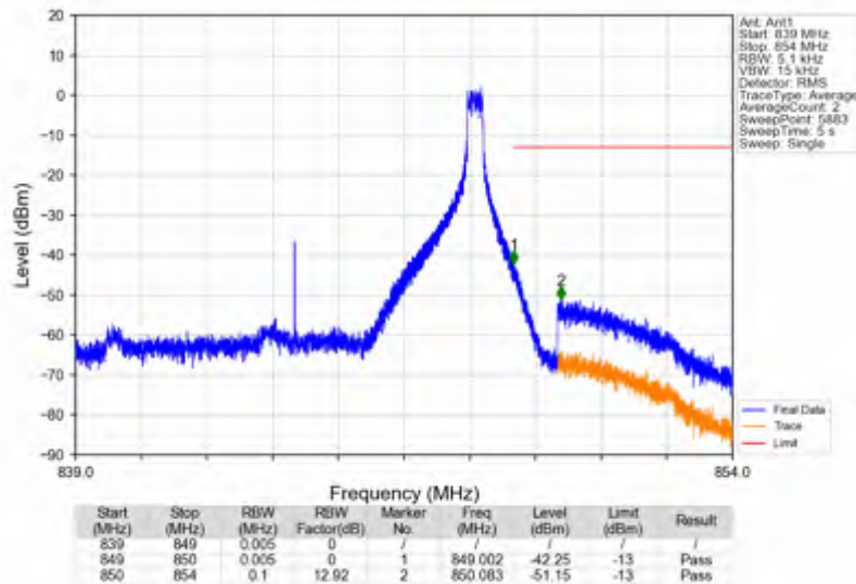
n5_30kHz_SISO_NTNV_10MHz_CP-OFDM QPSK_844MHz_Edge_1RB_Right
