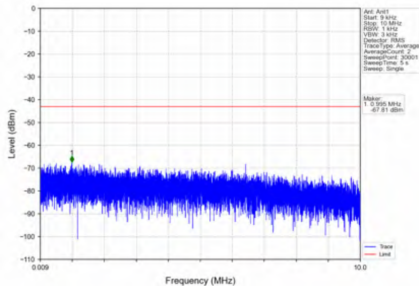
n5_30kHz_SISO_NTNV_15MHz_CP-OFDM_QPSK_831.5MHz_Outer_Full
