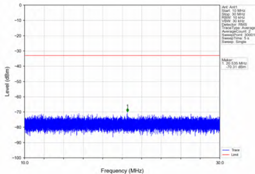
n5_30kHz_SISO_NTNV_10MHz_CP-OFDM_QPSK_829MHz_Edge_1RB_Left
