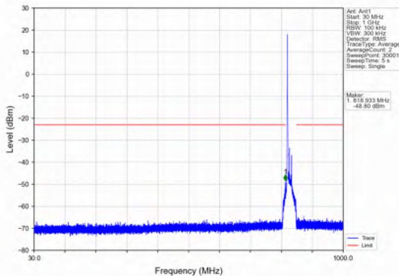
n5_30kHz_SISO_NTNV_15MHz_DFT-s-OFDM_QPSK_831.5MHz_Edge_1RB_Left
