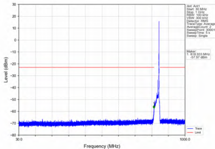
n5_30kHz_SISO_NTNV_15MHz_CP-OFDM QPSK_841.5MHz_Edge_1RB_Right
