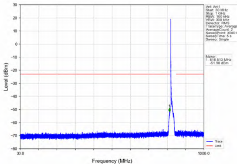
n5_30kHz_SISO_NTNV_10MHz_DFT-s-OFDM QPSK_829MHz_Inner_1RB_Left
