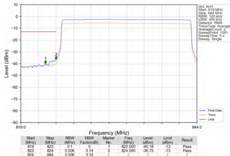
n5_30kHz_SISO_NTNV_20MHz_CP-OFDM QPSK_834MHz_Outer_Full
