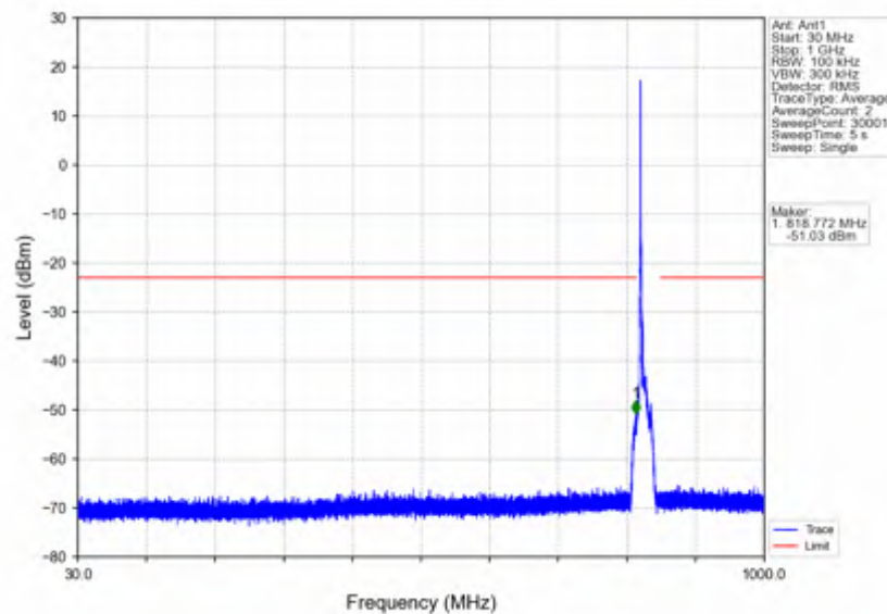
n5_30kHz_SISO_NTNV_10MHz_CP-OFDM_QPSK_829MHz_Inner_1RB_Left
