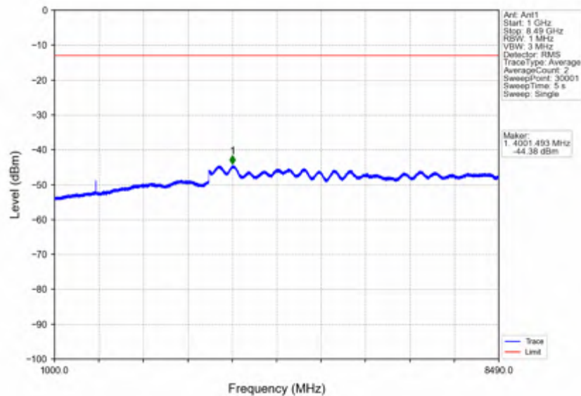
n5_30kHz_SISO_NTNV_20MHz_DFT-s-OFDM QPSK_834MHz_Edge_1RB_Left
