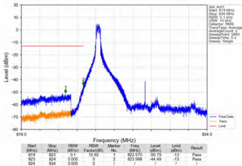
n5_30kHz_SISO_NTNV_10MHz_DFT-s-OFDM QPSK_829MHz_Inner_1RB_Left
