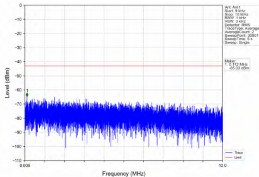
n5_30kHz_SISO_NTNV_15MHz_CP-OFDM_QPSK_841.5MHz_Outer_Full
