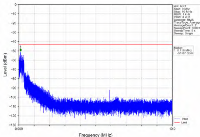
n5_30kHz_SISO_NTNV_15MHz_DFT-s-OFDM PI/2 BPSK 831.5MHz Inner_1RB_Left
