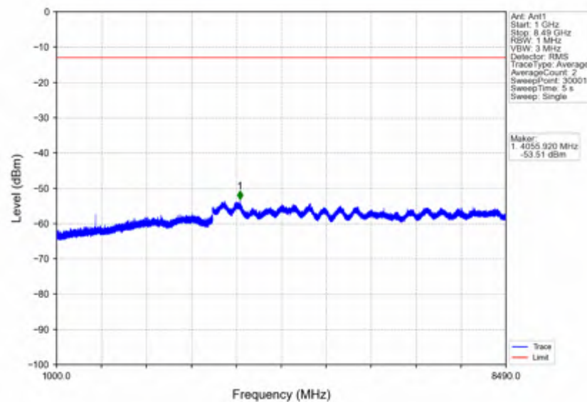
n5_30kHz_SISO_NTNV_10MHz_CP-OFDM QPSK_829MHz_Outer_Full
