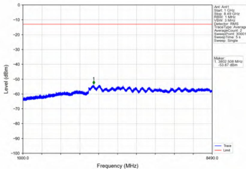
n5_30kHz_SISO_NTNV_20MHz_CP-OFDM QPSK_834MHz_Outer_Full
