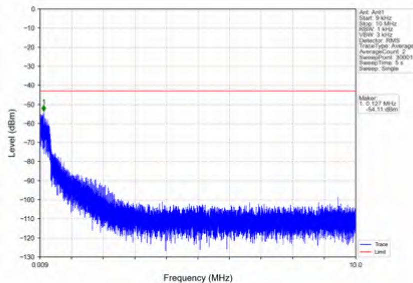
n5_30kHz_SISO_NTNV_20MHz_CP-OFDM_QPSK_834MHz_Edge_1RB_Left
