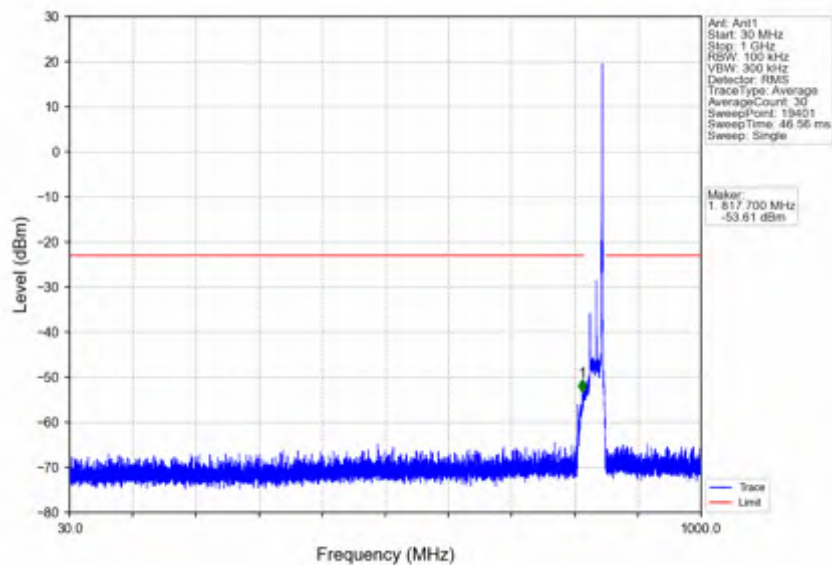
n5_15kHz_SISO_NTNV_20MHz_CP-OFDM QPSK_839MHz_Edge_1RB_Right
