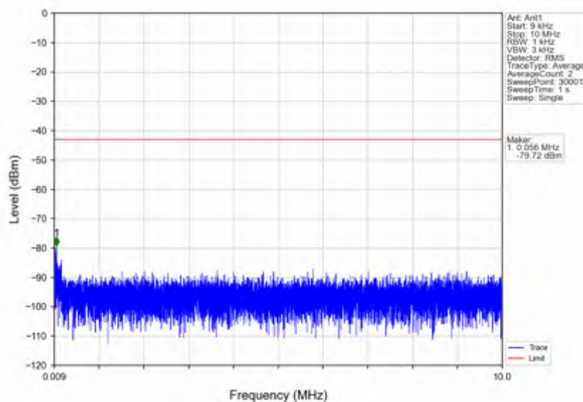
n7_15kHz_SISO_NTNV_5MHz_DFT-s-OFDM_PI/2_BPSK_2502.5MHz_Edge_1RB_Left
