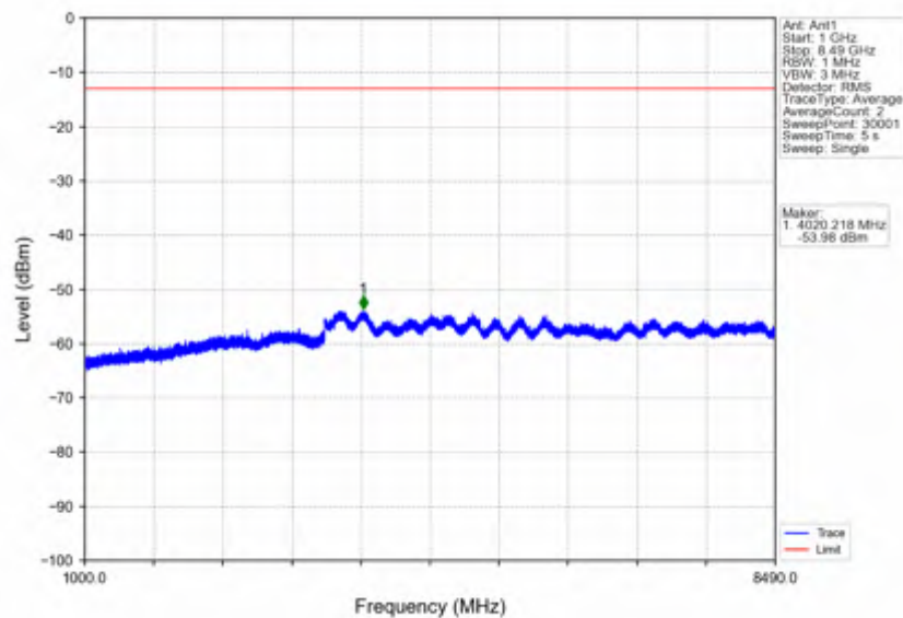
n5_30kHz_SISO_NTNV_10MHz_DFT-s-OFDM QPSK_844MHz_Inner_1RB_Right
