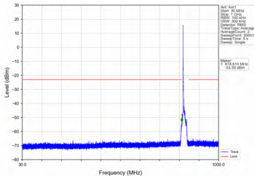
n5_30kHz_SISO_NTNV_10MHz_CP-OFDM_QPSK_829MHz_Edge_1RB_Left
