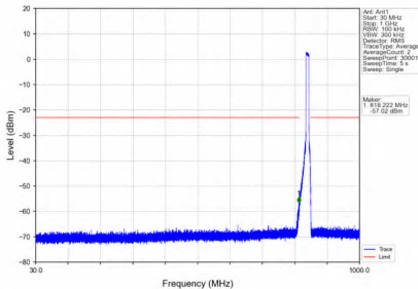
n5_30kHz_SISO_NTNV_10MHz_CP-OFDM QPSK_844MHz_Outer_Full
