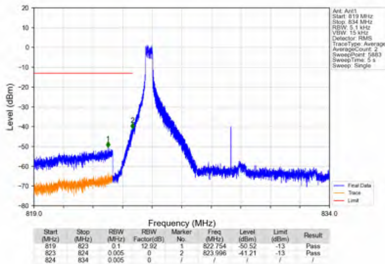
n5_30kHz_SISO_NTNV_10MHz_CP-OFDM_QPSK_829MHz_Edge_1RB_Left
