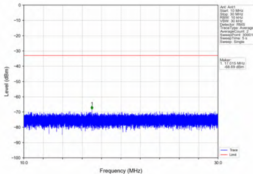
n5_30kHz_SISO_NTNV_20MHz_CP-OFDM QPSK_839MHz_Inner_1RB_Right
