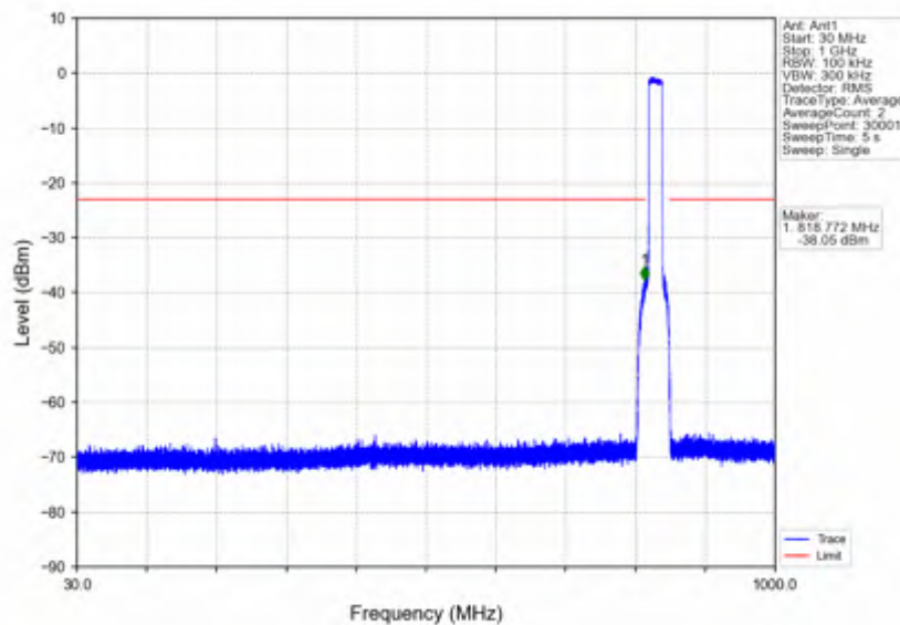
n5_30kHz_SISO_NTNV_20MHz_CP-OFDM QPSK_834MHz_Outer_Full
