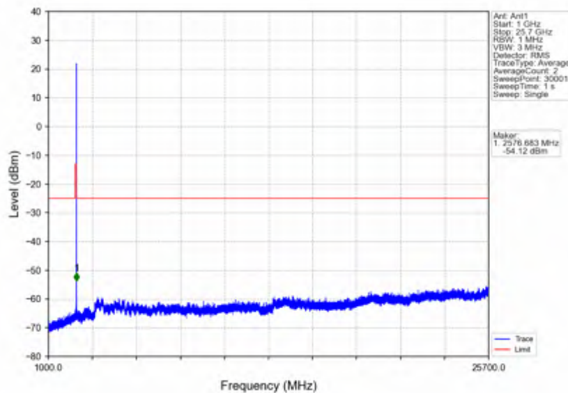
n7_15kHz_SISO_NTNV_5MHz_DFT-s-OFDM QPSK_2502.5MHz_Edge_1RB_Left
