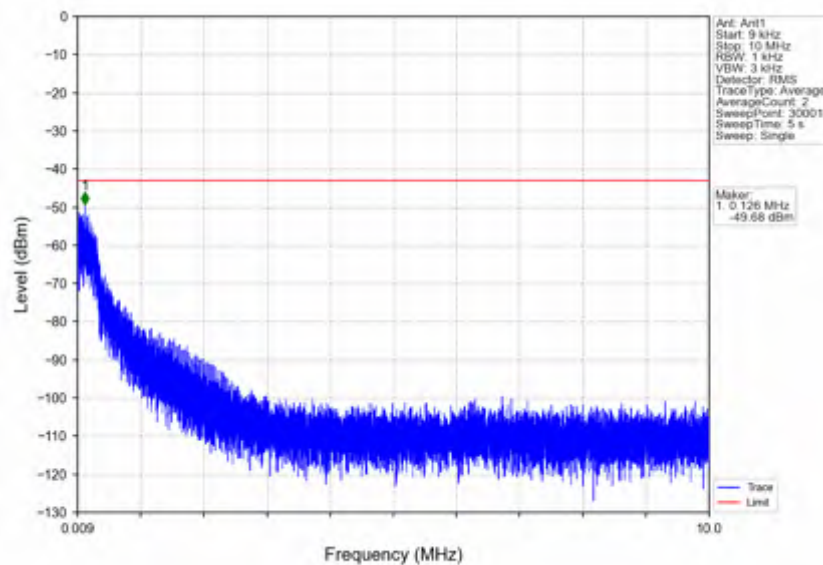
n5_30kHz_SISO_NTNV_15MHz_CP-OFDM QPSK_841.5MHz_Inner_1RB_Right
