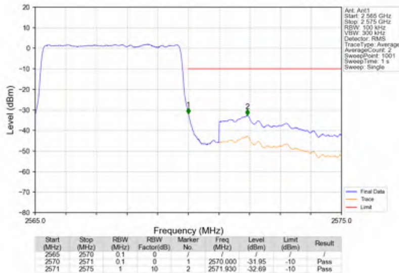
n7_15kHz_SISO_NTNV_5MHz_DFT-s-OFDM PI/2 BPSK_2567.5MHz_Outer_Full
