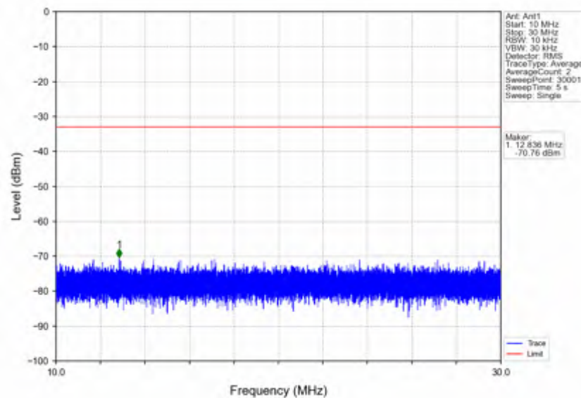
n5_30kHz_SISO_NTNV_10MHz_DFT-s-OFDM QPSK_844MHz_Inner_1RB_Right
