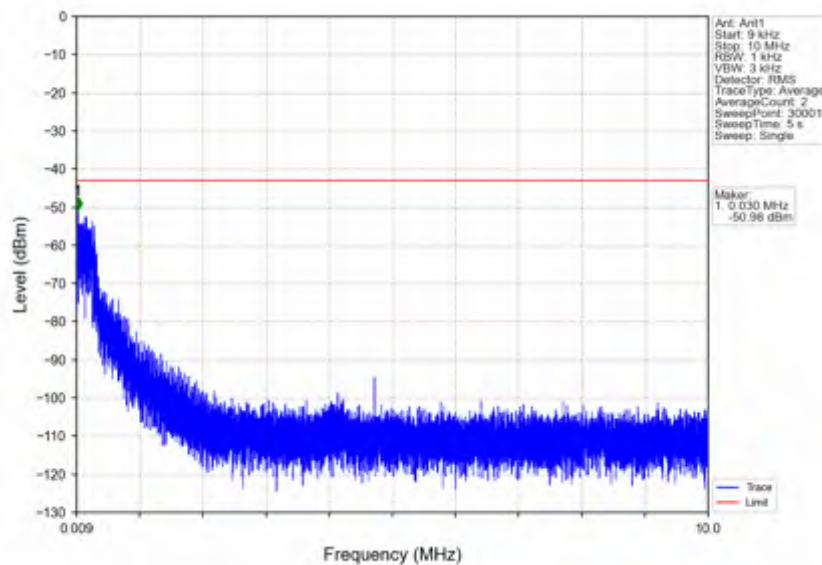
n5_30kHz_SISO_NTNV_10MHz_CP-OFDM QPSK_844MHz_Edge_1RB_Right
