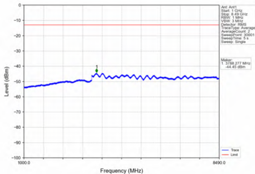
n5_30kHz_SISO_NTNV_20MHz_DFT-s-OFDM QPSK_839MHz_Inner_1RB_Right
