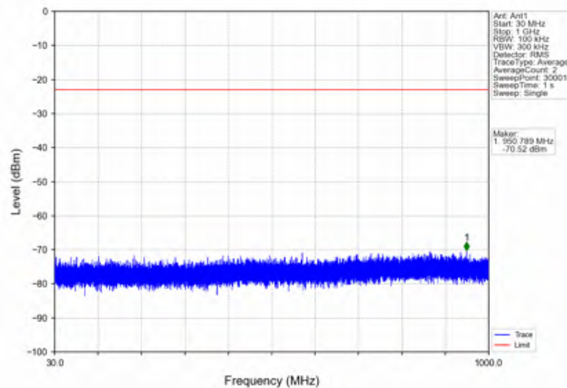
n7 15kHz SISO NTNV 5MHz DFT-s-OFDM PI/2 BPSK 2567.5MHz Outer Full
