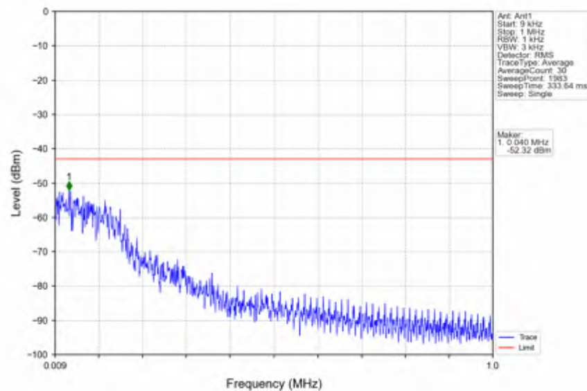
n5_15kHz_SISO_NTNV_20MHz_CP-OFDM QPSK_839MHz_Edge_1RB_Right
