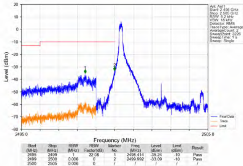
n7_15kHz_SISO_NTNV_5MHz_DFT-s-OFDM QPSK_2502.5MHz_Edge_1RB_Left
