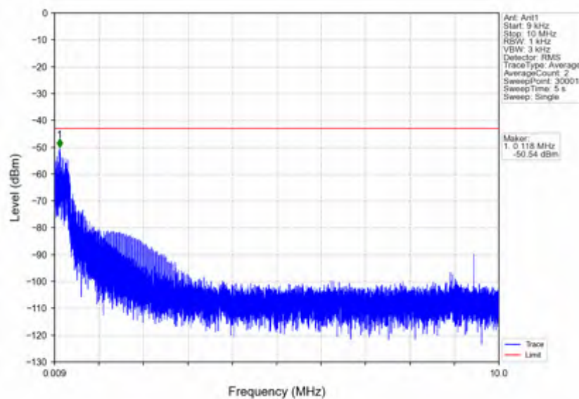
n5_30kHz_SISO_NTNV_20MHz_DFT-s-OFDM PI/2 BPSK_839MHz_Edge_1RB_Right
