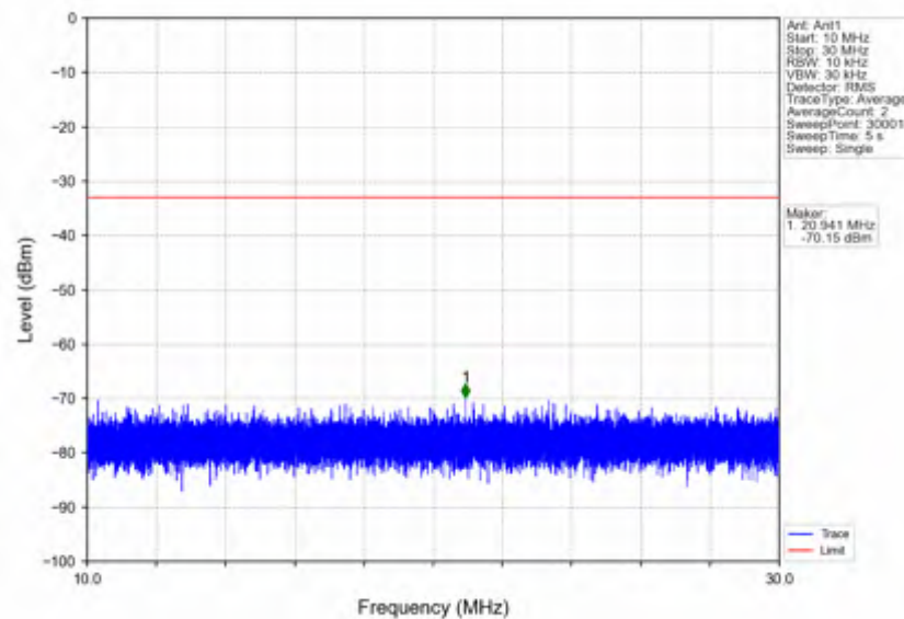
n5_30kHz_SISO_NTV_15MHz_CP-OFDM_QPSK_831.5MHz_Inner_1RB_Left
