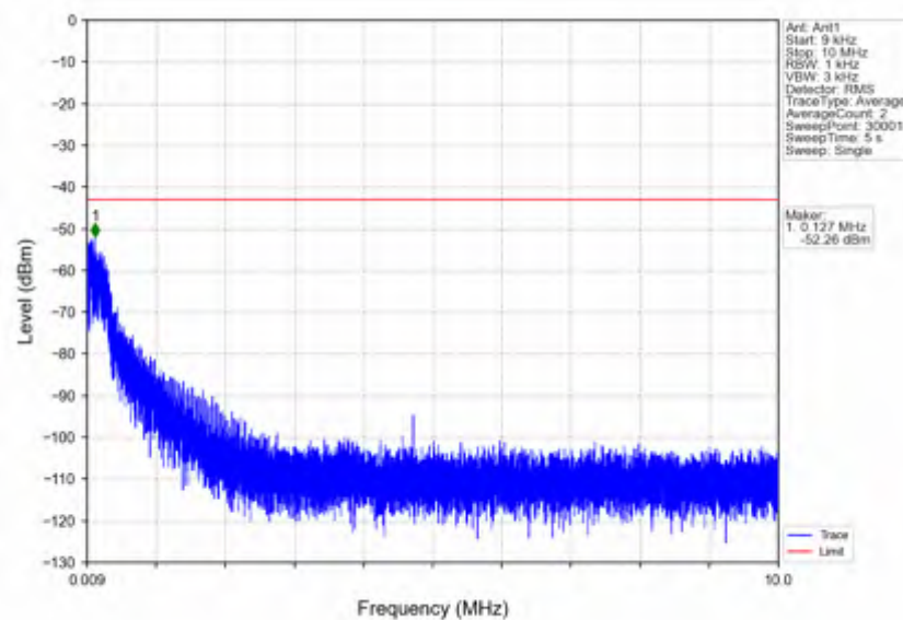
n5_30kHz_SISO_NTNV_10MHz_CP-OFDM_QPSK_829MHz_Inner_1RB_Left
