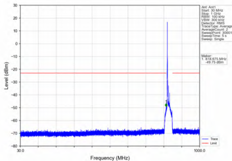
n5_30kHz_SISO_NTV_15MHz_CP-OFDM_QPSK_831.5MHz_Inner_1RB_Left
