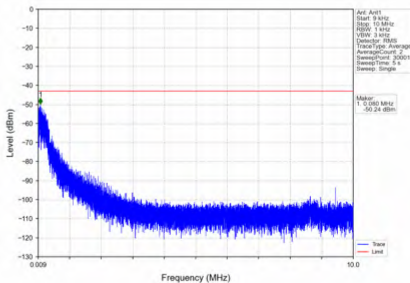
n5_30kHz_SISO_NTNV_20MHz_CP-OFDM_QPSK_839MHz_Inner_1RB_Right
