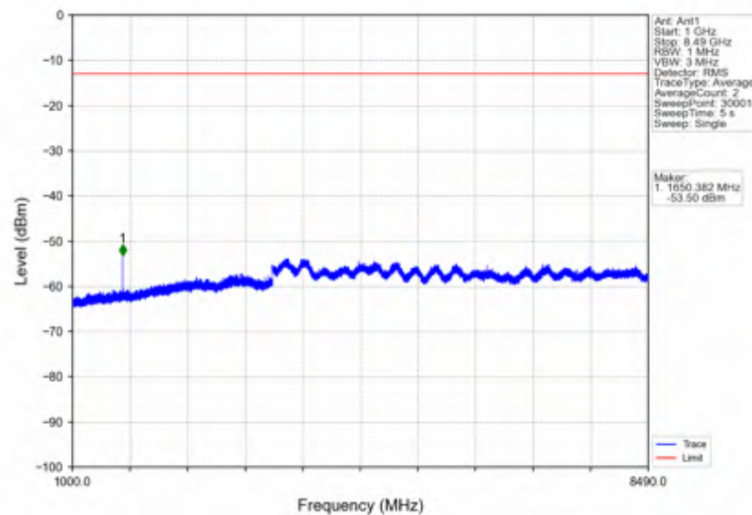
n5_30kHz_SISO_NTNV_10MHz_DFT-s-OFDM_PI/2_BPSK_836.5MHz_Edge_1RB_Left
