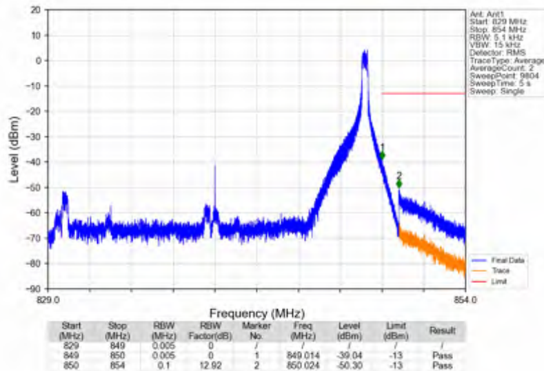
n5_30kHz_SISO_NTNV_20MHz_DFT-s-OFDM PI/2 BPSK_839MHz_Edge_1RB_Right
