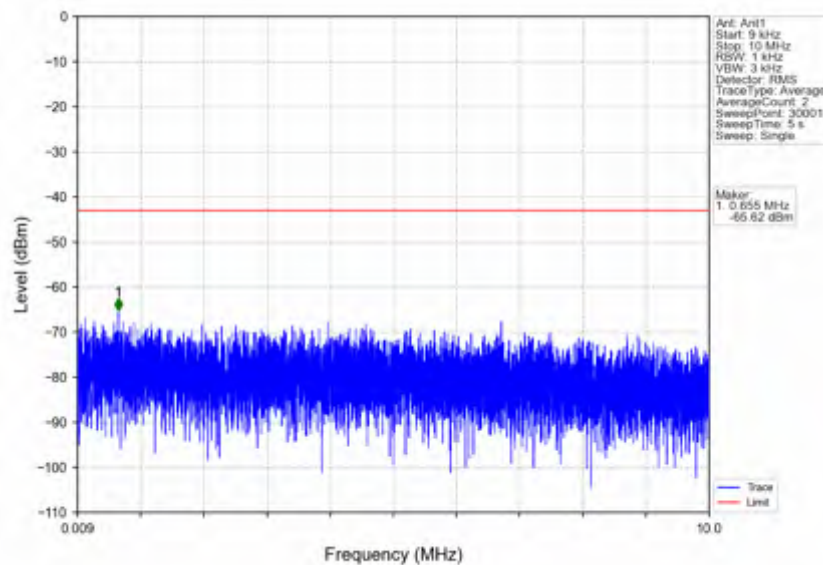
n5_30kHz_SISO_NTNV_20MHz_CP-OFDM QPSK_834MHz_Outer_Full
