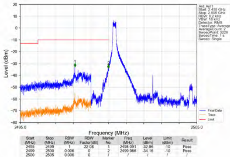
n7_15kHz_SISO_NTNV_5MHz_DFT-s-OFDM_PI/2_BPSK_2502.5MHz_Edge_1RB_Left
