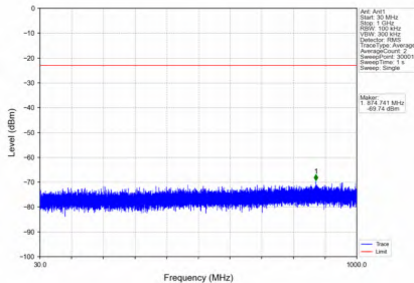
n7_15kHz_SISO_NTNV_5MHz_DFT-s-OFDM PI/2 BPSK_2502.5MHz_Edge_1RB_Left
