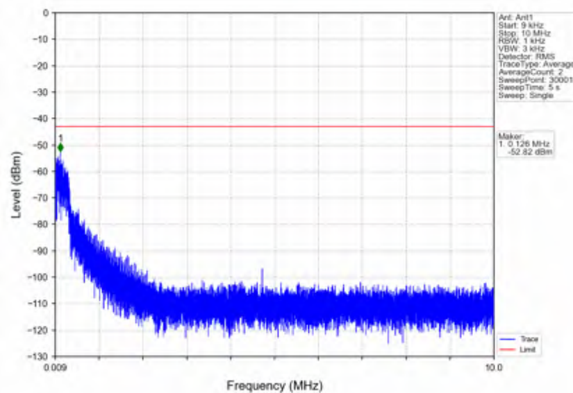
n5_30kHz_SISO_NTNV_10MHz_CP-OFDM_QPSK_829MHz_Edge_1RB_Left
