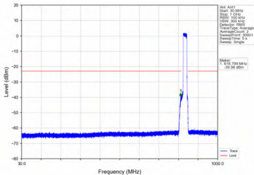
n5_30kHz_SISO_NTNV_20MHz_DFT-s-OFDM QPSK_839MHz_Outer_Full
