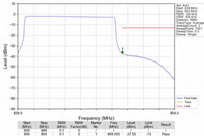
n5_30kHz_SISO_NTNV_10MHz_CP-OFDM QPSK_844MHz_Outer_Full
