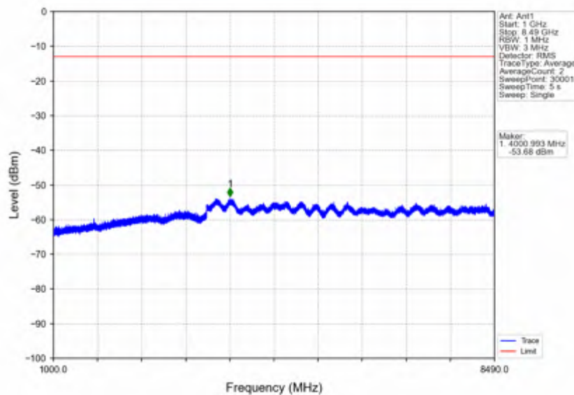
n5_30kHz_SISO_NTNV_10MHz_CP-OFDM QPSK_844MHz_Outer_Full
