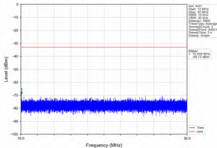
n5_30kHz_SISO_NTNV_15MHz_DFT-s-OFDM QPSK 841.5MHz Inner_1RB_Right
