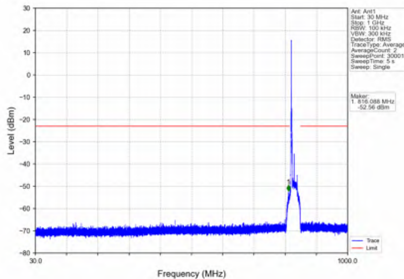
n5_30kHz_SISO_NTNV_20MHz_CP-OFDM_QPSK_834MHz_Edge_1RB_Left
