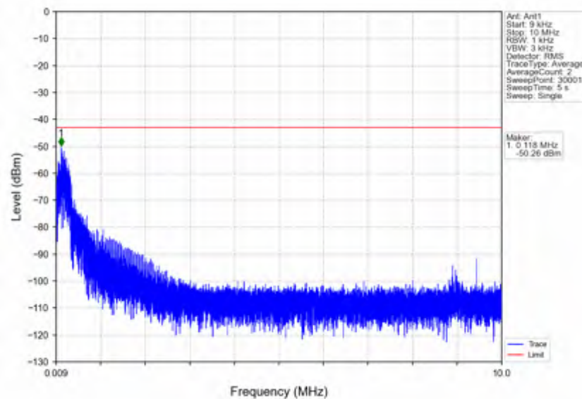
n5_30kHz_SISO_NTNV_20MHz_DFT-s-OFDM QPSK_839MHz_Edge_1RB_Right
