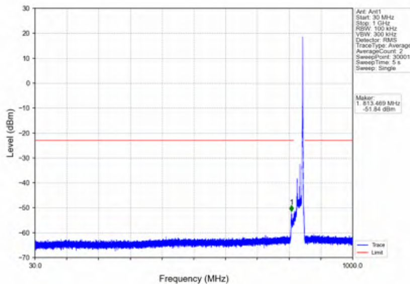
n5_30kHz_SISO_NTNV_20MHz_DFT-s-OFDM_QPSK_839MHz_Inner_1RB_Right
