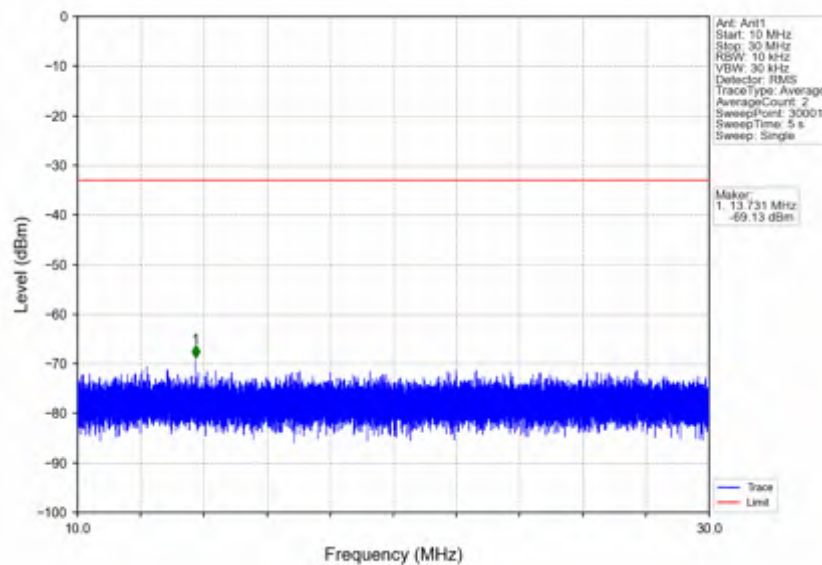
n5_30kHz_SISO_NTNV_20MHz_DFT-s-OFDM QPSK_834MHz_Outer_Full
