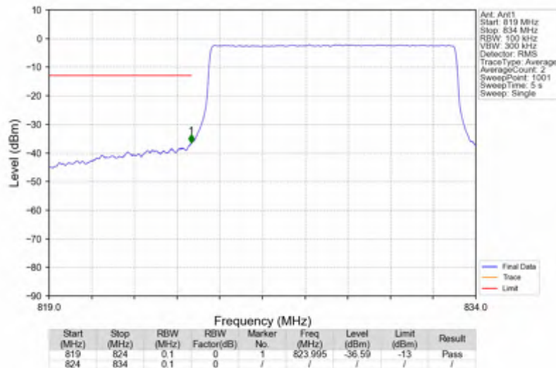
n5_30kHz_SISO_NTNV_10MHz_CP-OFDM QPSK_829MHz_Outer_Full
