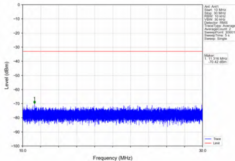
n5_30kHz_SISO_NTNV_20MHz_CP-OFDM_QPSK_834MHz_Edge_1RB_Left
