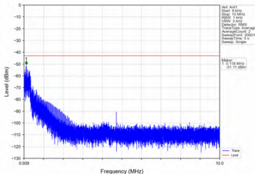
n5_30kHz_SISO_NTNV_10MHz_DFT-s-OFDM PI/2 BPSK 836.5MHz_Edge_1RB_Left
