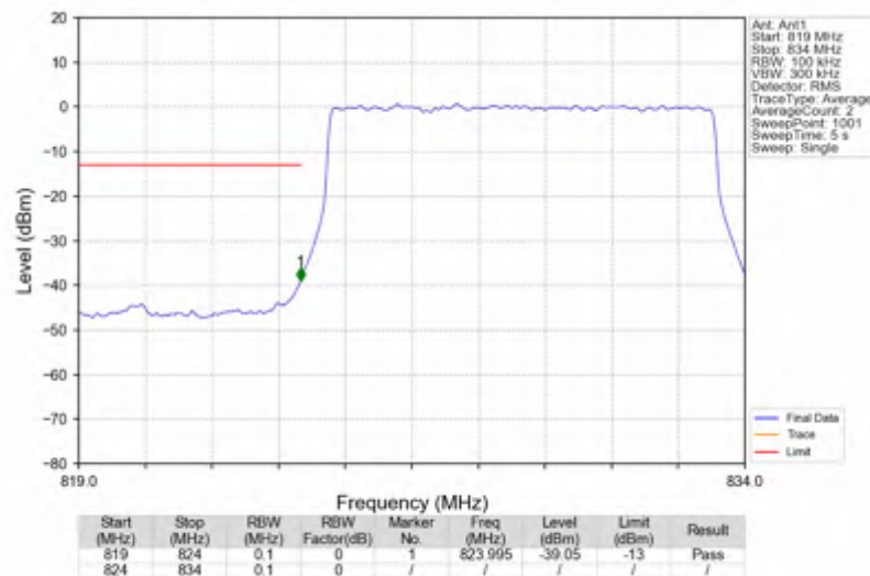
n5_30kHz_SISO_NTNV_10MHz_DFT-s-OFDM PI/2 BPSK_829MHz_Outer_Full
