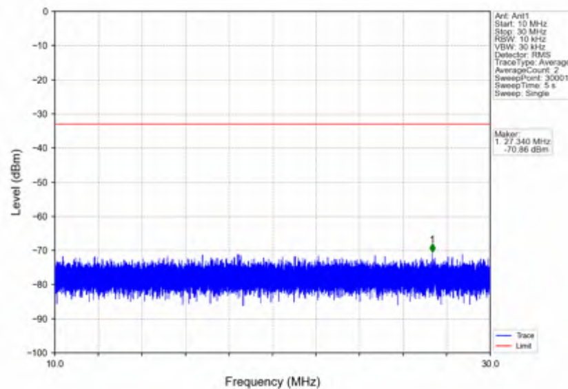
n5_30kHz_SISO_NTNV_10MHz_CP-OFDM_QPSK_829MHz_Inner_1RB_Left
