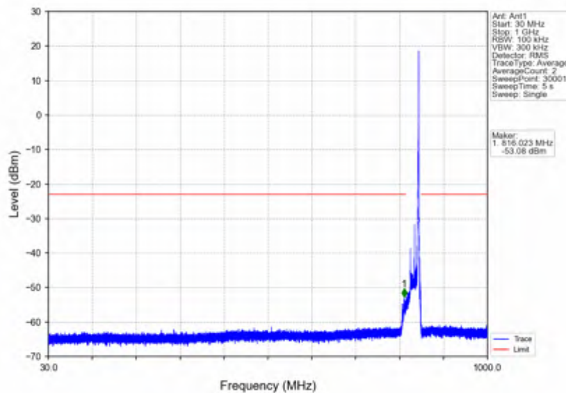
n5_30kHz_SISO_NTNV_20MHz_DFT-s-OFDM_QPSK_839MHz_Edge_1RB_Right
