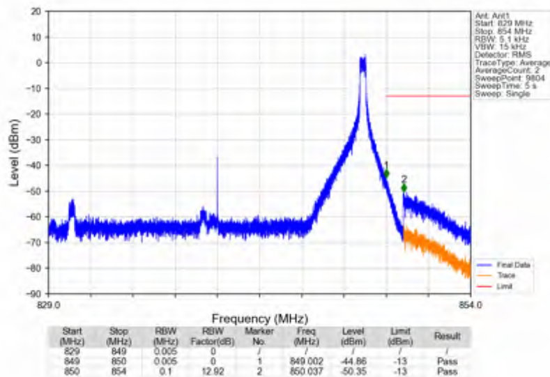
n5_30kHz_SISO_NTNV_20MHz_CP-OFDM_QPSK_839MHz_Inner_1RB_Right
