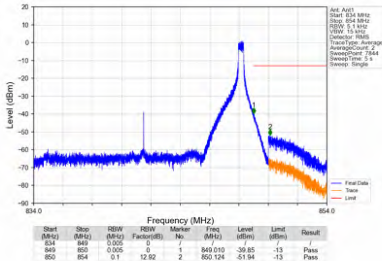
n5_30kHz_SISO_NTNV_15MHz_CP-OFDM QPSK_841.5MHz_Edge_1RB_Right
