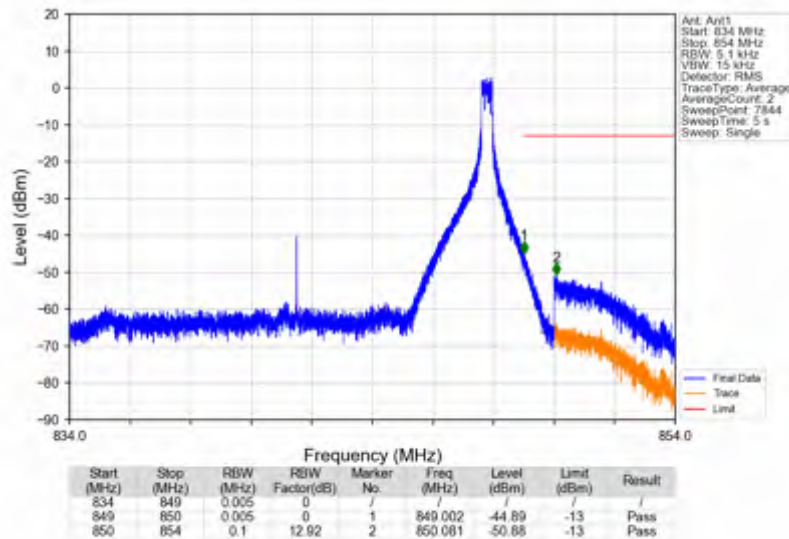
n5_30kHz_SISO_NTNV_15MHz_CP-OFDM QPSK_841.5MHz_Inner_1RB_Right
