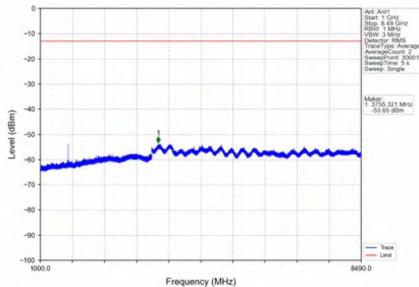
n5_30kHz_SISO_NTNV_10MHz_DFT-s-OFDM PI/2 BPSK_829MHz_Outer_Full
