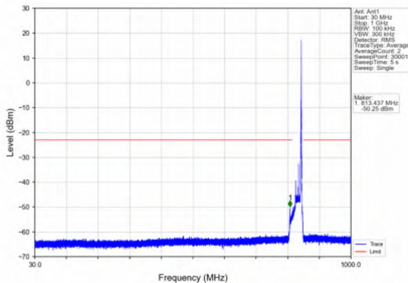
n5_30kHz_SISO_NTNV_20MHz_CP-OFDM QPSK_839MHz_Inner_1RB_Right
