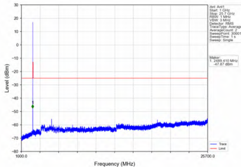
n7_15kHz_SISO_NTNV_5MHz_DFT-s-OFDM PI/2 BPSK_2502.5MHz_Outer_Full
