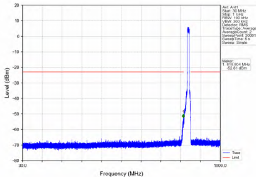
n5_30kHz_SISO_NTNV_10MHz_DFT-s-OFDM QPSK_844MHz_Outer_Full
