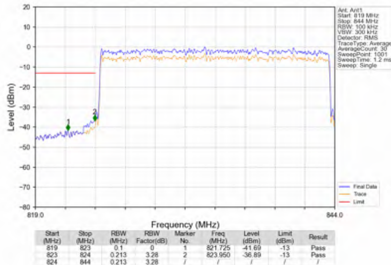
n5_15kHz_SISO_NTNV_20MHz_CP-OFDM QPSK_834MHz_Outer_Full
