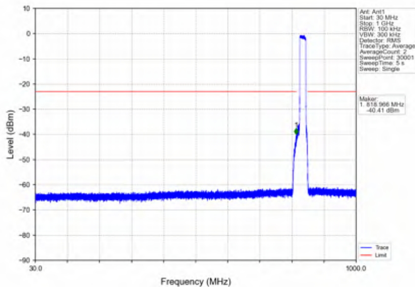
n5_30kHz_SISO_NTNV_20MHz_CP-OFDM_QPSK_839MHz_Outer_Full
