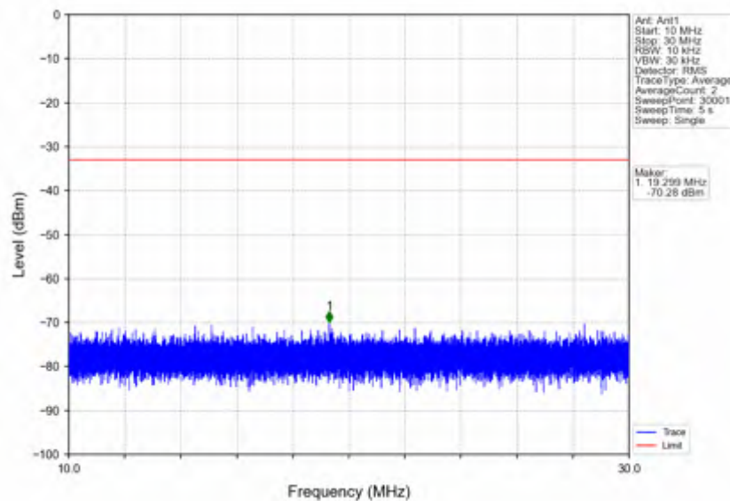
n5_30kHz_SISO_NTNV_10MHz_DFT-s-OFDM QPSK_829MHz_Outer_Full
