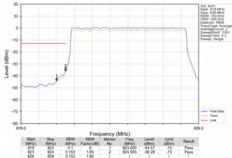
n5_30kHz_SISO_NTNV_15MHz_DFT-s-OFDM PI/2 BPSK_831.5MHz_Outer_Full
