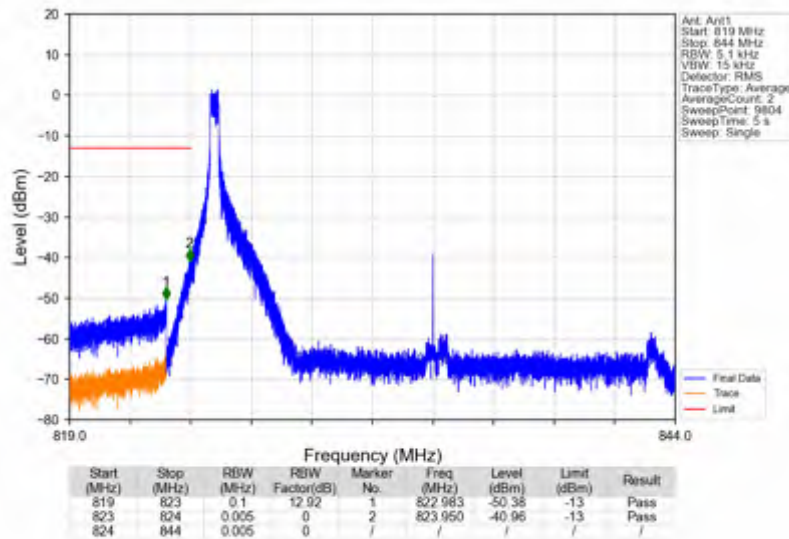
n5_30kHz_SISO_NTNV_20MHz_CP-OFDM_QPSK_834MHz_Edge_1RB_Left
