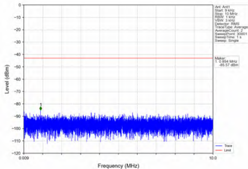
n7_15kHz_SISO_NTNV_5MHz_DFT-s-OFDM PI/2 BPSK_2502.5MHz_Outer_Full
