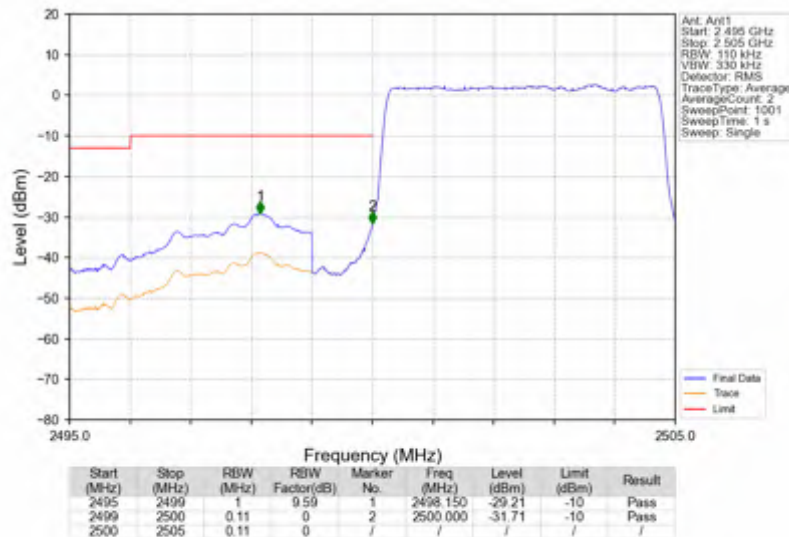
n7_15kHz_SISO_NTNV_5MHz_DFT-s-OFDM PI/2 BPSK_2502.5MHz_Outer_Full
