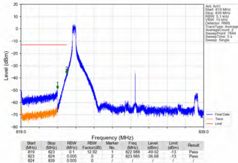
n5_30kHz_SISO_NTNV_15MHz_DFT-s-OFDM QPSK_831.5MHz_Edge_1RB_Left
