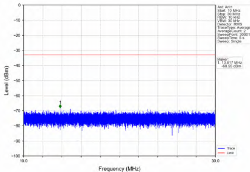
n5_30kHz_SISO_NTNV_20MHz_CP-OFDM QPSK_839MHz_Outer_Full
