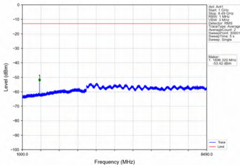
n5_30kHz_SISO_NTNV_15MHz_DFT-s-OFDM QPSK 841.5MHz_Edge_1RB_Right
