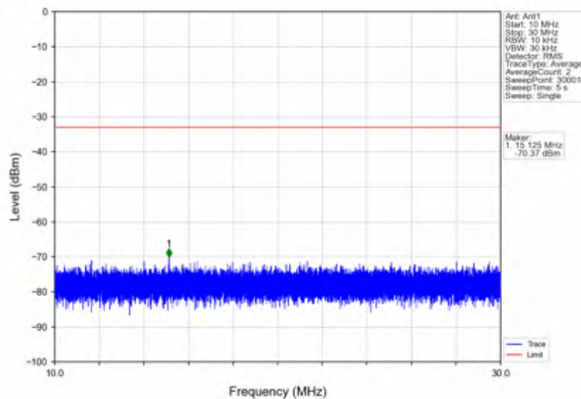
n5_30kHz_SISO_NTNV_10MHz_DFT-s-OFDM QPSK_844MHz_Outer_Full
