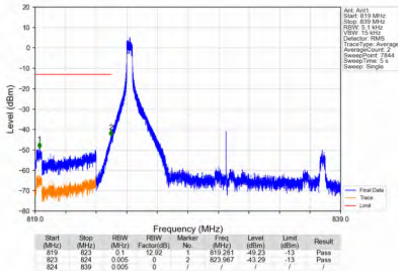
n5_30kHz_SISO_NTNV_15MHz_DFT-s-OFDM_QPSK_831.5MHz_Inner_1RB_Left
