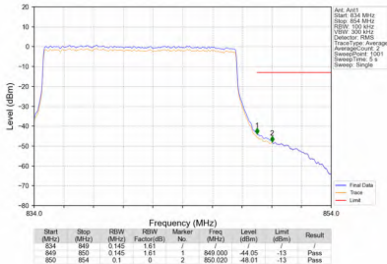
n5_30kHz_SISO_NTNV_15MHz_DFT-s-OFDM PI/2 BPSK_841.5MHz_Outer_Full
