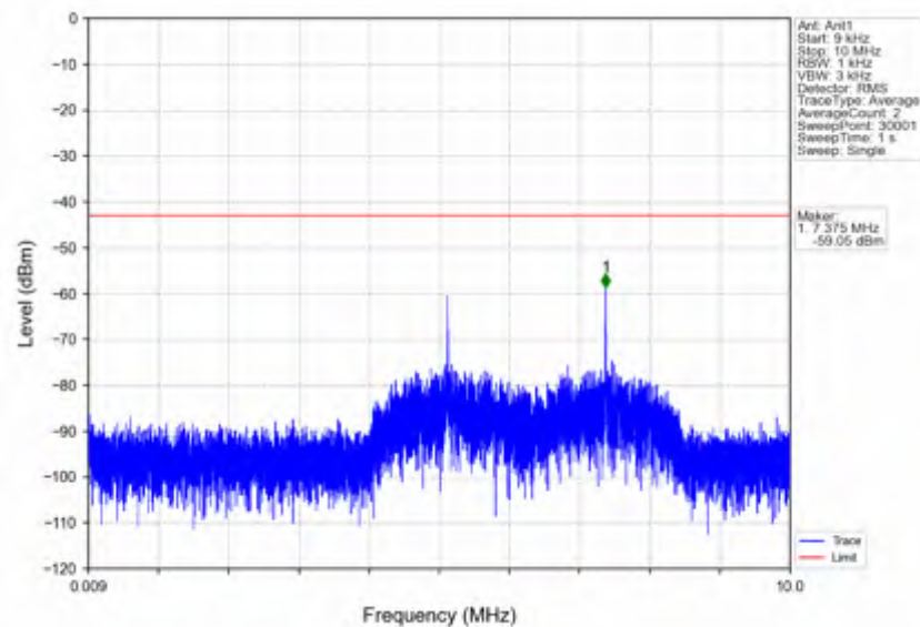
n7_15kHz_SISO_NTNV_5MHz_DFT-s-OFDM PI/2 BPSK_2567.5MHz_Outer_Full
