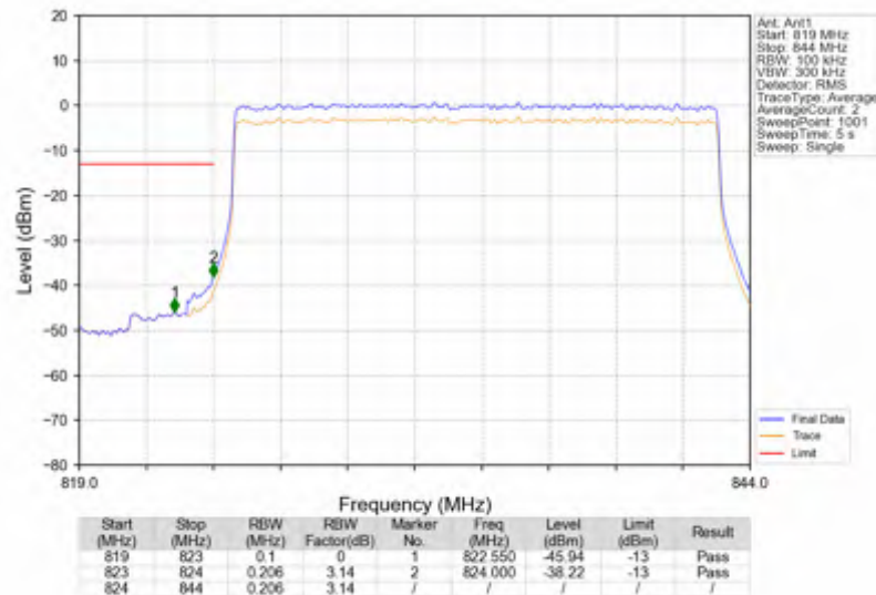
n5_30kHz_SISO_NTNV_20MHz_DFT-s-OFDM PI/2 BPSK_834MHz_Outer_Full
