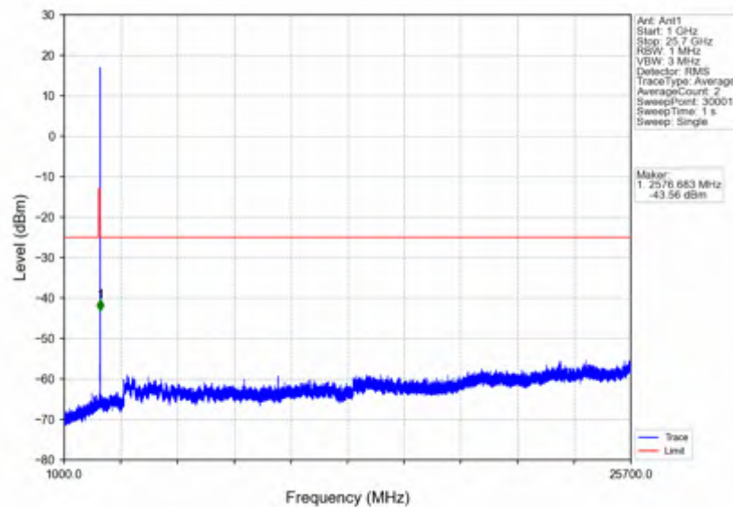
n7 15kHz SISO NTNV 5MHz DFT-s-OFDM PI/2 BPSK 2567.5MHz Outer Full
