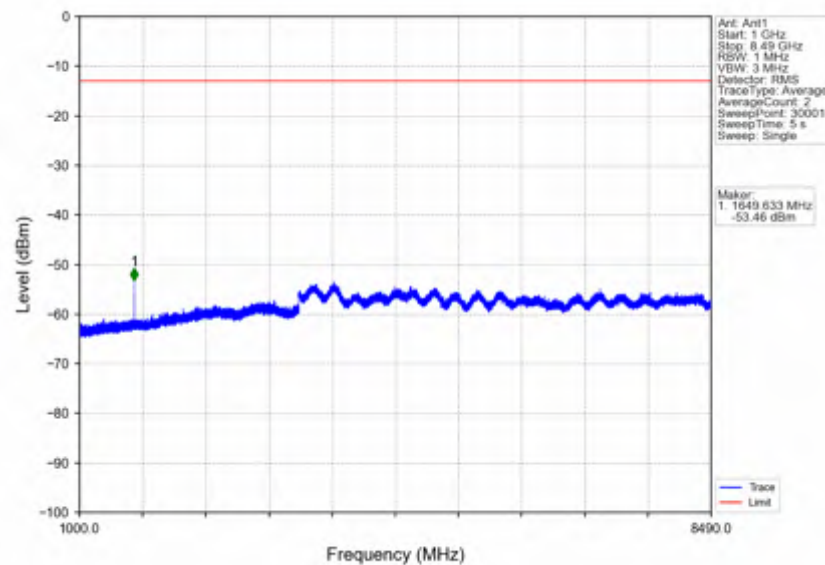
n5_30kHz_SISO_NTNV_15MHz_DFT-s-OFDM PI/2 BPSK_831.5MHz_Outer_Full
