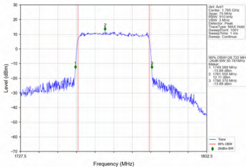
n66_15kHz_SISO_NTNV_30MHz_CP-OFDM QPSK_1765MHz_Outer_Full
