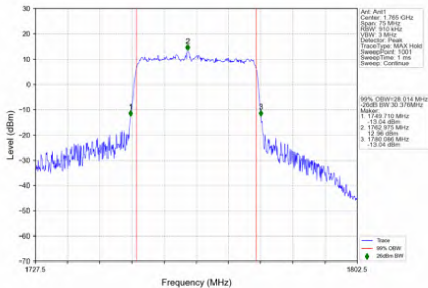
n66_30kHz_SISO_NTV_30MHz_CP-OFDM_QPSK_1765MHz_Outer_Full
