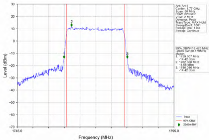
n66_30kHz_SISO_NTNV_20MHz_CP-OFDM 64 QAM_1770MHz_Outer_Full
