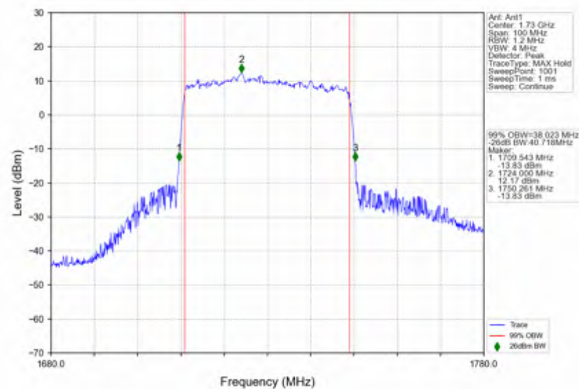
n66 30kHz SISO NTN 40MHz CP-OFDM 64 QAM 1730MHz Outer Full
