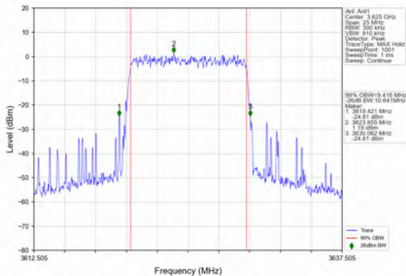
n78d_15kHz_SISO_NTNV_10MHz_CP-OFDM_16_QAM_3625.005MHz_Outer_Full
