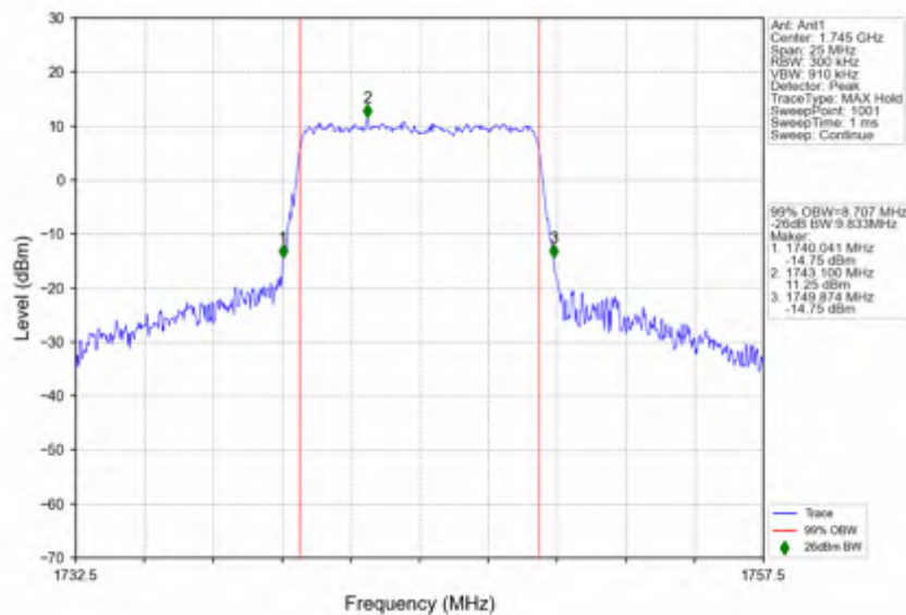
n66_30kHz_SISO_NTNV_10MHz_CP-OFDM_16_QAM_1745MHz_Outer_Full
