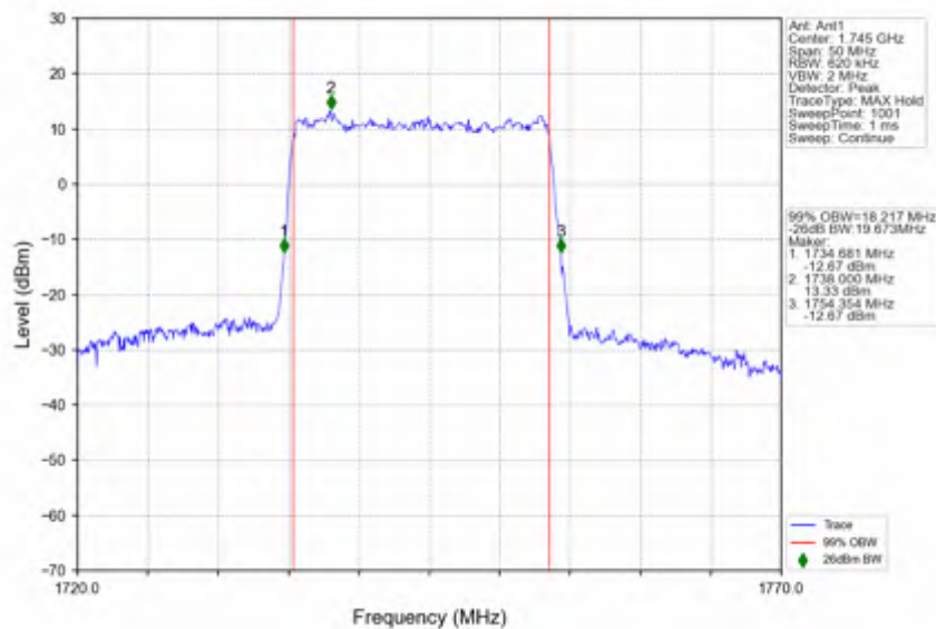
n66_15kHz_SISO_NTNV_20MHz_DFT-s-OFDM_16_QAM_1745MHz_Outer_Full
