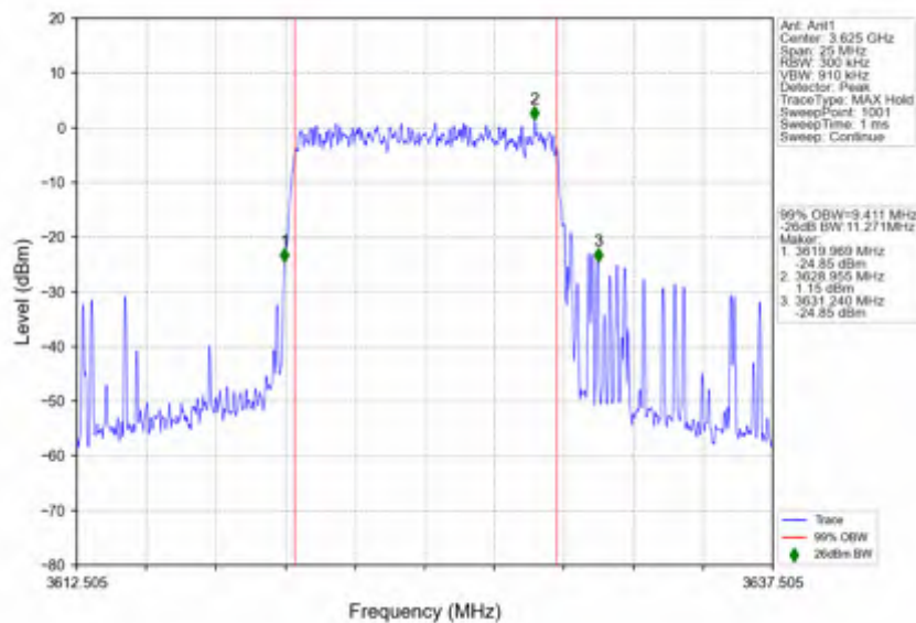
n78d_15kHz_SISO_NTNV_10MHz_CP-OFDM_256_QAM_3625.005MHz_Outer_Full
