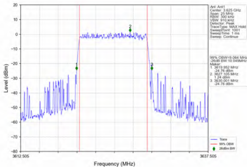
n78d_15kHz_SISO_NTNV_10MHz_DFT-s-OFDM_16_QAM_3625.005MHz_Outer_Full
