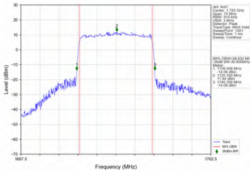
n66_15kHz_SISO_NTNV_30MHz_CP-OFDM QPSK_1725MHz_Outer_Full
