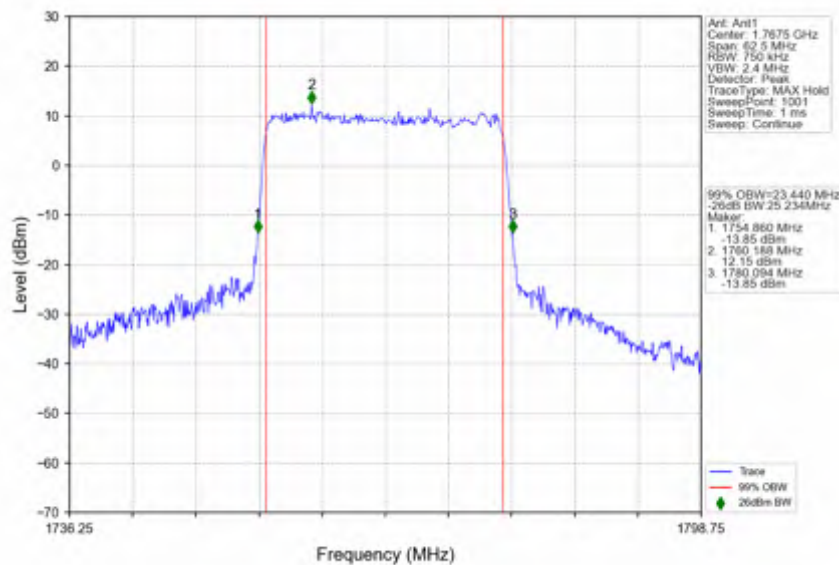
n66_30kHz_SISO_NTNV_25MHz_CP-OFDM 64 QAM_1767.5MHz_Outer_Full
