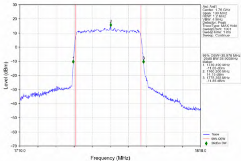
n66_30kHz_SISO_NTNV_40MHz_DFT-s-OFDM_QPSK_1760MHz_Outer_Full
