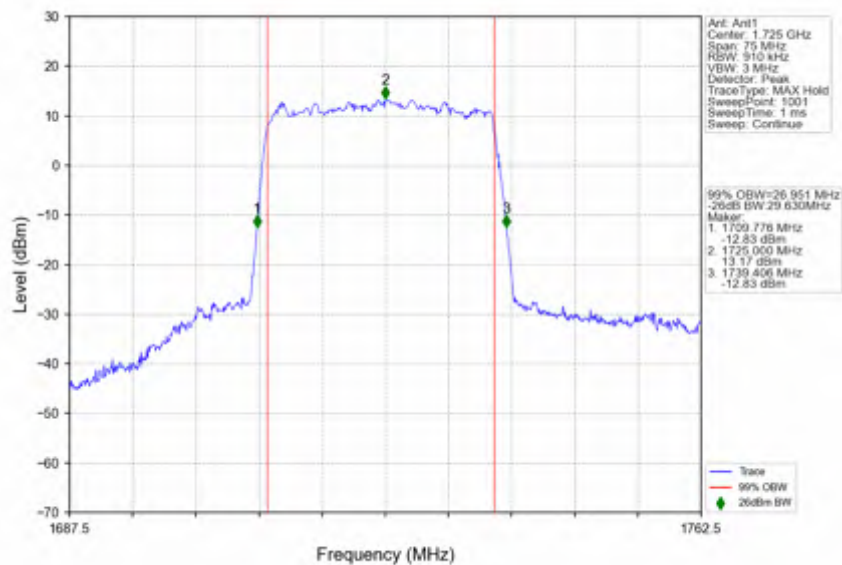
n66_30kHz_SISO_NTNV_30MHz_DFT-s-OFDM_QPSK_1725MHz_Outer_Full
