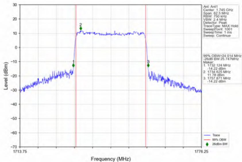
n66_15kHz_SISO_NTNV_25MHz_CP-OFDM_16 QAM_1745MHz_Outer_Full
