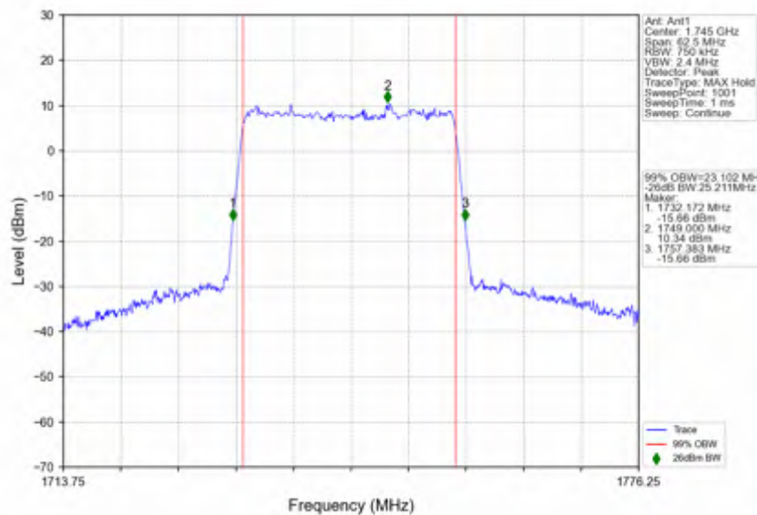
n66_30kHz_SISO_NTNV_25MHz_DFT-s-OFDM_256_QAM_1745MHz_Outer_Full
