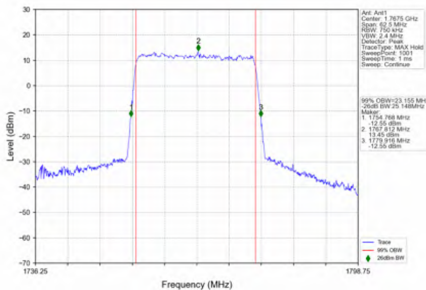
n66 30kHz SISO NTV 25MHz DFT-s-OFDM QPSK 1767.5MHz Outer Full
