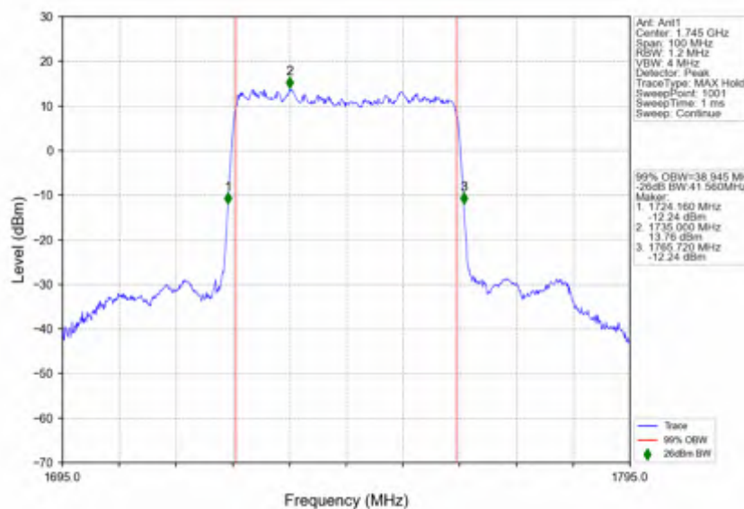
n66_15kHz_SISO_NTNV_40MHz_DFT-s-OFDM_PI/2_BPSK_1745MHz_Outer_Full
