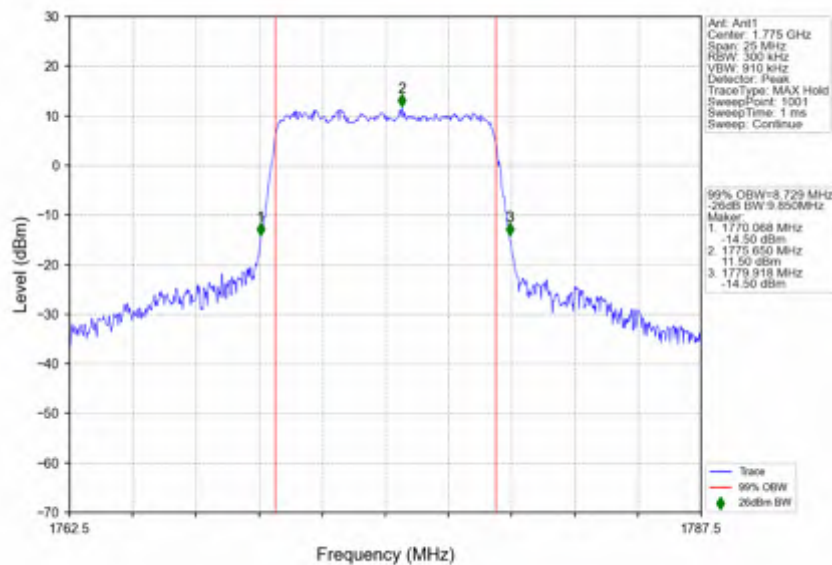
n66_30kHz_SISO_NTNV_10MHz_CP-OFDM QPSK_1775MHz_Outer_Full
