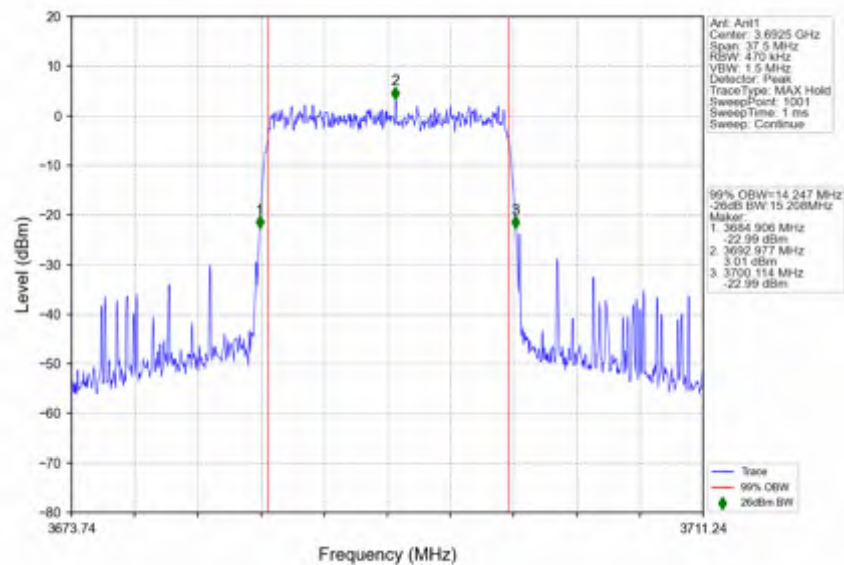
n78d_15kHz_SISO_NTNV_15MHz_CP-OFDM 64 QAM_3692.49MHz_Outer_Full
