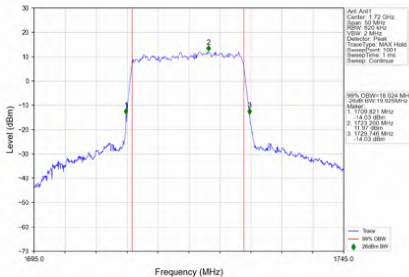
n66_30kHz_SISO_NTNV_20MHz_DFT-s-OFDM_64 QAM_1720MHz_Outer_Full
