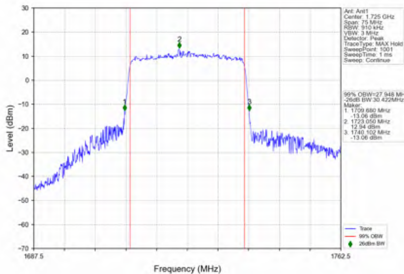
n66_30kHz_SISO_NTNV_30MHz_CP-OFDM QPSK_1725MHz_Outer_Full
