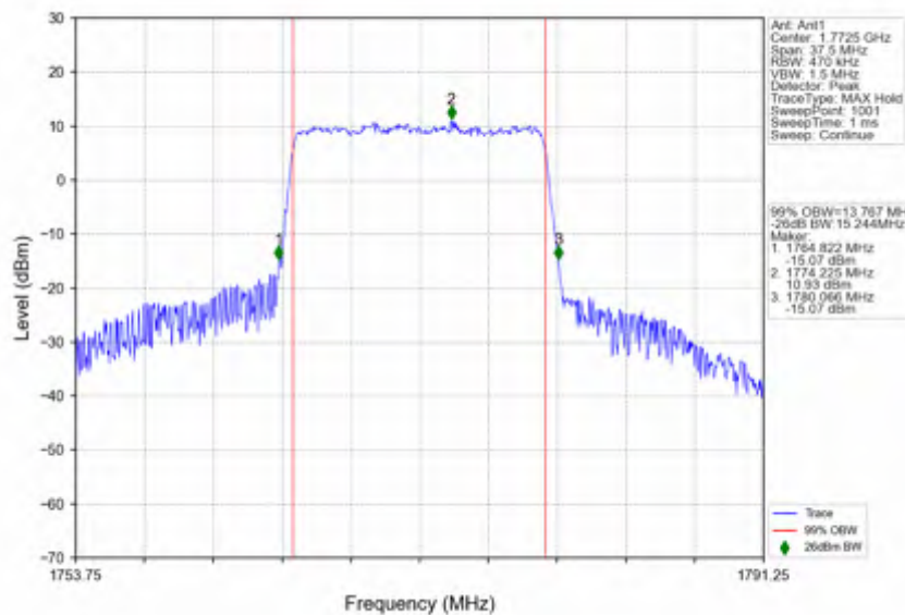
n66_30kHz_SISO_NTNV_15MHz_CP-OFDM 64 QAM_1772.5MHz_Outer_Full
