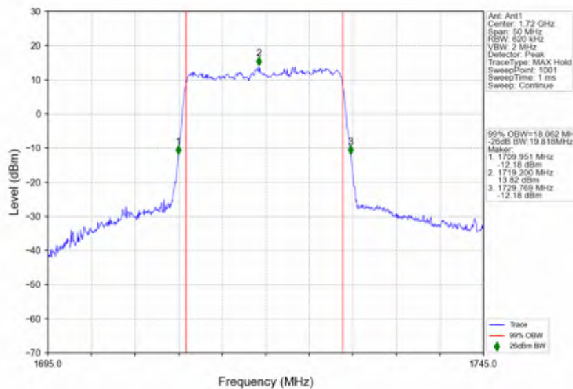
n66_30kHz_SISO_NTNV_20MHz_DFT-s-OFDM QPSK_1720MHz_Outer_Full
