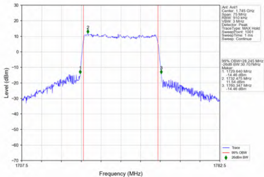
n66_30kHz_SISO_NTNV_30MHz_CP-OFDM_16_QAM_1745MHz_Outer_Full
