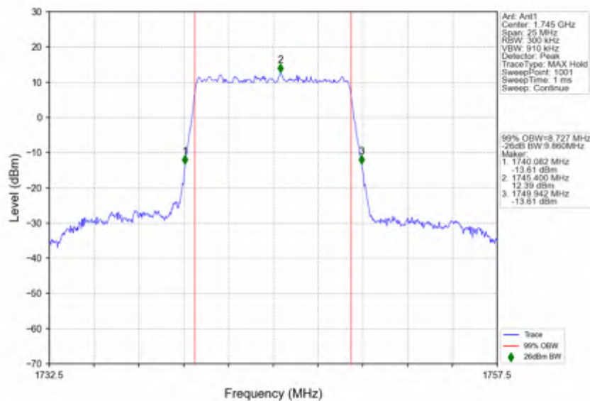
n66_30kHz_SISO_NTNV_10MHz_DFT-s-OFDM_16 QAM_1745MHz_Outer_Full
