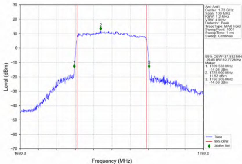
n66_30kHz_SISO_NTNV_40MHz_CP-OFDM QPSK_1730MHz_Outer_Full
