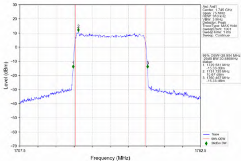
n66_15kHz_SISO_NTNV_30MHz_DFT-s-OFDM_256_QAM_1745MHz_Outer_Full
