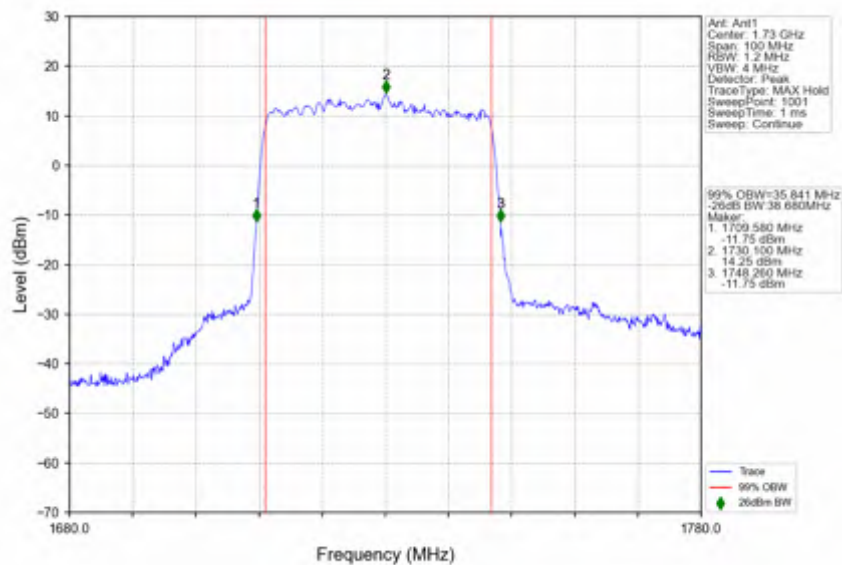
n66_30kHz_SISO_NTNV_40MHz_DFT-s-OFDM_QPSK_1730MHz_Outer_Full
