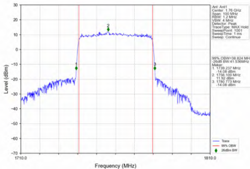
n66_15kHz_SISO_NTNV_40MHz_CP-OFDM QPSK_1760MHz_Outer_Full
