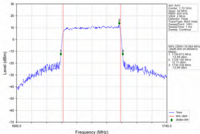
n66_15kHz_SISO_NTNV_20MHz_CP-OFDM QPSK_1720MHz_Outer_Full
