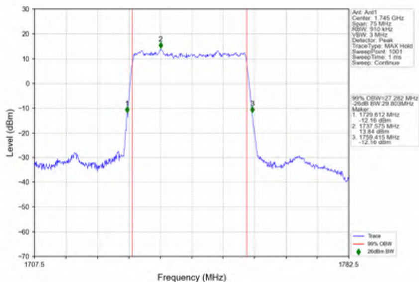
n66_30kHz_SISO_NTNV_30MHz_DFT-s-OFDM_PI/2_BPSK_1745MHz_Outer_Full
