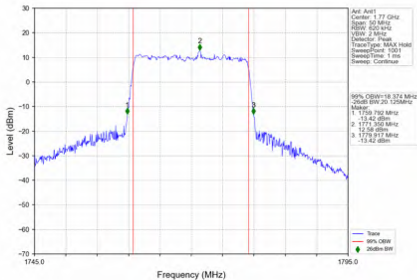
n66_30kHz_SISO_NTNV_20MHz_CP-OFDM_QPSK_1770MHz_Outer_Full
