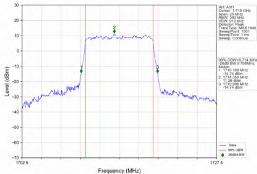
n66_30kHz_SISO_NTNV_10MHz_CP-OFDM_64 QAM_1715MHz_Outer_Full
