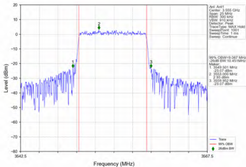
n78d_15kHz_SISO_NTNV_10MHz_DFT-s-OFDM 64 QAM_3555MHz_Outer_Full
