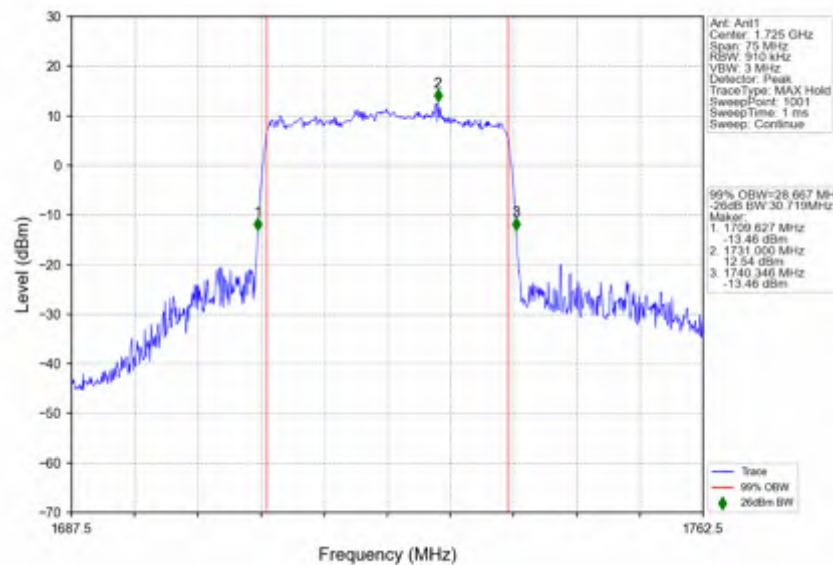
n66_15kHz_SISO_NTNV_30MHz_CP-OFDM 64 QAM_1725MHz_Outer_Full
