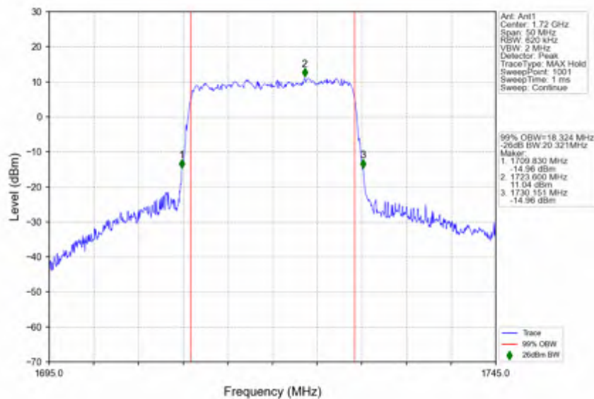
n66_30kHz_SISO_NTNV_20MHz_CP-OFDM_64_QAM_1720MHz_Outer_Full
