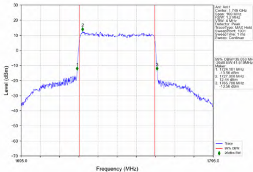
n66_15kHz_SISO_NTNV_40MHz_CP-OFDM_16_QAM_1745MHz_Outer_Full
