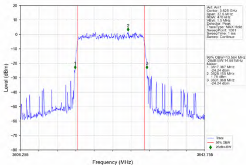
n78d_15kHz_SISO_NTNV_15MHz_DFT-s-OFDM_PI/2_BPSK_3625.005MHz_Outer_Full
