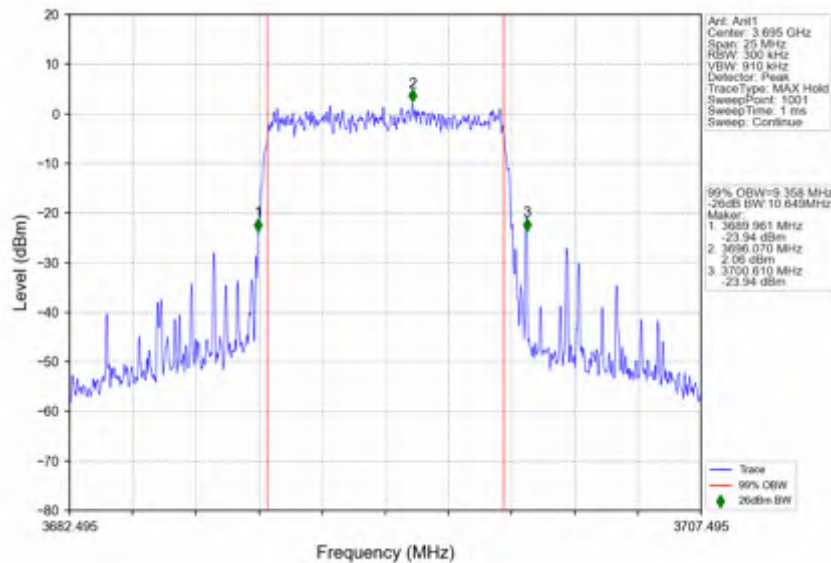
n78d_15kHz_SISO_NTNV_10MHz_CP-OFDM_64_QAM_3694.995MHz_Outer_Full
