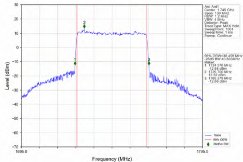
n66_30kHz_SISO_NTNV_40MHz_CP-OFDM_16_QAM_1745MHz_Outer_Full
