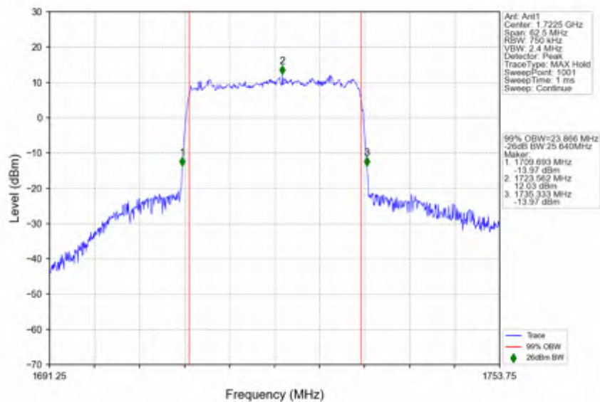
n66_15kHz_SISO_NTNV_25MHz_CP-OFDM_QPSK_1722.5MHz_Outer_Full
