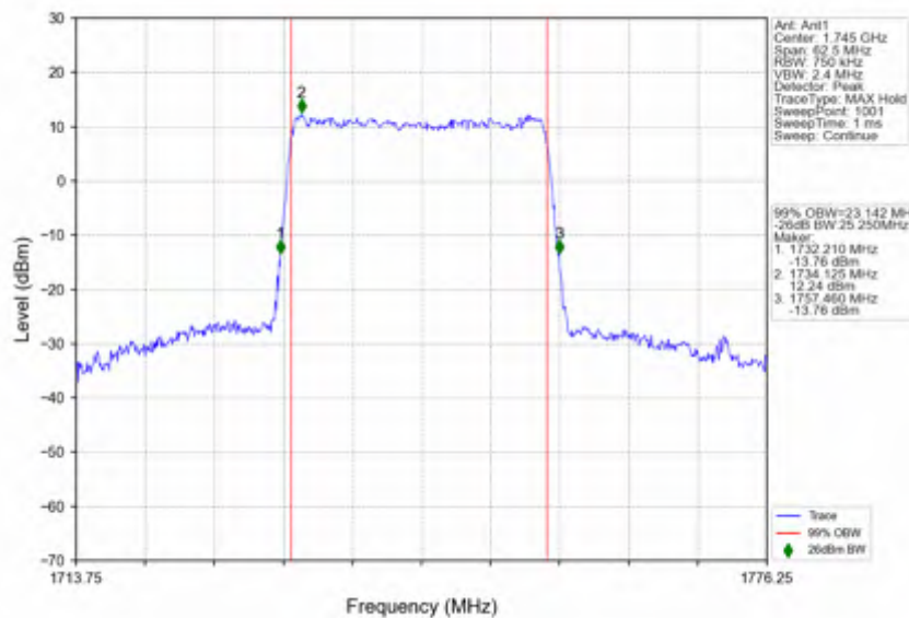
n66 30kHz SISO NTNv 25MHz DFT-s-OFDM 16 QAM 1745MHz Outer Full
