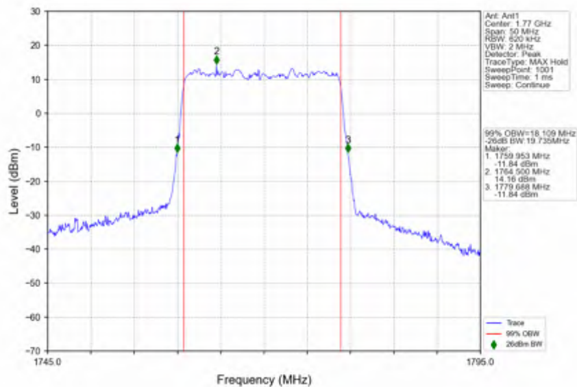
n66_30kHz_SISO_NTNV_20MHz_DFT-s-OFDM QPSK_1770MHz_Outer_Full
