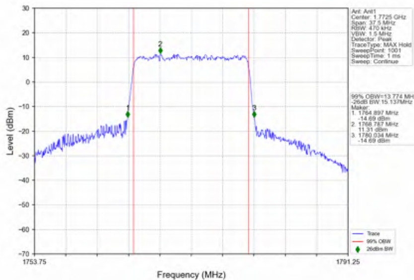
n66 30kHz SISO NTN 15MHz CP-OFDM QPSK 1772.5MHz Outer Full
