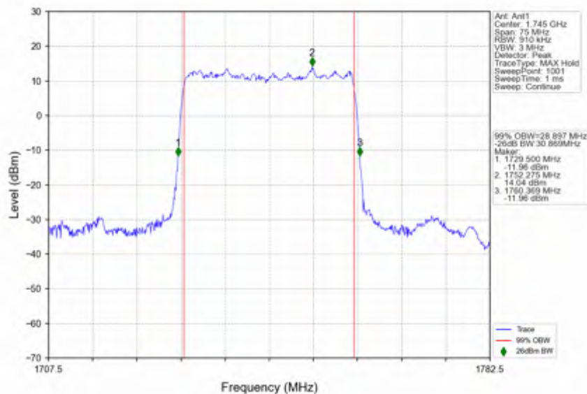
n66_15kHz_SISO_NTNV_30MHz_DFT-s-OFDM_PI/2_BPSK_1745MHz_Outer_Full
