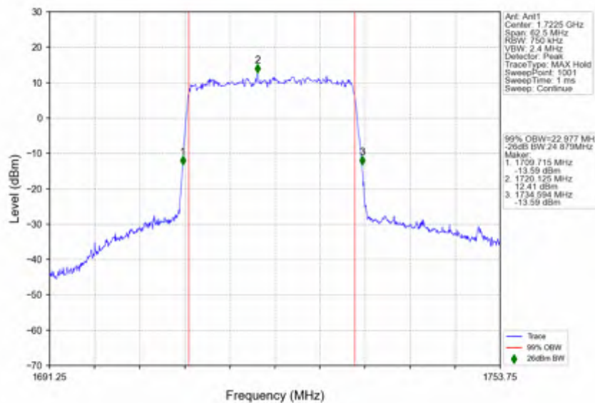
n66_15kHz_SISO_NTV_25MHz_DFT-s-OFDM_64 QAM_1722.5MHz_Outer_Full
