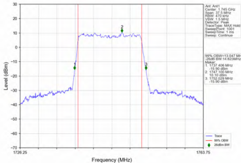
n66_30kHz_SISO_NTNV_15MHz_DFT-s-OFDM_256_QAM_1745MHz_Outer_Full
