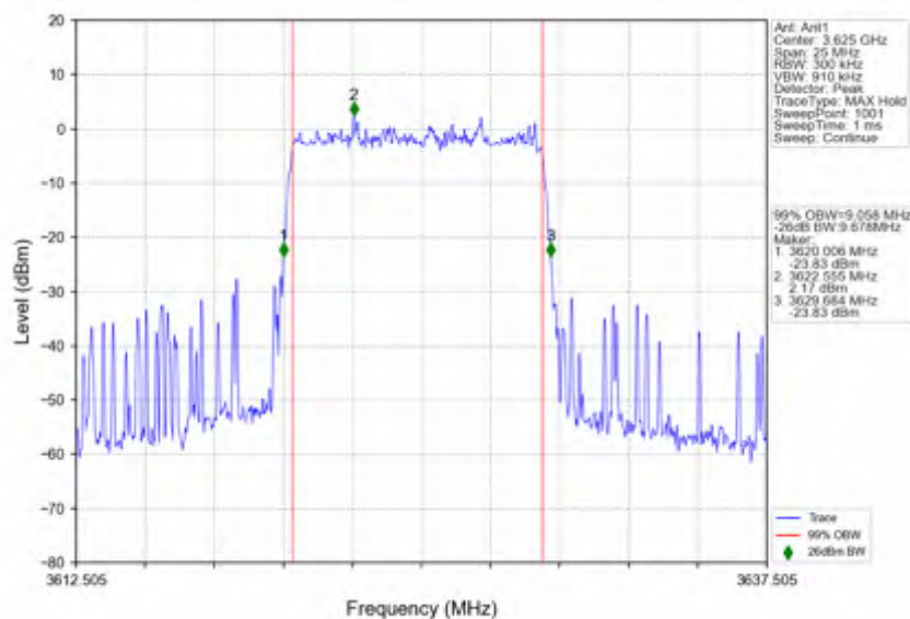
n78d_15kHz_SISO_NTNV_10MHz_DFT-s-OFDM PI/2 BPSK_3625.005MHz_Outer_Full
