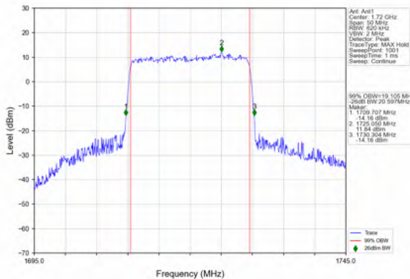
n66_15kHz_SISO_NTNV_20MHz_CP-OFDM 64 QAM_1720MHz_Outer_Full
