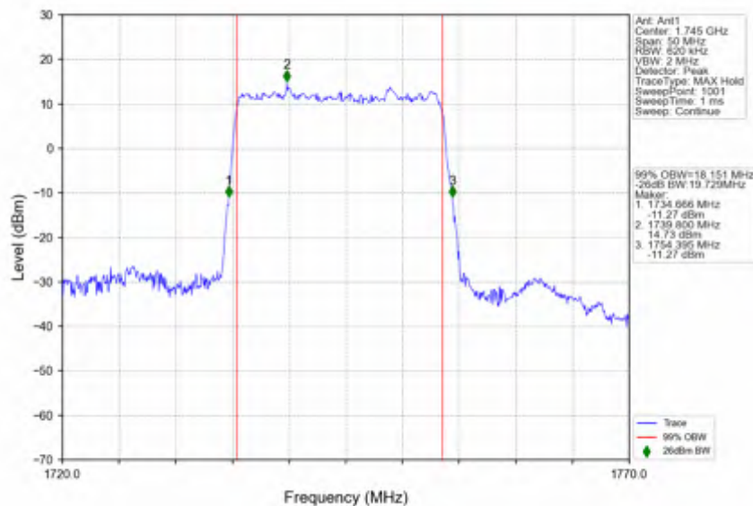
n66_15kHz_SISO_NTNV_20MHz_DFT-s-OFDM_PI/2_BPSK_1745MHz_Outer_Full
