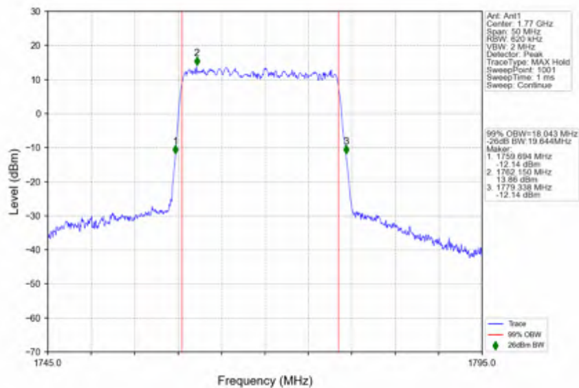
n66_15kHz_SISO_NTNV_20MHz_DFT-s-OFDM QPSK_1770MHz_Outer_Full
