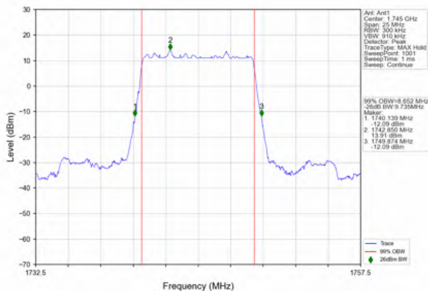
n66_30kHz_SISO_NTNV_10MHz_DFT-s-OFDM_PI/2_BPSK_1745MHz_Outer_Full
