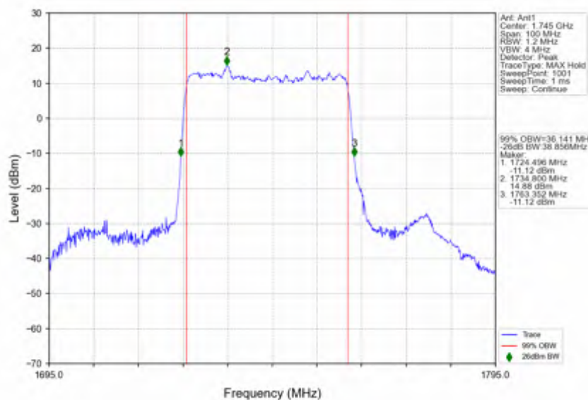
n66_30kHz_SISO_NTNV_40MHz_DFT-s-OFDM_PI/2_BPSK_1745MHz_Outer_Full
