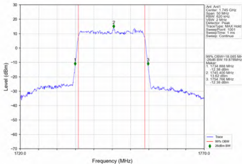
n66_30kHz_SISO_NTNV_20MHz_DFT-s-OFDM_16_QAM_1745MHz_Outer_Full
