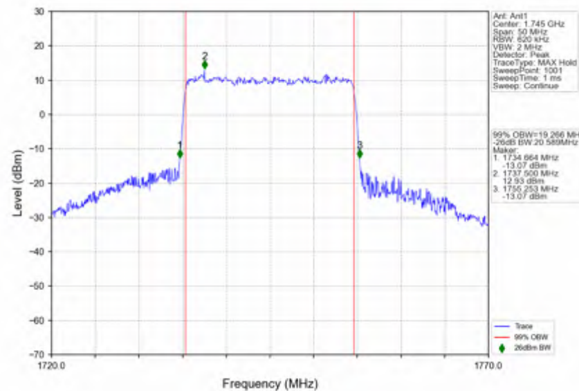
n66_15kHz_SISO_NTNV_20MHz_CP-OFDM_16_QAM_1745MHz_Outer_Full
