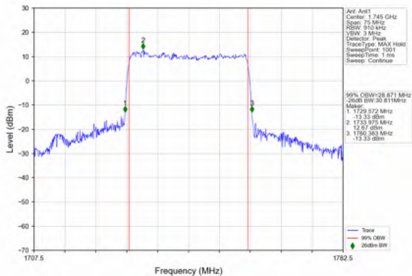
n66_15kHz_SISO_NTNV_30MHz_CP-OFDM_16_QAM_1745MHz_Outer_Full
