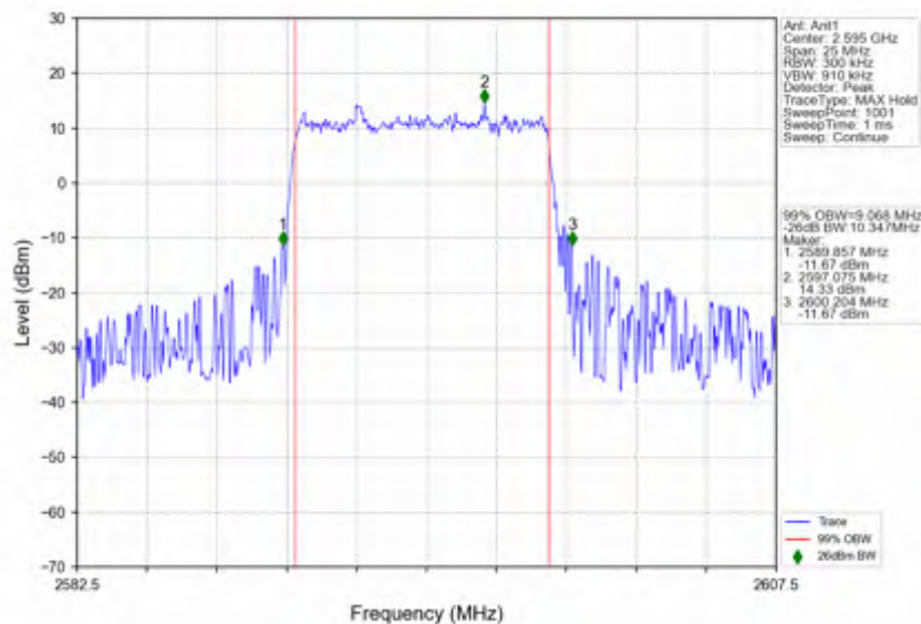
n38_15kHz_SISO_NTNV_10MHz_DFT-s-OFDM_PI/2_BPSK_2595MHz_Outer_Full
