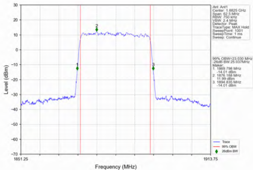
n25_30kHz_SISO_NTV_25MHz_DFT-s-OFDM_16_QAM_1882.5MHz_Outer_Full
