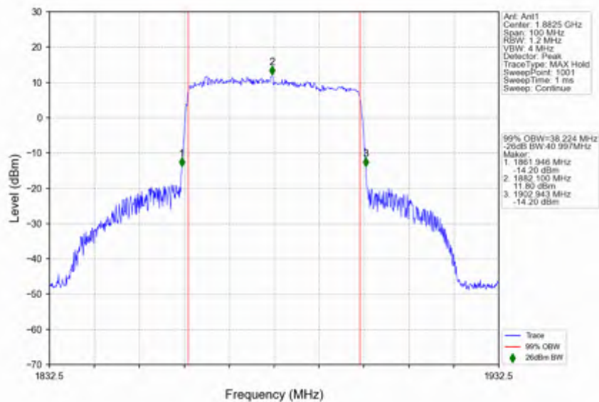
n25_30kHz_SISO_NTNV_40MHz_CP-OFDM 16 QAM_1882.5MHz_Outer_Full
