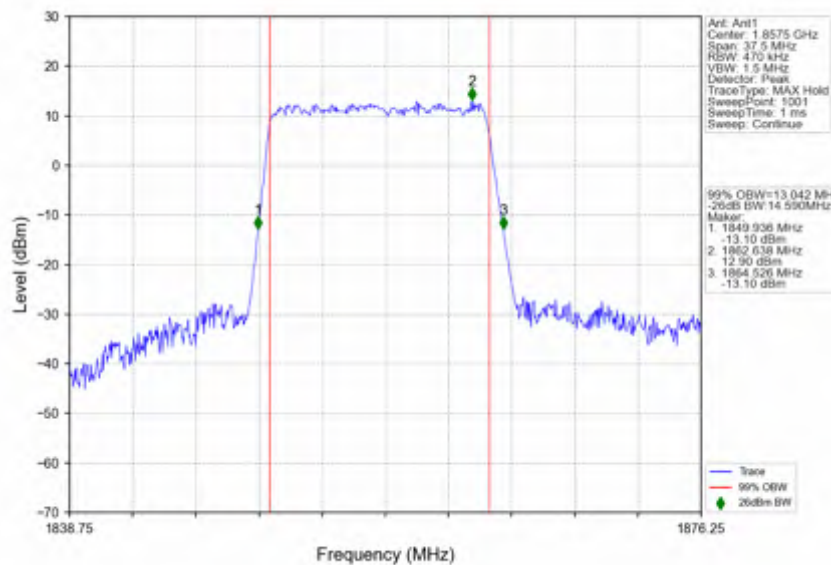
n25_30kHz_SISO_NTNV_15MHz_DFT-s-OFDM QPSK_1857.5MHz_Outer_Full
