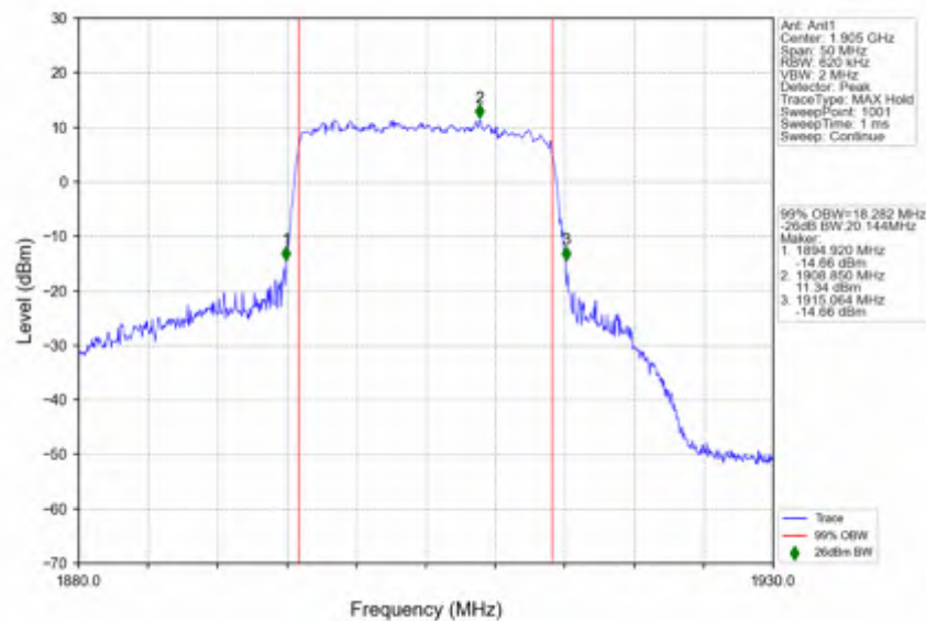
n25_30kHz_SISO_NTNV_20MHz_CP-OFDM QPSK_1905MHz_Outer_Full
