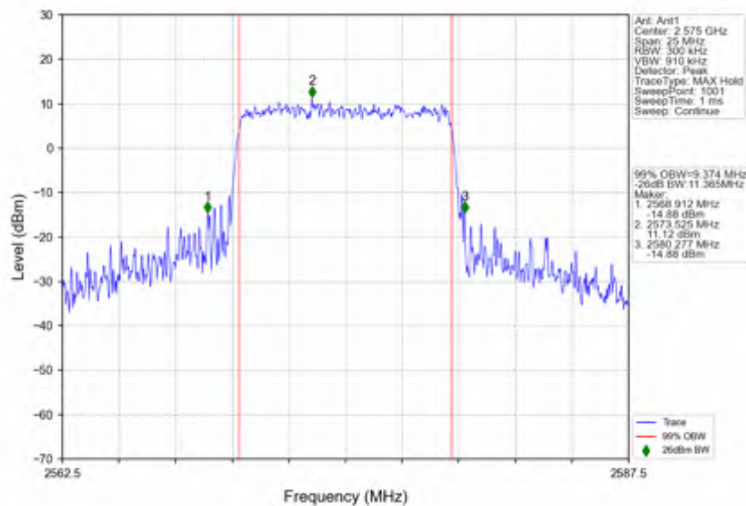
n38 15kHz SISO NTN 10MHz CP-OFDM 64 QAM 2575MHz Outer Full
