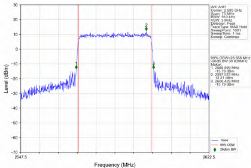
n38_15kHz_SISO_NTNV_30MHz_CP-OFDM_QPSK_2585MHz_Outer_Full
