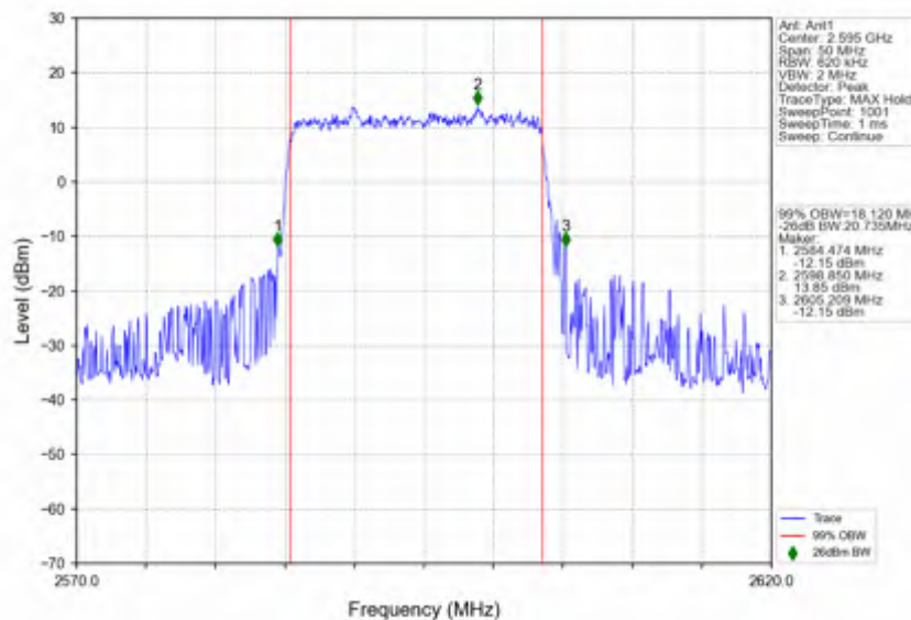
n38_15kHz_SISO_NTNV_20MHz_DFT-s-OFDM_PI/2_BPSK_2595MHz_Outer_Full
