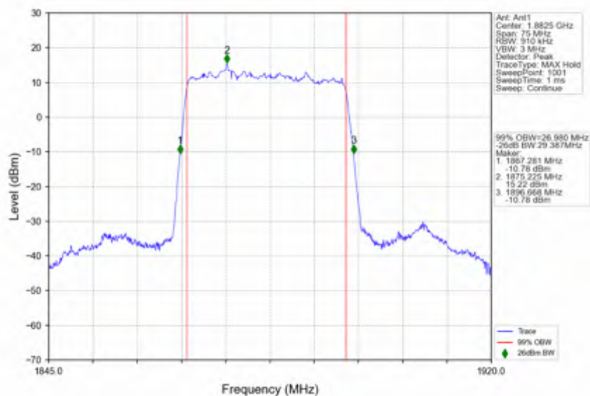
n25_30kHz_SISO_NTNV_30MHz_DFT-s-OFDM_PI/2_BPSK_1882.5MHz_Outer_Full
