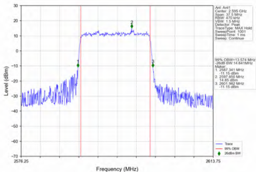
n38_15kHz_SISO_NTNV_15MHz_DFT-s-OFDM PI/2 BPSK_2595MHz_Outer_Full
