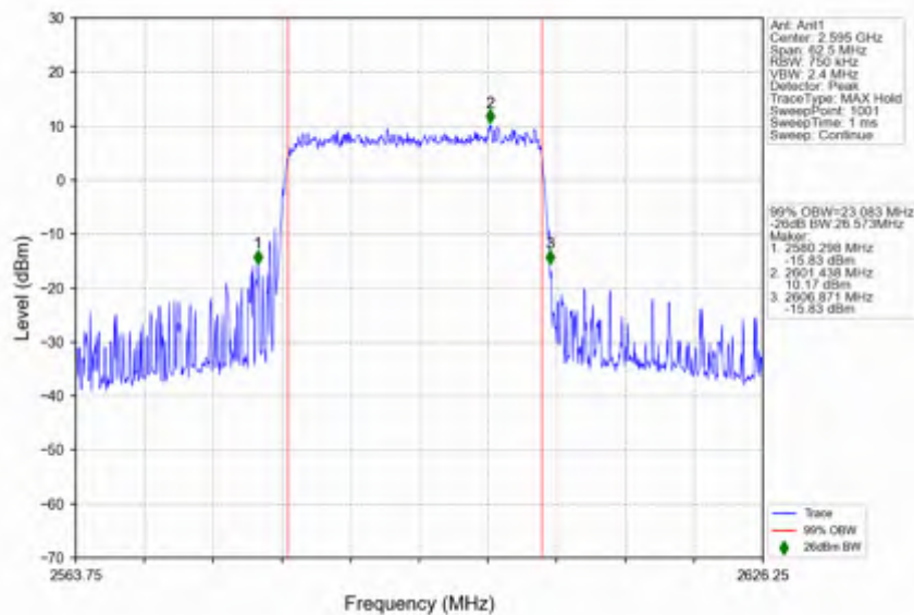
n38_15kHz_SISO_NTNV_25MHz_DFT-s-OFDM_256_QAM_2595MHz_Outer_Full
