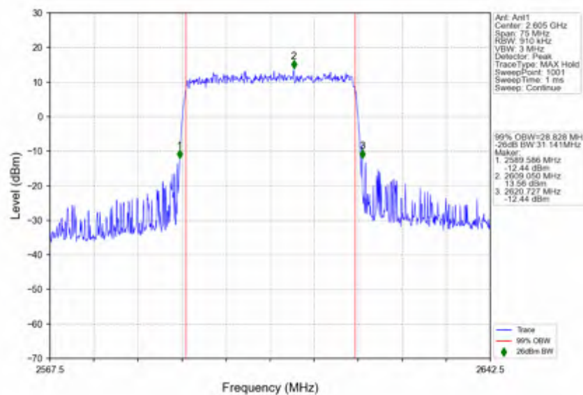
n38 15kHz SISO NTNV 30MHz DFT-s-OFDM QPSK 2605MHz Outer Full
