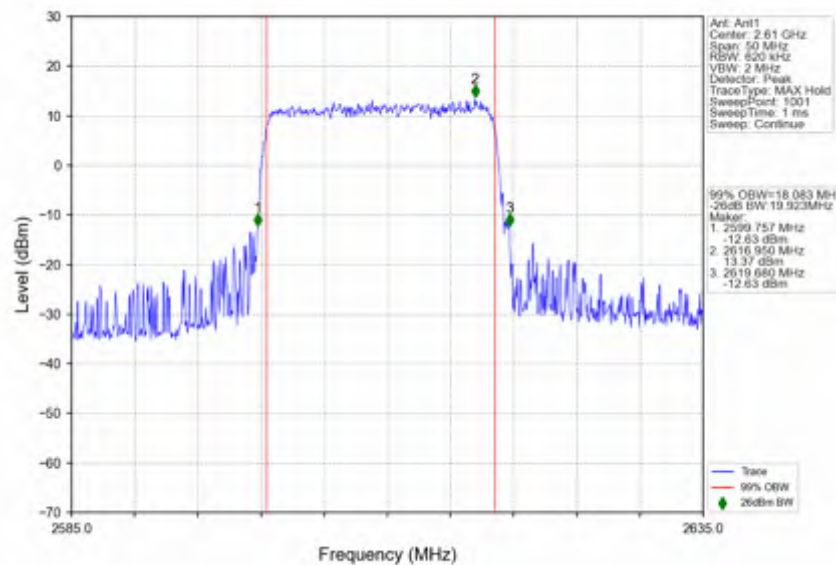
n38_15kHz_SISO_NTNV_20MHz_DFT-s-OFDM QPSK_2610MHz_Outer_Full
