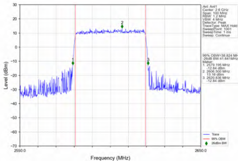
n38_15kHz_SISO_NTNV_40MHz_DFT-s-OFDM QPSK_2600MHz_Outer_Full
