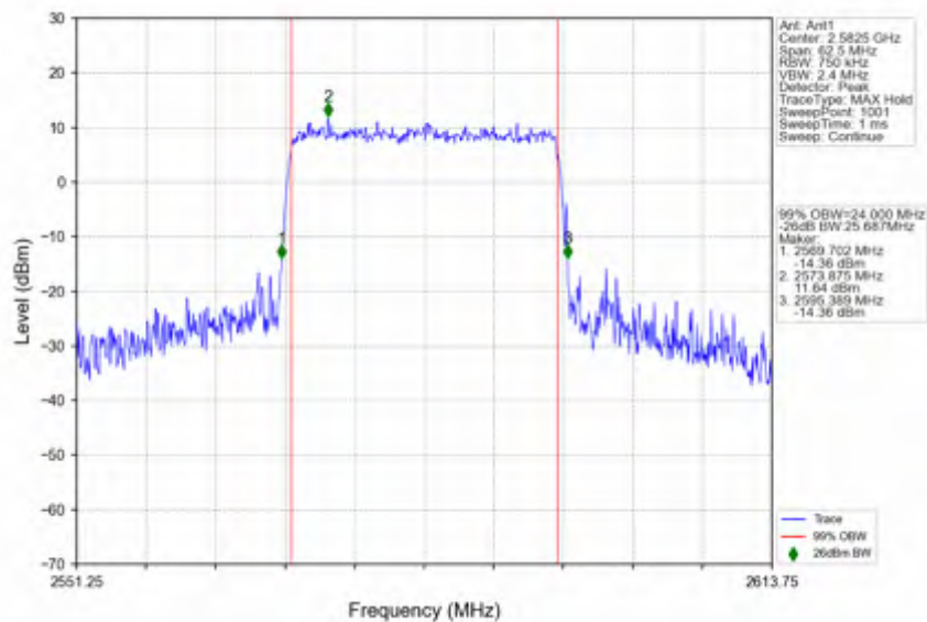
n38_15kHz_SISO_NTNV_25MHz_CP-OFDM 64 QAM_2582.5MHz_Outer_Full
