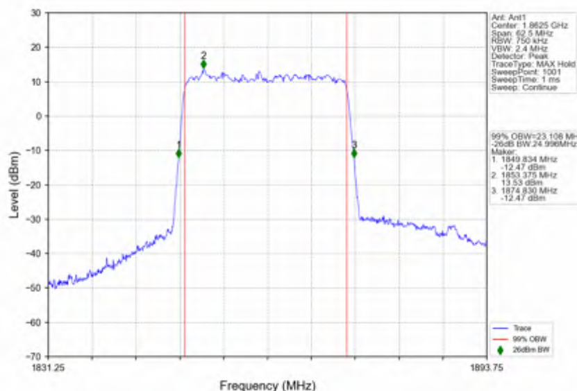
n25_30kHz_SISO_NTNV_25MHz_DFT-s-OFDM QPSK_1862.5MHz_Outer_Full
