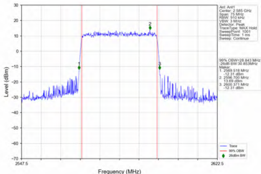
n38_15kHz_SISO_NTNV_30MHz_DFT-s-OFDM QPSK_2585MHz_Outer_Full
