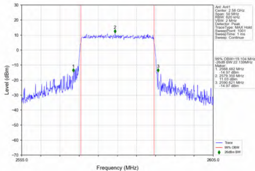
n38_15kHz_SISO_NTNV_20MHz_CP-OFDM 64 QAM_2580MHz_Outer_Full
