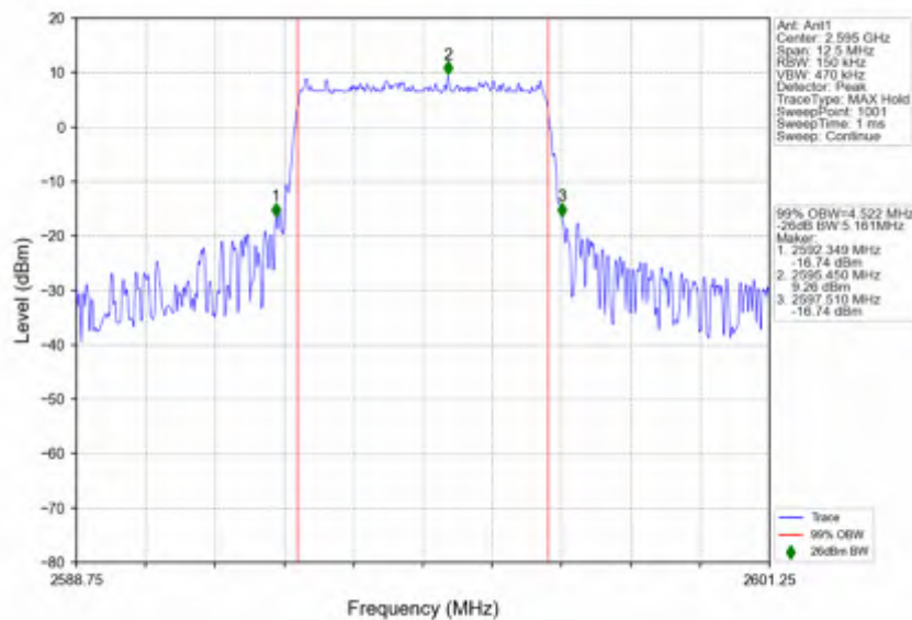
n38_15kHz_SISO_NTNV_5MHz_DFT-s-OFDM_256_QAM_2595MHz_Outer_Full
