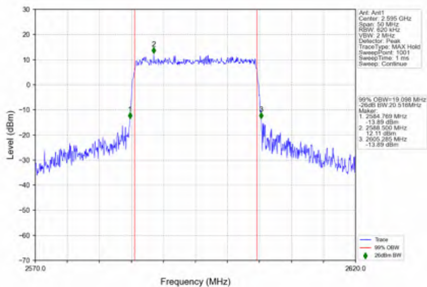
n38 15kHz SISO NTNV 20MHz CP-OFDM 16 QAM 2595MHz Outer Full
