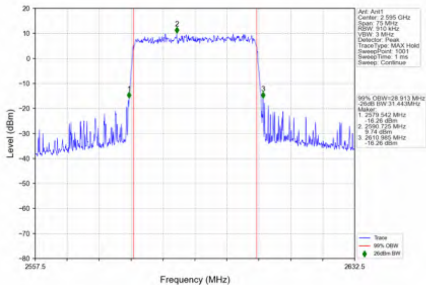
n38_15kHz_SISO_NTNV_30MHz_DFT-s-OFDM 256 QAM 2595MHz_Outer_Full
