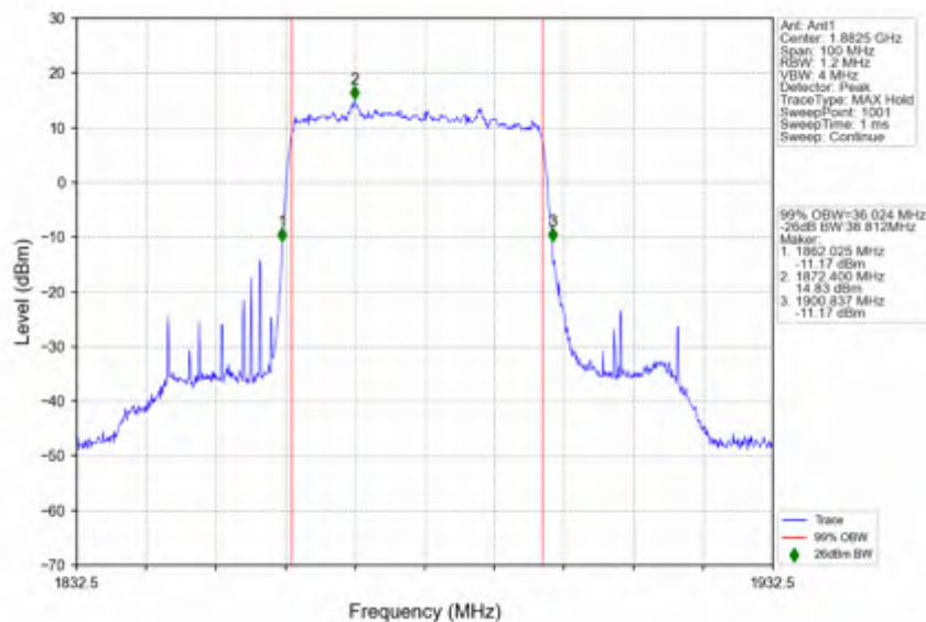
n25_30kHz_SISO_NTNV_40MHz_DFT-s-OFDM_PI/2_BPSK_1882.5MHz_Outer_Full
