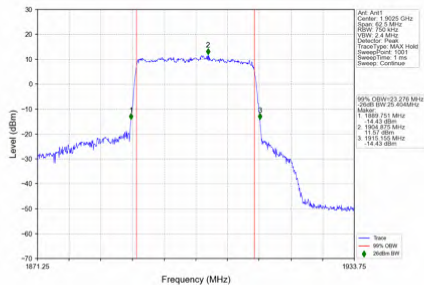
n25 30kHz SISO NTNV 25MHz CP-OFDM QPSK 1902.5MHz Outer Full
