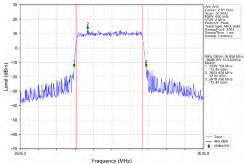
n38_15kHz_SISO_NTNV_20MHz_DFT-s-OFDM_64_QAM_2610MHz_Outer_Full
