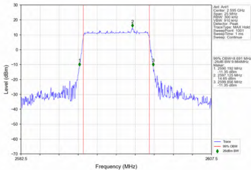
n38_30kHz_SISO_NTNV_10MHz_DFT-s-OFDM_PI/2_BPSK_2595MHz_Outer_Full
