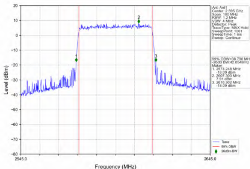
n38_15kHz_SISO_NTNV_40MHz_CP-OFDM 256 QAM_2595MHz_Outer_Full
