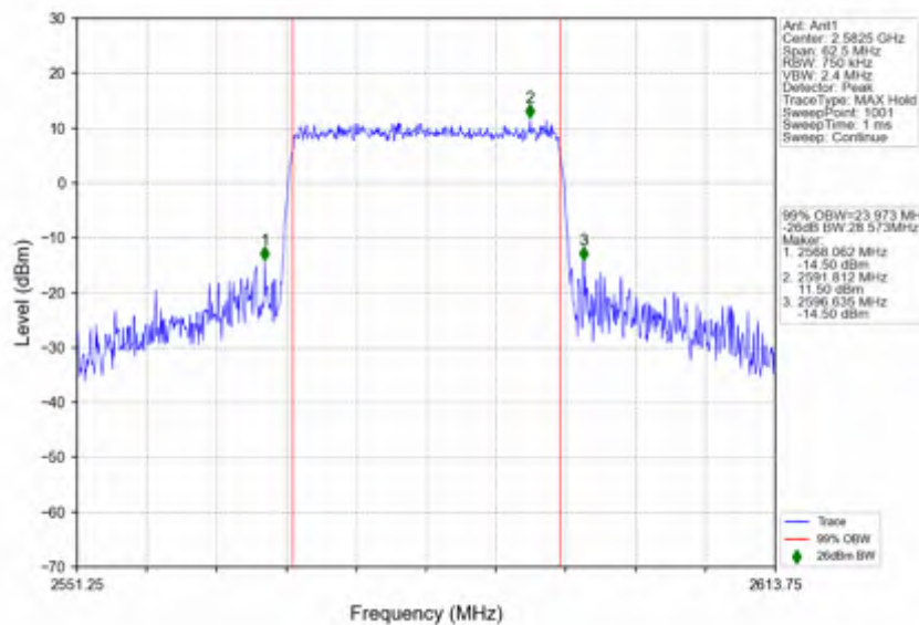
n38_15kHz_SISO_NTNV_25MHz_CP-OFDM_QPSK_2582.5MHz_Outer_Full
