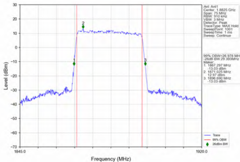
n25_30kHz_SISO_NTNV_30MHz_DFT-s-OFDM_16QAM_1882.5MHz_Outer_Full
