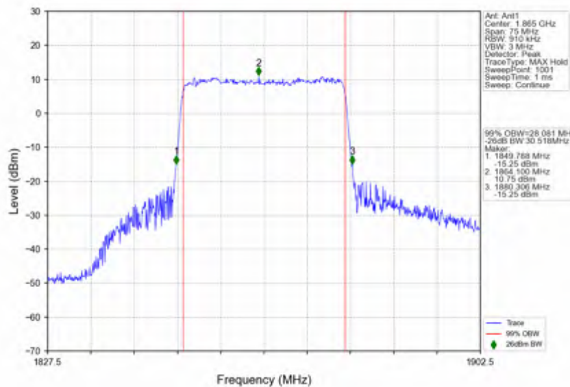
n25_30kHz_SISO_NTNV_30MHz_CP-OFDM 64 QAM_1865MHz_Outer_Full
