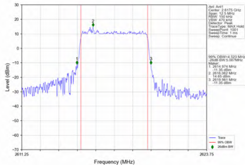
n38_15kHz_SISO_NTNV_5MHz_DFT-s-OFDM QPSK_2617.5MHz_Outer_Full
