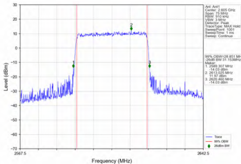
n38_15kHz_SISO_NTNV_30MHz_DFT-s-OFDM_64_QAM_2605MHz_Outer_Full
