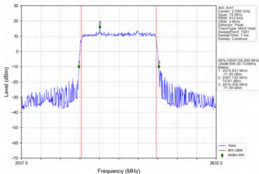
n38_15kHz_SISO_NTNV_30MHz_DFT-s-OFDM_PI/2_BPSK_2595MHz_Outer_Full
