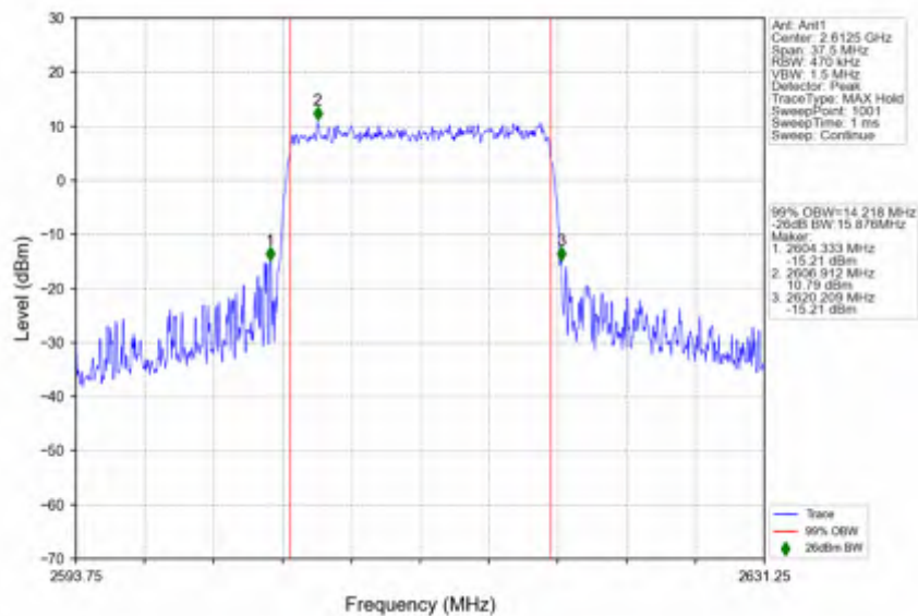
n38_15kHz_SISO_NTNV_15MHz_CP-OFDM_64_QAM_2612.5MHz_Outer_Full
