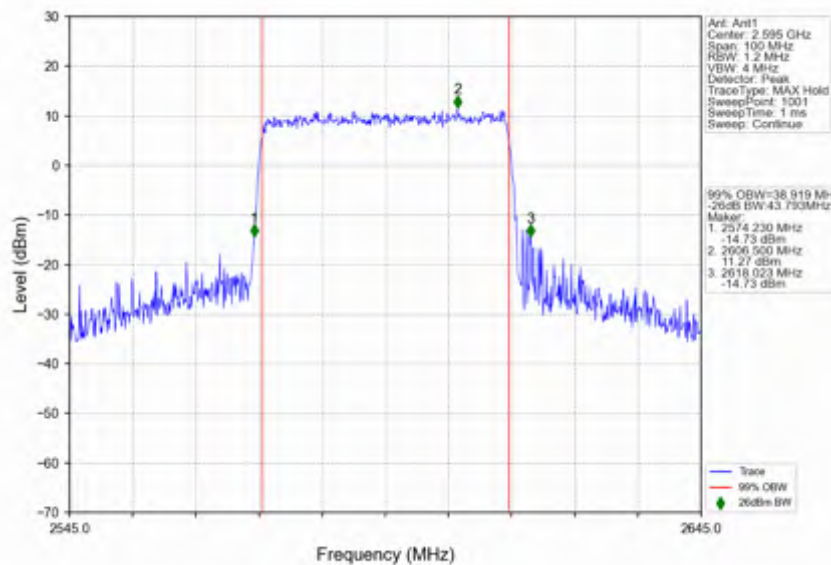
n38_15kHz_SISO_NTNV_40MHz_CP-OFDM_16_QAM_2595MHz_Outer_Full
