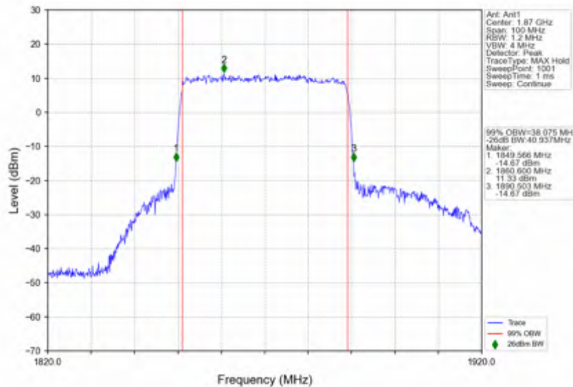
n25_30kHz_SISO_NTNV_40MHz_CP-OFDM QPSK_1870MHz_Outer_Full
