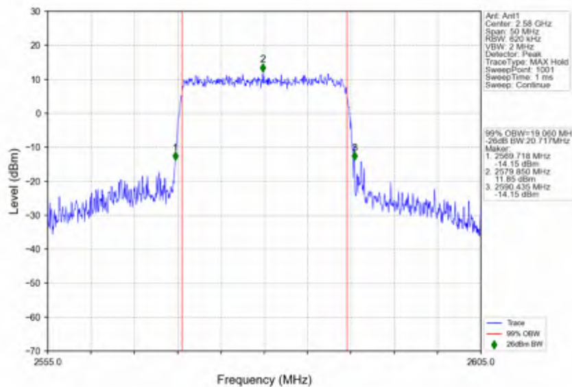
n38_15kHz_SISO_NTNV_20MHz_CP-OFDM QPSK_2580MHz_Outer_Full
