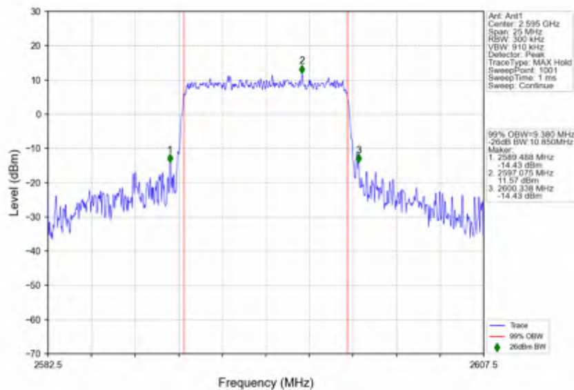
n38 15kHz SISO NTN 10MHz CP-OFDM 16 QAM 2595MHz Outer Full
