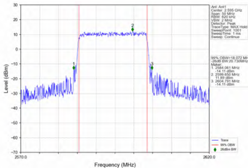
n38_15kHz_SISO_NTNV_20MHz_DFT-s-OFDM_16_QAM_2595MHz_Outer_Full
