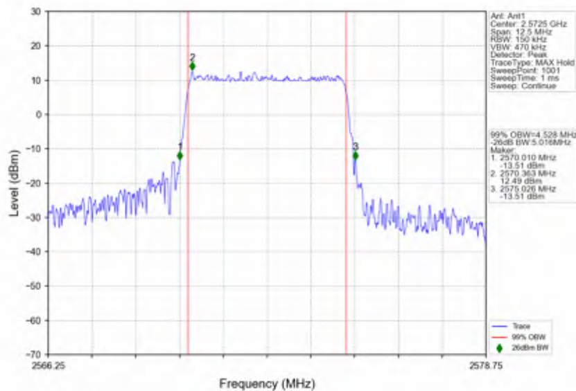
n38_15kHz_SISO_NTNV_5MHz_DFT-s-OFDM QPSK_2572.5MHz_Outer_Full
