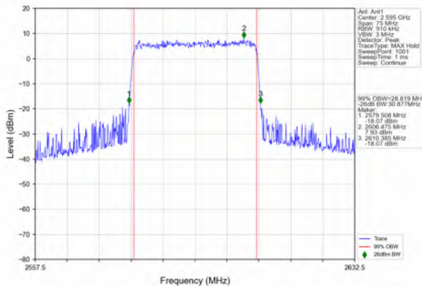
n38 15kHz SISO NTNV 30MHz CP-OFDM 256 QAM 2595MHz Outer Full
