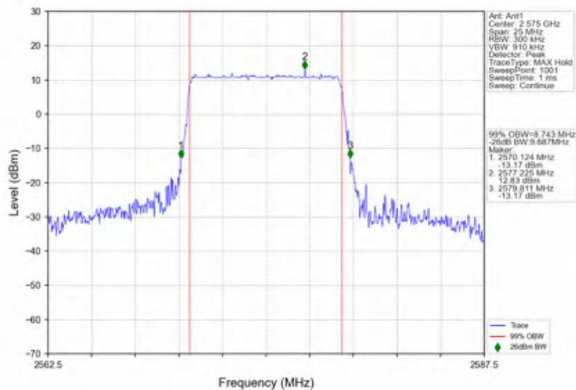
n38_30kHz_SISO_NTNV_10MHz_DFT-s-OFDM QPSK_2575MHz_Outer_Full
