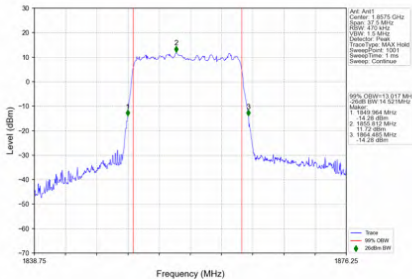
n25_30kHz_SISO_NTV_15MHz_DFT-s-OFDM 64 QAM_1857.5MHz_Outer_Full
