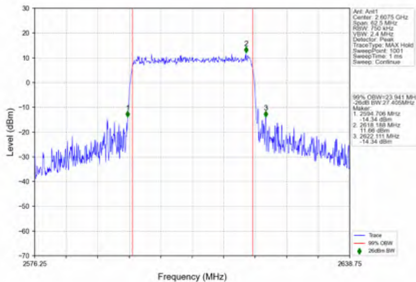
n38_15kHz_SISO_NTNV_25MHz_CP-OFDM QPSK_2607.5MHz_Outer_Full
