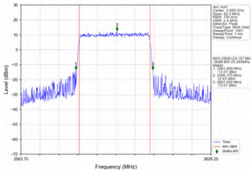
n38 15kHz SISO NTV 25MHz DFT-s-OFDM 16 QAM 2595MHz Outer Full
