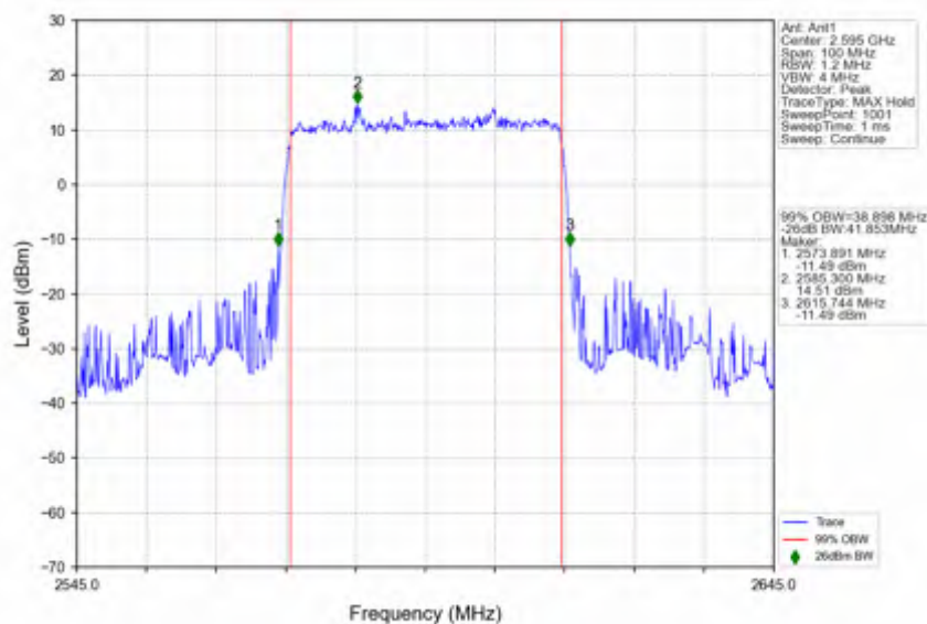
n38_15kHz_SISO_NTNV_40MHz_DFT-s-OFDM_PI/2_BPSK_2595MHz_Outer_Full
