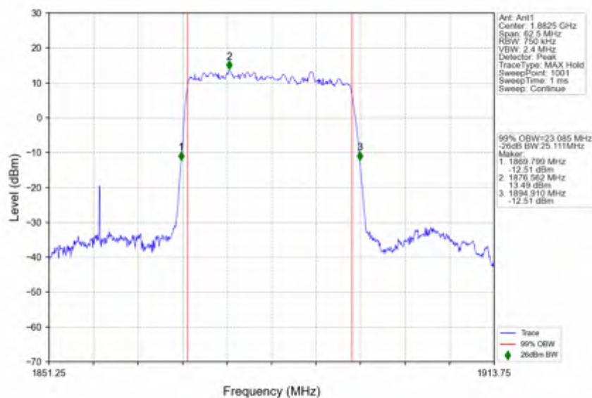
n25_30kHz_SISO_NTNV_25MHz_DFT-s-OFDM PI/2 BPSK_1882.5MHz_Outer_Full
