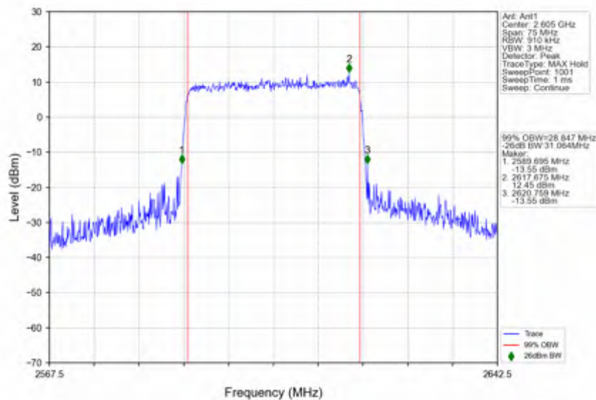
n38_15kHz_SISO_NTNV_30MHz_CP-OFDM QPSK_2605MHz_Outer_Full
