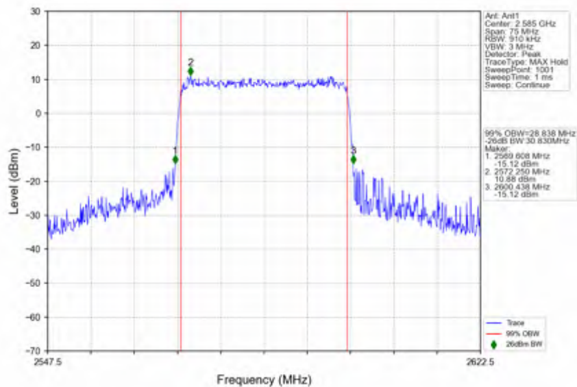
n38_15kHz_SISO_NTNV_30MHz_CP-OFDM_64_QAM_2585MHz_Outer_Full
