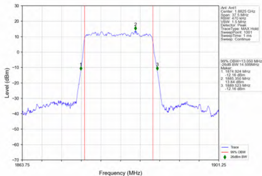
n25_30kHz_SISO_NTNV_15MHz_DFT-s-OFDM PI/2 BPSK_1882.5MHz_Outer_Full
