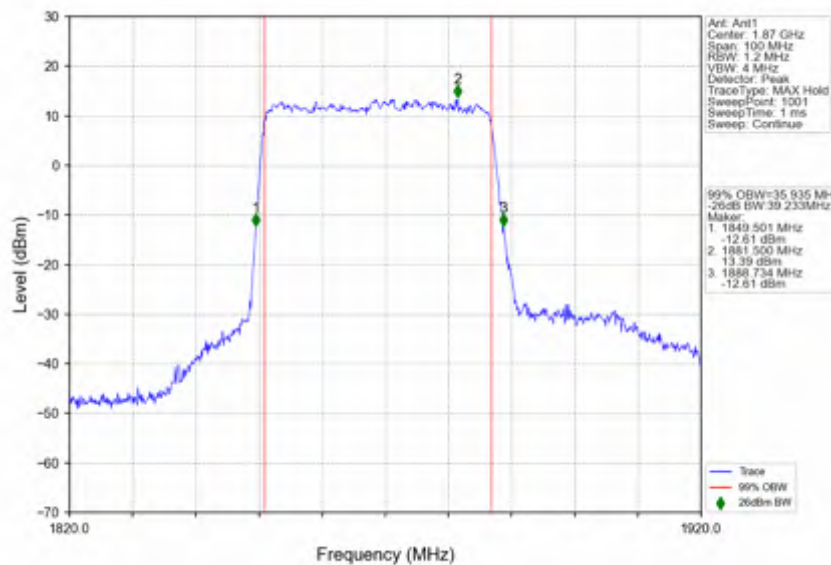
n25_30kHz_SISO_NTNV_40MHz_DFT-s-OFDM QPSK_1870MHz_Outer_Full
