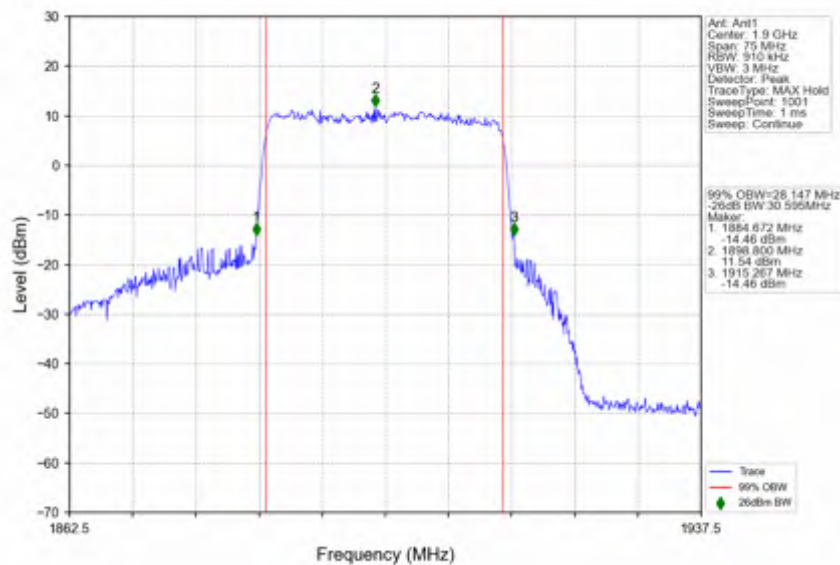
n25_30kHz_SISO_NTNV_30MHz_CP-OFDM QPSK_1900MHz_Outer_Full
