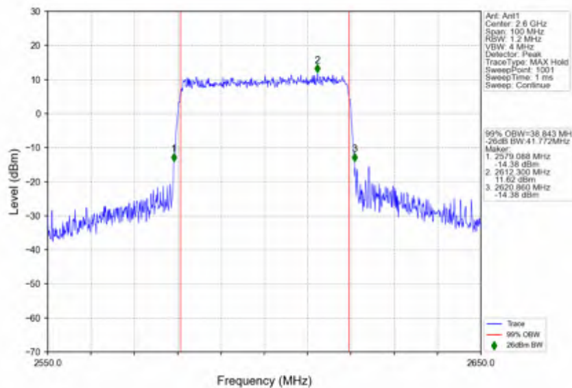
n38_15kHz_SISO_NTV_40MHz_CP-OFDM_QPSK_2600MHz_Outer_Full
