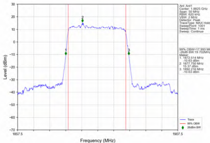
n25_30kHz_SISO_NTNV_20MHz_DFT-s-OFDM_PI/2_BPSK_1882.5MHz_Outer_Full
