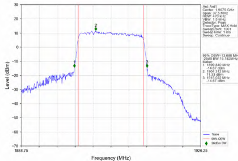
n25_30kHz_SISO_NTNV_15MHz_CP-OFDM_QPSK_1907.5MHz_Outer_Full
