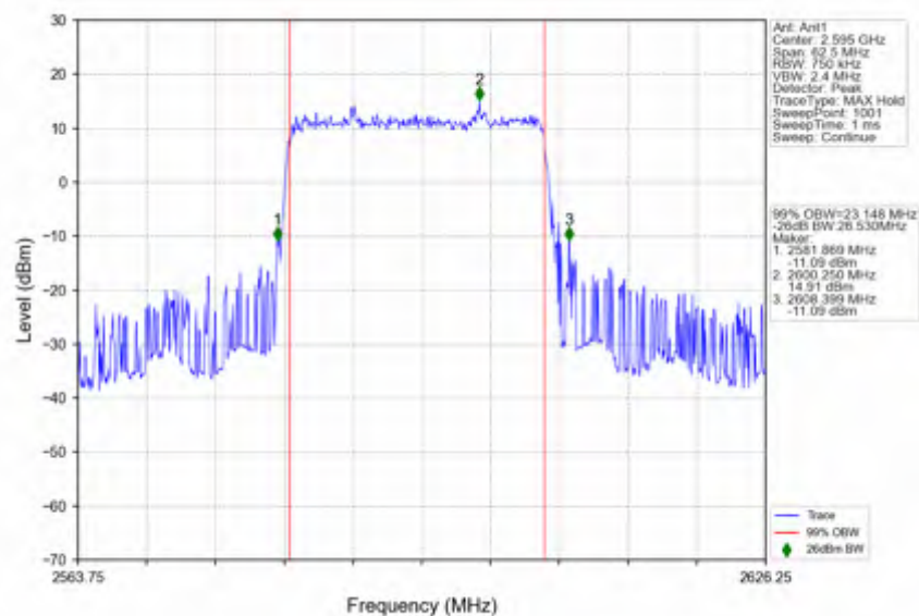
n38_15kHz_SISO_NTNV_25MHz_DFT-s-OFDM PI/2 BPSK_2595MHz_Outer_Full
