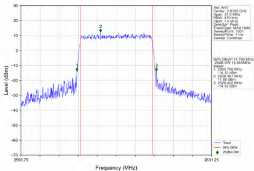
n38 15kHz SISO NTNV 15MHz CP-OFDM QPSK 2612.5MHz Outer Full
