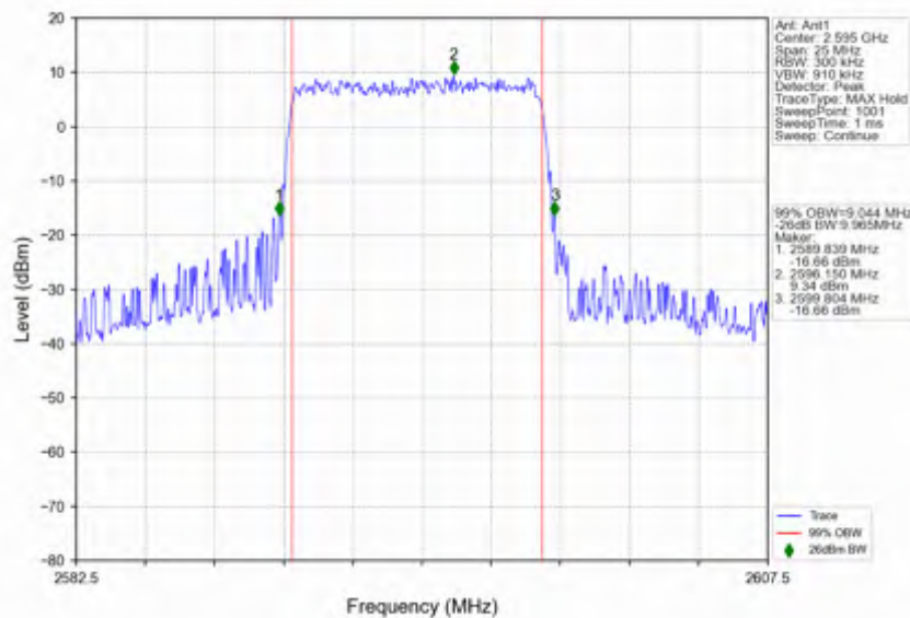
n38_15kHz_SISO_NTNV_10MHz_DFT-s-OFDM_256_QAM_2595MHz_Outer_Full
