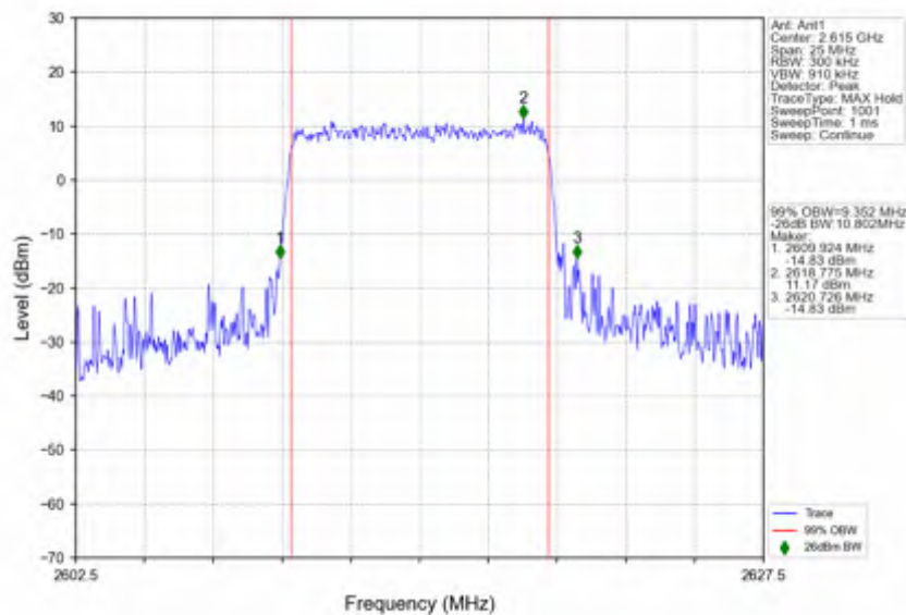
n38_15kHz_SISO_NTV_10MHz_CP-OFDM_QPSK_2615MHz_Outer_Full
