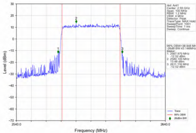
n38_15kHz_SISO_NTNV_40MHz_DFT-s-OFDM QPSK_2590MHz_Outer_Full
