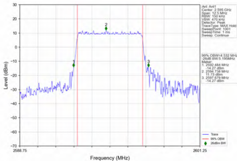
n38_15kHz_SISO_NTNV_5MHz_DFT-s-OFDM_16_QAM_2595MHz_Outer_Full
