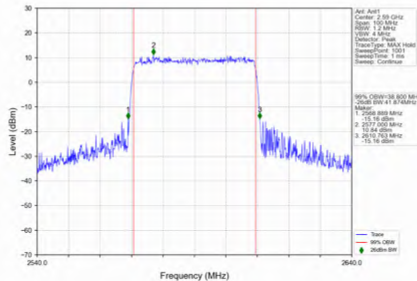
n38_15kHz_SISO_NTNV_40MHz_CP-OFDM 64 QAM_2590MHz_Outer_Full
