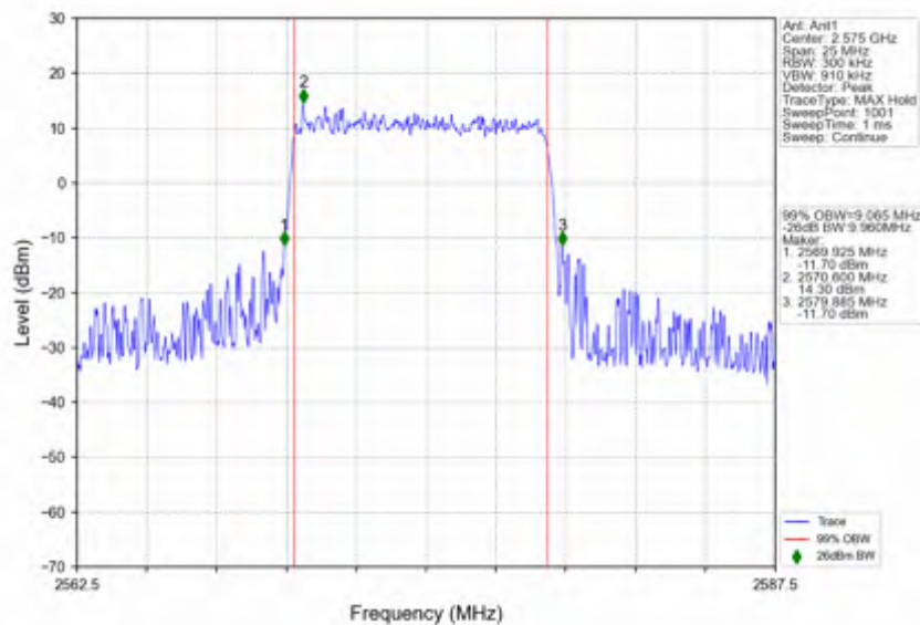
n38_15kHz_SISO_NTNV_10MHz_DFT-s-OFDM QPSK_2575MHz_Outer_Full
