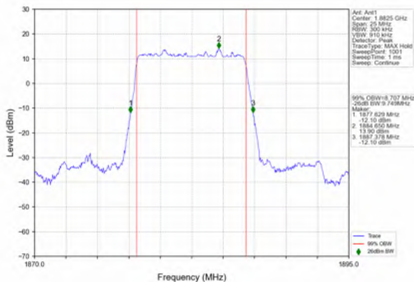
n25_30kHz_SISO_NTNV_10MHz_DFT-s-OFDM_PI/2_BPSK_1882.5MHz_Outer_Full
