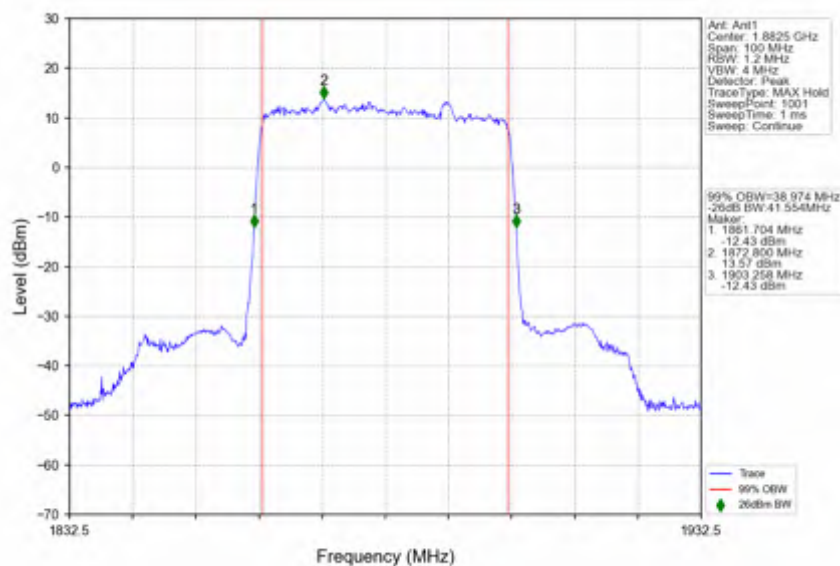
n25_15kHz_SISO_NTNV_40MHz_DFT-s-OFDM_PI/2_BPSK_1882.5MHz_Outer_Full
