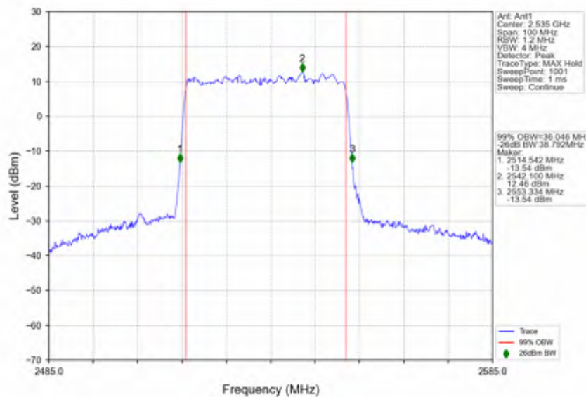
n7_30kHz_SISO_NTNV_40MHz_DFT-s-OFDM_16_QAM_2535MHz_Outer_Full
