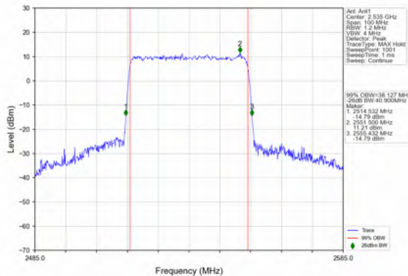
n7_30kHz_SISO_NTNV_40MHz_CP-OFDM_16_QAM_2535MHz_Outer_Full
