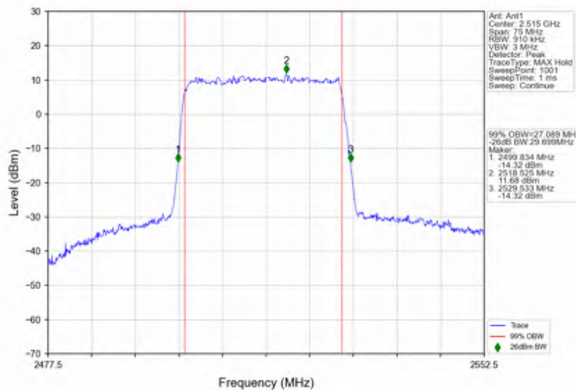
n7_30kHz_SISO_NTNV_30MHz_DFT-s-OFDM 64 QAM_2515MHz_Outer_Full
