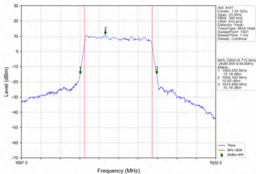
n25_30kHz_SISO_NTNV_10MHz_CP-OFDM 64 QAM_1910MHz_Outer_Full
