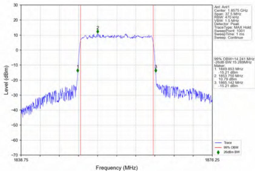
n25_15kHz_SISO_NTNV_15MHz_CP-OFDM 64 QAM_1857.5MHz_Outer_Full
