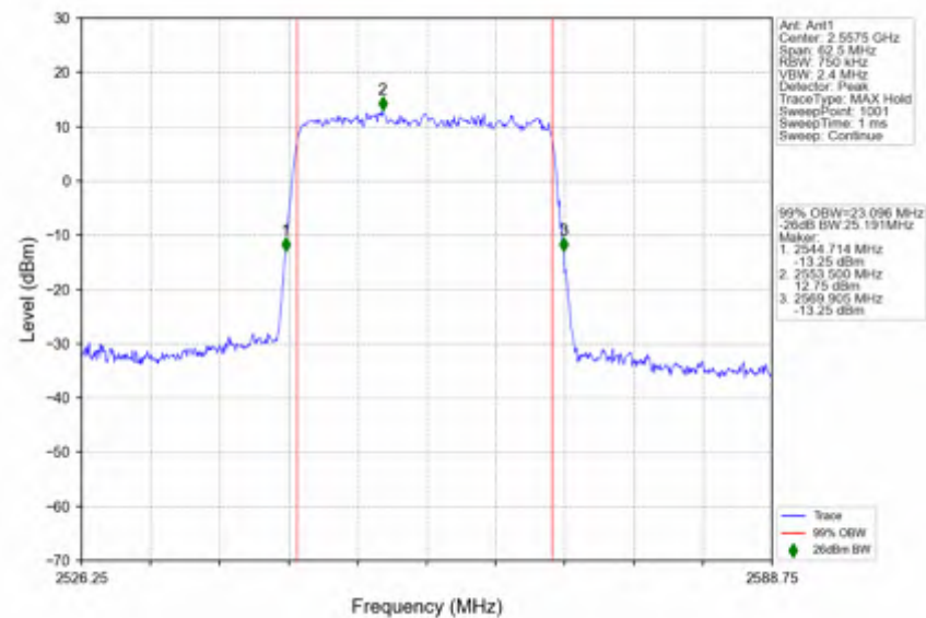
n7_30kHz_SISO_NTNV_25MHz_DFT-s-OFDM_QPSK_2557.5MHz_Outer_Full
