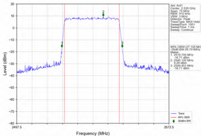
n7_30kHz_SISO_NTNV_30MHz_DFT-s-OFDM_256_QAM_2535MHz_Outer_Full
