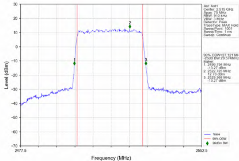
n7_30kHz_SISO_NTNV_30MHz_DFT-s-OFDM QPSK_2515MHz_Outer_Full
