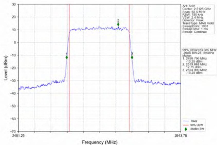
n7_30kHz_SISO_NTNV_25MHz_DFT-s-OFDM QPSK_2512.5MHz_Outer_Full
