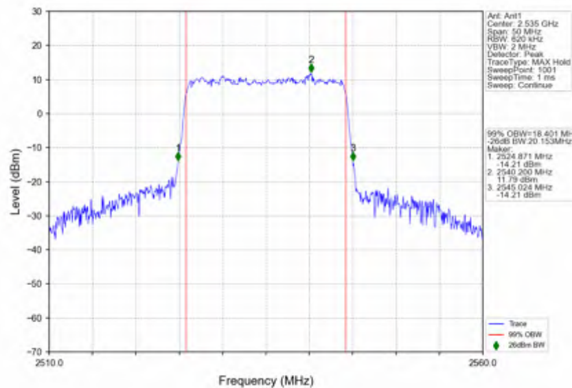
n7_30kHz_SISO_NTNV_20MHz_CP-OFDM 16 QAM_2535MHz_Outer_Full
