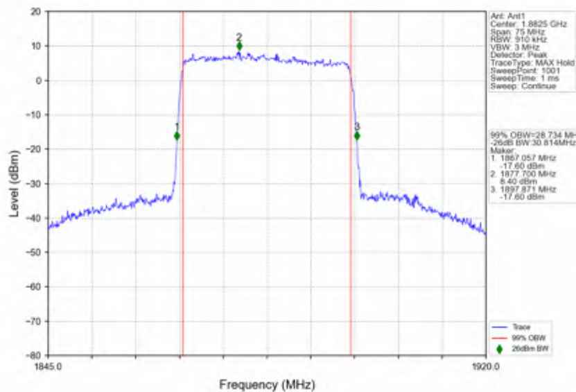
n25_15kHz_SISO_NTNV_30MHz_CP-OFDM 256 QAM_1882.5MHz_Outer_Full
