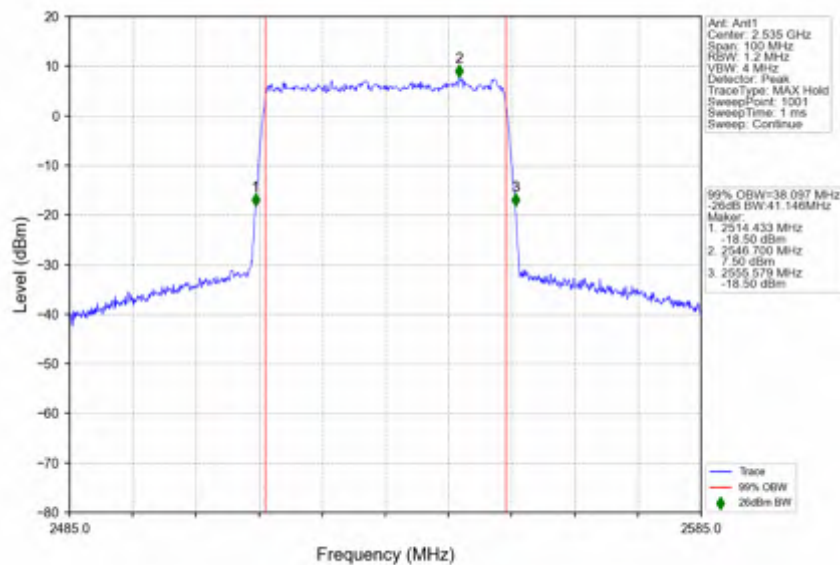
n7_30kHz_SISO_NTNV_40MHz_CP-OFDM_256_QAM_2535MHz_Outer_Full
