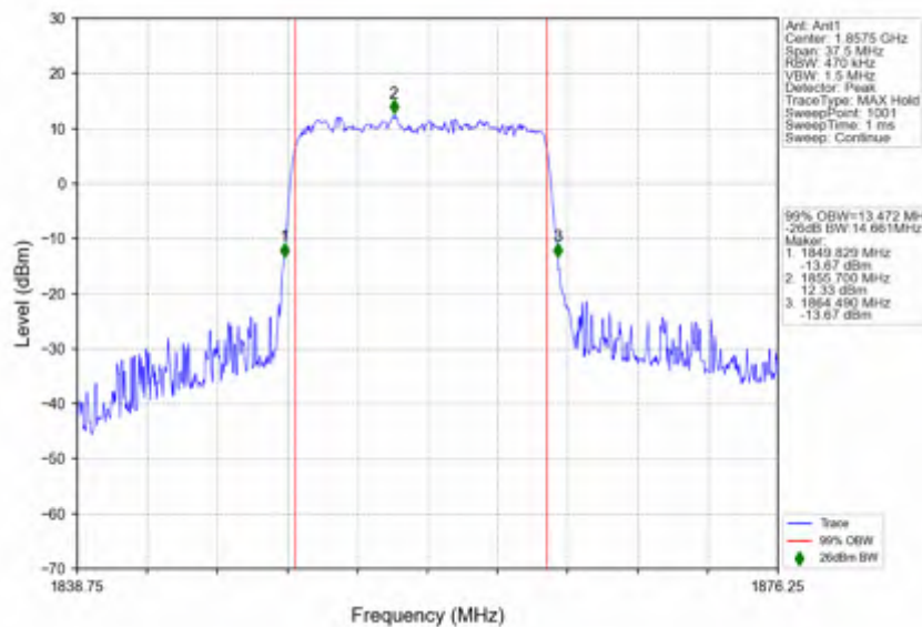
n25_15kHz_SISO_NTV_15MHz_DFT-s-OFDM 64 QAM_1857.5MHz_Outer_Full
