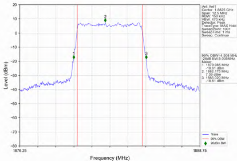
n25_15kHz_SISO_NTNV_5MHz_CP-OFDM 256 QAM_1882.5MHz_Outer_Full
