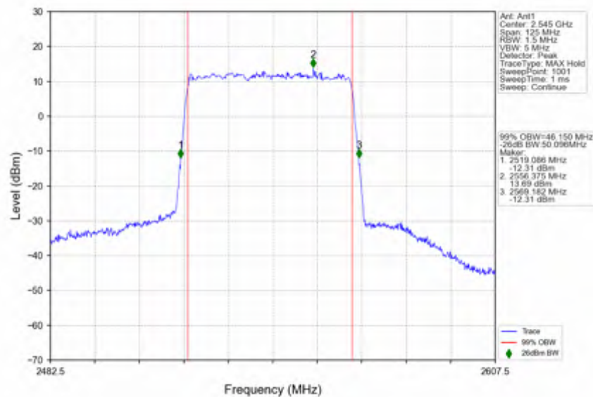
n7_30kHz_SISO_NTNV_50MHz_DFT-s-OFDM_QPSK_2545MHz_Outer_Full
