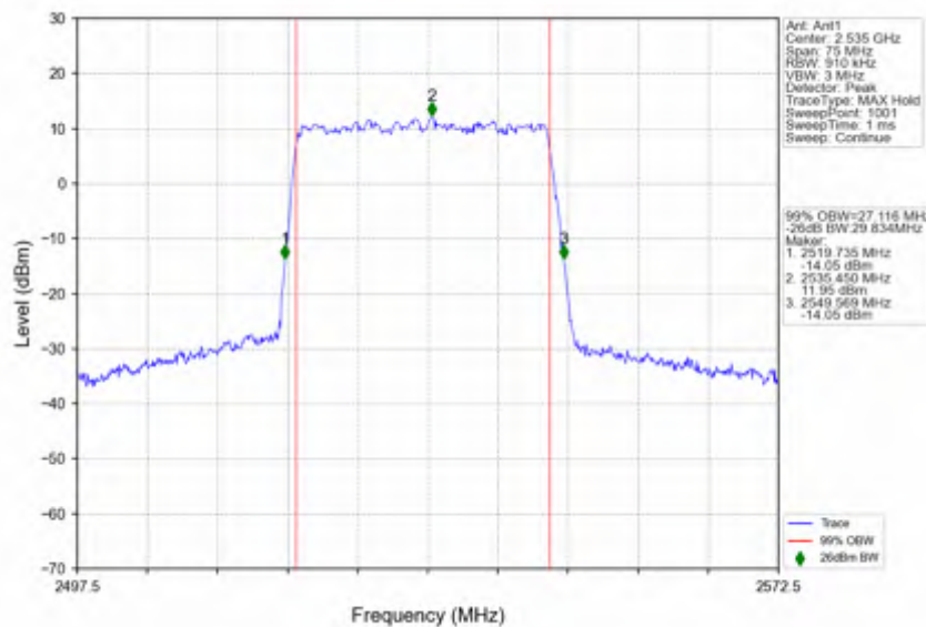
n7_30kHz_SISO_NTNV_30MHz_DFT-s-OFDM_16_QAM_2535MHz_Outer_Full
