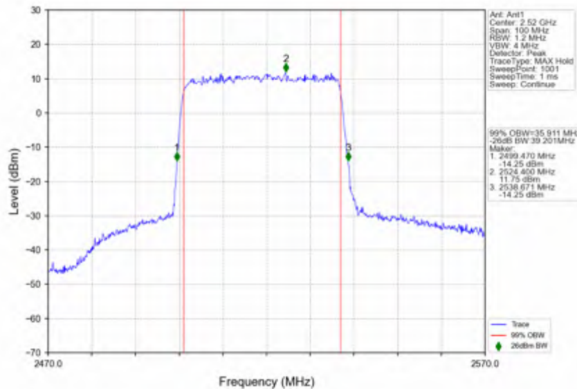
n7_30kHz_SISO_NTNV_40MHz_DFT-s-OFDM_64 QAM_2520MHz_Outer_Full
