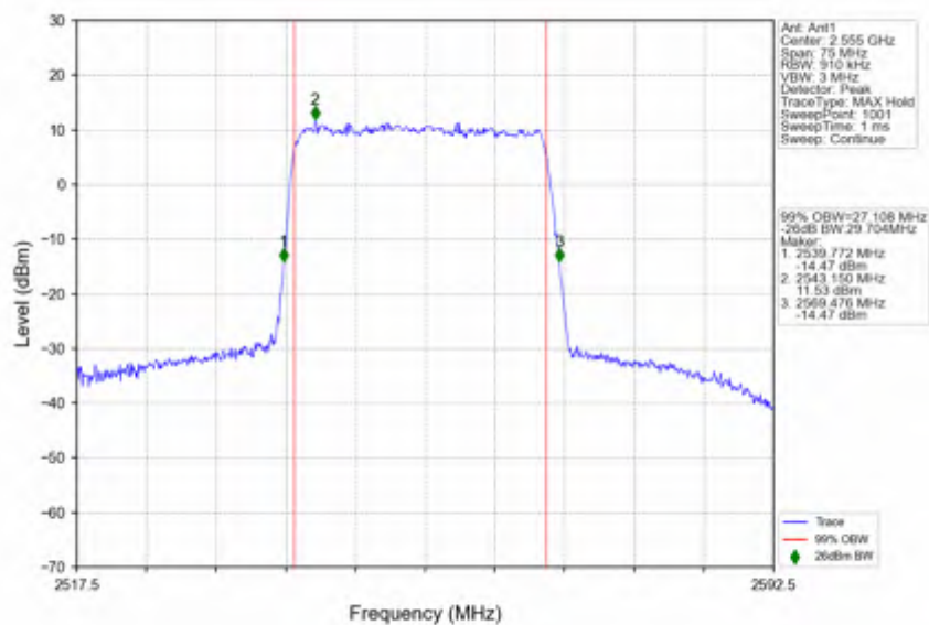
n7 30kHz SISO NTNV 30MHz DFT-s-OFDM 64 QAM 2555MHz Outer Full
