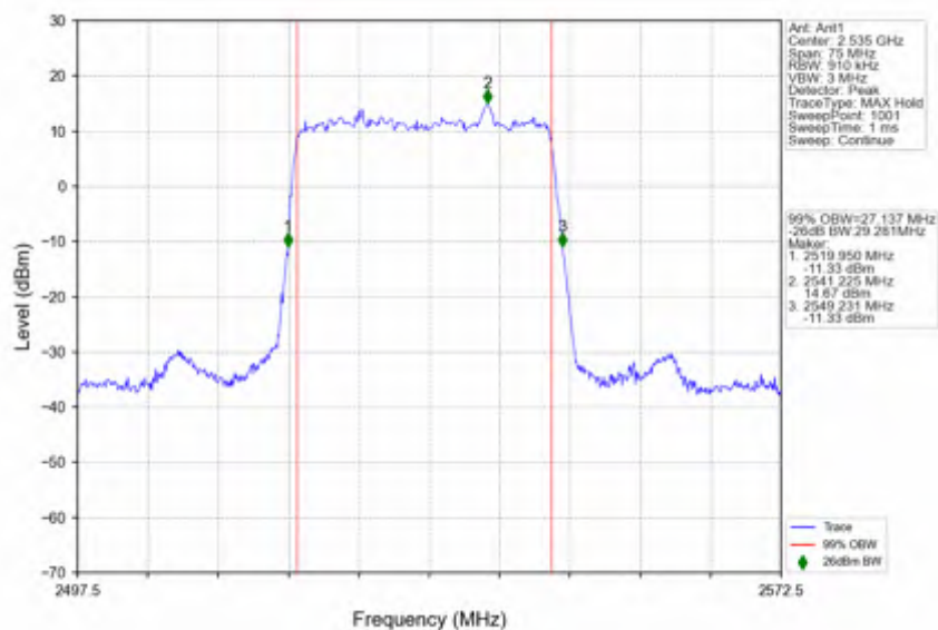
n7_30kHz_SISO_NTNV_30MHz_DFT-s-OFDM_PI/2_BPSK_2535MHz_Outer_Full
