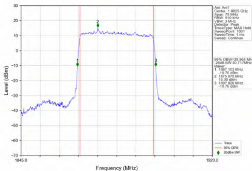
n25_15kHz_SISO_NTNV_30MHz_DFT-s-OFDM_PI/2_BPSK_1882.5MHz_Outer_Full
