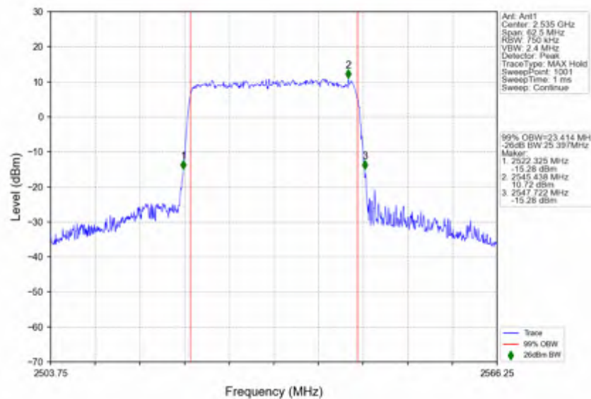
n7 30kHz SISO NTN 25MHz CP-OFDM 16 QAM 2535MHz Outer Full
