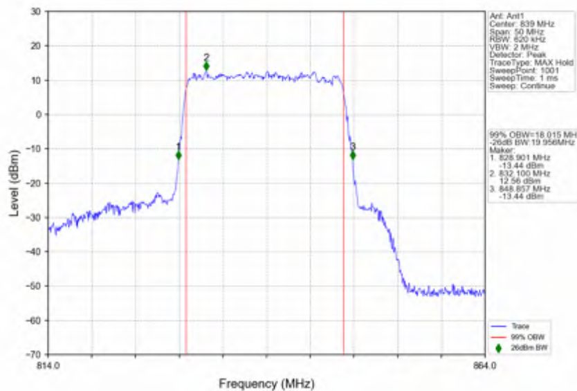
n5_30kHz_SISO_NTNV_20MHz_DFT-s-OFDM 64 QAM_839MHz_Outer_Full
