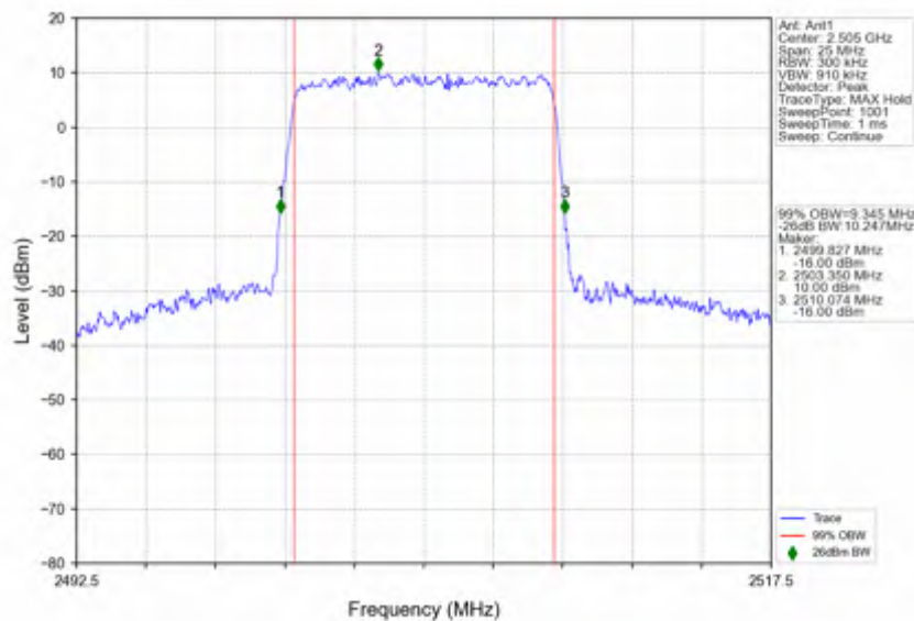
n7 15kHz SISO NTV 10MHz CP-OFDM QPSK 2505MHz Outer Full
