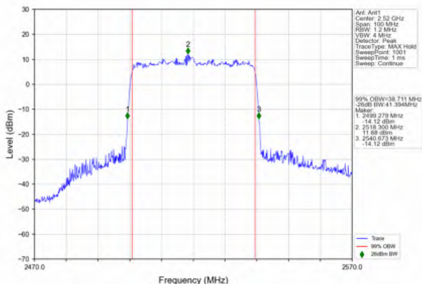
n7 15kHz SISO NTN 40MHz CP-OFDM 64 QAM 2520MHz Outer Full
