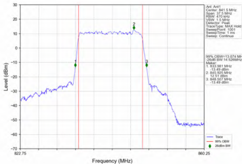
n5_30kHz_SISO_NTNV_15MHz_DFT-s-OFDM_64_QAM_841.5MHz_Outer_Full
