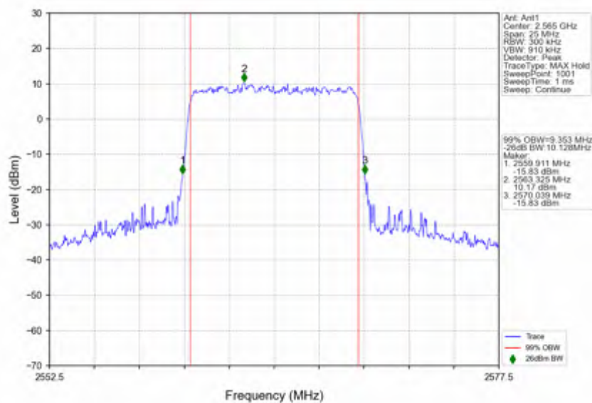
n7 15kHz SISO NTN 10MHz CP-OFDM QPSK 2565MHz Outer Full
