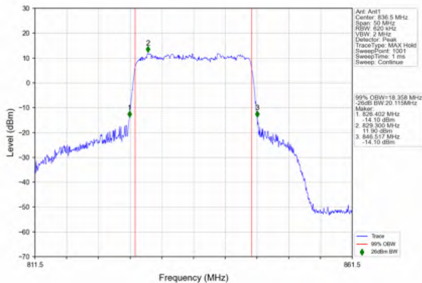
n5_30kHz_SISO_NTNV_20MHz_CP-OFDM_16_QAM_836.5MHz_Outer_Full
