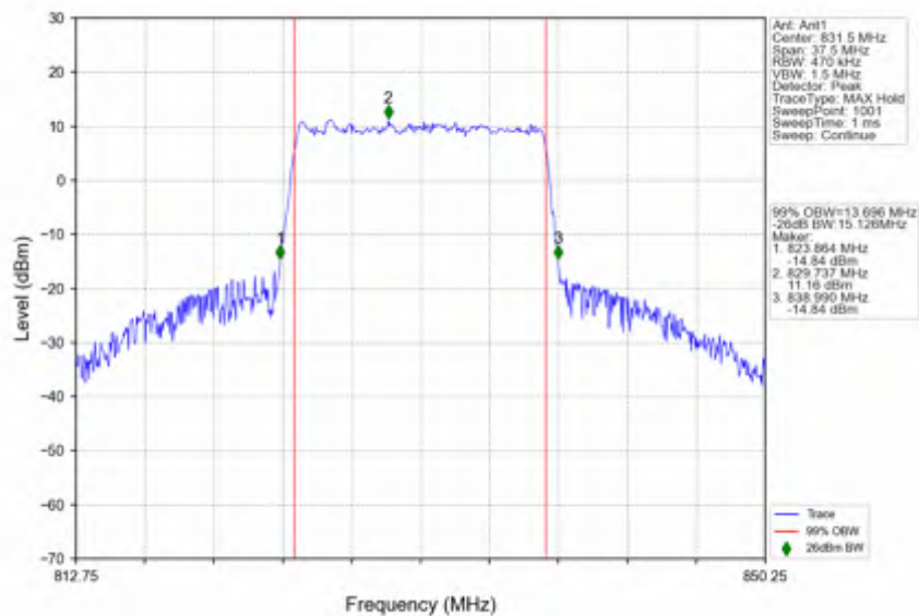
n5_30kHz_SISO_NTNV_15MHz_CP-OFDM 64 QAM 831.5MHz_Outer_Full
