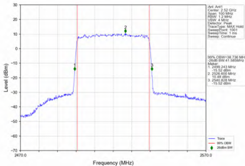
n7_15kHz_SISO_NTNV_40MHz_DFT-s-OFDM_64 QAM_2520MHz_Outer_Full
