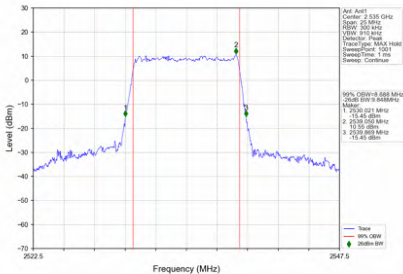
n7_30kHz_SISO_NTNV_10MHz_CP-OFDM_16_QAM_2535MHz_Outer_Full
