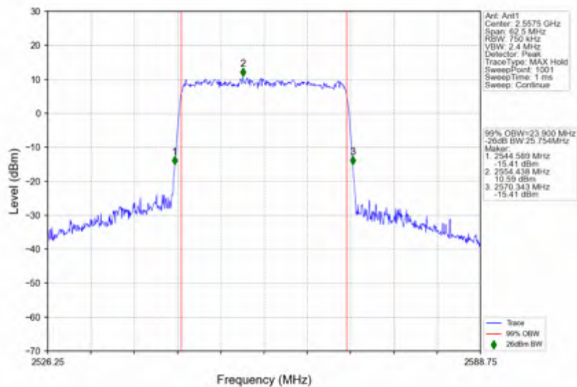
n7_15kHz_SISO_NTNV_25MHz_CP-OFDM QPSK_2557.5MHz_Outer_Full
