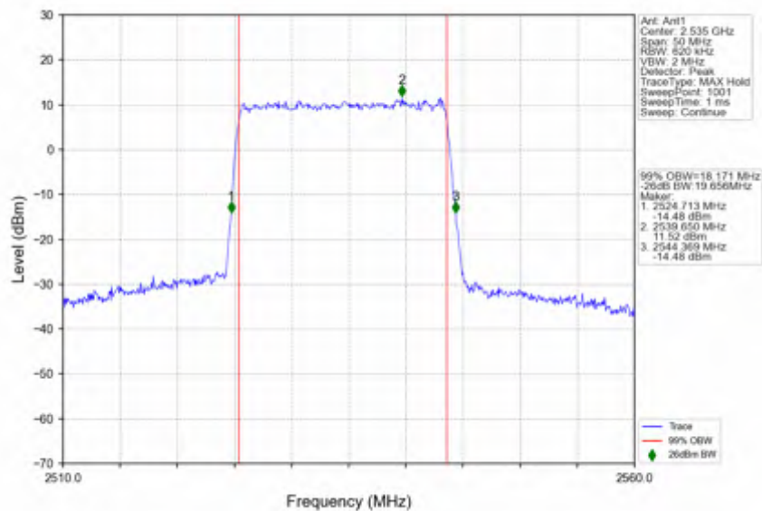
n7_15kHz_SISO_NTNV_20MHz_DFT-s-OFDM_16_QAM_2535MHz_Outer_Full
