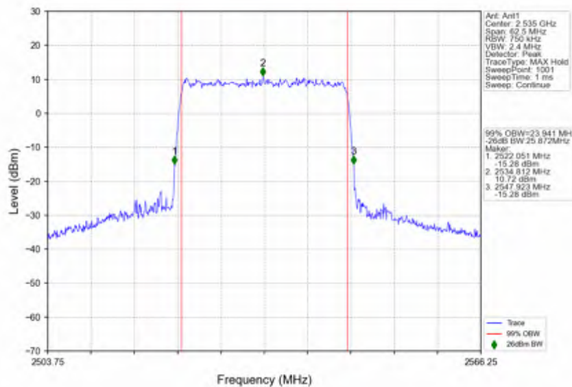
n7_15kHz_SISO_NTNV_25MHz_CP-OFDM_16_QAM_2535MHz_Outer_Full
