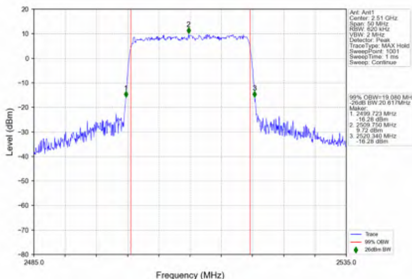
n7_15kHz_SISO_NTNV_20MHz_CP-OFDM 64 QAM_2510MHz_Outer_Full
