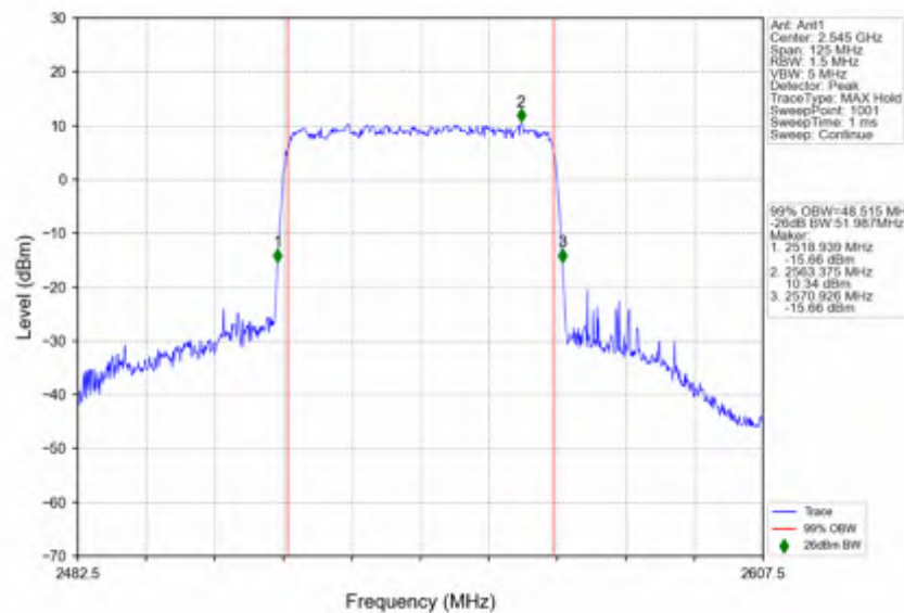
n7_15kHz_SISO_NTNV_50MHz_CP-OFDM_QPSK_2545MHz_Outer_Full
