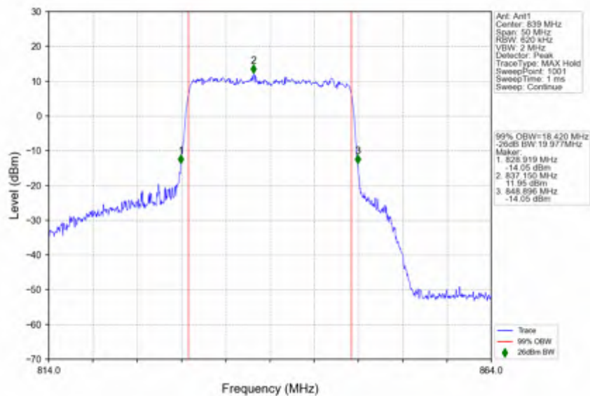
n5 30kHz SISO NTN 20MHz CP-OFDM 64 QAM 839MHz Outer Full
