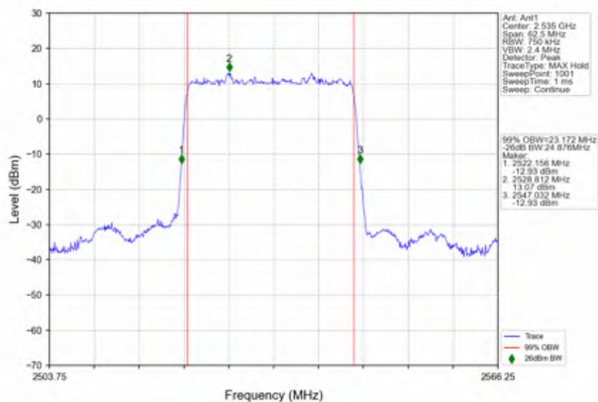
n7 15kHz SISO NTNV 25MHz DFT-s-OFDM PI/2 BPSK 2535MHz Outer Full
