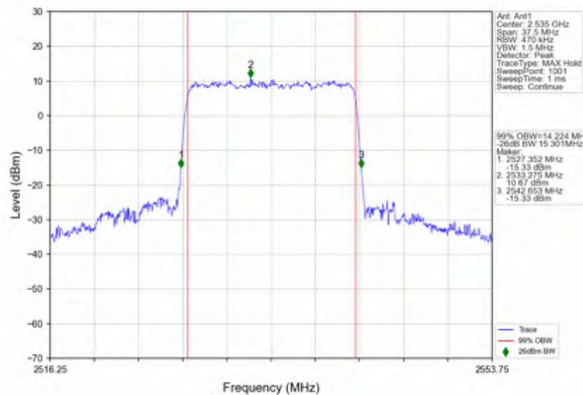
n7_15kHz_SISO_NTNV_15MHz_CP-OFDM_16_QAM_2535MHz_Outer_Full
