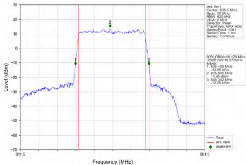
n5_30kHz_SISO_NTNV_20MHz_DFT-s-OFDM_16_QAM_836.5MHz_Outer_Full
