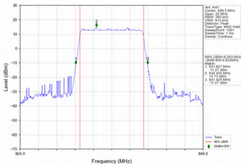
n5_30kHz_SISO_NTNV_10MHz_DFT-s-OFDM_PI/2_BPSK_836.5MHz_Outer_Full
