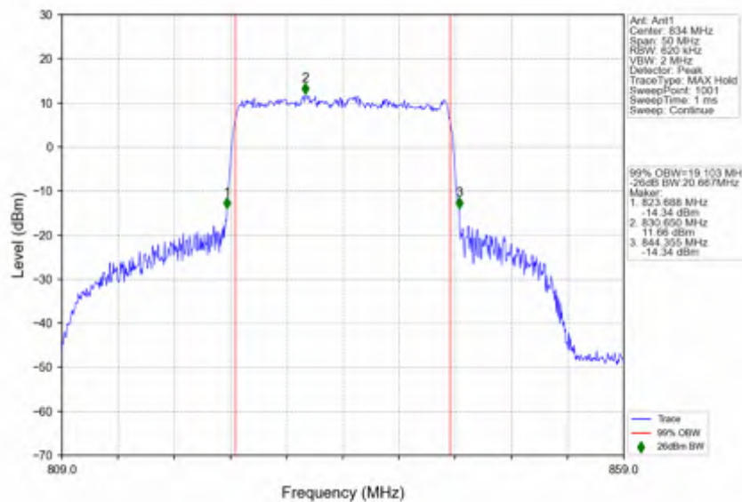
n5_15kHz_SISO_NTNV_20MHz_CP-OFDM 64 QAM_834MHz_Outer_Full
