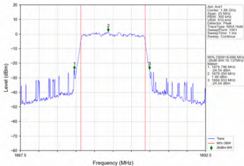
n2 30kHz SISO NTV 10MHz CP-OFDM 256 QAM 1880MHz Outer Full
