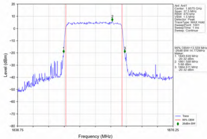
n2_15kHz_SISO_NTNV_15MHz_DFT-s-OFDM QPSK_1857.5MHz_Outer_Full
