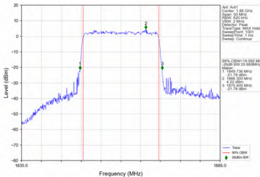
n2_15kHz_SISO_NTNV_20MHz_CP-OFDM 64 QAM_1860MHz_Outer_Full
