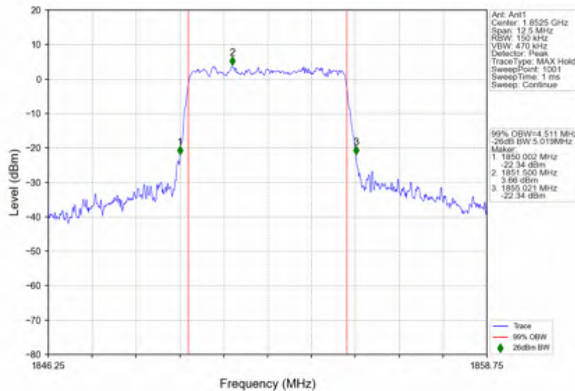
n2_15kHz_SISO_NTNV_5MHz_CP-OFDM_QPSK_1852.5MHz_Outer_Full
