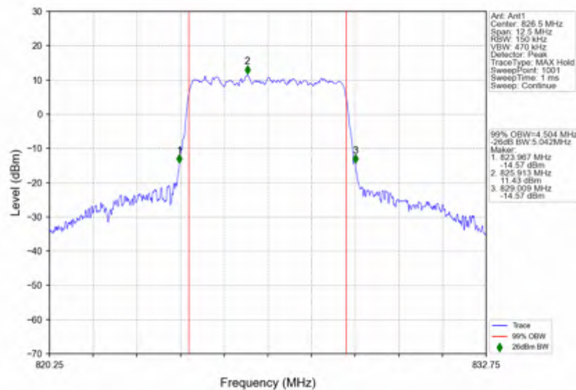
n5_15kHz_SISO_NTNV_5MHz_CP-OFDM QPSK 826.5MHz_Outer_Full
