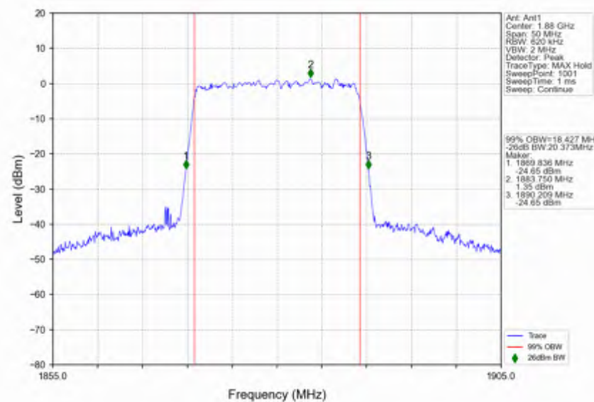
n2_30kHz_SISO_NTNV_20MHz_CP-OFDM_256_QAM_1880MHz_Outer_Full
