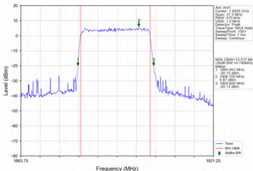
n2 15kHz SISO NTNV 15MHz DFT-s-OFDM 64 QAM 1902.5MHz Outer Full
