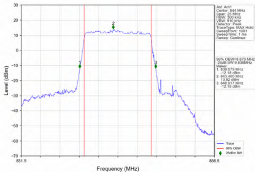
n5_30kHz_SISO_NTNV_10MHz_DFT-s-OFDM QPSK_844MHz_Outer_Full
