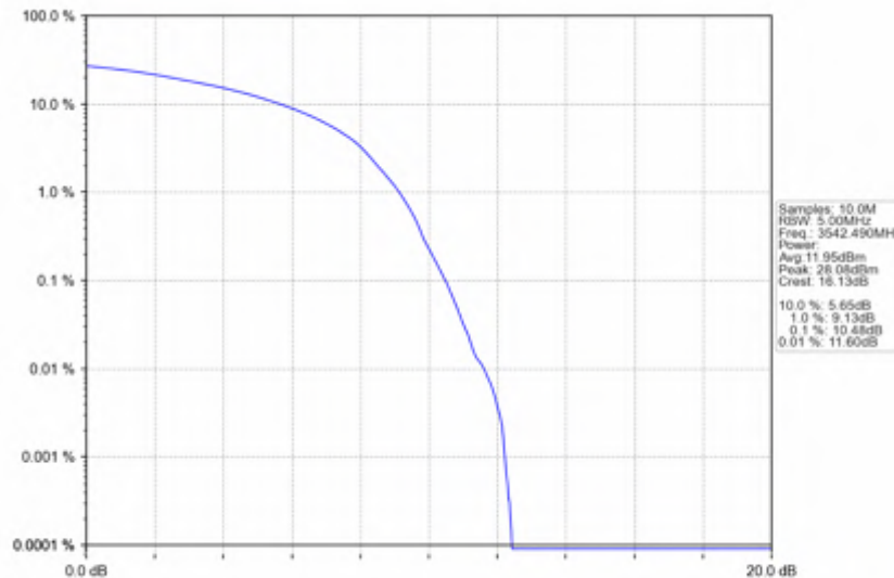
n78e_30kHz_SISO_NTNV_15MHz_DFT-s-OFDM_256_QAM_3542.49MHz_Outer_Full
