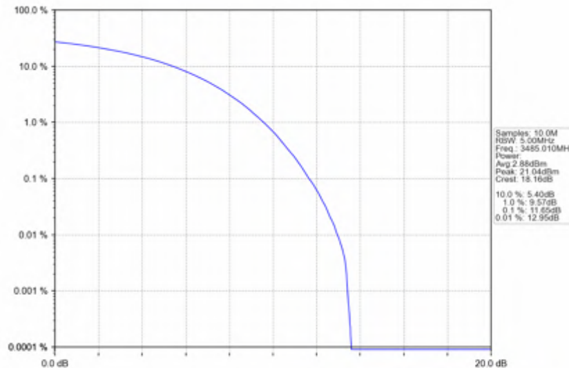
n78e_30kHz_SISO_NTNV_70MHz_CP-OFDM_256_QAM_3485.01MHz_Outer_Full
