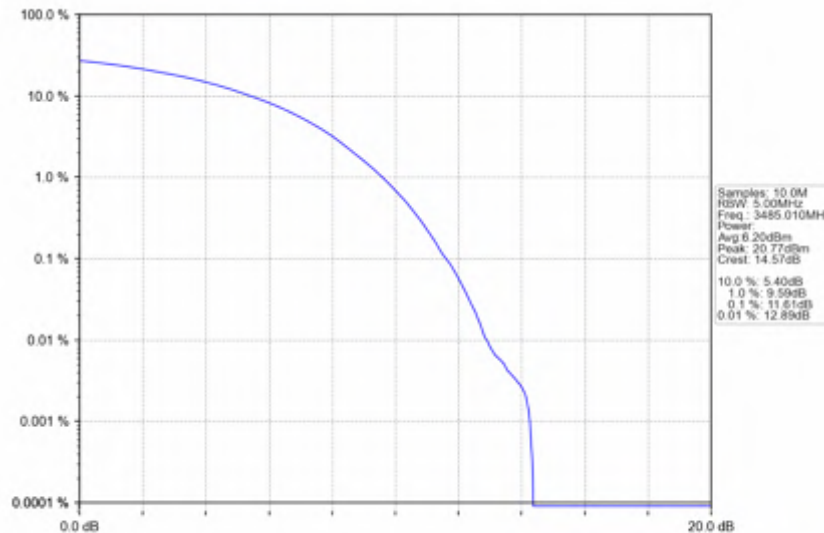
n78e_30kHz_SISO_NTNV_70MHz_CP-OFDM_QPSK_3485.01MHz_Outer_Full
