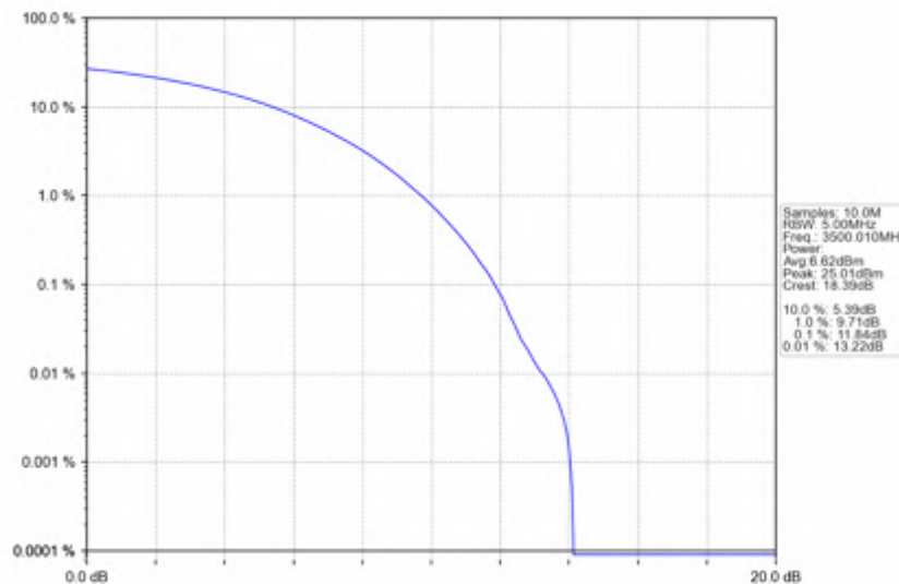
n78e_30kHz_SISO_NTNV_30MHz_CP-OFDM_256_QAM_3500.01MHz_Outer_Full
