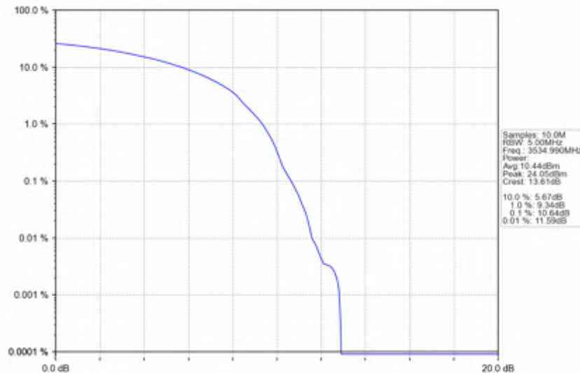
n78e_30kHz_SISO_NTNV_30MHz_DFT-s-OFDM_QPSK_3534.99MHz_Outer_Full
