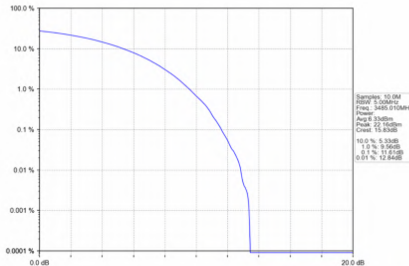
n78e_30kHz_SISO_NTNV_70MHz_CP-OFDM_16_QAM_3485.01MHz_Outer_Full
