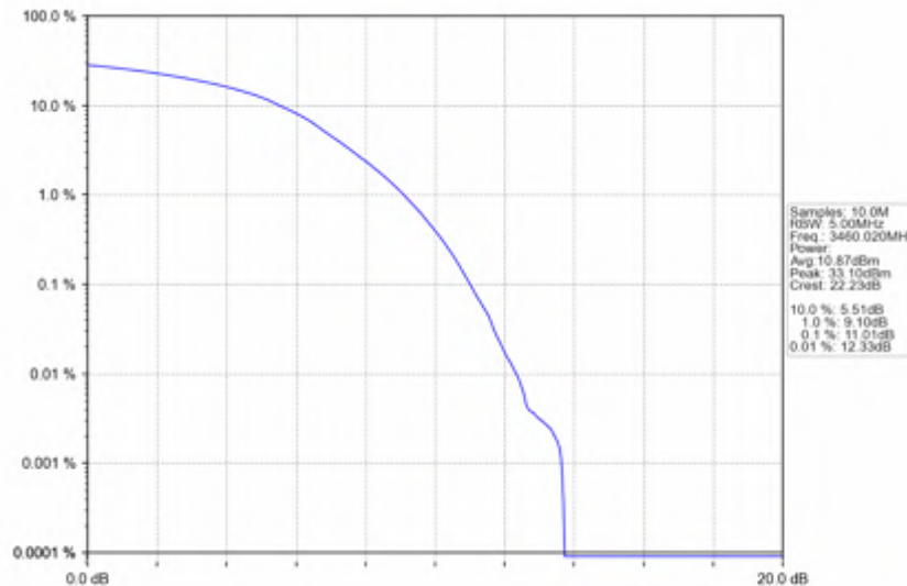
n78e_30kHz_SISO_NTNV_20MHz_DFT-s-OFDM_256_QAM_3460.02MHz_Outer_Full
