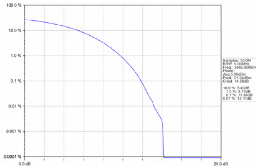
n78e_30kHz_SISO_NTNV_30MHz_CP-OFDM_256_QAM_3465MHz_Outer_Full
