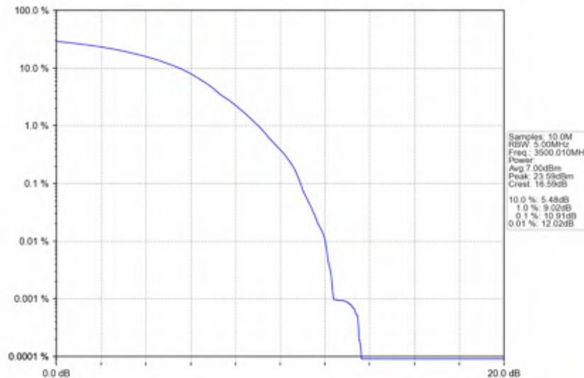
n78e_30kHz_SISO_NTNV_60MHz_DFT-s-OFDM_QPSK_3500.01MHz_Outer_Full
