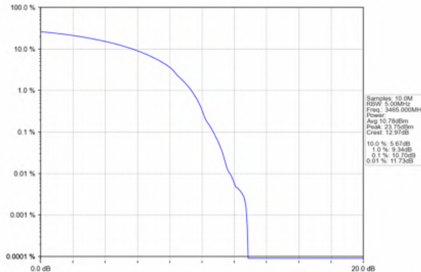
n78e_30kHz_SISO_NTNV_30MHz_DFT-s-OFDM QPSK_3465MHz_Outer_Full
