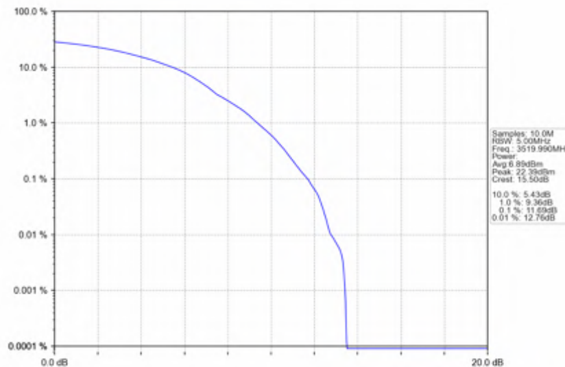
n78e_30kHz_SISO_NTNV_60MHz_DFT-s-OFDM 16 QAM_3519.99MHz_Outer_Full
