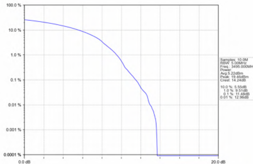
n78e_30kHz_SISO_NTNV_90MHz_DFT-s-OFDM QPSK_3495MHz_Outer_Full
