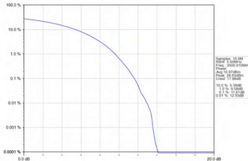
n78e_30kHz_SISO_NTNV_25MHz_CP-OFDM QPSK_3500.01MHz_Outer_Full
