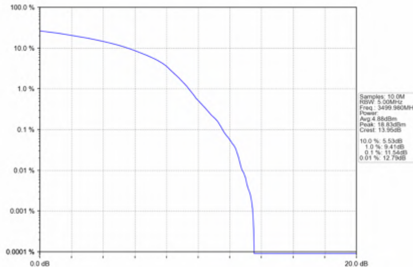
n78e_30kHz_SISO_NTNV_100MHz_DFT-s-OFDM 16 QAM_3499.98MHz_Outer_Full
