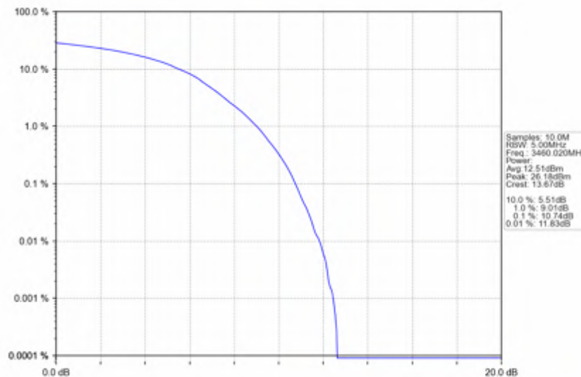
n78e_30kHz_SISO_NTNV_20MHz_DFT-s-OFDM 64 QAM_3460.02MHz_Outer_Full
