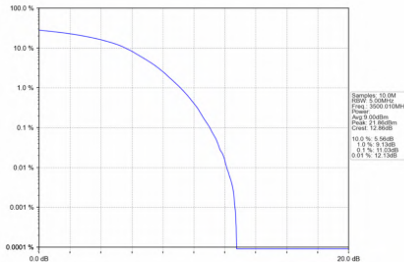
n78e_30kHz_SISO_NTNV_40MHz_DFT-s-OFDM_QPSK_3500.01MHz_Outer_Full
