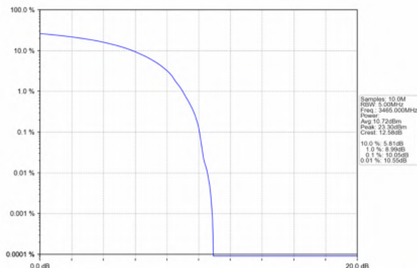
n78e 30kHz SISO NTNV 30MHz DFT-s-OFDM PI/2 BPSK 3465MHz Outer Full
