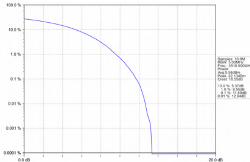
n78e_30kHz_SISO_NTNV_80MHz_CP-OFDM QPSK_3510MHz_Outer_Full
