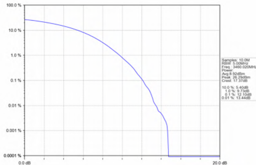
n78e_30kHz_SISO_NTNV_20MHz_CP-OFDM_256_QAM_3460.02MHz_Outer_Full
