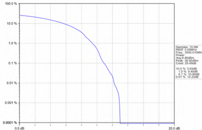
n78e_30kHz_SISO_NTNV_25MHz_DFT-s-OFDM_256_QAM_3500.01MHz_Outer_Full
