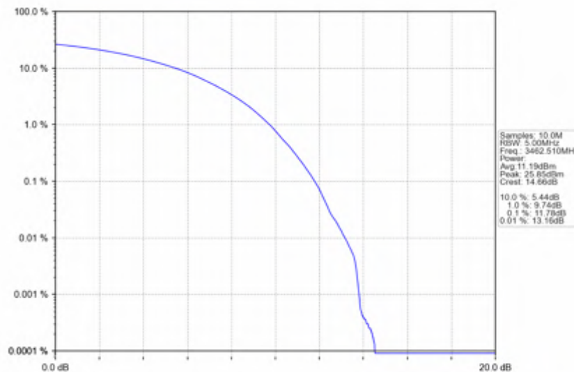
n78e_30kHz_SISO_NTNV_25MHz_CP-OFDM_QPSK_3462.51MHz_Outer_Full
