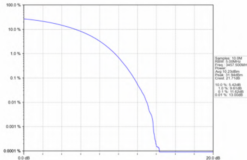
n78e_30kHz_SISO_NTNV_15MHz_CP-OFDM_256_QAM_3457.5MHz_Outer_Full
