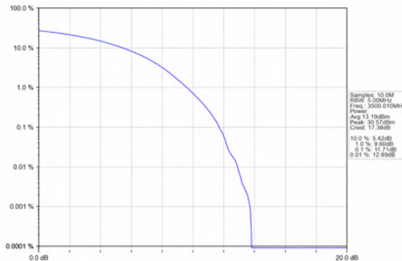
n78e_30kHz_SISO_NTNV_15MHz_CP-OFDM_QPSK_3500.01MHz_Outer_Full
