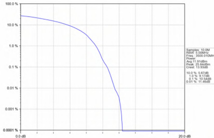
n78e_30kHz_SISO_NTV_15MHz_DFT-s-OFDM_256_QAM_3500.01MHz_Outer_Full
