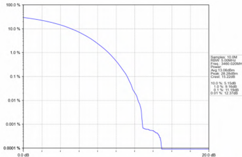
n78e_30kHz_SISO_NTNV_20MHz_CP-OFDM_QPSK_3460.02MHz_Outer_Full
