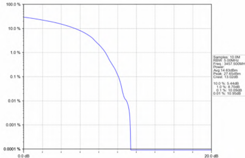
n78e_30kHz_SISO_NTNV_15MHz_DFT-s-OFDM_16_QAM_3457.5MHz_Outer_Full
