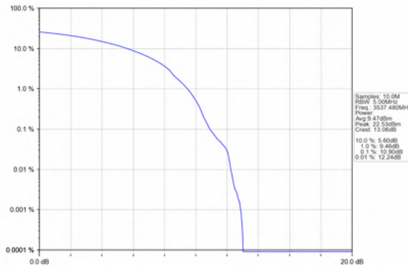
n78e_30kHz_SISO_NTNV_25MHz_DFT-s-OFDM_256_QAM_3537.48MHz_Outer_Full
