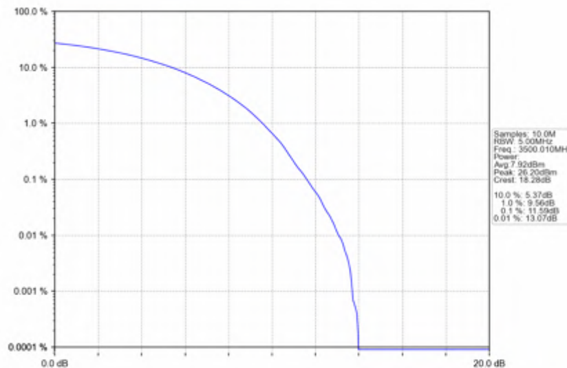
n78e_30kHz_SISO_NTNV_50MHz_CP-OFDM 16 QAM_3500.01MHz_Outer_Full
