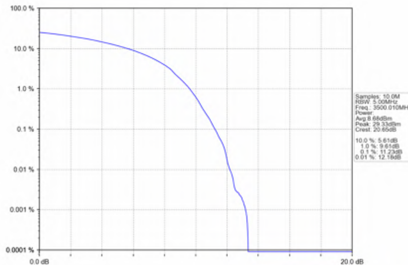
n78e_30kHz_SISO_NTNV_30MHz_DFT-s-OFDM_256_QAM_3500.01MHz_Outer_Full
