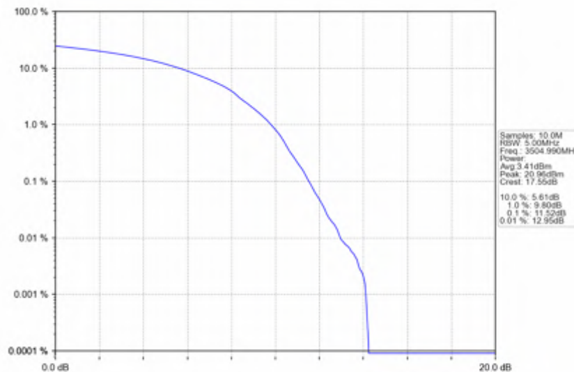
n78e_30kHz_SISO_NTNV_90MHz_DFT-s-OFDM_256_QAM_3504.99MHz_Outer_Full
