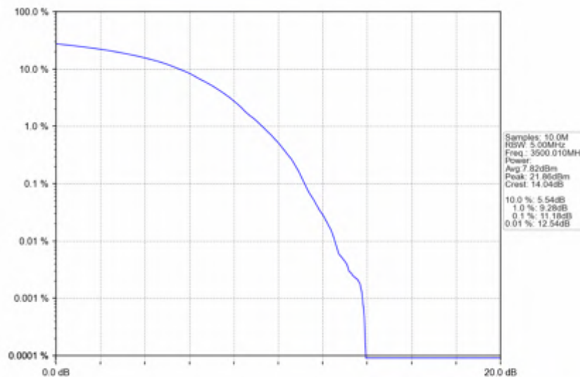
n78e_30kHz_SISO_NTNV_50MHz_DFT-s-OFDM_QPSK_3500.01MHz_Outer_Full
