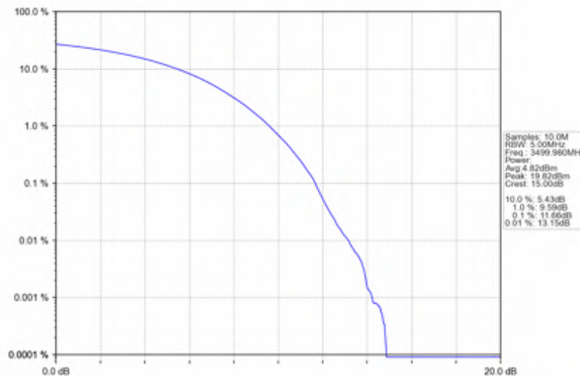
n78e_30kHz_SISO_NTNV_100MHz_CP-OFDM 16 QAM_3499.98MHz_Outer_Full
