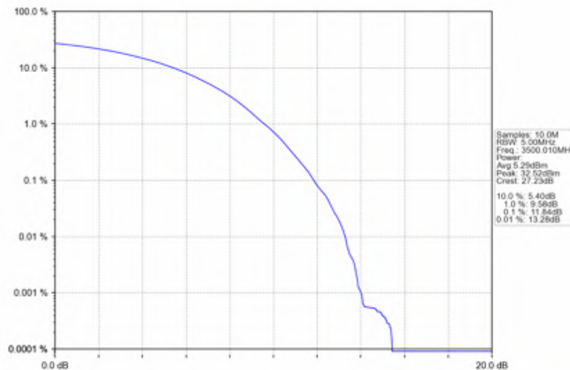
n78e_30kHz_SISO_NTNV_40MHz_CP-OFDM_256_QAM_3500.01MHz_Outer_Full
