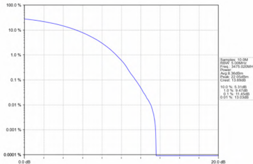
n78e_30kHz_SISO_NTNV_50MHz_CP-OFDM 16 QAM_3475.02MHz_Outer_Full
