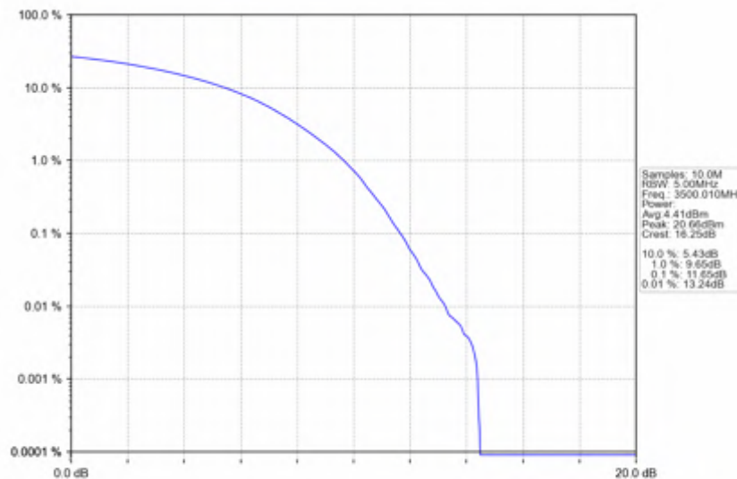
n78e_30kHz_SISO_NTNV_50MHz_CP-OFDM_256_QAM_3500.01MHz_Outer_Full
