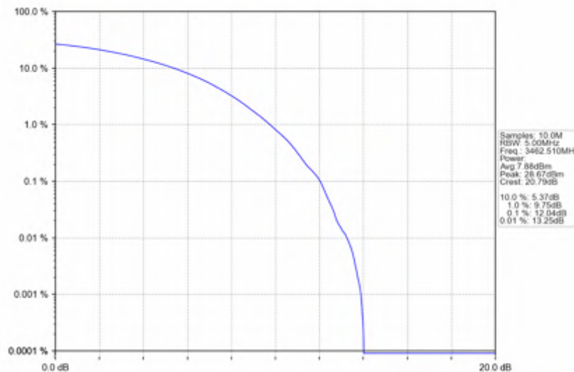
n78e_30kHz_SISO_NTNV_25MHz_CP-OFDM_256_QAM_3462.51MHz_Outer_Full
