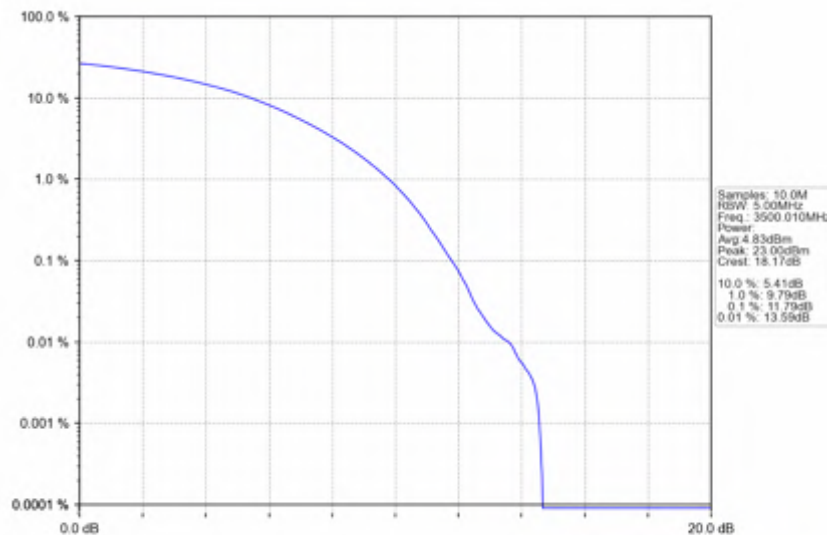
n78e_30kHz_SISO_NTNV_90MHz_CP-OFDM QPSK_3500.01MHz_Outer_Full
