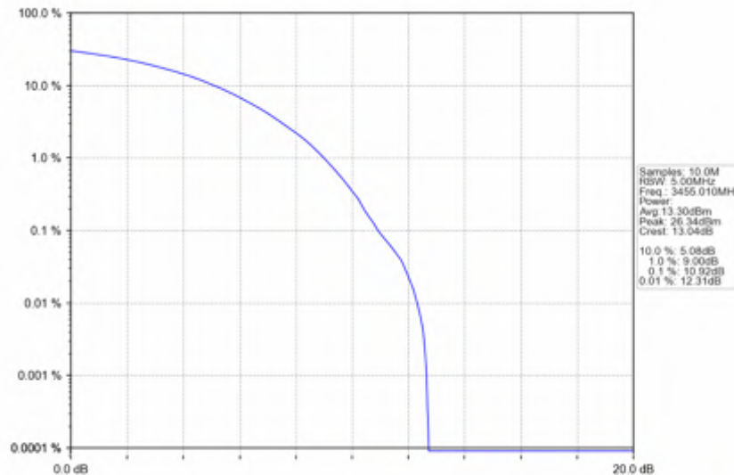
n78e_30kHz_SISO_NTNV_10MHz_CP-OFDM_256_QAM_3455.01MHz_Outer_Full
