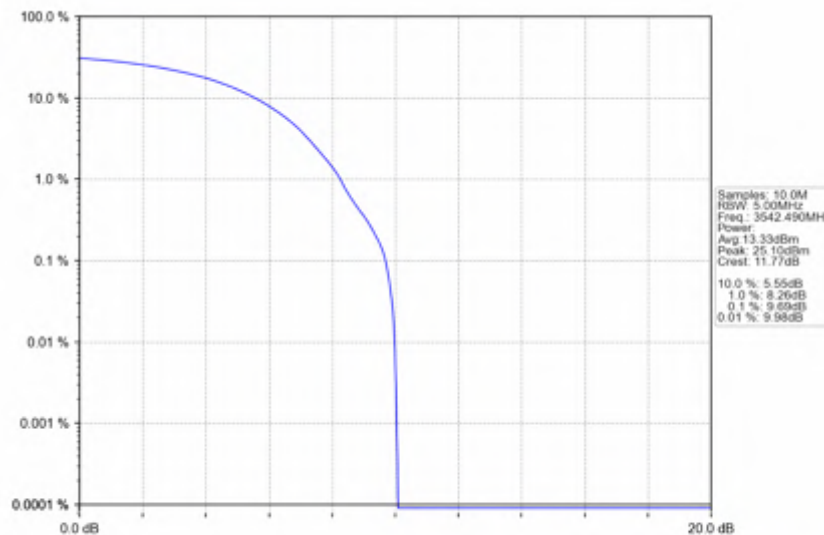
n78e_30kHz_SISO_NTNV_15MHz_DFT-s-OFDM PI/2 BPSK_3542.49MHz_Outer_Full
