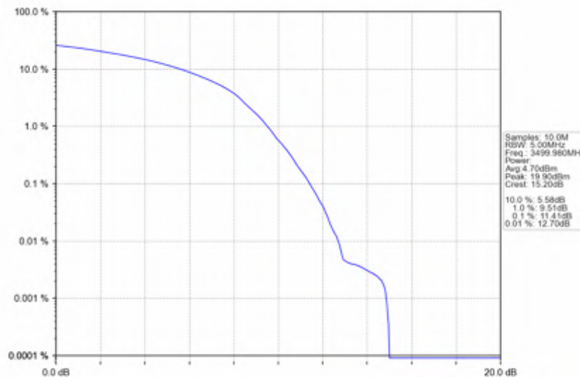
n78e_30kHz_SISO_NTNV_100MHz_DFT-s-OFDM_QPSK_3499.98MHz_Outer_Full
