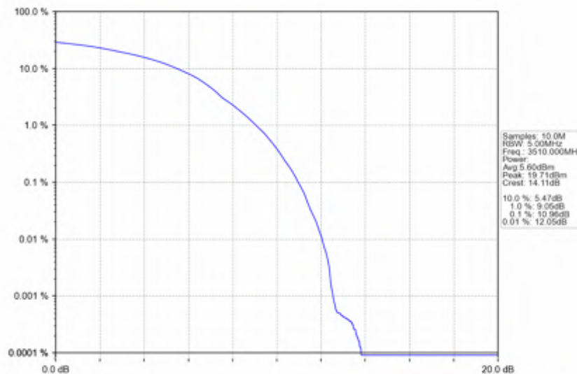
n78e_30kHz_SISO_NTNV_80MHz_DFT-s-OFDM PI/2 BPSK_3510MHz_Outer_Full
