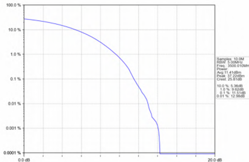
n78e_30kHz_SISO_NTNV_20MHz_CP-OFDM 64 QAM_3500.01MHz_Outer_Full
