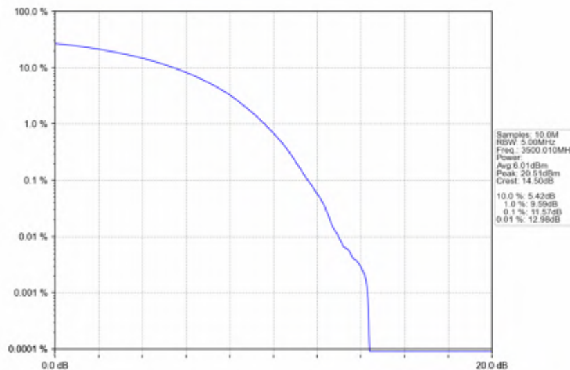
n78e_30kHz_SISO_NTNV_70MHz_CP-OFDM_QPSK_3500.01MHz_Outer_Full
