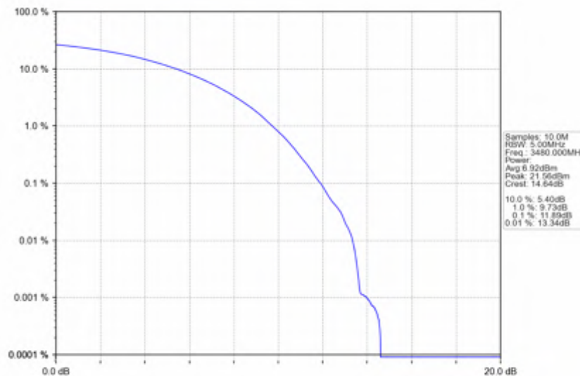
n78e_30kHz_SISO_NTNV_60MHz_CP-OFDM_QPSK_3480MHz_Outer_Full
