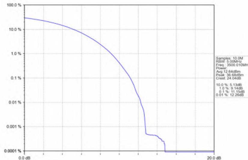
n78e_30kHz_SISO_NTNV_20MHz_CP-OFDM QPSK_3500.01MHz_Outer_Full
