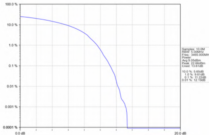
n78e_30kHz_SISO_NTNV_30MHz_DFT-s-OFDM_256_QAM_3465MHz_Outer_Full
