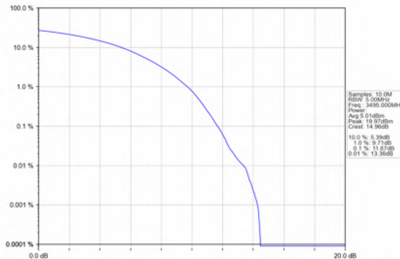
n78e_30kHz_SISO_NTNV_90MHz_CP-OFDM_QPSK_3495MHz_Outer_Full
