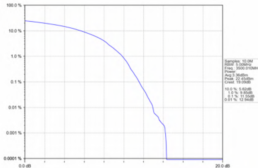
n78e_30kHz_SISO_NTNV_90MHz_DFT-s-OFDM_256_QAM_3500.01MHz_Outer_Full
