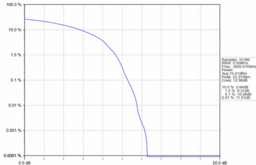
n78e_30kHz_SISO_NTNV_30MHz_DFT-s-OFDM_QPSK_3500.01MHz_Outer_Full
