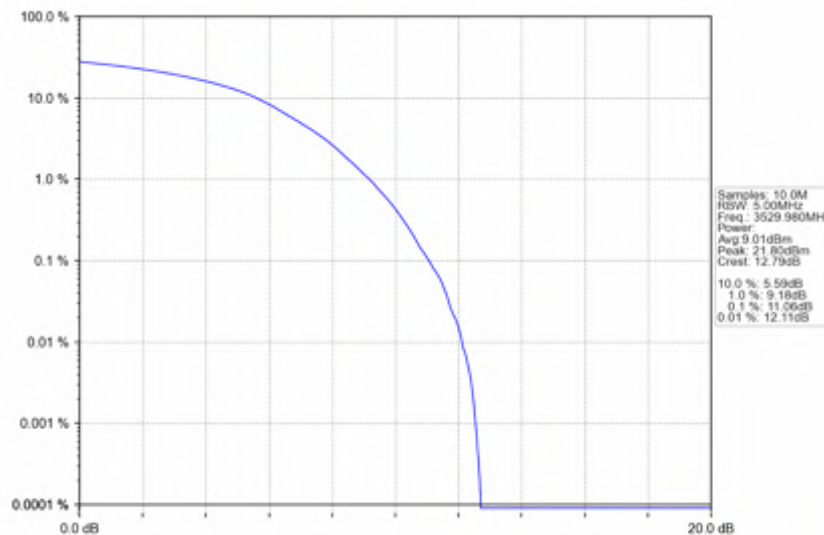
n78e_30kHz_SISO_NTNV_40MHz_DFT-s-OFDM_QPSK_3529.98MHz_Outer_Full
