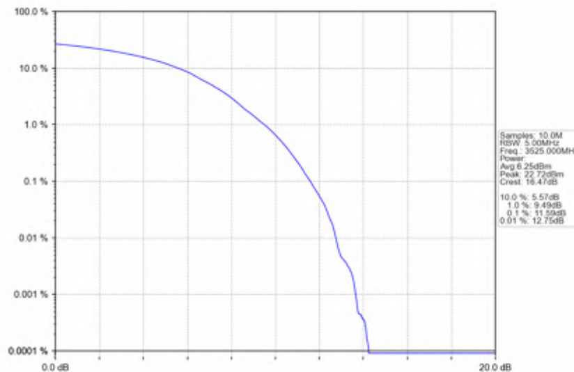
n78e_30kHz_SISO_NTNV_50MHz_DFT-s-OFDM_256_QAM_3525MHz_Outer_Full
