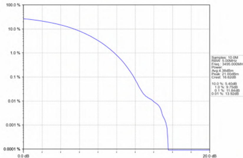
n78e_30kHz_SISO_NTNV_90MHz_CP-OFDM 64 QAM_3495MHz_Outer_Full
