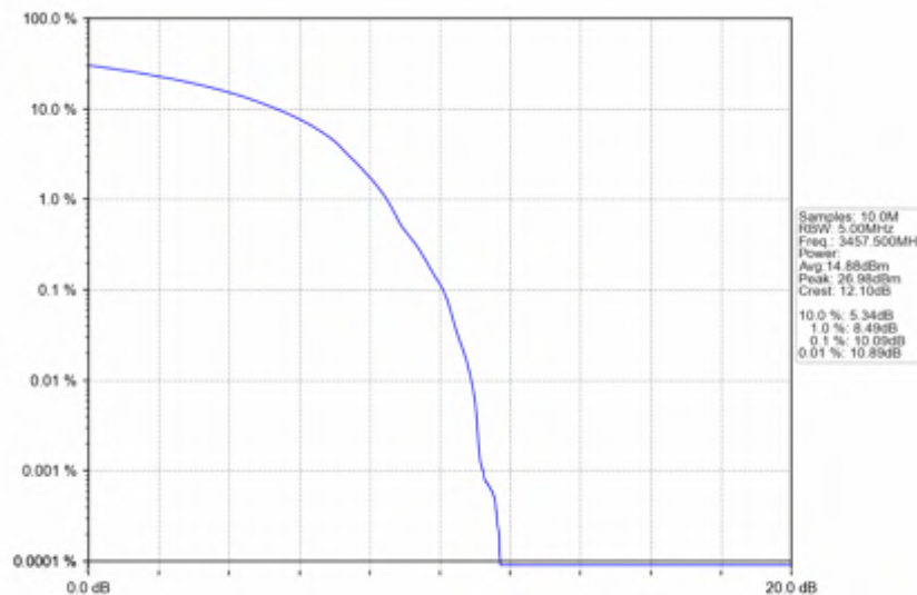
n78e_30kHz_SISO_NTNV_15MHz_DFT-s-OFDM 64 QAM_3457.5MHz_Outer_Full
