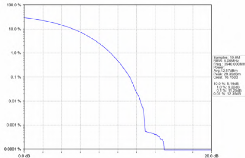
n78e_30kHz_SISO_NTNV_20MHz_CP-OFDM QPSK_3540MHz_Outer_Full
