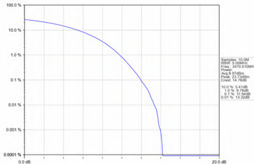
n78e_30kHz_SISO_NTNV_40MHz_CP-OFDM_QPSK_3470.01MHz_Outer_Full
