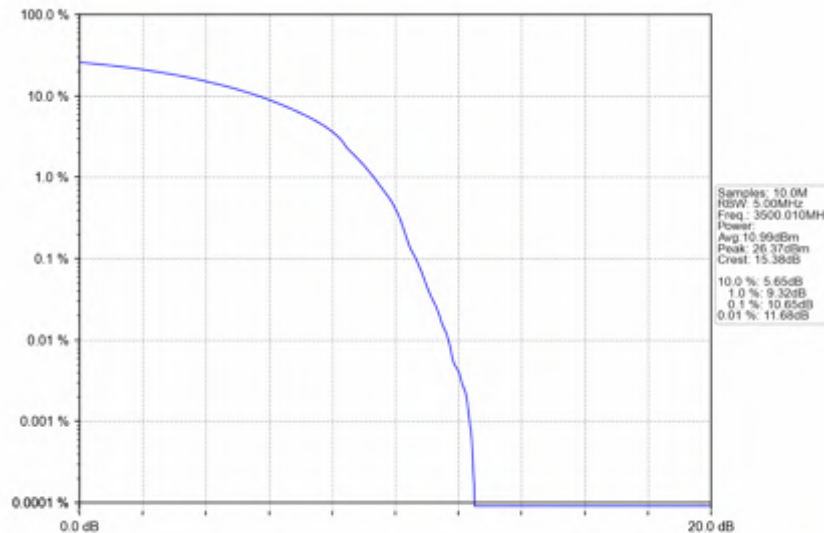
n78e_30kHz_SISO_NTNV_25MHz_DFT-s-OFDM_QPSK_3500.01MHz_Outer_Full
