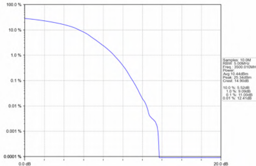
n78e_30kHz_SISO_NTNV_20MHz_DFT-s-OFDM_256_QAM_3500.01MHz_Outer_Full
