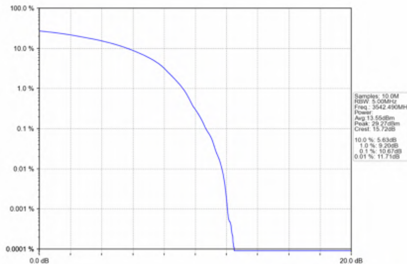
n78e_30kHz_SISO_NTV_15MHz_DFT-s-OFDM 64 QAM_3542.49MHz_Outer_Full
