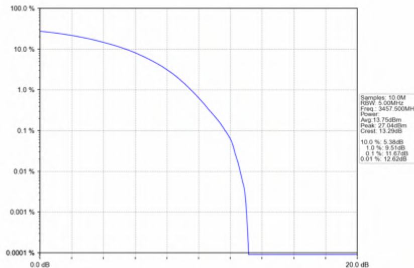
n78e_30kHz_SISO_NTNV_15MHz_CP-OFDM_16_QAM_3457.5MHz_Outer_Full
