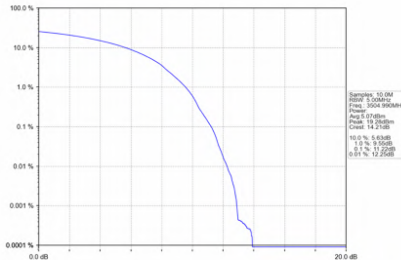
n78e_30kHz_SISO_NTNV_90MHz_DFT-s-OFDM PI/2 BPSK_3504.99MHz_Outer_Full
