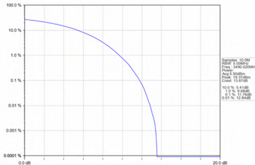
n78e_30kHz_SISO_NTNV_80MHz_CP-OFDM_QPSK_3490.02MHz_Outer_Full
