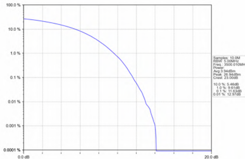
n78e_30kHz_SISO_NTNV_100MHz_CP-OFDM 64 QAM_3500.01MHz_Outer_Full
