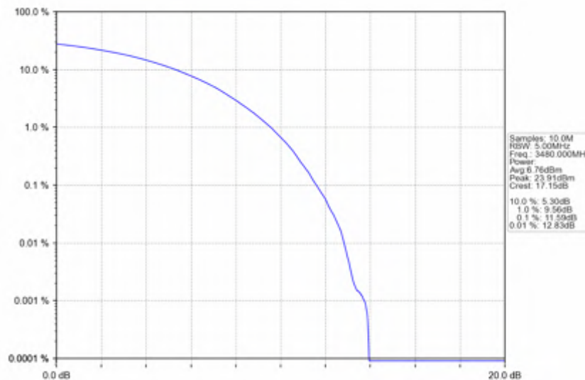
n78e_30kHz_SISO_NTNV_60MHz_CP-OFDM 64 QAM_3480MHz_Outer_Full
