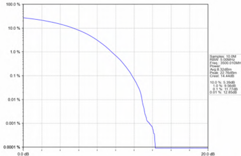
n78e_30kHz_SISO_NTNV_40MHz_CP-OFDM 64 QAM_3500.01MHz_Outer_Full
