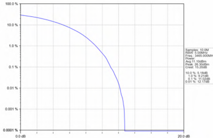
n78e_30kHz_SISO_NTNV_30MHz_CP-OFDM_QPSK_3465MHz_Outer_Full
