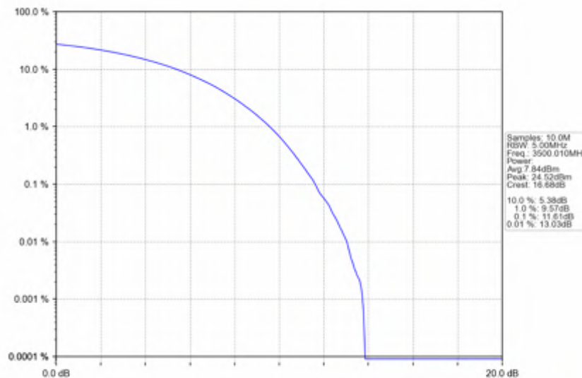
n78e_30kHz_SISO_NTNV_50MHz_CP-OFDM QPSK_3500.01MHz_Outer_Full
