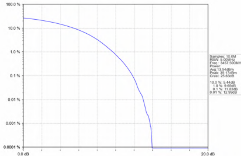
n78e_30kHz_SISO_NTNV_15MHz_CP-OFDM_QPSK_3457.5MHz_Outer_Full
