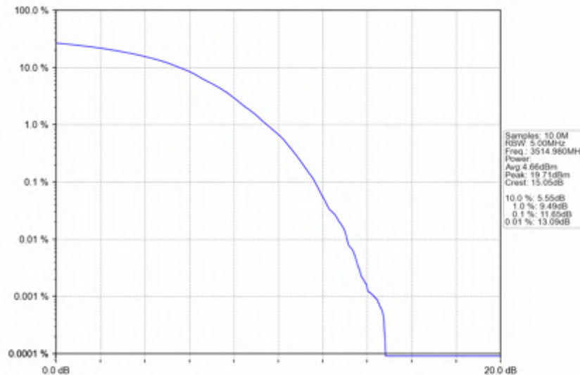
n78e_30kHz_SISO_NTNV_70MHz_DFT-s-OFDM_256_QAM_3514.98MHz_Outer_Full
