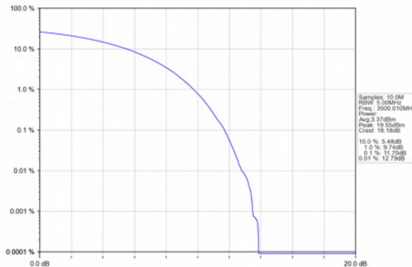
n78e_30kHz_SISO_NTNV_60MHz_CP-OFDM_256_QAM_3500.01MHz_Outer_Full
