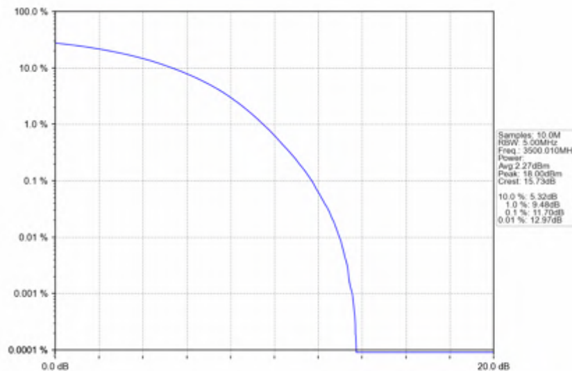
n78e_30kHz_SISO_NTNV_80MHz_CP-OFDM_256_QAM_3500.01MHz_Outer_Full
