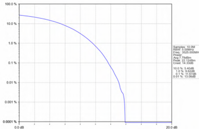
n78e_30kHz_SISO_NTNV_50MHz_CP-OFDM QPSK_3525MHz_Outer_Full
