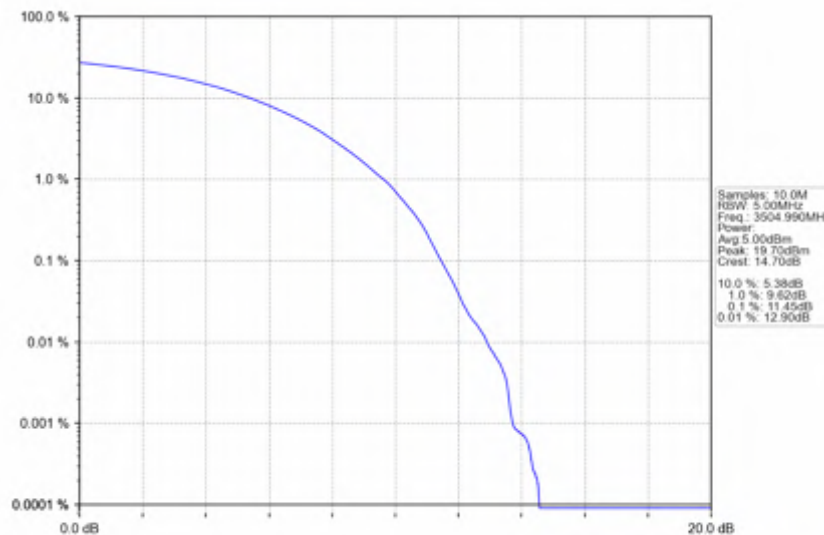
n78e_30kHz_SISO_NTNV_90MHz_CP-OFDM 16 QAM_3504.99MHz_Outer_Full
