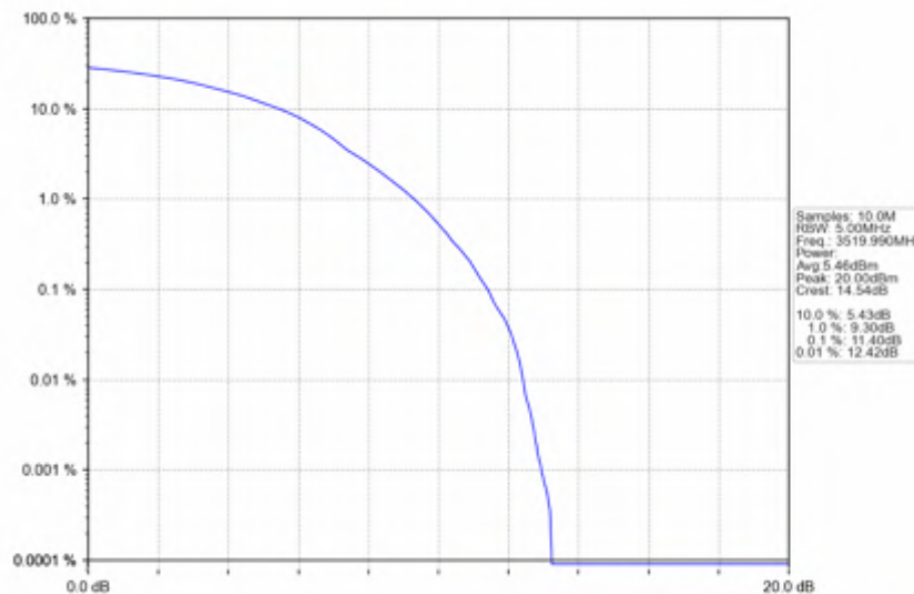
n78e_30kHz_SISO_NTNV_60MHz_DFT-s-OFDM_256_QAM_3519.99MHz_Outer_Full
