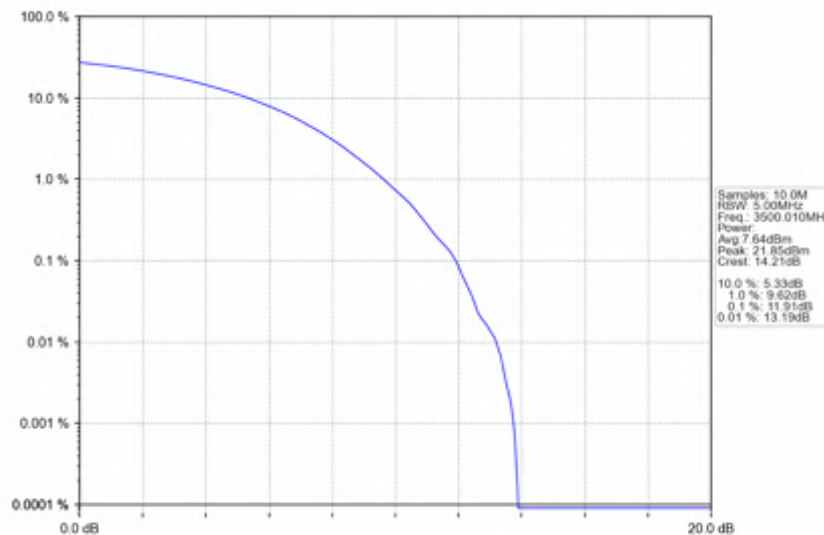
n78e_30kHz_SISO_NTNV_25MHz_CP-OFDM_256_QAM_3500.01MHz_Outer_Full
