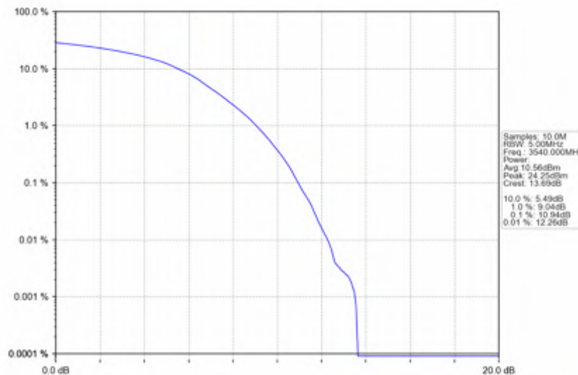
n78e_30kHz_SISO_NTNV_20MHz_DFT-s-OFDM_256_QAM_3540MHz_Outer_Full
