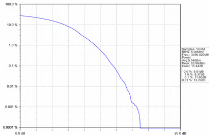
n78e_30kHz_SISO_NTNV_80MHz_DFT-s-OFDM QPSK_3490.02MHz_Outer_Full
