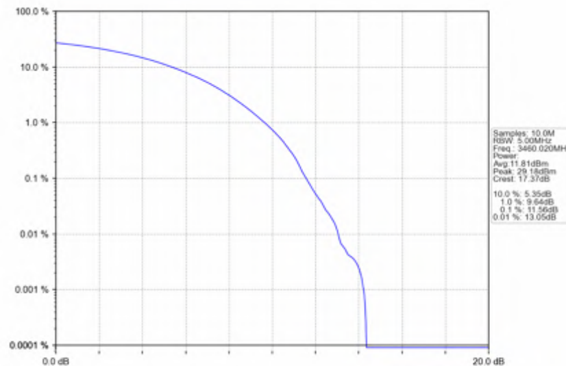
n78e_30kHz_SISO_NTNV_20MHz_CP-OFDM 64 QAM_3460.02MHz_Outer_Full
