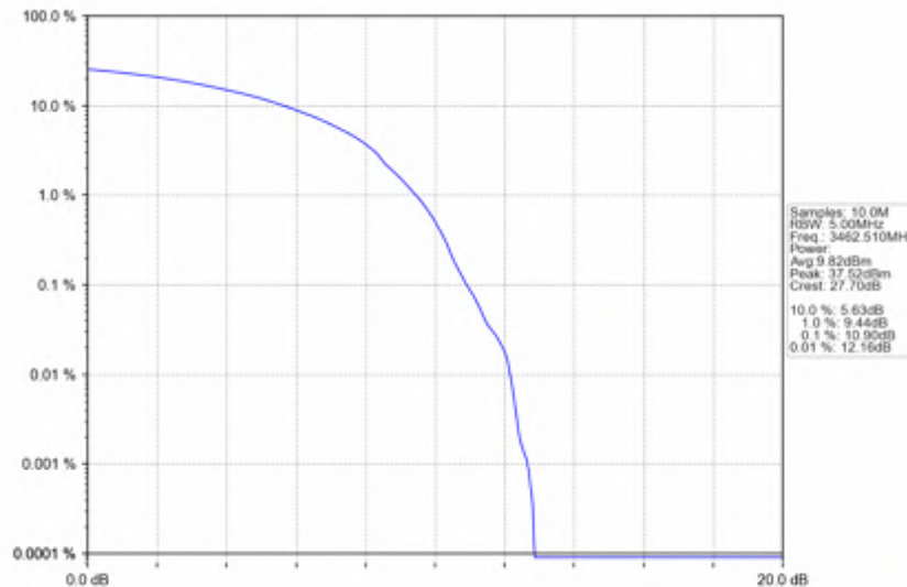
n78e_30kHz_SISO_NTNV_25MHz_DFT-s-OFDM_256_QAM_3462.51MHz_Outer_Full
