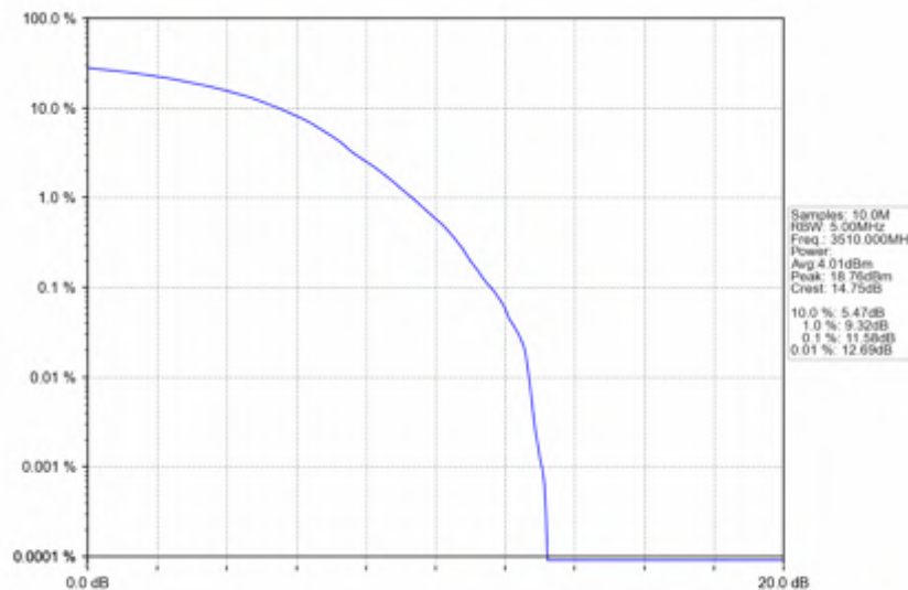
n78e_30kHz_SISO_NTNV_80MHz_DFT-s-OFDM_256_QAM_3510MHz_Outer_Full
