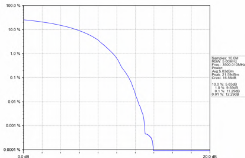
n78e_30kHz_SISO_NTNV_90MHz_DFT-s-OFDM PI/2 BPSK_3500.01MHz_Outer_Full
