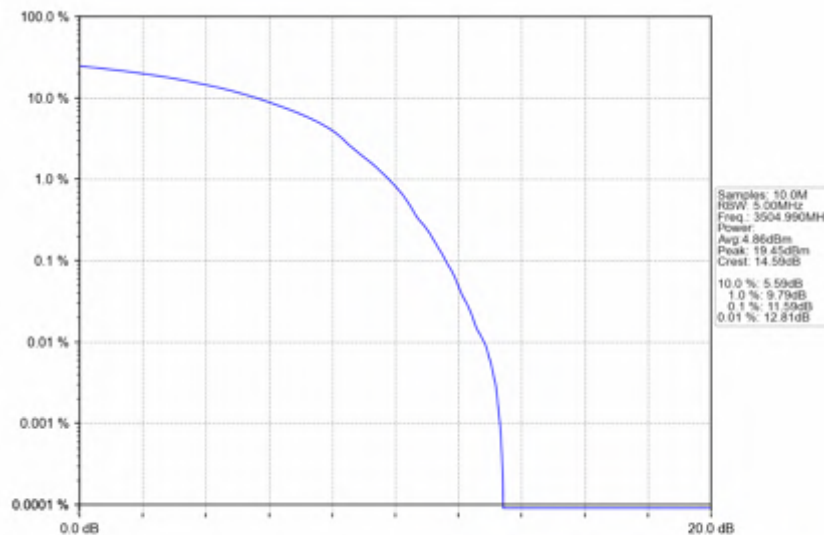
n78e_30kHz_SISO_NTV_90MHz_DFT-s-OFDM 16 QAM_3504.99MHz_Outer_Full
