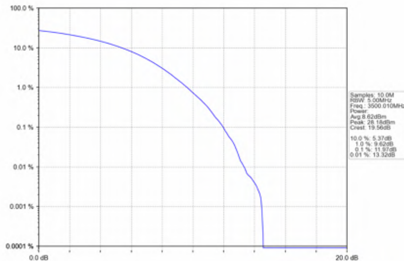
n78e_30kHz_SISO_NTNV_20MHz_CP-OFDM_256_QAM_3500.01MHz_Outer_Full
