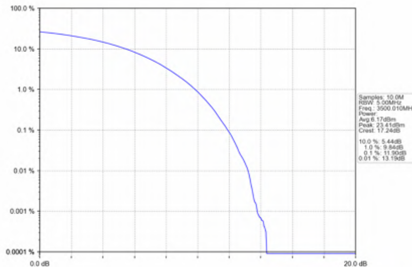
n78e_30kHz_SISO_NTNV_60MHz_CP-OFDM 64 QAM_3500.01MHz_Outer_Full
