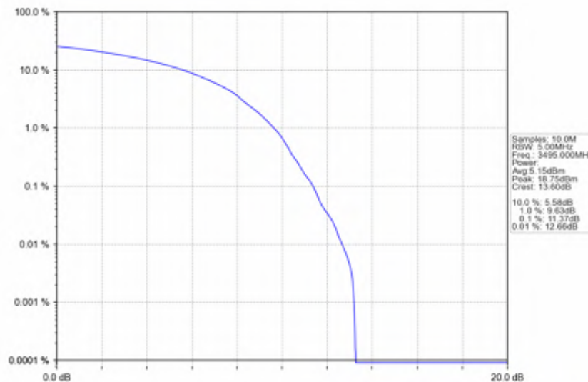
n78e_30kHz_SISO_NTV_90MHz_DFT-s-OFDM 64 QAM_3495MHz_Outer_Full
