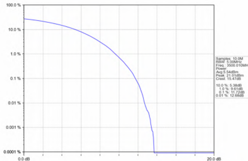
n78e_30kHz_SISO_NTNV_80MHz_CP-OFDM QPSK_3500.01MHz_Outer_Full
