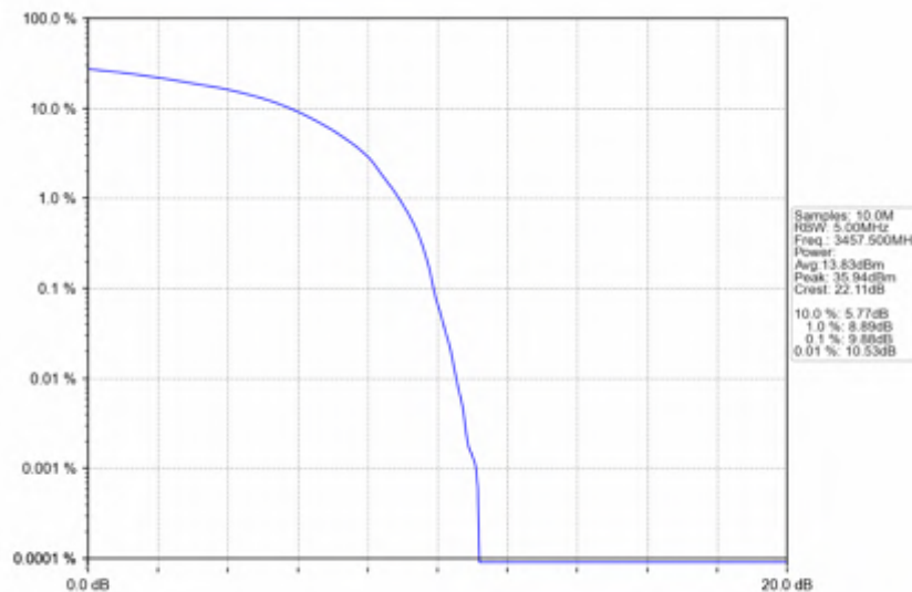
n78e_30kHz_SISO_NTNV_15MHz_DFT-s-OFDM QPSK_3457.5MHz_Outer_Full
