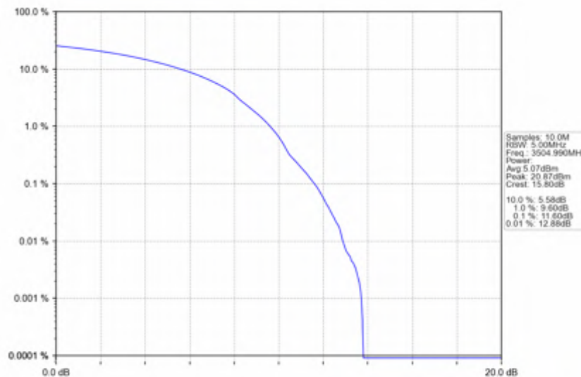
n78e_30kHz_SISO_NTNV_90MHz_DFT-s-OFDM_QPSK_3504.99MHz_Outer_Full
