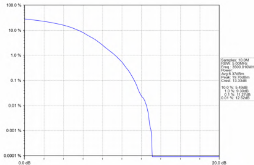
n78e_30kHz_SISO_NTNV_70MHz_DFT-s-OFDM_QPSK_3500.01MHz_Outer_Full
