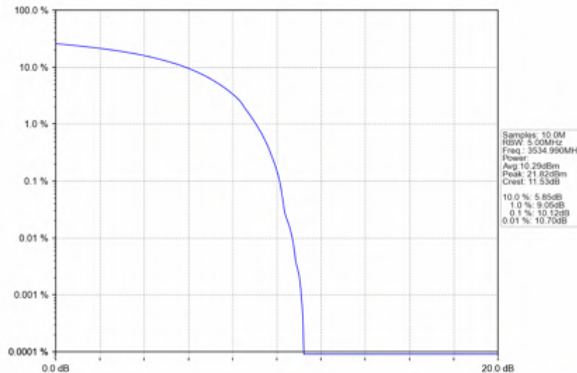
n78e_30kHz_SISO_NTNV_30MHz_DFT-s-OFDM PI/2 BPSK_3534.99MHz_Outer_Full
