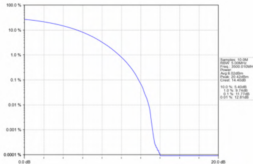
n78e_30kHz_SISO_NTNV_70MHz_CP-OFDM_16_QAM_3500.01MHz_Outer_Full
