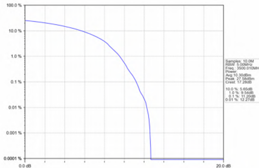
n78e_30kHz_SISO_NTV_30MHz_DFT-s-OFDM_64_QAM_3500.01MHz_Outer_Full
