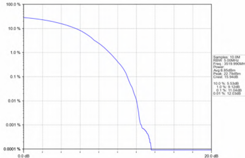
n78e_30kHz_SISO_NTNV_60MHz_DFT-s-OFDM_QPSK_3519.99MHz_Outer_Full
