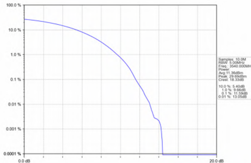
n78e_30kHz_SISO_NTNV_20MHz_CP-OFDM 64 QAM_3540MHz_Outer_Full
