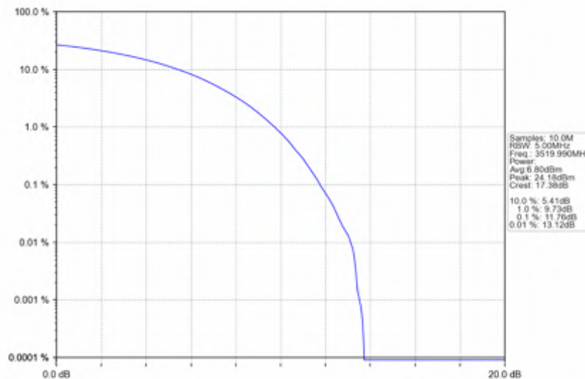
n78e_30kHz_SISO_NTNV_60MHz_CP-OFDM 16 QAM_3519.99MHz_Outer_Full
