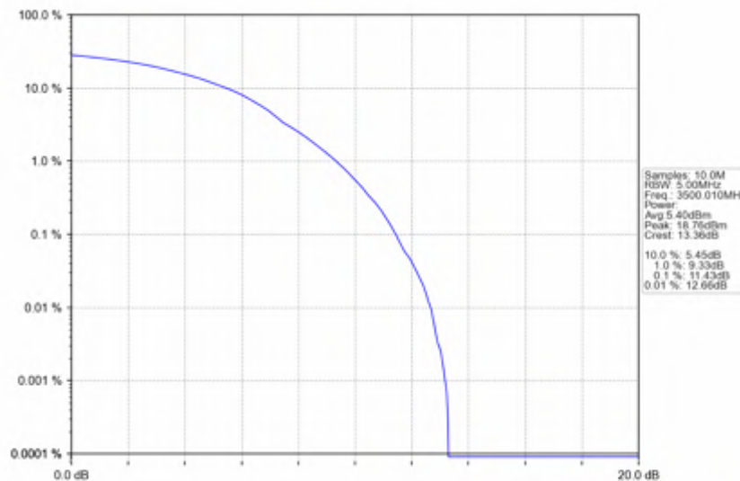
n78e_30kHz_SISO_NTNV_60MHz_DFT-s-OFDM_256_QAM_3500.01MHz_Outer_Full
