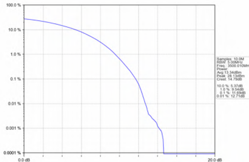
n78e_30kHz_SISO_NTNV_15MHz_CP-OFDM_16_QAM_3500.01MHz_Outer_Full
