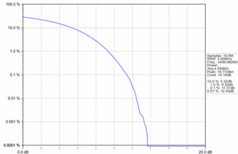
n78e_30kHz_SISO_NTNV_100MHz_CP-OFDM 64 QAM_3499.98MHz_Outer_Full
