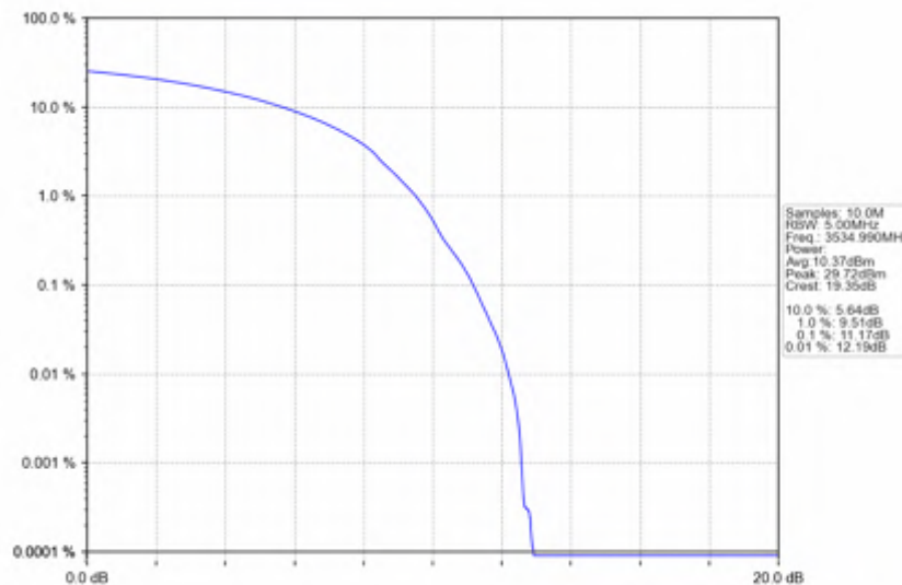
n78e_30kHz_SISO_NTV_30MHz_DFT-s-OFDM_64_QAM_3534.99MHz_Outer_Full
