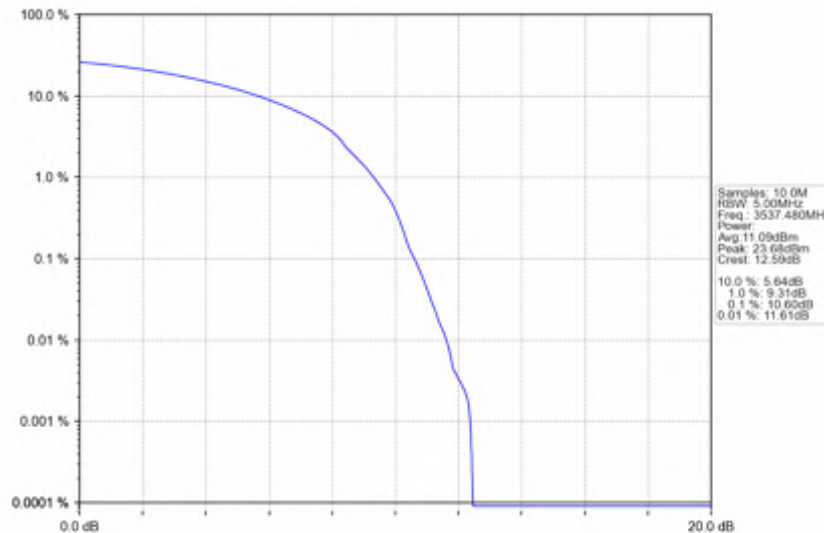
n78e_30kHz_SISO_NTNV_25MHz_DFT-s-OFDM_QPSK_3537.48MHz_Outer_Full
