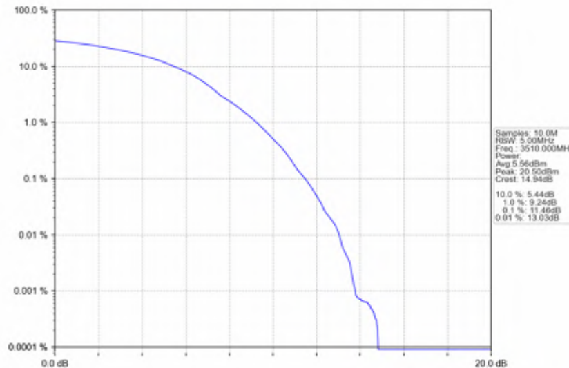
n78e_30kHz_SISO_NTNV_80MHz_DFT-s-OFDM_QPSK_3510MHz_Outer_Full
