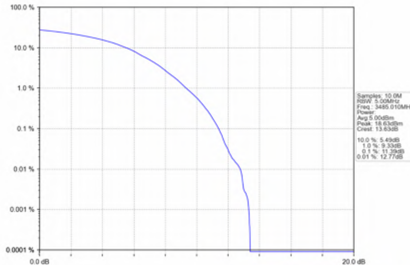
n78e_30kHz_SISO_NTNV_70MHz_DFT-s-OFDM_256_QAM_3485.01MHz_Outer_Full
