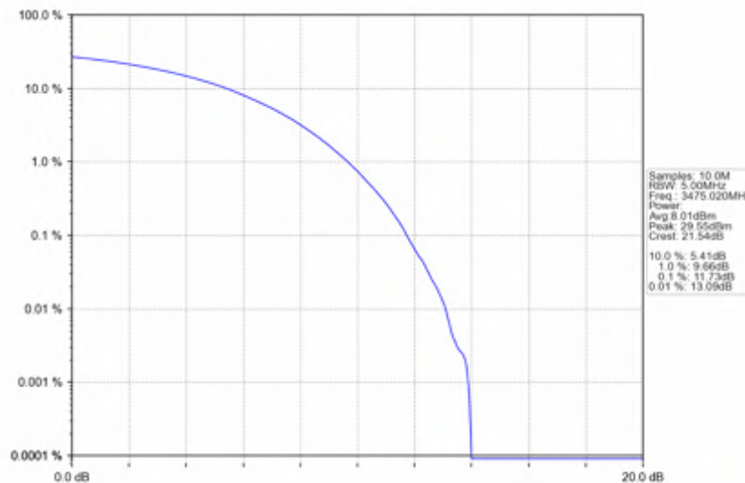
n78e_30kHz_SISO_NTNV_50MHz_CP-OFDM_QPSK_3475.02MHz_Outer_Full
