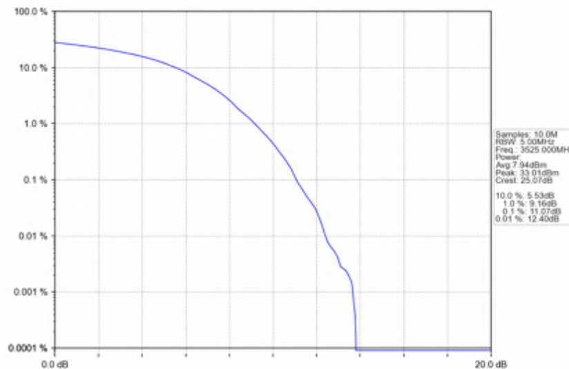
n78e_30kHz_SISO_NTNV_50MHz_DFT-s-OFDM_QPSK_3525MHz_Outer_Full
