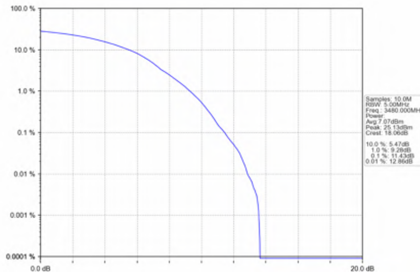
n78e_30kHz_SISO_NTNV_60MHz_DFT-s-OFDM 64 QAM_3480MHz_Outer_Full
