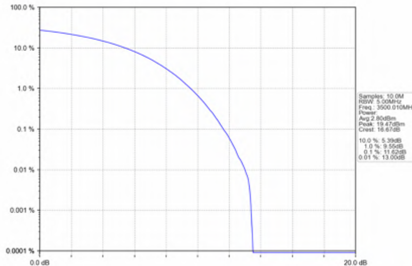
n78e_30kHz_SISO_NTNV_70MHz_CP-OFDM_256_QAM_3500.01MHz_Outer_Full
