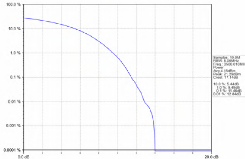
n78e_30kHz_SISO_NTNV_100MHz_CP-OFDM 64 QAM_3500.01MHz_Outer_Full
