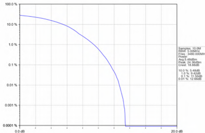
n78e_30kHz_SISO_NTNV_60MHz_DFT-s-OFDM_256_QAM_3480MHz_Outer_Full
