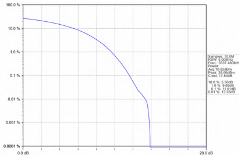
n78e_30kHz_SISO_NTNV_25MHz_CP-OFDM QPSK_3537.48MHz_Outer_Full
