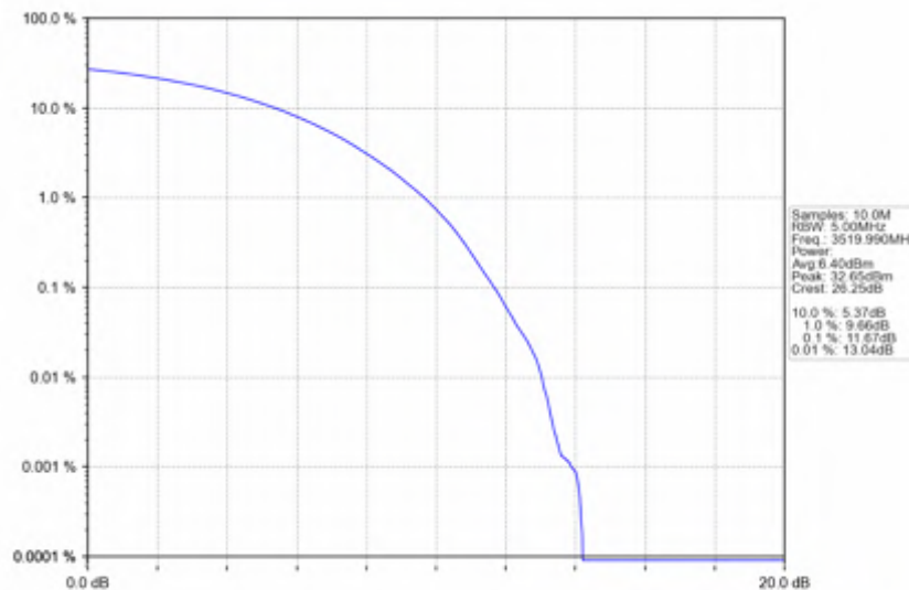
n78e_30kHz_SISO_NTNV_60MHz_CP-OFDM 64 QAM_3519.99MHz_Outer_Full
