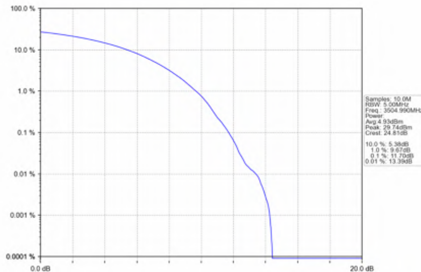
n78e_30kHz_SISO_NTNV_90MHz_CP-OFDM QPSK_3504.99MHz_Outer_Full
