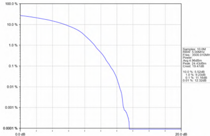
n78e_30kHz_SISO_NTNV_100MHz_DFT-s-OFDM 64 QAM_3500.01MHz_Outer_Full
