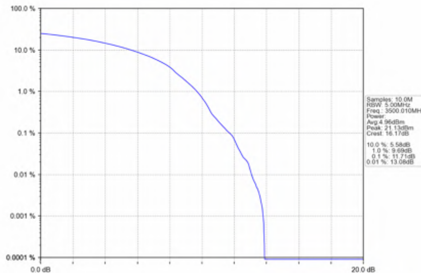
n78e_30kHz_SISO_NTNV_90MHz_DFT-s-OFDM_QPSK_3500.01MHz_Outer_Full
