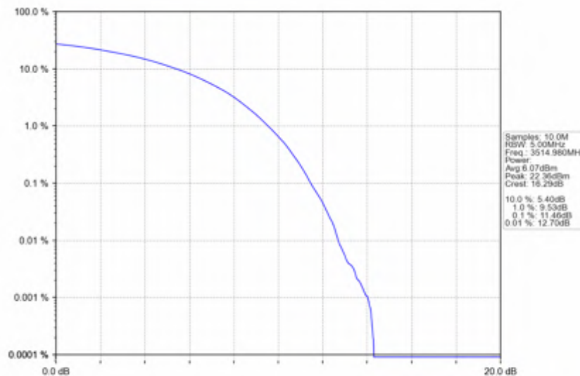
n78e_30kHz_SISO_NTNV_70MHz_CP-OFDM_QPSK_3514.98MHz_Outer_Full
