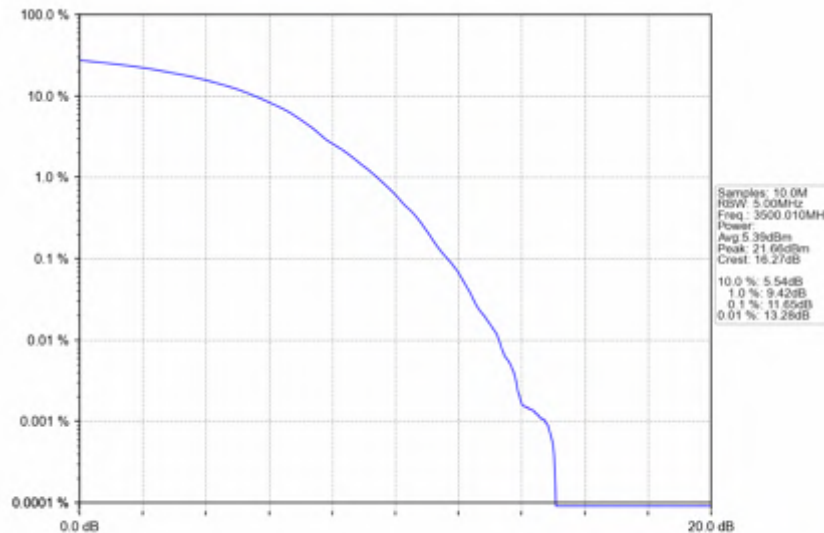
n78e_30kHz_SISO_NTNV_80MHz_DFT-s-OFDM_QPSK_3500.01MHz_Outer_Full
