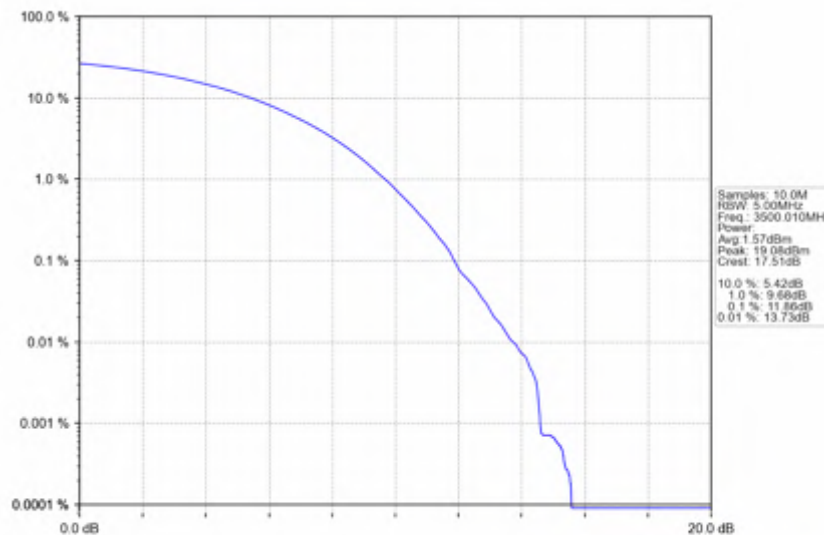
n78e_30kHz_SISO_NTNV_90MHz_CP-OFDM_256_QAM_3500.01MHz_Outer_Full
