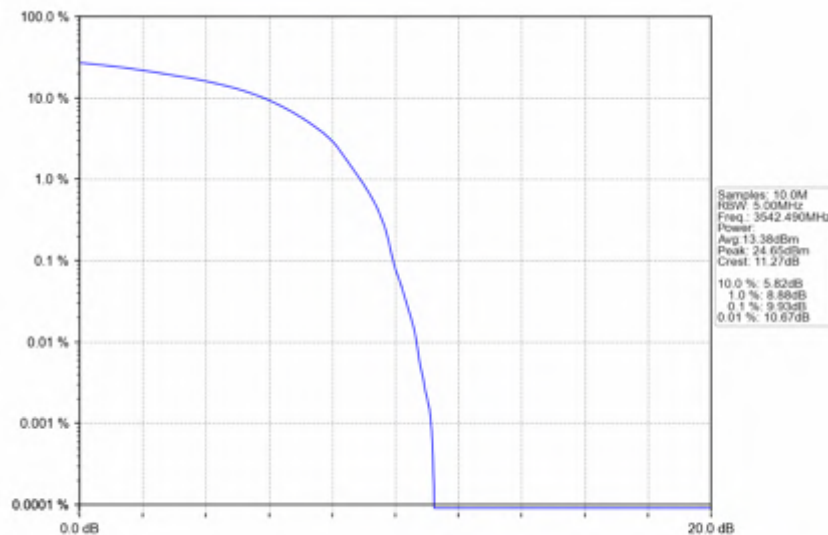
n78e_30kHz_SISO_NTNV_15MHz_DFT-s-OFDM_QPSK_3542.49MHz_Outer_Full
