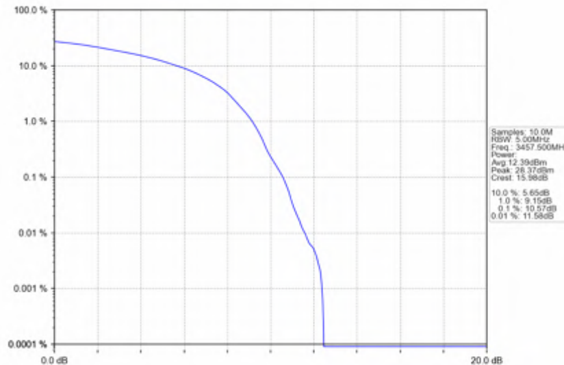
n78e_30kHz_SISO_NTV_15MHz_DFT-s-OFDM_256_QAM_3457.5MHz_Outer_Full
