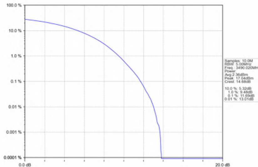
n78e_30kHz_SISO_NTNV_80MHz_CP-OFDM_256_QAM_3490.02MHz_Outer_Full
