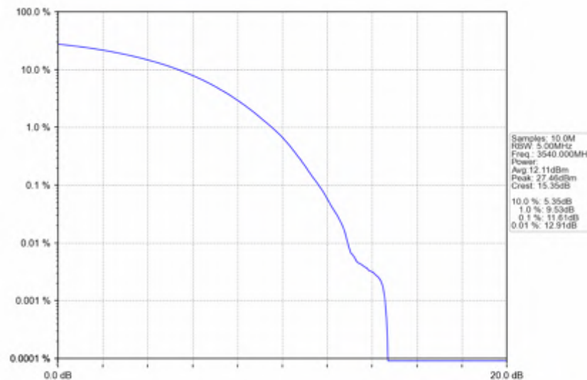
n78e_30kHz_SISO_NTNV_20MHz_CP-OFDM 16 QAM_3540MHz_Outer_Full
