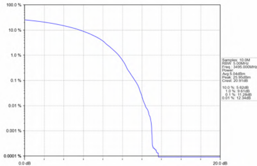
n78e_30kHz_SISO_NTNV_90MHz_DFT-s-OFDM PI/2 BPSK_3495MHz_Outer_Full
