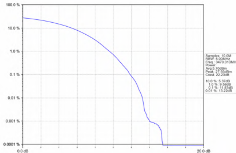
n78e_30kHz_SISO_NTNV_40MHz_CP-OFDM_256_QAM_3470.01MHz_Outer_Full
