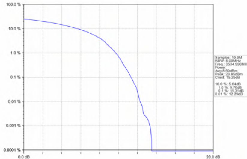
n78e_30kHz_SISO_NTNV_30MHz_DFT-s-OFDM_256_QAM_3534.99MHz_Outer_Full
