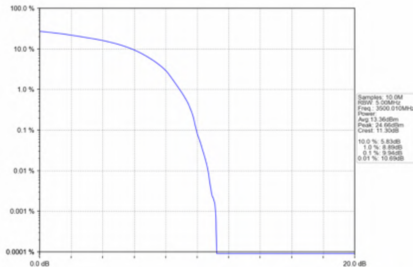
n78e_30kHz_SISO_NTNV_15MHz_DFT-s-OFDM_QPSK_3500.01MHz_Outer_Full
