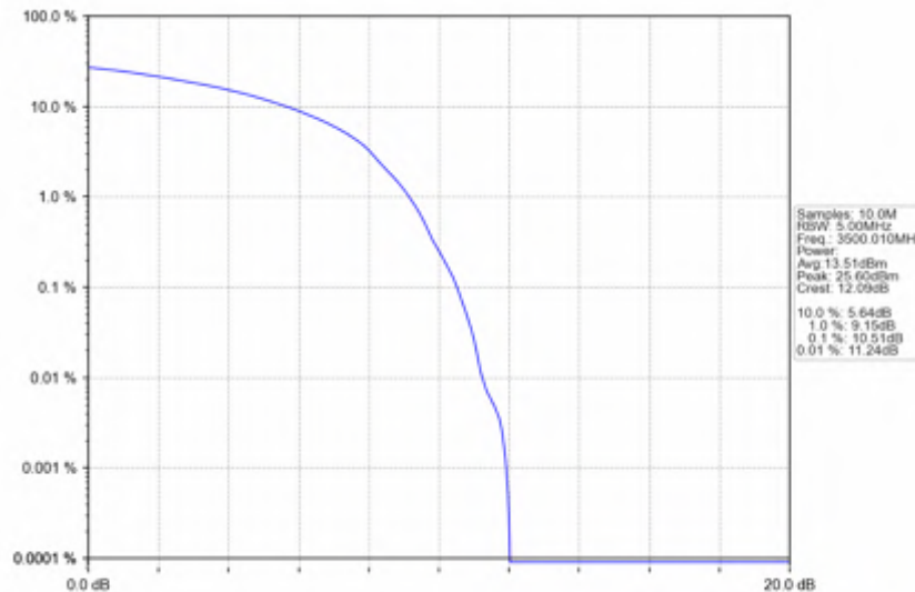
n78e_30kHz_SISO_NTNV_15MHz_DFT-s-OFDM_16_QAM_3500.01MHz_Outer_Full
