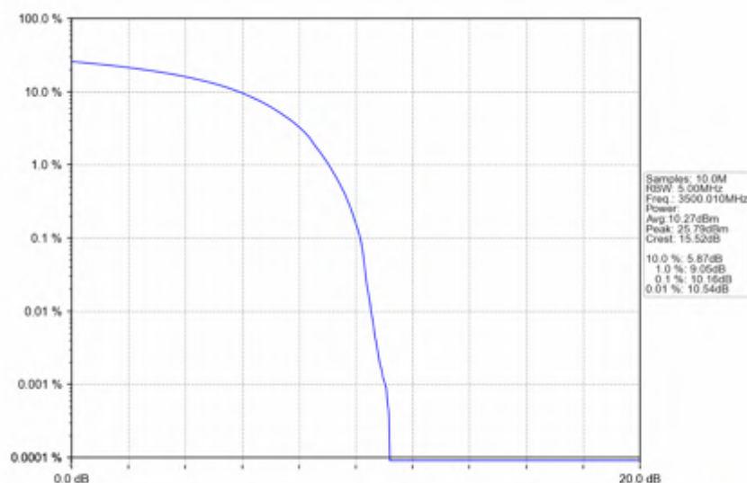
n78e 30kHz SISO NTNV 30MHz DFT-s-OFDM PI/2 BPSK 3500.01MHz Outer Full
