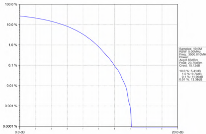
n78e_30kHz_SISO_NTNV_40MHz_CP-OFDM QPSK_3500.01MHz_Outer_Full
