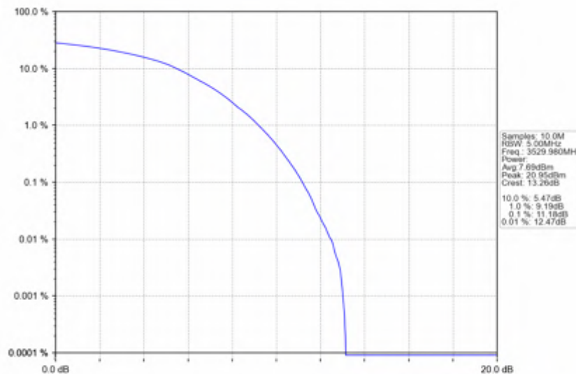
n78e_30kHz_SISO_NTNV_40MHz_DFT-s-OFDM_256_QAM_3529.98MHz_Outer_Full
