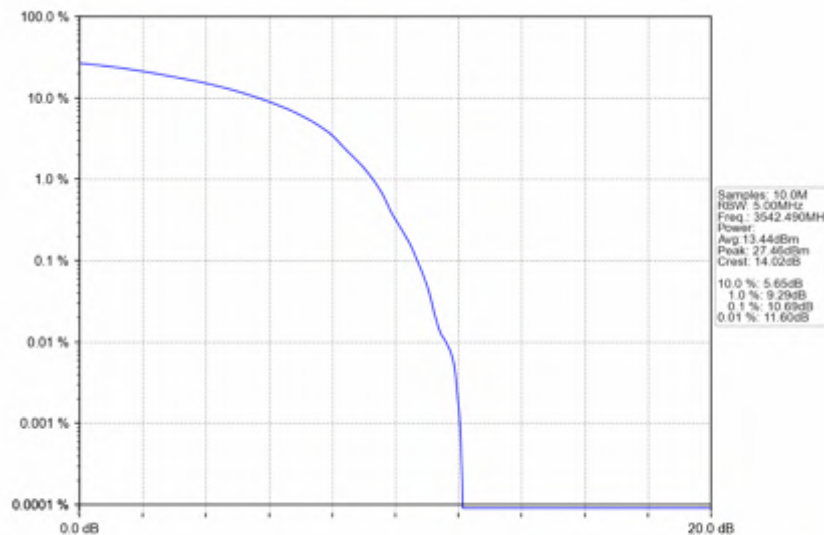
n78e_30kHz_SISO_NTNV_15MHz_DFT-s-OFDM 16 QAM_3542.49MHz_Outer_Full
