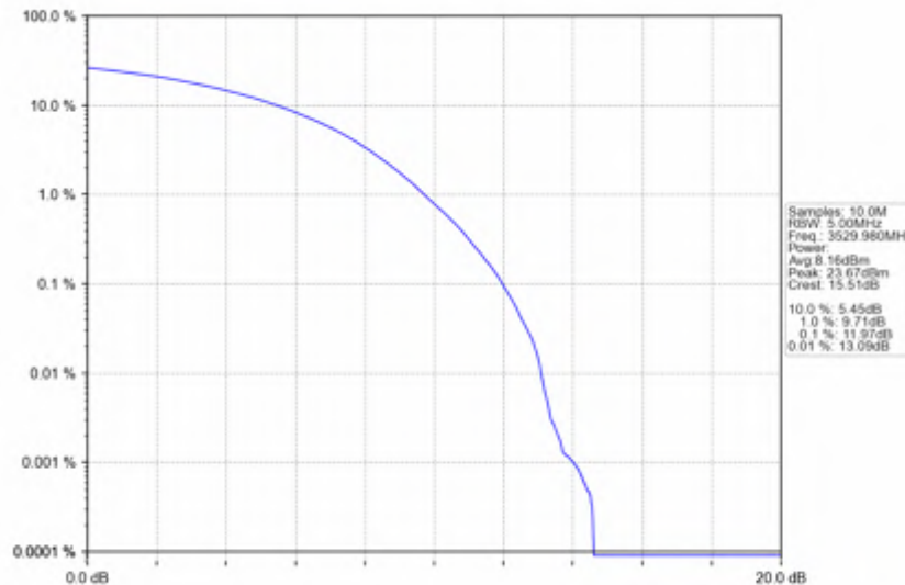
n78e_30kHz_SISO_NTNV_40MHz_CP-OFDM 64 QAM_3529.98MHz_Outer_Full
