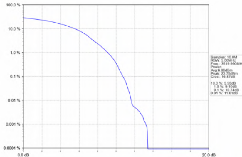
n78e_30kHz_SISO_NTNV_60MHz_DFT-s-OFDM PI/2 BPSK_3519.99MHz_Outer_Full
