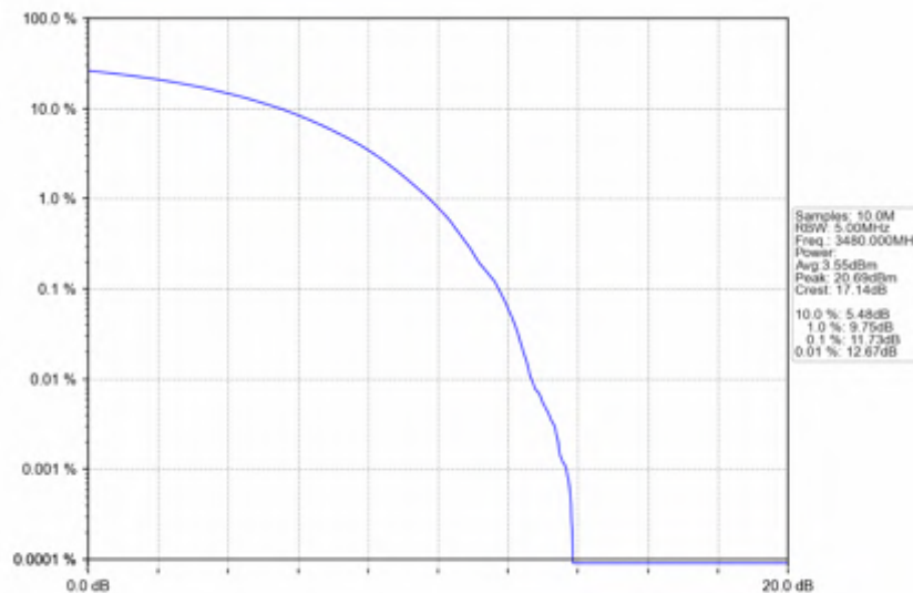
n78e_30kHz_SISO_NTNV_60MHz_CP-OFDM_256_QAM_3480MHz_Outer_Full
