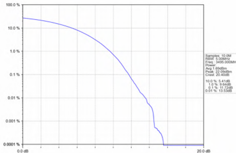
n78e_30kHz_SISO_NTNV_90MHz_CP-OFDM_256_QAM_3495MHz_Outer_Full
