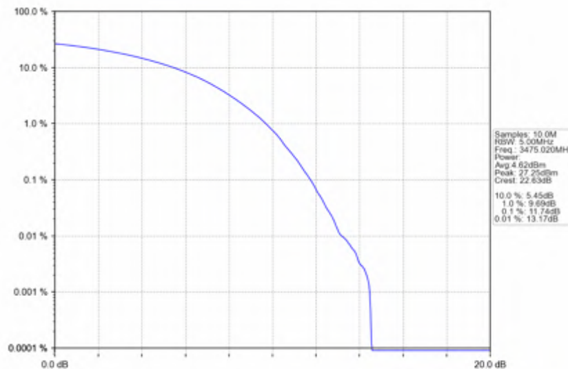
n78e_30kHz_SISO_NTNV_50MHz_CP-OFDM_256_QAM_3475.02MHz_Outer_Full
