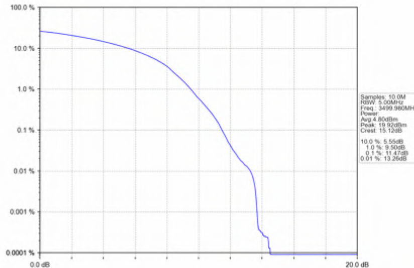
n78e_30kHz_SISO_NTNV_100MHz_DFT-s-OFDM 64 QAM_3499.98MHz_Outer_Full
