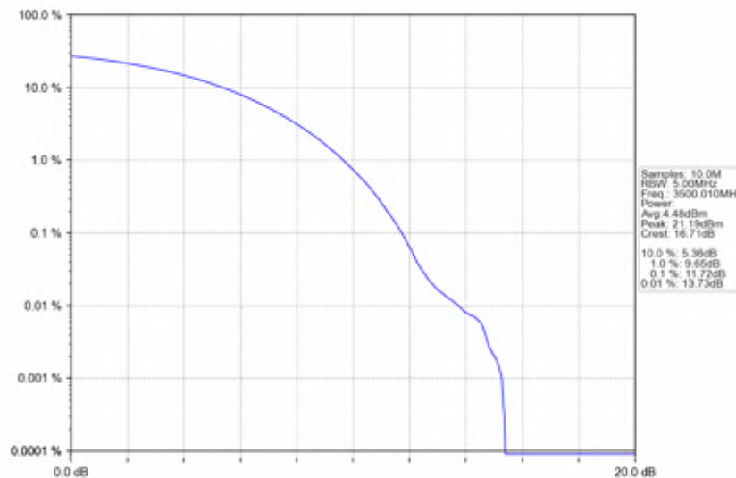
n78e_30kHz_SISO_NTNV_90MHz_CP-OFDM 64 QAM_3500.01MHz_Outer_Full
