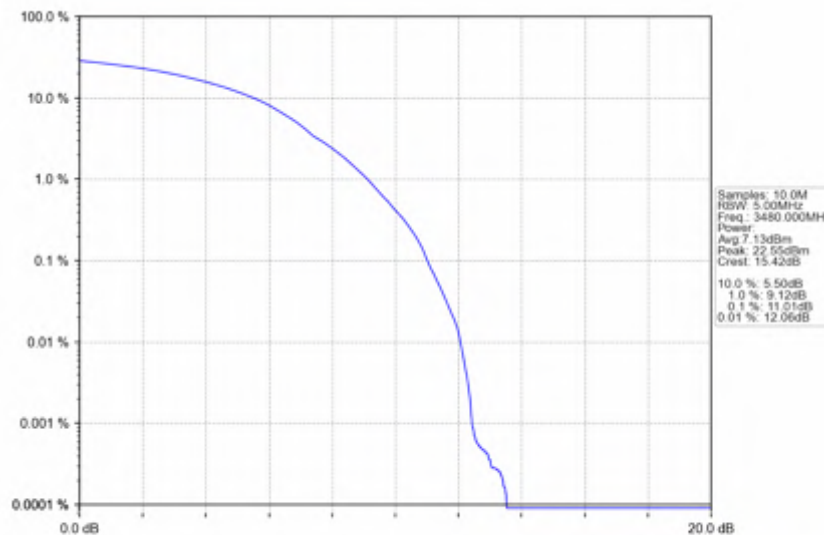
n78e_30kHz_SISO_NTNV_60MHz_DFT-s-OFDM QPSK_3480MHz_Outer_Full
