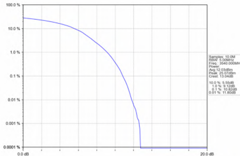
n78e_30kHz_SISO_NTNV_20MHz_DFT-s-OFDM 64 QAM_3540MHz_Outer_Full
