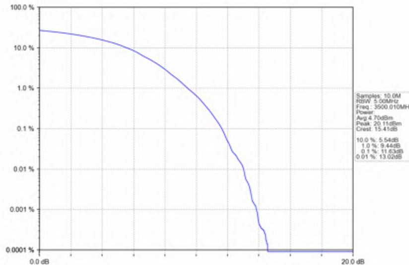
n78e_30kHz_SISO_NTNV_70MHz_DFT-s-OFDM_256_QAM_3500.01MHz_Outer_Full
