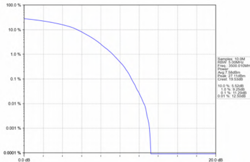
n78e_30kHz_SISO_NTNV_40MHz_DFT-s-OFDM_256_QAM_3500.01MHz_Outer_Full
