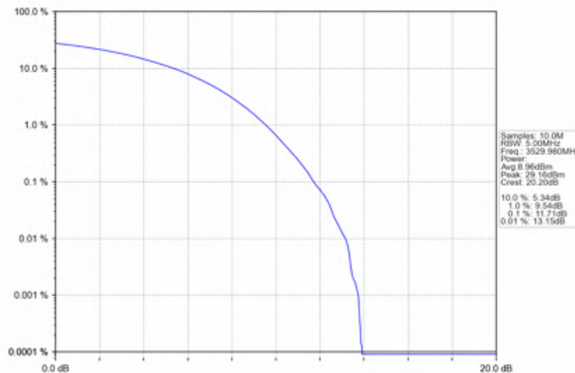
n78e_30kHz_SISO_NTNV_40MHz_CP-OFDM QPSK_3529.98MHz_Outer_Full
