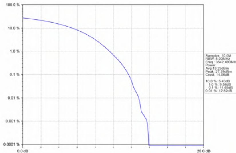
n78e_30kHz_SISO_NTNV_15MHz_CP-OFDM_QPSK_3542.49MHz_Outer_Full
