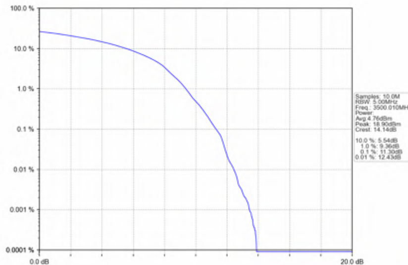
n78e_30kHz_SISO_NTNV_100MHz_DFT-s-OFDM_QPSK_3500.01MHz_Outer_Full
