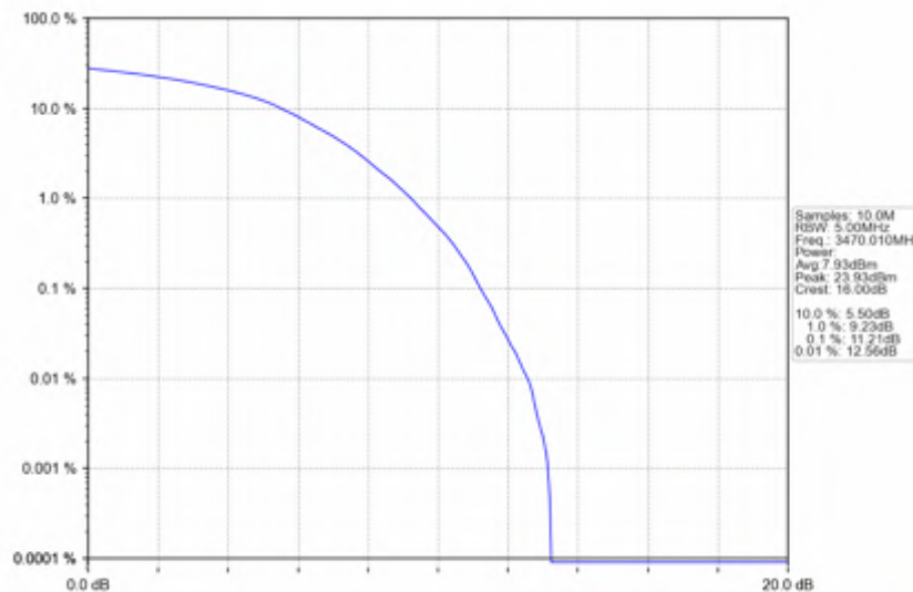
n78e_30kHz_SISO_NTNV_40MHz_DFT-s-OFDM_256_QAM_3470.01MHz_Outer_Full
