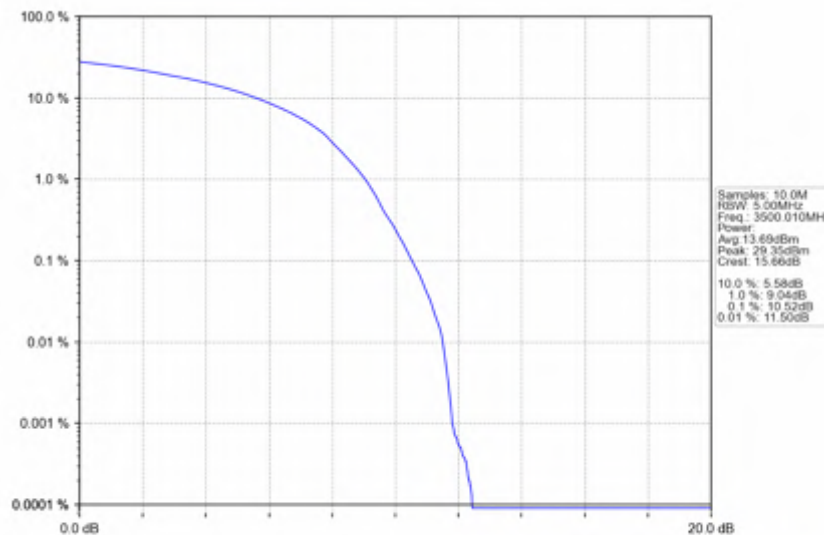
n78e_30kHz_SISO_NTV_15MHz_DFT-s-OFDM 64 QAM_3500.01MHz_Outer_Full
