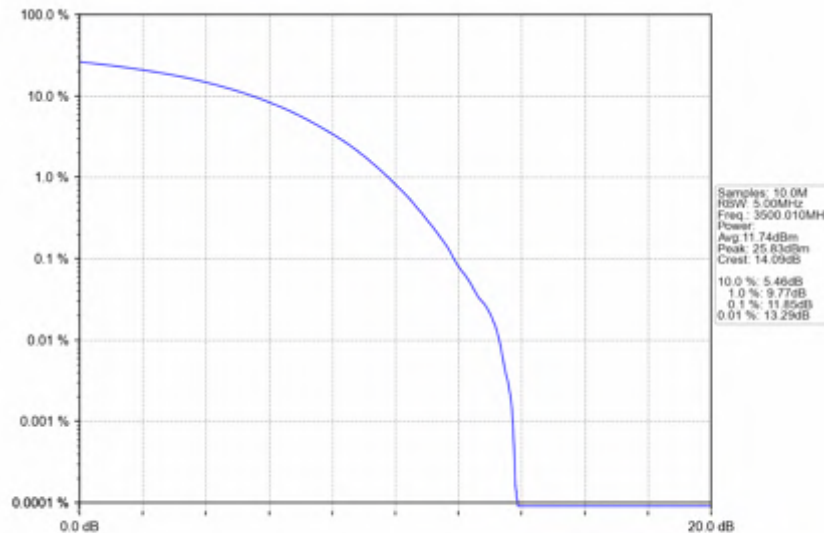
n78e_30kHz_SISO_NTNV_10MHz_CP-OFDM_256_QAM_3500.01MHz_Outer_Full
