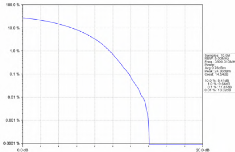
n78e_30kHz_SISO_NTNV_15MHz_CP-OFDM_256_QAM_3500.01MHz_Outer_Full
