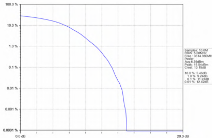
n78e_30kHz_SISO_NTNV_70MHz_DFT-s-OFDM_QPSK_3514.98MHz_Outer_Full
