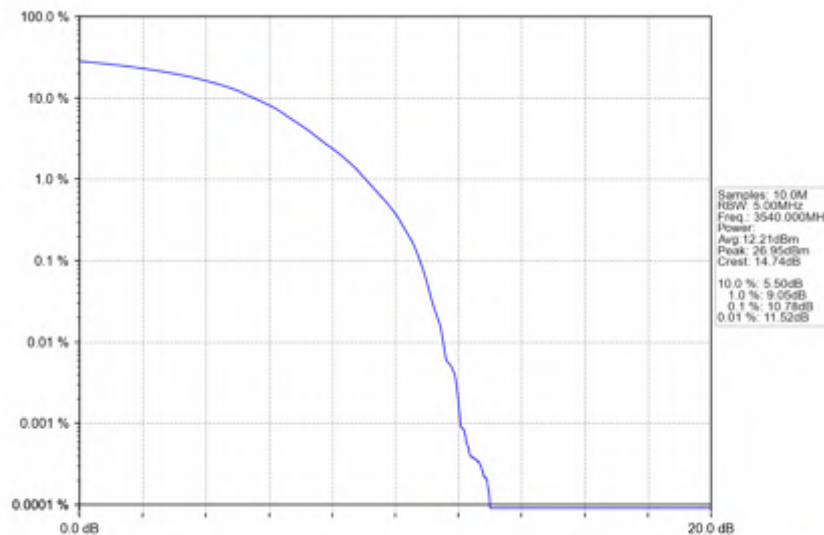
n78e_30kHz_SISO_NTNV_20MHz_DFT-s-OFDM 16 QAM_3540MHz_Outer_Full
