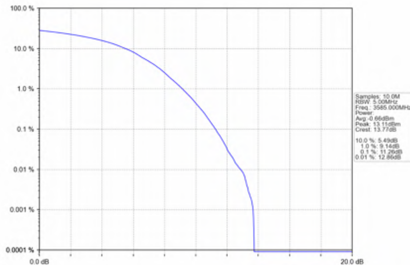
n78d_30kHz_SISO_NTNV_70MHz_DFT-s-OFDM QPSK_3585MHz_Outer_Full
