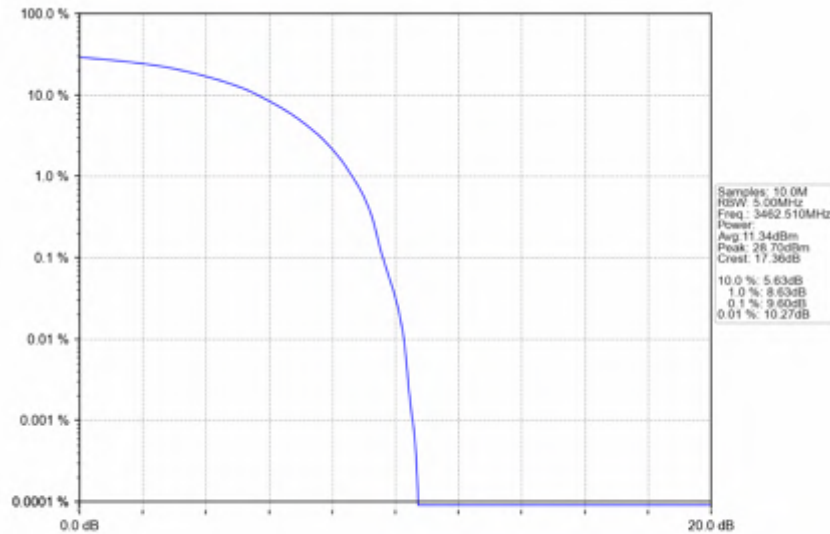
n78e 15kHz SISO NTNV 25MHz DFT-s-OFDM PI/2 BPSK 3462.51MHz Outer Full
