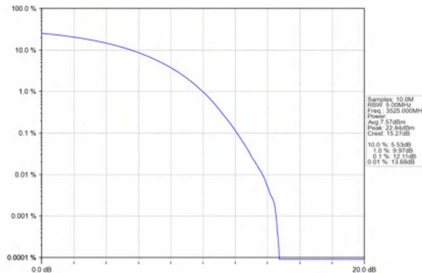
n78e_15kHz_SISO_NTNV_50MHz_CP-OFDM 16 QAM_3525MHz_Outer_Full
