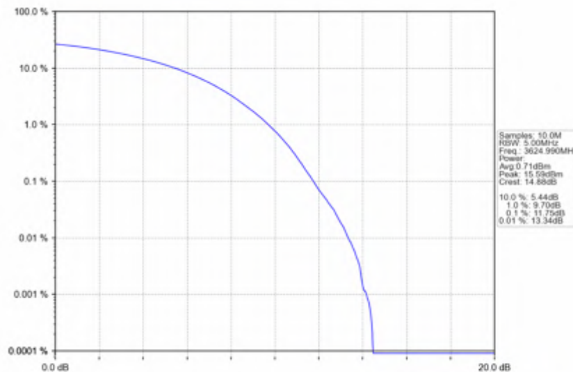
n78d_30kHz_SISO_NTNV_60MHz_CP-OFDM_256_QAM_3624.99MHz_Outer_Full
