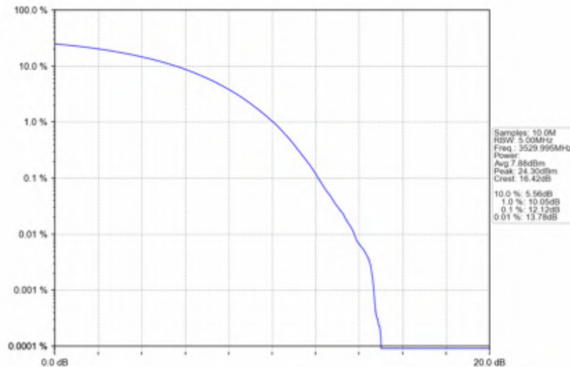
n78e_15kHz_SISO_NTNV_40MHz_CP-OFDM_64_QAM_3529.995MHz_Outer_Full
