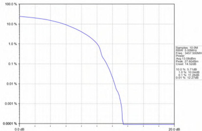
n78e_15kHz_SISO_NTNV_15MHz_DFT-s-OFDM 64 QAM_3457.5MHz_Outer_Full
