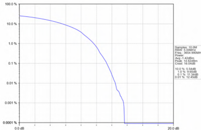
n78d_30kHz_SISO_NTNV_90MHz_DFT-s-OFDM_QPSK_3654.99MHz_Outer_Full
