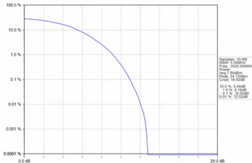
n78e_15kHz_SISO_NTNV_50MHz_DFT-s-OFDM PI/2 BPSK_3525MHz_Outer_Full
