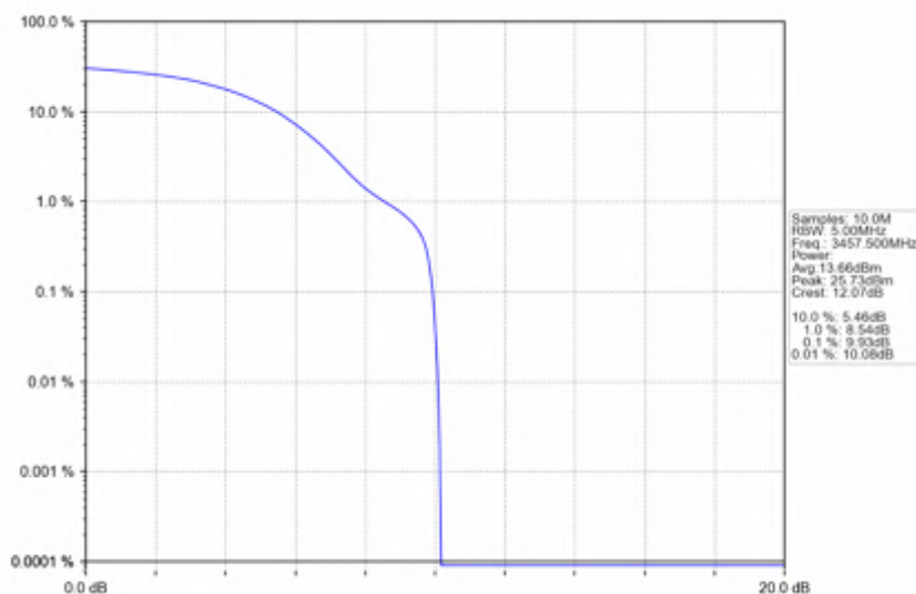
n78e 15kHz SISO NTNV 15MHz DFT-s-OFDM PI/2 BPSK 3457.5MHz Outer Full
