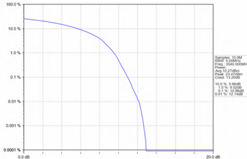
n78e_15kHz_SISO_NTNV_20MHz_DFT-s-OFDM_256_QAM_3540MHz_Outer_Full
