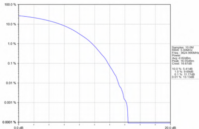
n78d_30kHz_SISO_NTNV_80MHz_CP-OFDM_16_QAM_3624.99MHz_Outer_Full
