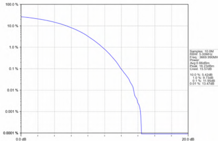
n78d_30kHz_SISO_NTNV_60MHz_CP-OFDM_QPSK_3669.99MHz_Outer_Full
