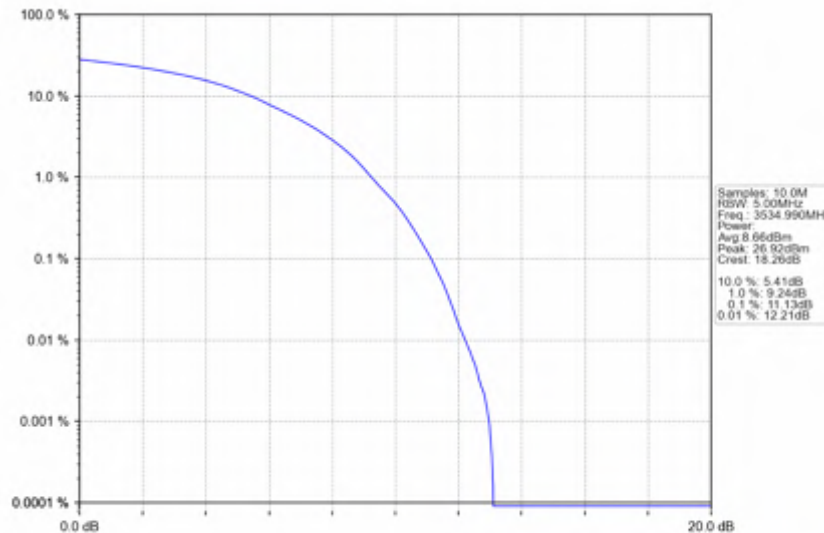
n78e_15kHz_SISO_NTNV_30MHz_DFT-s-OFDM_256_QAM_3534.99MHz_Outer_Full
