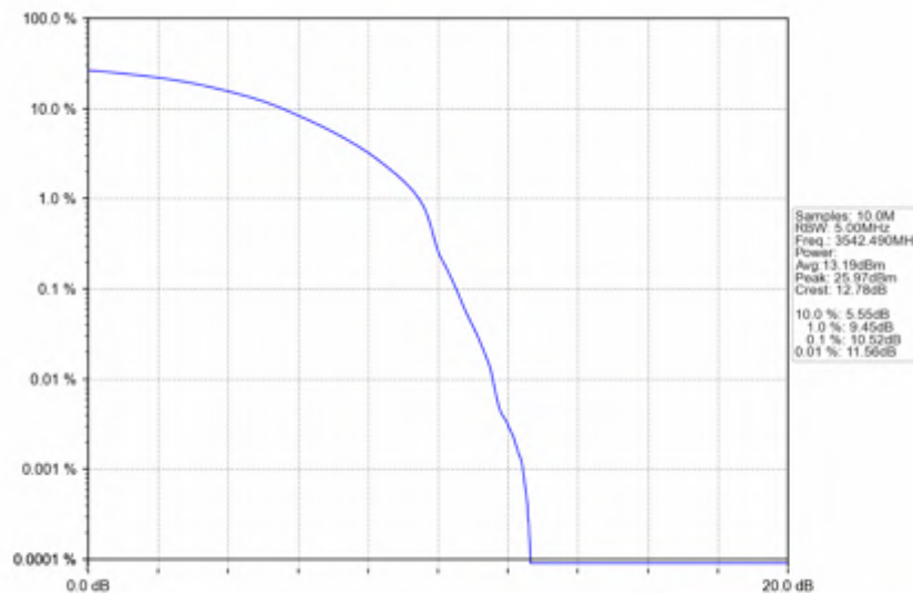
n78e_15kHz_SISO_NTNV_15MHz_DFT-s-OFDM 16 QAM_3542.49MHz_Outer_Full
