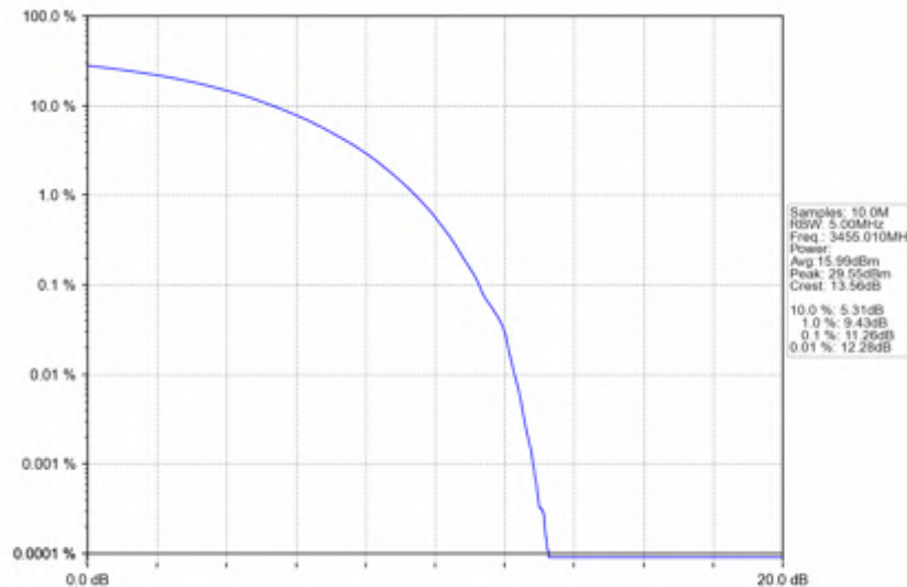
n78e_30kHz_SISO_NTNV_10MHz_CP-OFDM_QPSK_3455.01MHz_Outer_Full
