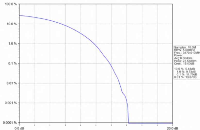
n78e_15kHz_SISO_NTNV_40MHz_CP-OFDM 64 QAM_3470.01MHz_Outer_Full
