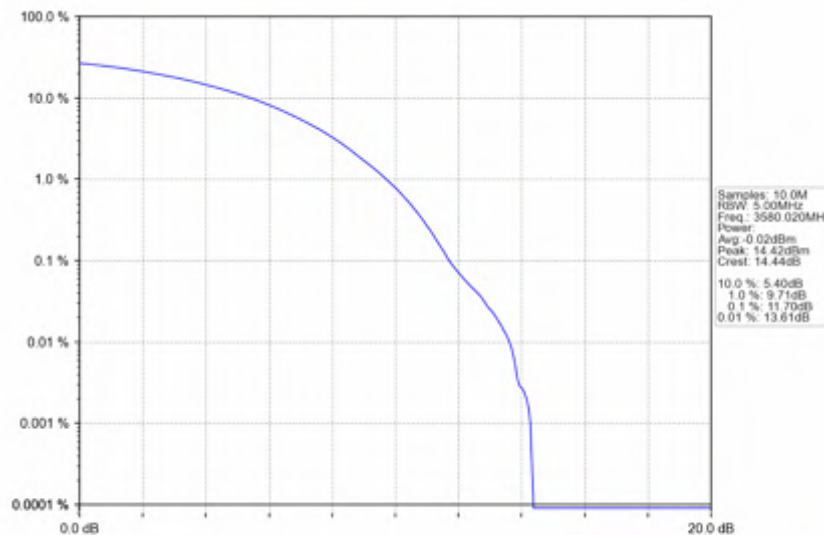
n78d_30kHz_SISO_NTNV_60MHz_CP-OFDM_256_QAM_3580.02MHz_Outer_Full
