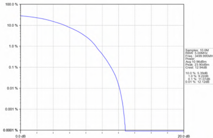
n78e_15kHz_SISO_NTNV_25MHz_DFT-s-OFDM 64 QAM_3499.995MHz_Outer_Full
