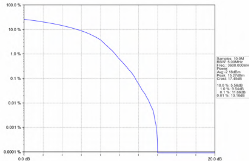
n78d_30kHz_SISO_NTNV_100MHz_DFT-s-OFDM 64 QAM_3600MHz_Outer_Full
