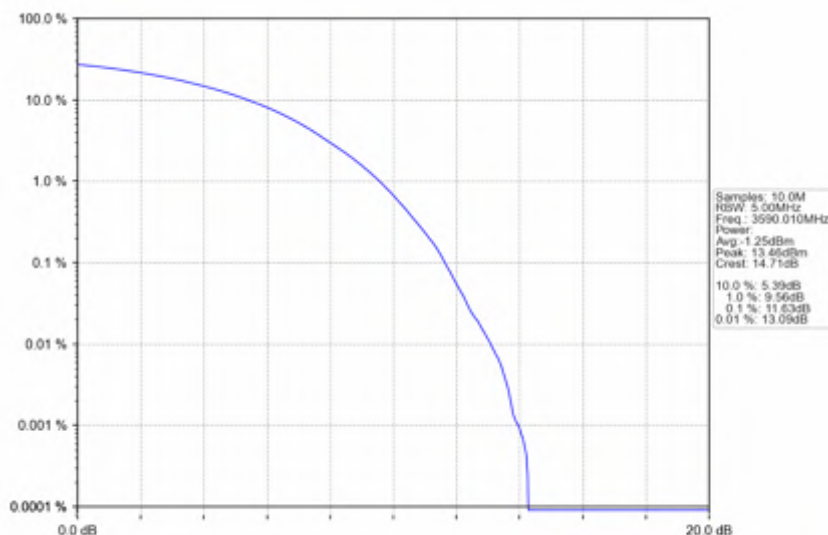
n78d_30kHz_SISO_NTNV_80MHz_CP-OFDM_16_QAM_3590.01MHz_Outer_Full
