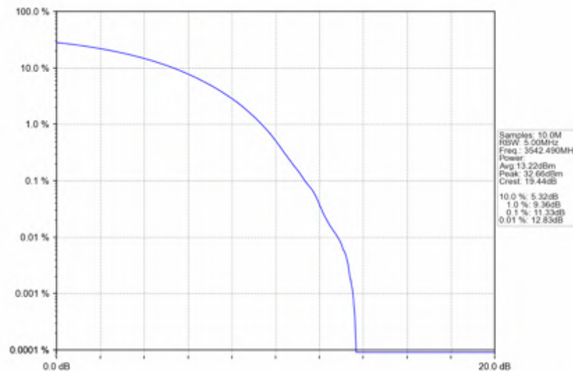
n78e_15kHz_SISO_NTNV_15MHz_CP-OFDM QPSK_3542.49MHz_Outer_Full
