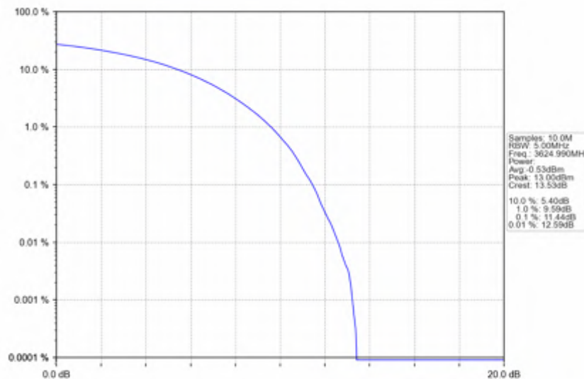
n78d_30kHz_SISO_NTNV_80MHz_CP-OFDM_256_QAM_3624.99MHz_Outer_Full
