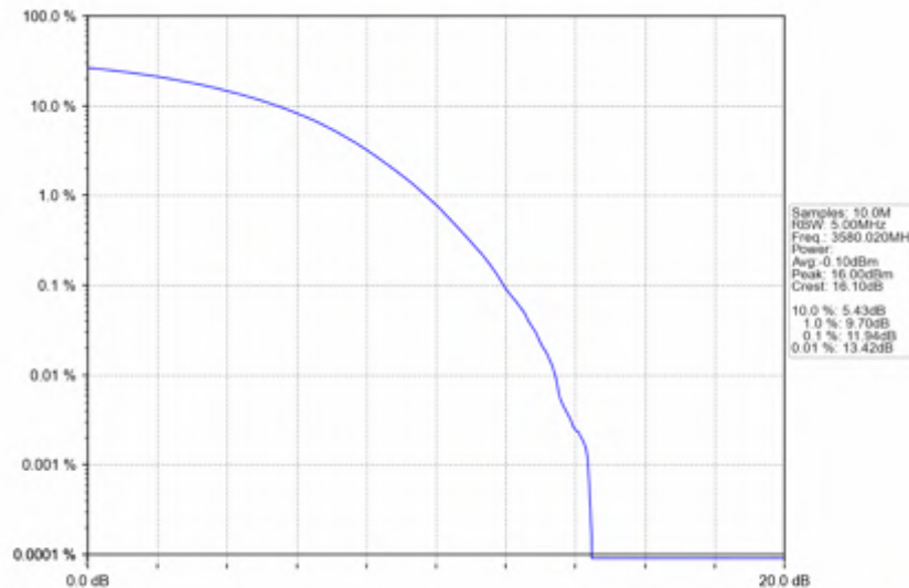
n78d_30kHz_SISO_NTNV_60MHz_CP-OFDM_QPSK_3580.02MHz_Outer_Full
