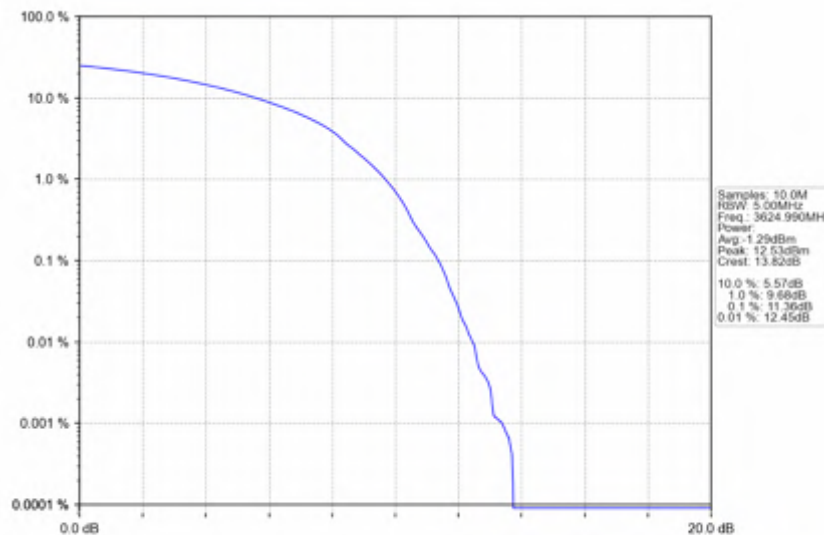
n78d_30kHz_SISO_NTNV_90MHz_DFT-s-OFDM_QPSK_3624.99MHz_Outer_Full
