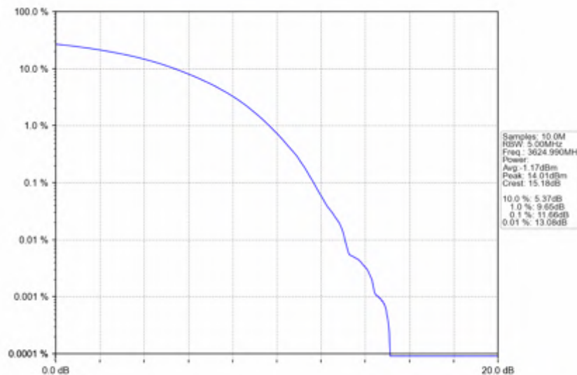
n78d_30kHz_SISO_NTNV_90MHz_CP-OFDM QPSK_3624.99MHz_Outer_Full
