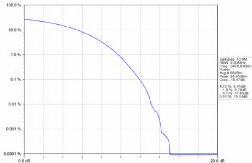
n78e_15kHz_SISO_NTNV_40MHz_CP-OFDM_16_QAM_3470.01MHz_Outer_Full
