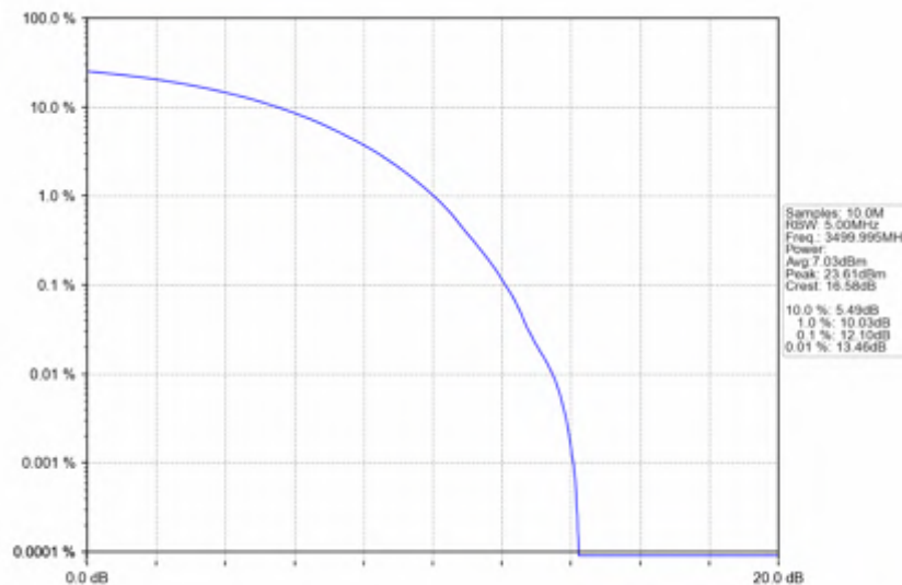
n78e_15kHz_SISO_NTNV_50MHz_CP-OFDM 64 QAM_3499.995MHz_Outer_Full
