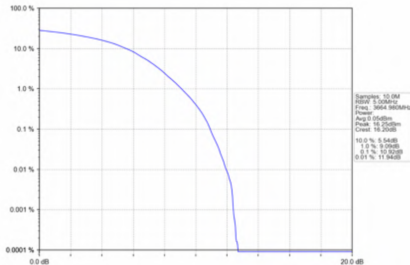
n78d_30kHz_SISO_NTNV_70MHz_DFT-s-OFDM PI/2 BPSK_3664.98MHz_Outer_Full
