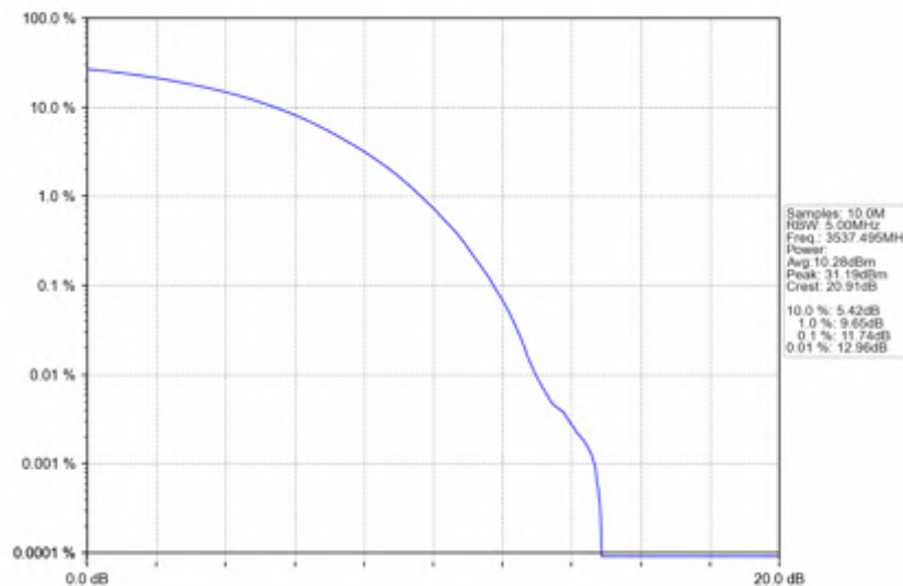
n78e_15kHz_SISO_NTNV_25MHz_CP-OFDM_64_QAM_3537.495MHz_Outer_Full
