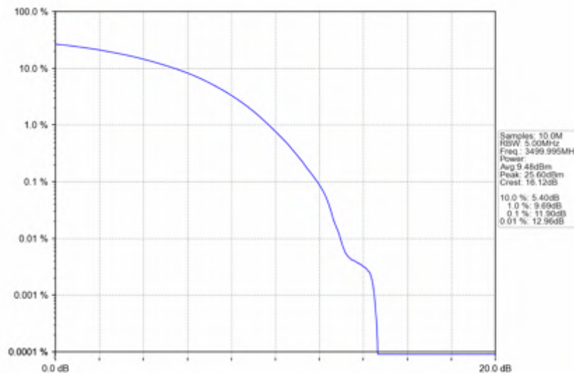
n78e_15kHz_SISO_NTNV_30MHz_CP-OFDM 64 QAM_3499.995MHz_Outer_Full
