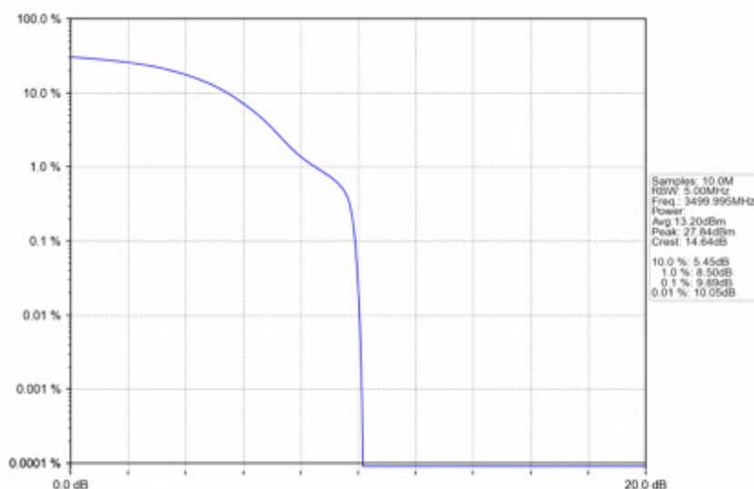
n78e 15kHz SISO NTNV 15MHz DFT-s-OFDM PI/2 BPSK 3499.995MHz Outer Full
