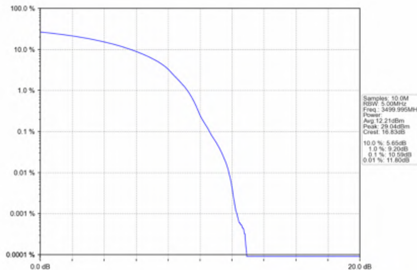
n78e_15kHz_SISO_NTNV_20MHz_DFT-s-OFDM_16_QAM_3499.995MHz_Outer_Full
