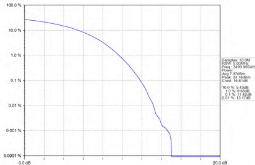
n78e_15kHz_SISO_NTNV_25MHz_CP-OFDM_256_QAM_3499.995MHz_Outer_Full
