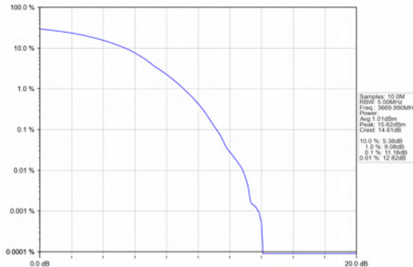
n78d_30kHz_SISO_NTNV_60MHz_DFT-s-OFDM_256_QAM_3669.99MHz_Outer_Full
