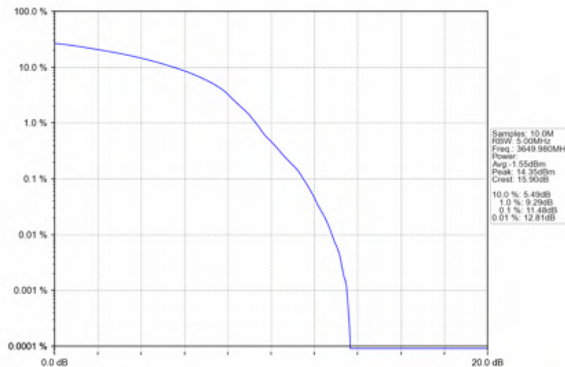
n78d_30kHz_SISO_NTNV_100MHz_DFT-s-OFDM 16 QAM_3649.98MHz_Outer_Full
