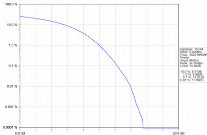
n78e_15kHz_SISO_NTNV_40MHz_CP-OFDM 16 QAM_3529.995MHz_Outer_Full
