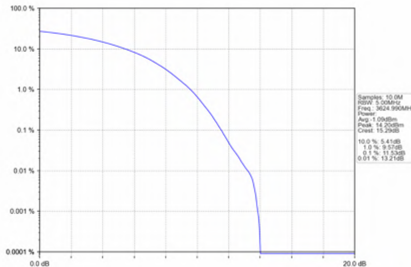
n78d_30kHz_SISO_NTNV_90MHz_CP-OFDM_16_QAM_3624.99MHz_Outer_Full
