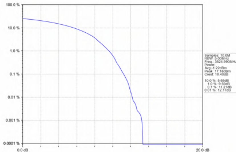
n78d_30kHz_SISO_NTNV_90MHz_DFT-s-OFDM PI/2 BPSK_3624.99MHz_Outer_Full
