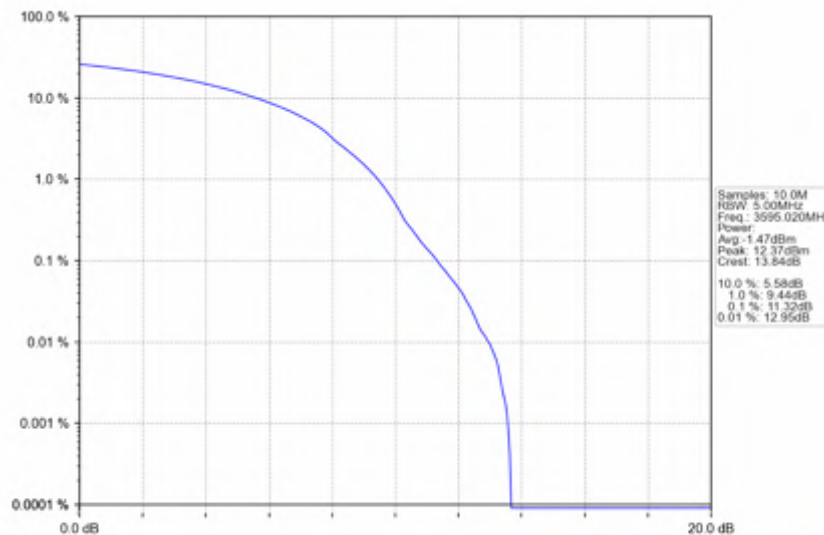
n78d_30kHz_SISO_NTNV_90MHz_DFT-s-OFDM_256_QAM_3595.02MHz_Outer_Full
