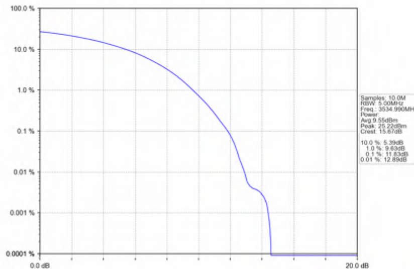
n78e_15kHz_SISO_NTNV_30MHz_CP-OFDM 64 QAM_3534.99MHz_Outer_Full
