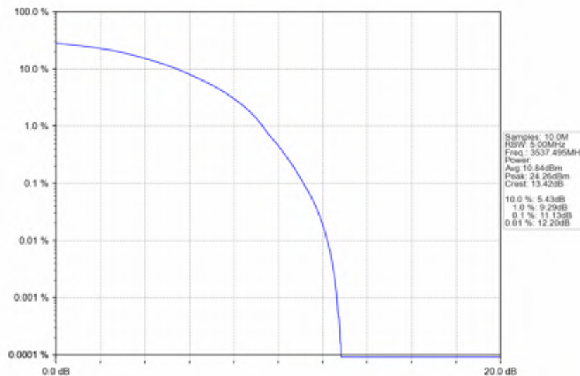
n78e_15kHz_SISO_NTNV_25MHz_DFT-s-OFDM 64 QAM_3537.495MHz_Outer_Full
