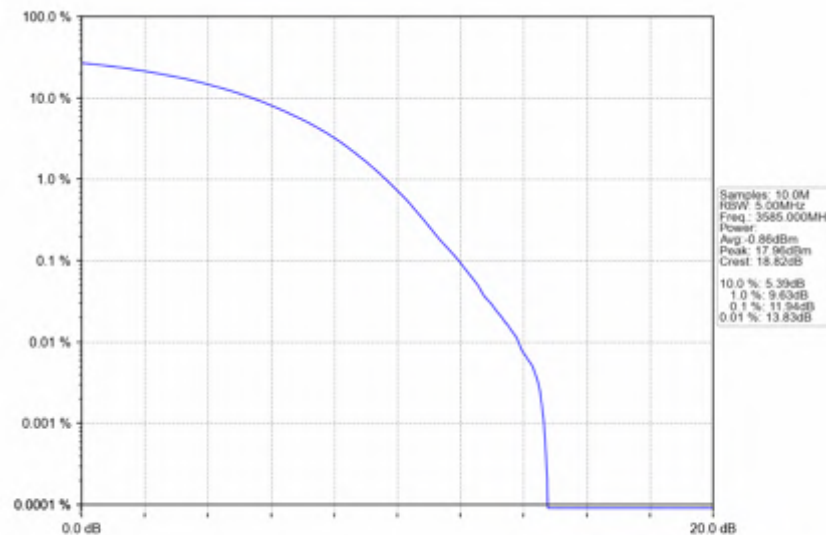
n78d_30kHz_SISO_NTNV_70MHz_CP-OFDM 64 QAM_3585MHz_Outer_Full
