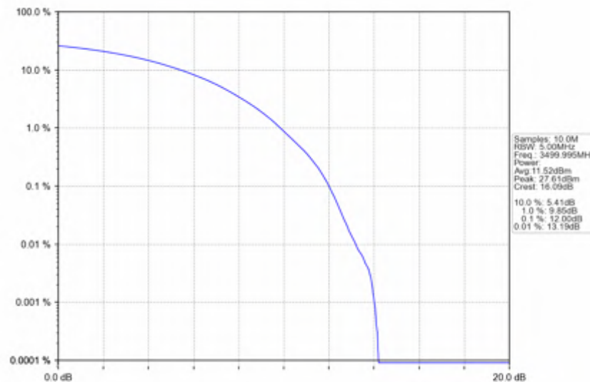
n78e_15kHz_SISO_NTNV_20MHz_CP-OFDM QPSK_3499.995MHz_Outer_Full
