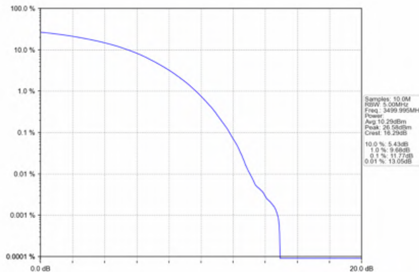
n78e_15kHz_SISO_NTNV_25MHz_CP-OFDM_64_QAM_3499.995MHz_Outer_Full
