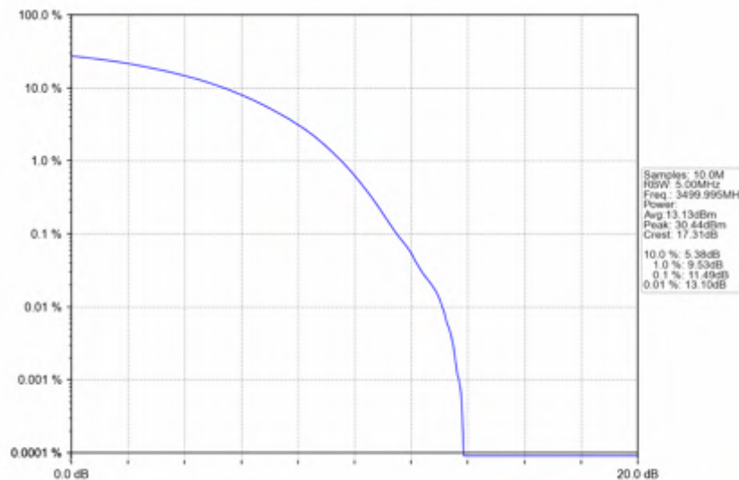
n78e 15kHz SISO NTV 15MHz CP-OFDM 16 QAM 3499.995MHz Outer Full
