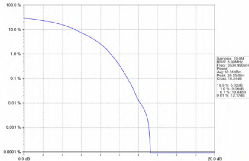
n78e_15kHz_SISO_NTNV_30MHz_DFT-s-OFDM 64 QAM_3534.99MHz_Outer_Full
