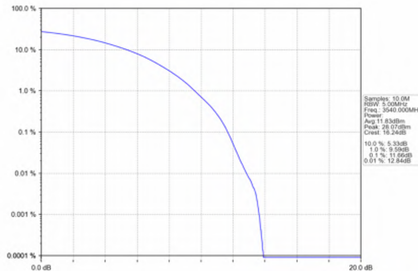
n78e_15kHz_SISO_NTNV_20MHz_CP-OFDM QPSK_3540MHz_Outer_Full
