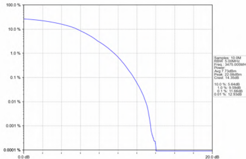
n78e_15kHz_SISO_NTNV_50MHz_DFT-s-OFDM QPSK_3475.005MHz_Outer_Full
