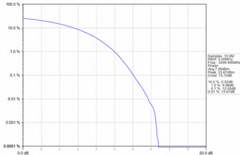
n78e_15kHz_SISO_NTNV_40MHz_CP-OFDM_64_QAM_3499.995MHz_Outer_Full
