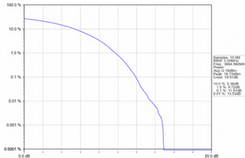
n78d_30kHz_SISO_NTNV_70MHz_CP-OFDM 16 QAM_3664.98MHz_Outer_Full
