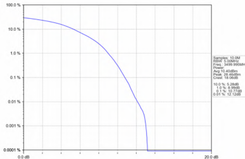
n78e_15kHz_SISO_NTNV_30MHz_DFT-s-OFDM 64 QAM_3499.995MHz_Outer_Full
