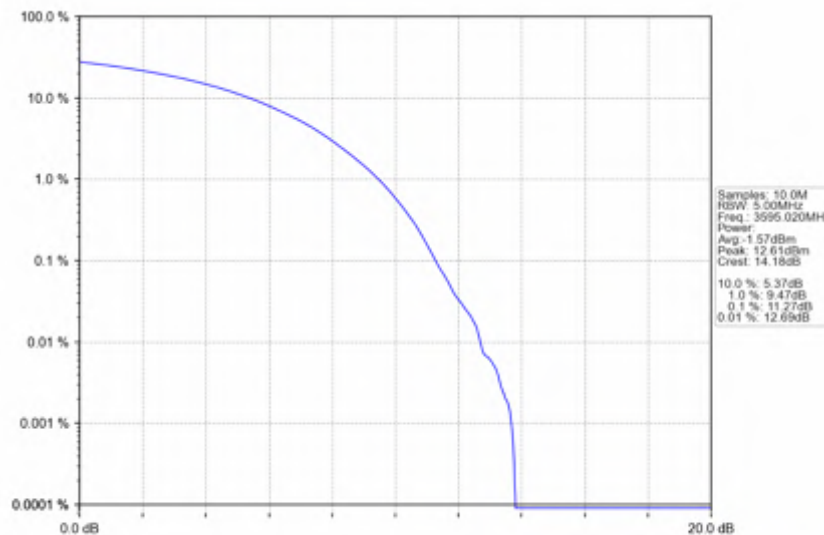
n78d_30kHz_SISO_NTNV_90MHz_CP-OFDM_16_QAM_3595.02MHz_Outer_Full
