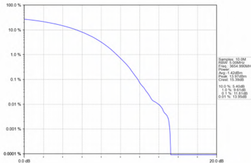
n78d_30kHz_SISO_NTNV_90MHz_CP-OFDM QPSK_3654.99MHz_Outer_Full
