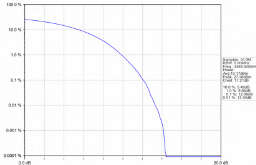
n78e_15kHz_SISO_NTNV_30MHz_CP-OFDM_QPSK_3465MHz_Outer_Full
