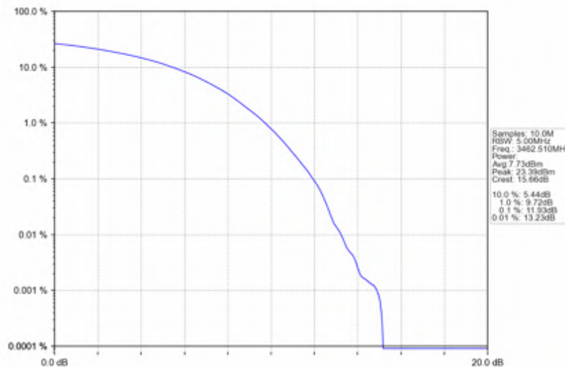
n78e_15kHz_SISO_NTNV_25MHz_CP-OFDM_256_QAM_3462.51MHz_Outer_Full
