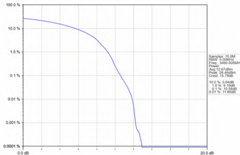
n78e_15kHz_SISO_NTNV_20MHz_DFT-s-OFDM_16_QAM_3460.005MHz_Outer_Full
