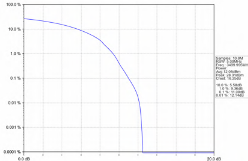
n78e_15kHz_SISO_NTNV_20MHz_DFT-s-OFDM 64 QAM_3499.995MHz_Outer_Full
