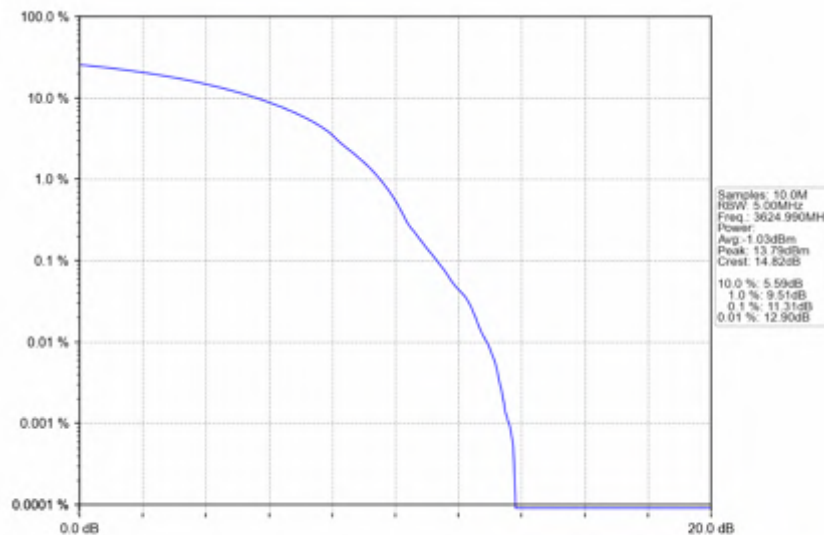
n78d_30kHz_SISO_NTNV_90MHz_DFT-s-OFDM_256_QAM_3624.99MHz_Outer_Full
