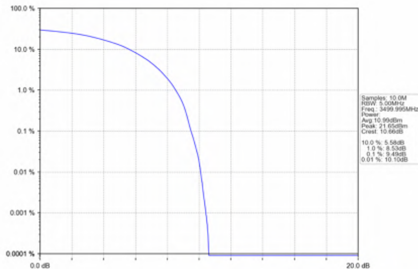
n78e_15kHz_SISO_NTNV_25MHz_DFT-s-OFDM_PI/2_BPSK_3499.995MHz_Outer_Full
