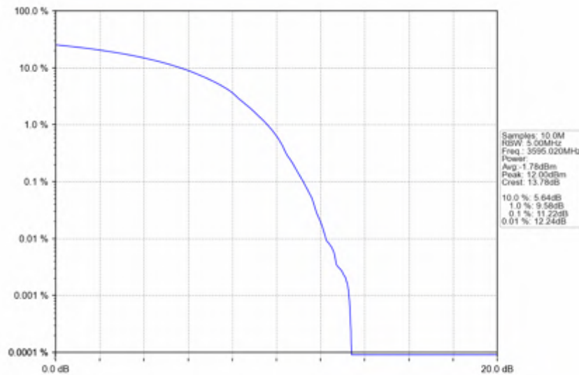
n78d_30kHz_SISO_NTNV_90MHz_DFT-s-OFDM PI/2 BPSK_3595.02MHz_Outer_Full
