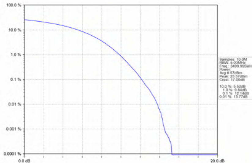
n78e_15kHz_SISO_NTNV_40MHz_CP-OFDM_16_QAM_3499.995MHz_Outer_Full
