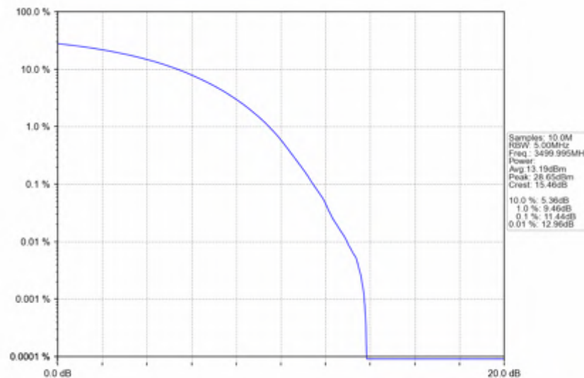
n78e_15kHz_SISO_NTNV_15MHz_CP-OFDM QPSK_3499.995MHz_Outer_Full
