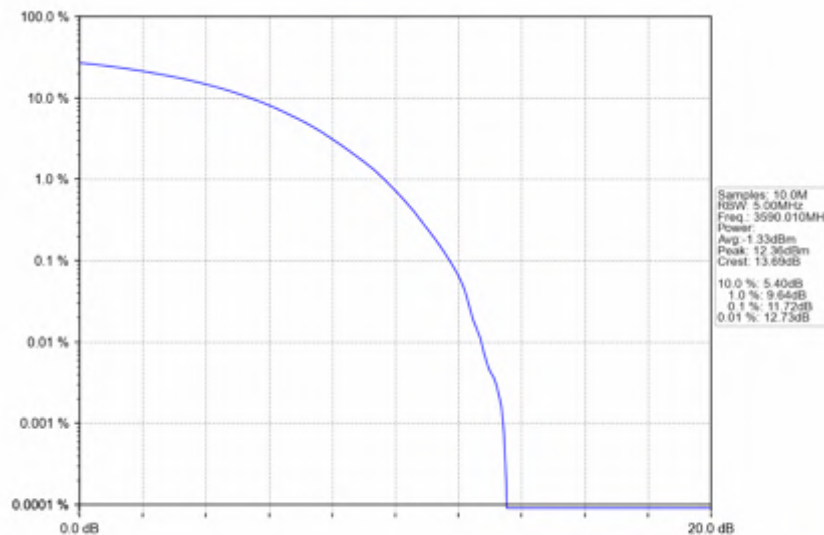
n78d_30kHz_SISO_NTNV_80MHz_CP-OFDM_256_QAM_3590.01MHz_Outer_Full
