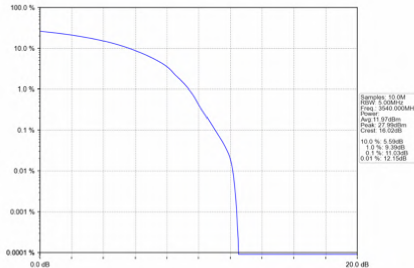
n78e_15kHz_SISO_NTNV_20MHz_DFT-s-OFDM 64 QAM_3540MHz_Outer_Full
