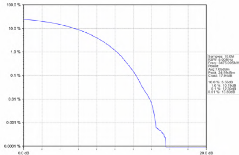
n78e_15kHz_SISO_NTNV_50MHz_CP-OFDM 64 QAM_3475.005MHz_Outer_Full
