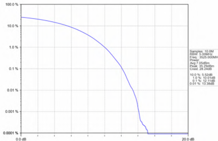
n78e_15kHz_SISO_NTNV_50MHz_CP-OFDM 64 QAM_3525MHz_Outer_Full
