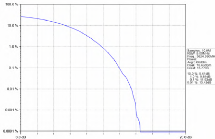
n78d_30kHz_SISO_NTNV_60MHz_CP-OFDM_QPSK_3624.99MHz_Outer_Full
