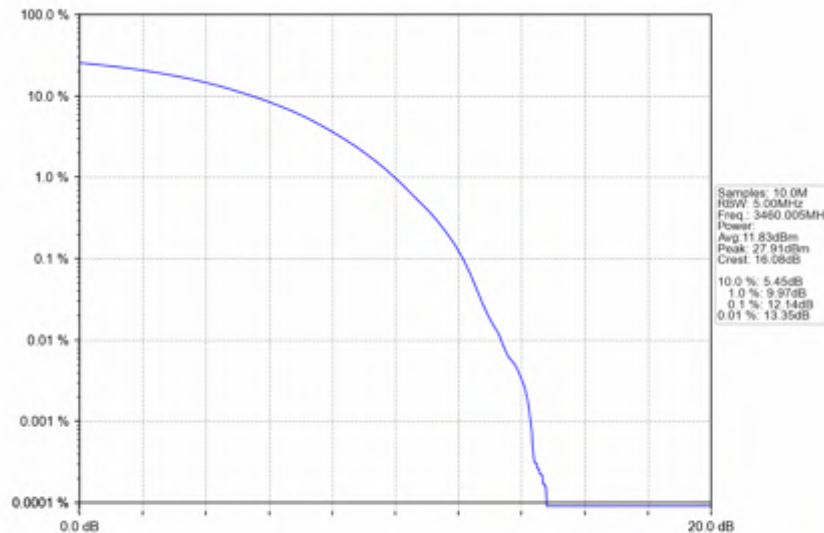
n78e_15kHz_SISO_NTNV_20MHz_CP-OFDM_QPSK_3460.005MHz_Outer_Full
