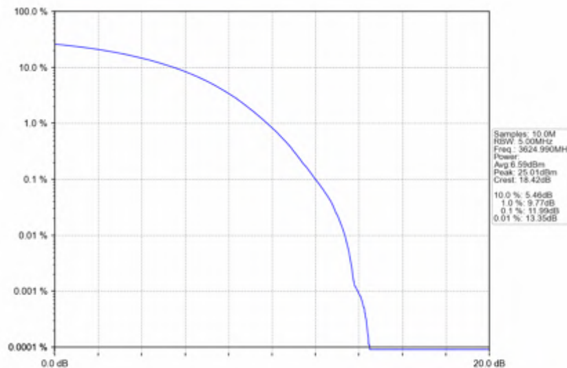
n78d_30kHz_SISO_NTNV_15MHz_CP-OFDM_QPSK_3624.99MHz_Outer_Full
