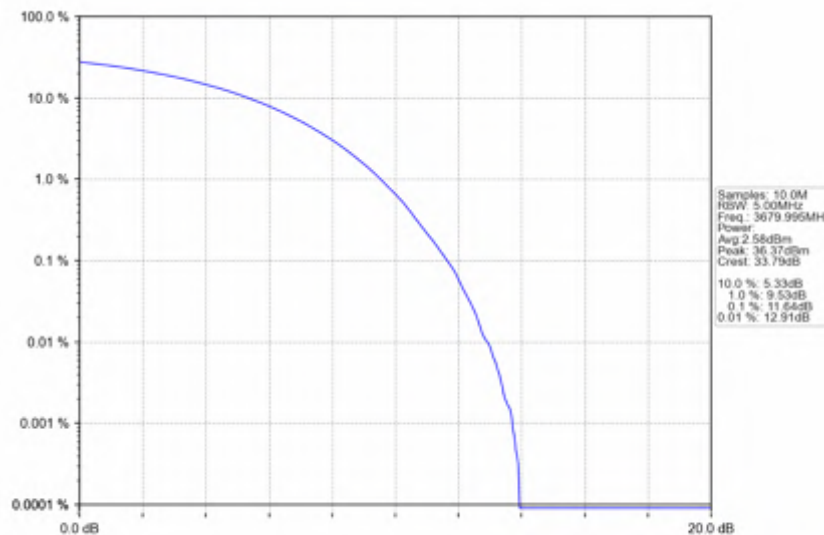
n78d_15kHz_SISO_NTNV_40MHz_CP-OFDM 64 QAM_3679.995MHz_Outer_Full
