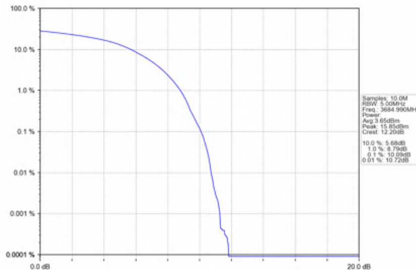
n78d_15kHz_SISO_NTNV_30MHz_DFT-s-OFDM PI/2 BPSK_3684.99MHz_Outer_Full
