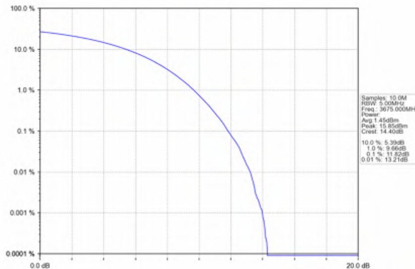
n78d_15kHz_SISO_NTNV_50MHz_CP-OFDM 64 QAM_3675MHz_Outer_Full
