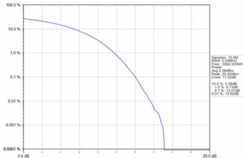
n78d_15kHz_SISO_NTNV_25MHz_CP-OFDM 64 QAM_3562.5MHz_Outer_Full
