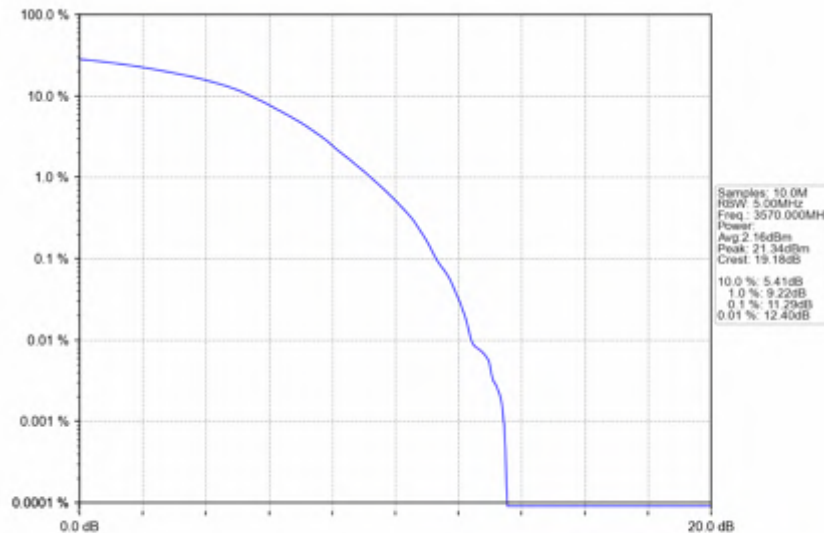
n78d_30kHz_SISO_NTNV_40MHz_DFT-s-OFDM_256_QAM_3570MHz_Outer_Full
