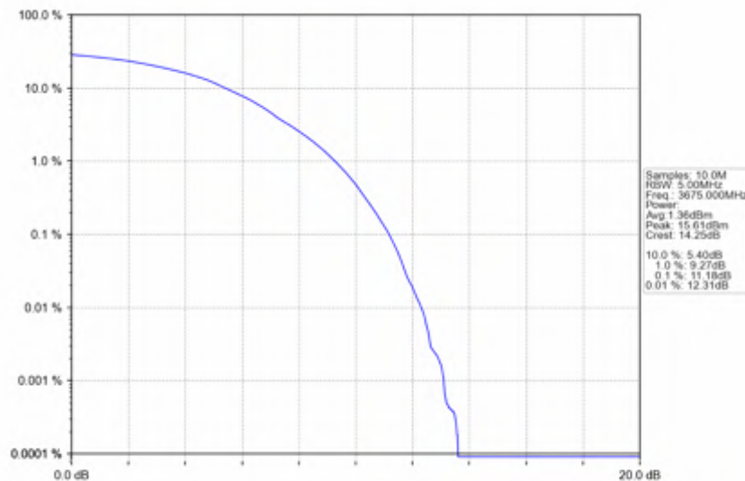
n78d_15kHz_SISO_NTNV_50MHz_DFT-s-OFDM QPSK_3675MHz_Outer_Full
