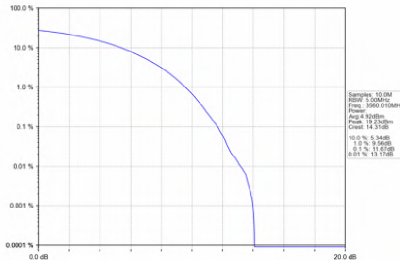
n78d_30kHz_SISO_NTNV_20MHz_CP-OFDM_QPSK_3560.01MHz_Outer_Full
