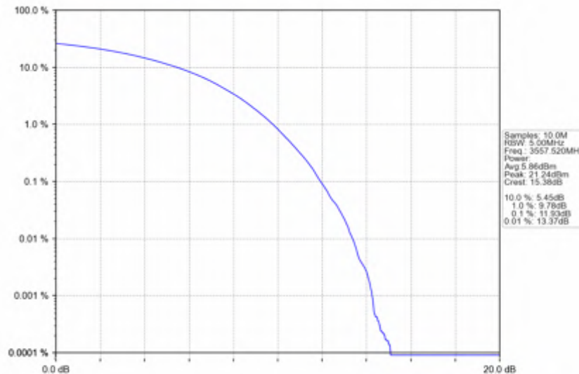
n78d_30kHz_SISO_NTNV_15MHz_CP-OFDM_256_QAM_3557.52MHz_Outer_Full
