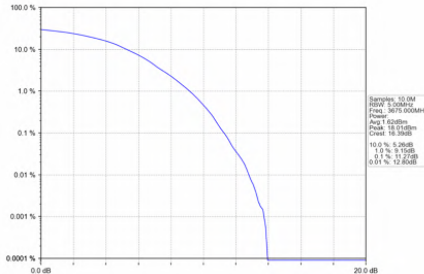
n78d_15kHz_SISO_NTNV_50MHz_DFT-s-OFDM 64 QAM_3675MHz_Outer_Full
