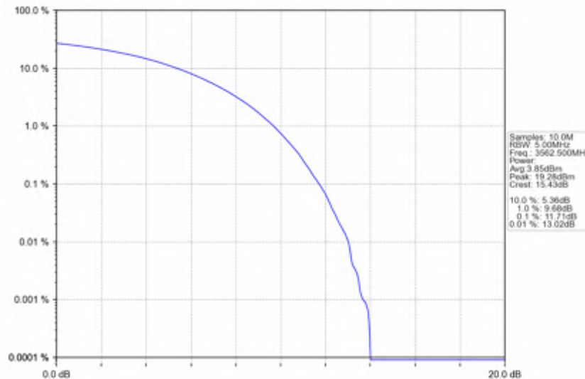
n78d_30kHz_SISO_NTNV_25MHz_CP-OFDM_QPSK_3562.5MHz_Outer_Full
