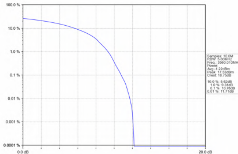
n78d_15kHz_SISO_NTV_20MHz_DFT-s-OFDM_16_QAM_3560.01MHz_Outer_Full
