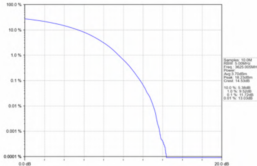
n78d_15kHz_SISO_NTNV_30MHz_CP-OFDM 64 QAM_3625.005MHz_Outer_Full
