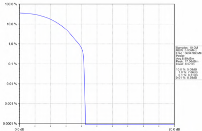
n78d_30kHz_SISO_NTNV_10MHz_DFT-s-OFDM PI/2 BPSK_3694.98MHz_Outer_Full
