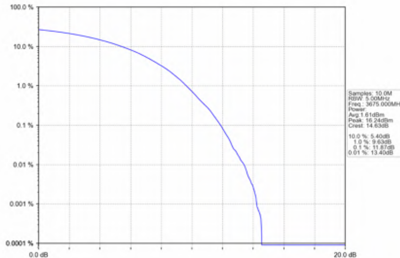
n78d_30kHz_SISO_NTNV_50MHz_CP-OFDM 64 QAM_3675MHz_Outer_Full
