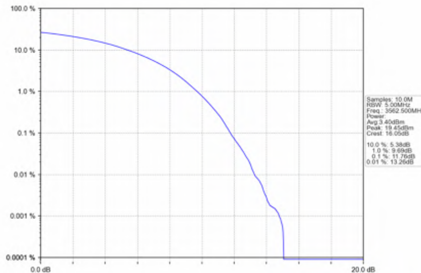
n78d_15kHz_SISO_NTNV_25MHz_CP-OFDM QPSK_3562.5MHz_Outer_Full
