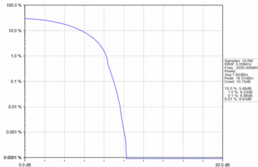
n78d_30kHz_SISO_NTNV_10MHz_DFT-s-OFDM QPSK_3555MHz_Outer_Full
