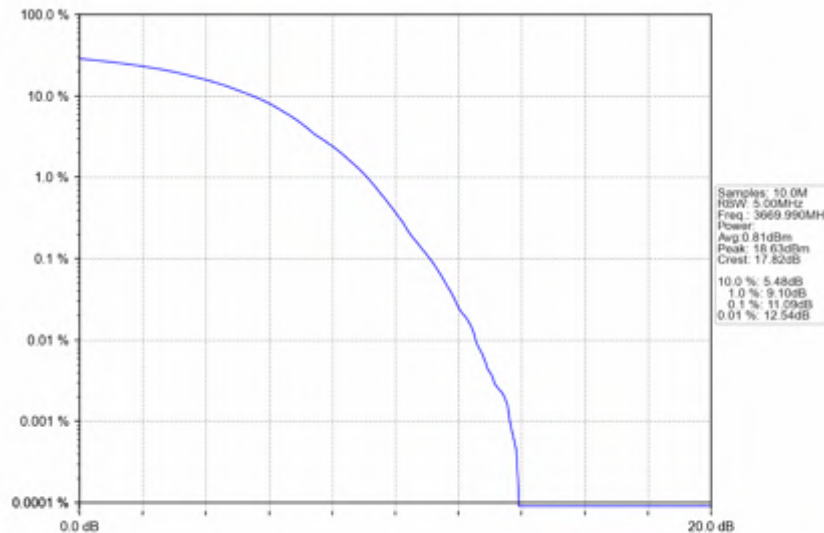
n78d_30kHz_SISO_NTV_60MHz_DFT-s-OFDM_64_QAM_3669.99MHz_Outer_Full
