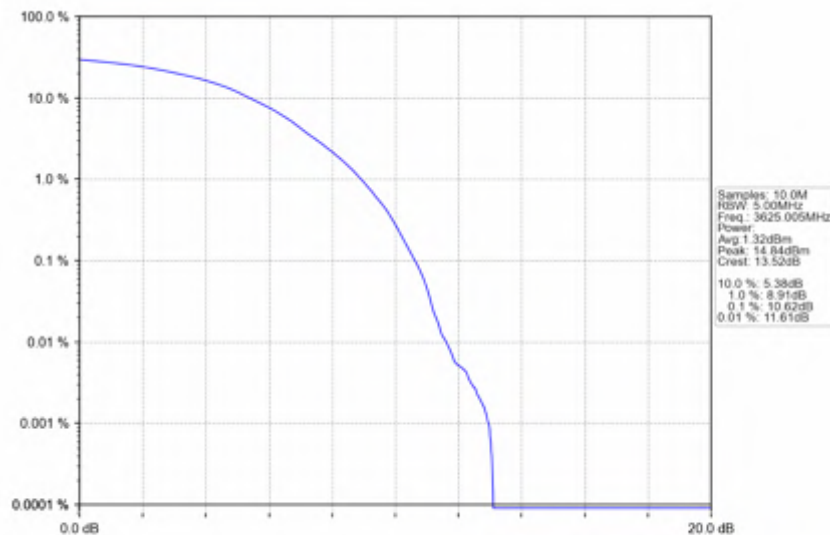
n78d_15kHz_SISO_NTNV_50MHz_DFT-s-OFDM_PI/2_BPSK_3625.005MHz_Outer_Full
