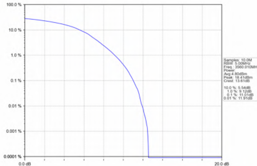
n78d_30kHz_SISO_NTV_20MHz_DFT-s-OFDM_16_QAM_3560.01MHz_Outer_Full
