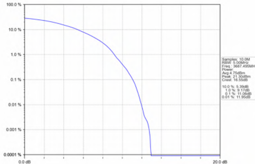
n78d_15kHz_SISO_NTNV_25MHz_DFT-s-OFDM 16 QAM_3687.495MHz_Outer_Full
