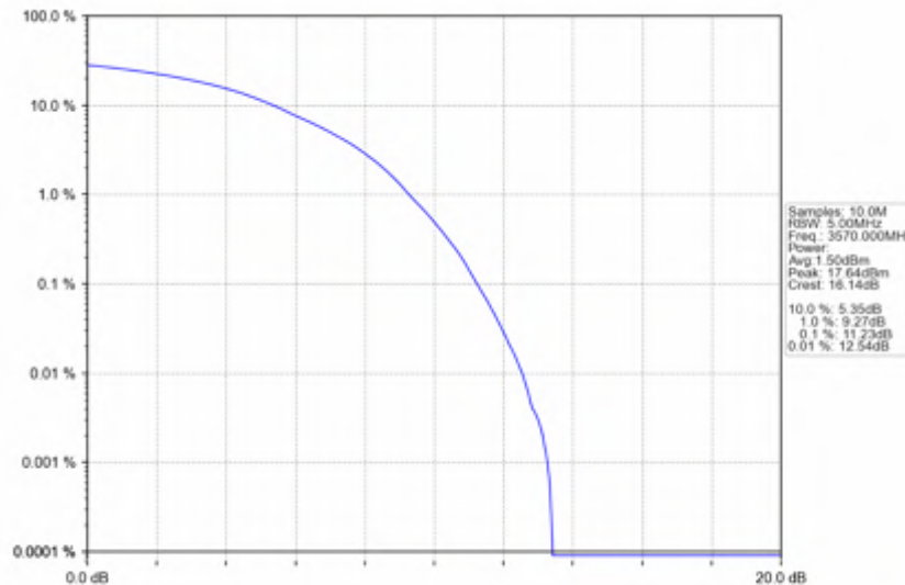
n78d_15kHz_SISO_NTNV_40MHz_DFT-s-OFDM_64_QAM_3570MHz_Outer_Full
