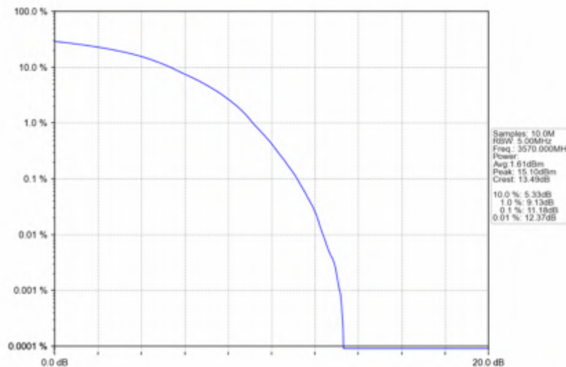
n78d_15kHz_SISO_NTNV_40MHz_DFT-s-OFDM_16_QAM_3570MHz_Outer_Full
