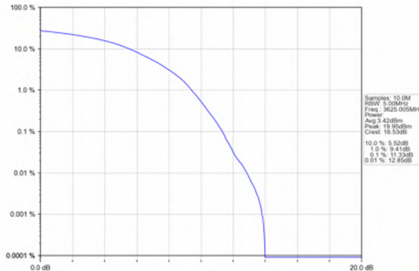
n78d_15kHz_SISO_NTNV_30MHz_DFT-s-OFDM 64 QAM_3625.005MHz_Outer_Full
