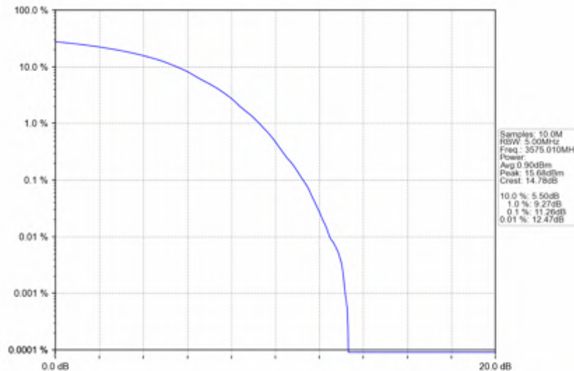
n78d_30kHz_SISO_NTNV_50MHz_DFT-s-OFDM_256_QAM_3575.01MHz_Outer_Full
