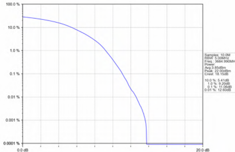
n78d_15kHz_SISO_NTNV_30MHz_DFT-s-OFDM 64 QAM_3684.99MHz_Outer_Full
