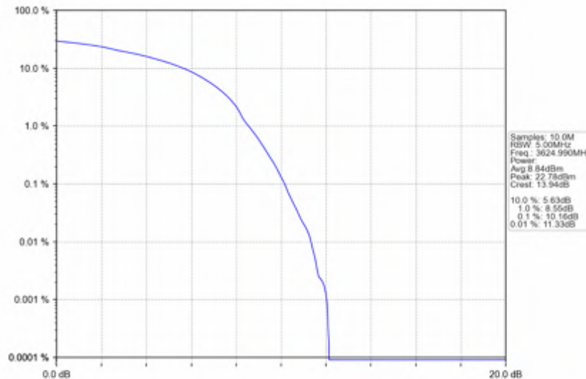
n78d_30kHz_SISO_NTNV_10MHz_DFT-s-OFDM_256_QAM_3624.99MHz_Outer_Full
