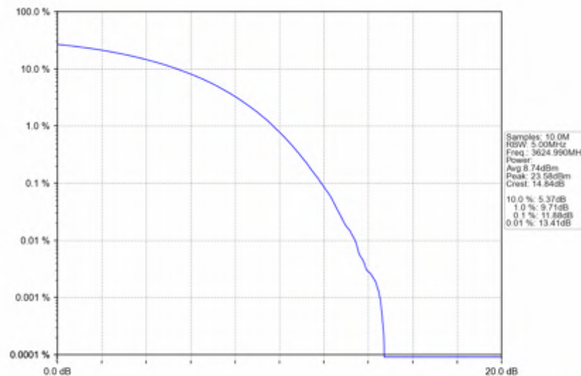
n78d_30kHz_SISO_NTNV_10MHz_CP-OFDM 16 QAM_3624.99MHz_Outer_Full
