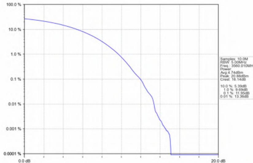
n78d_30kHz_SISO_NTNV_20MHz_CP-OFDM_256_QAM_3560.01MHz_Outer_Full
