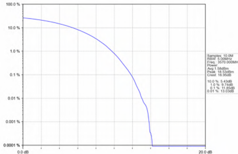
n78d_30kHz_SISO_NTNV_40MHz_CP-OFDM_QPSK_3570MHz_Outer_Full
