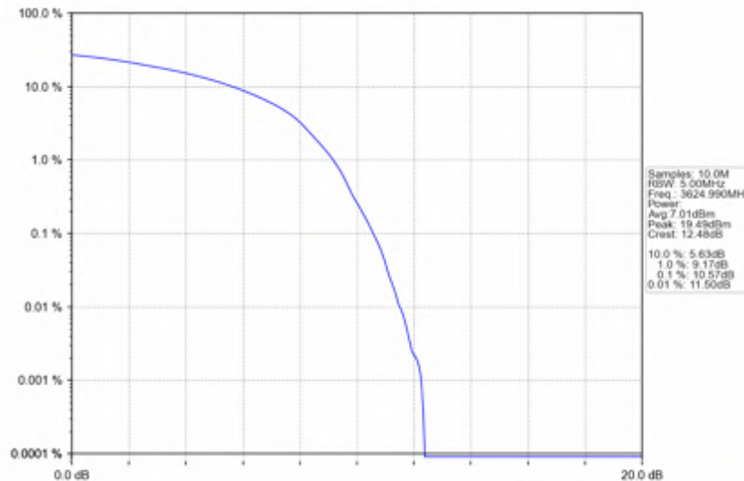
n78d_30kHz_SISO_NTNV_15MHz_DFT-s-OFDM_256_QAM_3624.99MHz_Outer_Full
