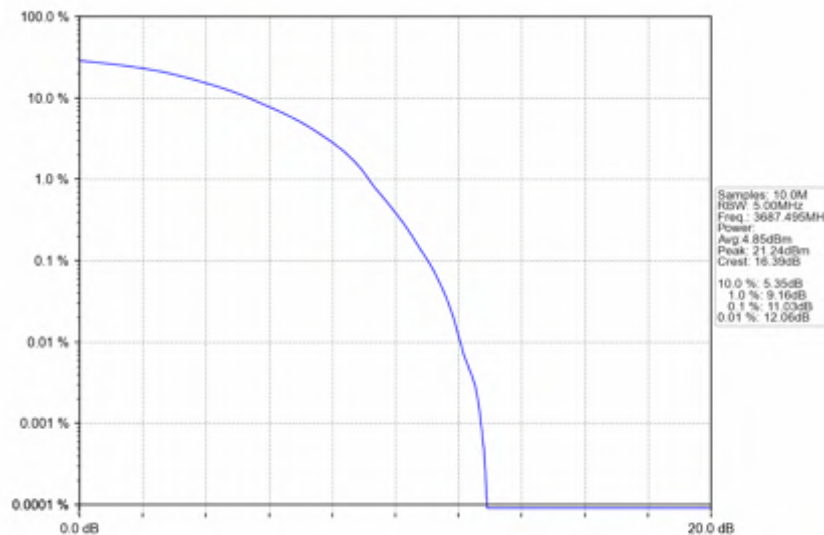
n78d_15kHz_SISO_NTNV_25MHz_DFT-s-OFDM 256 QAM_3687.495MHz_Outer_Full
