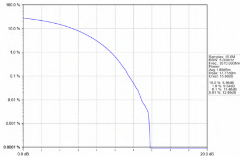
n78d_30kHz_SISO_NTNV_40MHz_CP-OFDM_256_QAM_3570MHz_Outer_Full
