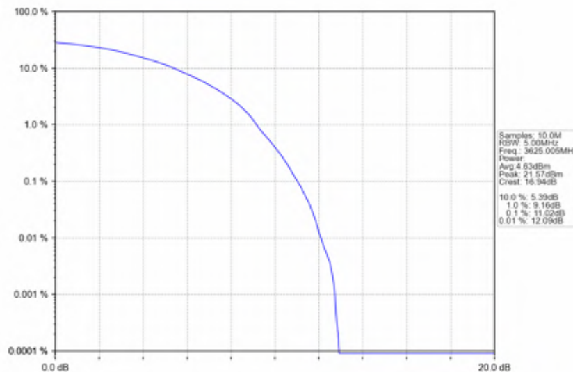
n78d_15kHz_SISO_NTV_25MHz_DFT-s-OFDM_256_QAM_3625.005MHz_Outer_Full
