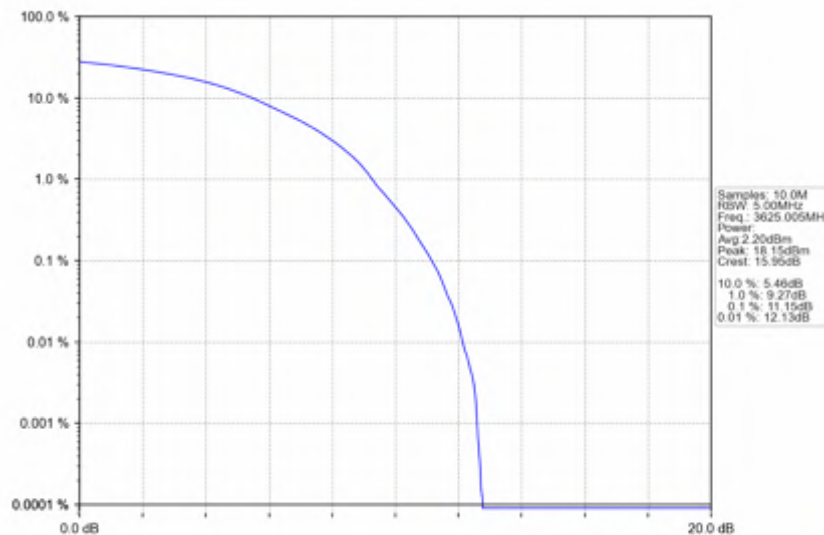
n78d_15kHz_SISO_NTNV_40MHz_DFT-s-OFDM QPSK_3625.005MHz_Outer_Full
