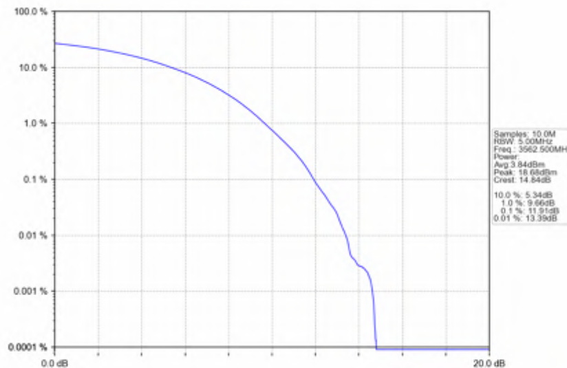
n78d_30kHz_SISO_NTNV_25MHz_CP-OFDM_16_QAM_3562.5MHz_Outer_Full
