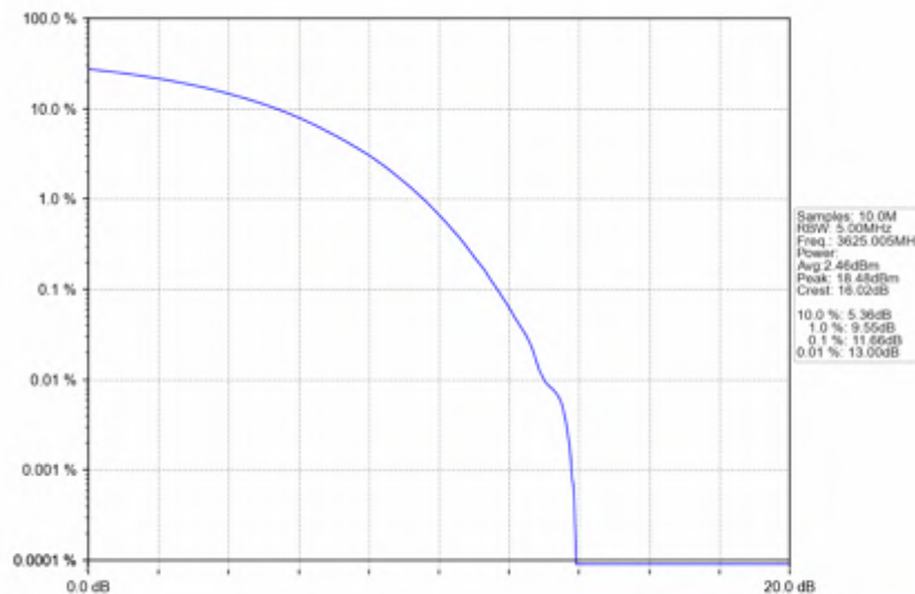
n78d_15kHz_SISO_NTNV_40MHz_CP-OFDM_256_QAM_3625.005MHz_Outer_Full
