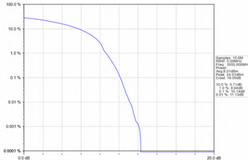
n78d_30kHz_SISO_NTNV_10MHz_DFT-s-OFDM_256_QAM_3555MHz_Outer_Full
