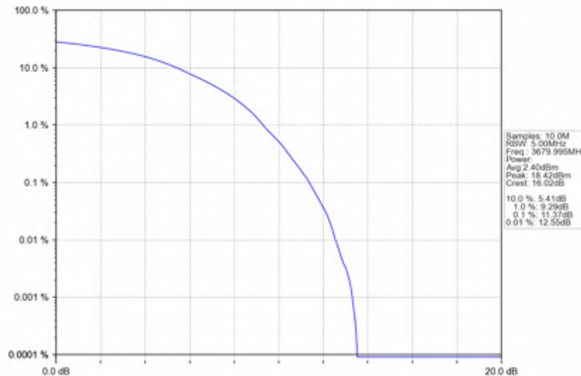
n78d_15kHz_SISO_NTNV_40MHz_DFT-s-OFDM_16_QAM_3679.995MHz_Outer_Full
