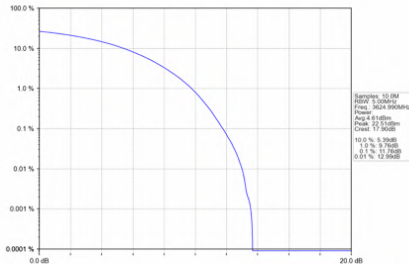
n78d_30kHz_SISO_NTNV_25MHz_CP-OFDM QPSK_3624.99MHz_Outer_Full
