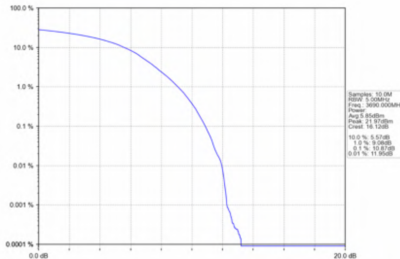
n78d_30kHz_SISO_NTNV_20MHz_DFT-s-OFDM_256_QAM_3690MHz_Outer_Full
