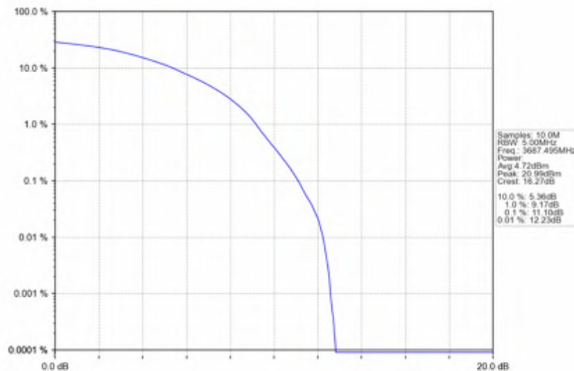
n78d_15kHz_SISO_NTNV_25MHz_DFT-s-OFDM 64 QAM_3687.495MHz_Outer_Full
