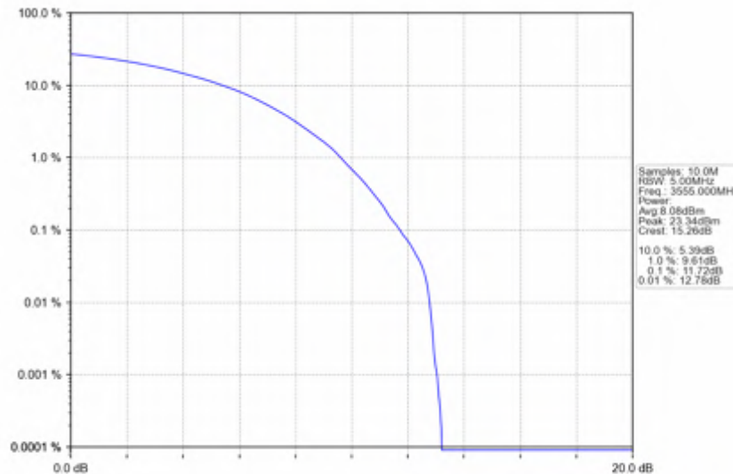
n78d_30kHz_SISO_NTNV_10MHz_CP-OFDM_QPSK_3555MHz_Outer_Full
