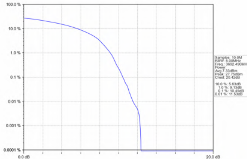
n78d_30kHz_SISO_NTNV_15MHz_DFT-s-OFDM_256_QAM_3692.49MHz_Outer_Full
