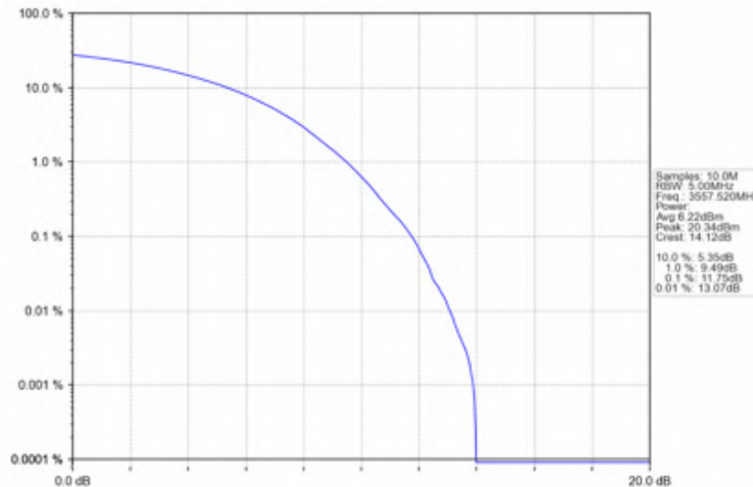
n78d_30kHz_SISO_NTNV_15MHz_CP-OFDM_QPSK_3557.52MHz_Outer_Full
