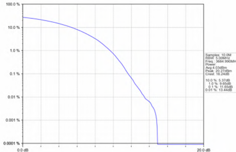
n78d_30kHz_SISO_NTNV_30MHz_CP-OFDM 64 QAM_3684.99MHz_Outer_Full
