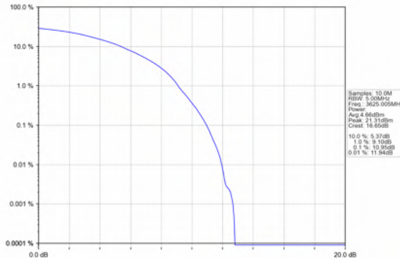
n78d_15kHz_SISO_NTNV_25MHz_DFT-s-OFDM_16_QAM_3625.005MHz_Outer_Full
