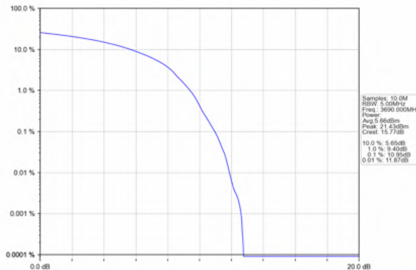
n78d_15kHz_SISO_NTNV_20MHz_DFT-s-OFDM_256_QAM_3690MHz_Outer_Full
