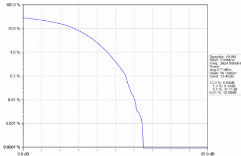
n78d_30kHz_SISO_NTNV_40MHz_DFT-s-OFDM_QPSK_3624.99MHz_Outer_Full
