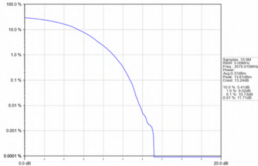
n78d 15kHz SISO NTNV 50MHz DFT-s-OFDM PI/2 BPSK 3575.01MHz Outer Full
