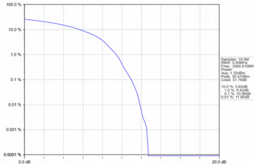
n78d_15kHz_SISO_NTNV_20MHz_DFT-s-OFDM_256_QAM_3560.01MHz_Outer_Full
