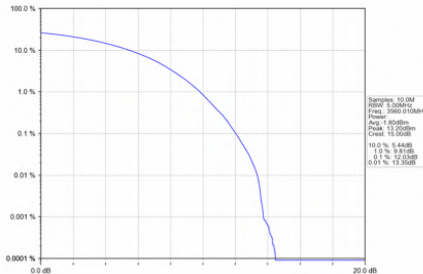
n78d_15kHz_SISO_NTNV_20MHz_CP-OFDM_QPSK_3560.01MHz_Outer_Full
