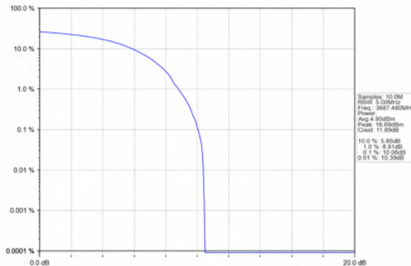
n78d_30kHz_SISO_NTNV_25MHz_DFT-s-OFDM PI/2 BPSK_3687.48MHz_Outer_Full
