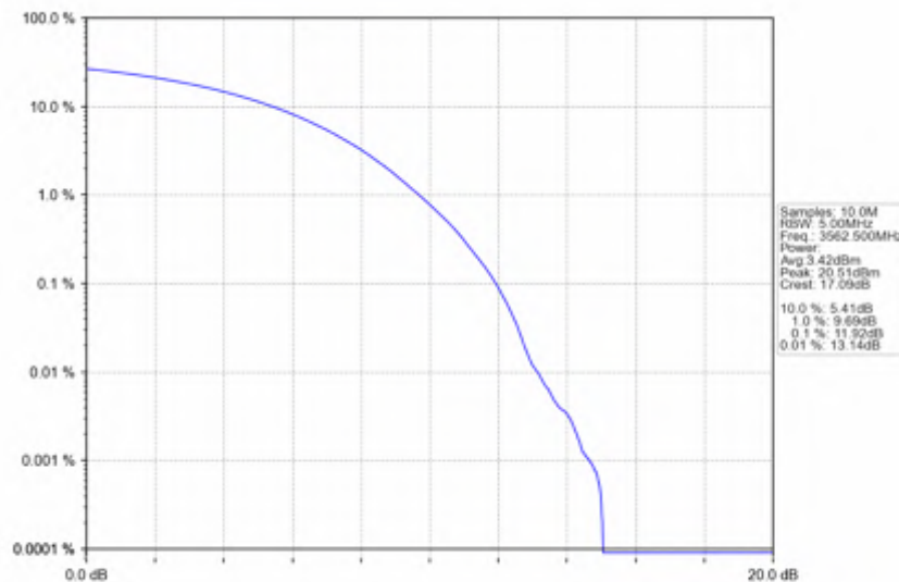
n78d_15kHz_SISO_NTNV_25MHz_CP-OFDM_16_QAM_3562.5MHz_Outer_Full
