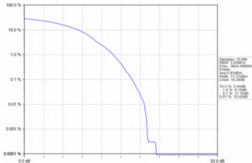
n78d_30kHz_SISO_NTNV_60MHz_DFT-s-OFDM_QPSK_3624.99MHz_Outer_Full
