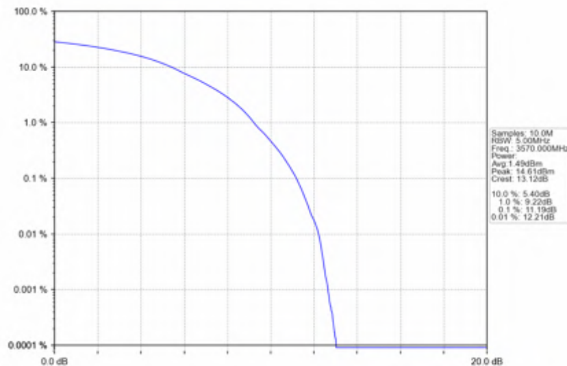
n78d_15kHz_SISO_NTNV_40MHz_DFT-s-OFDM_256_QAM_3570MHz_Outer_Full
