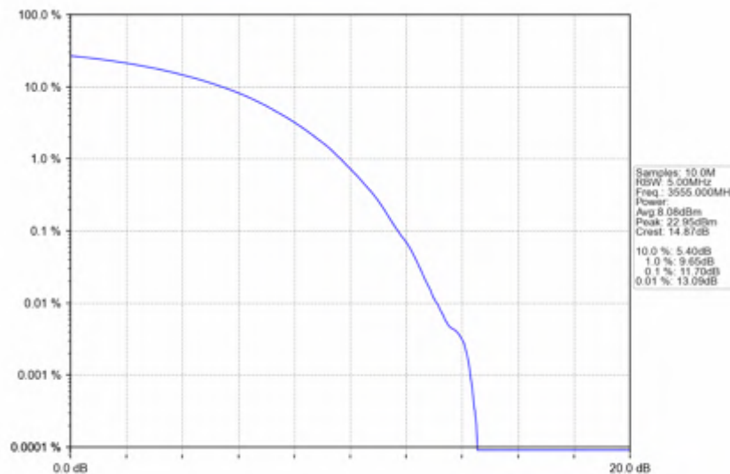
n78d_30kHz_SISO_NTNV_10MHz_CP-OFDM_256_QAM_3555MHz_Outer_Full
