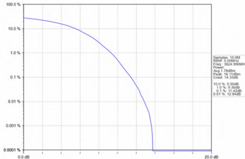
n78d_30kHz_SISO_NTNV_50MHz_DFT-s-OFDM_256_QAM_3624.99MHz_Outer_Full
