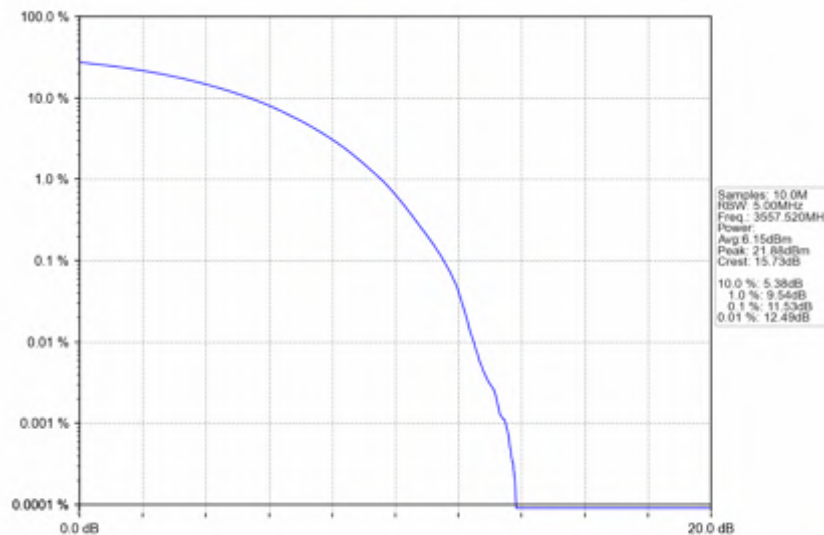
n78d_30kHz_SISO_NTNV_15MHz_CP-OFDM_16_QAM_3557.52MHz_Outer_Full
