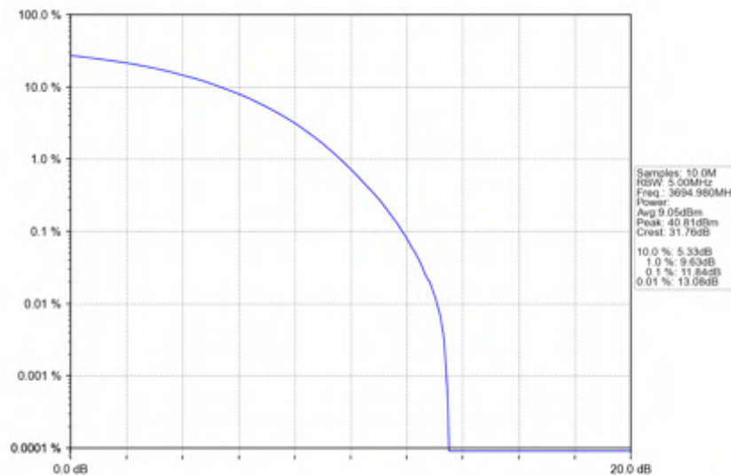
n78d_30kHz_SISO_NTNV_10MHz_CP-OFDM 16 QAM_3694.98MHz_Outer_Full
