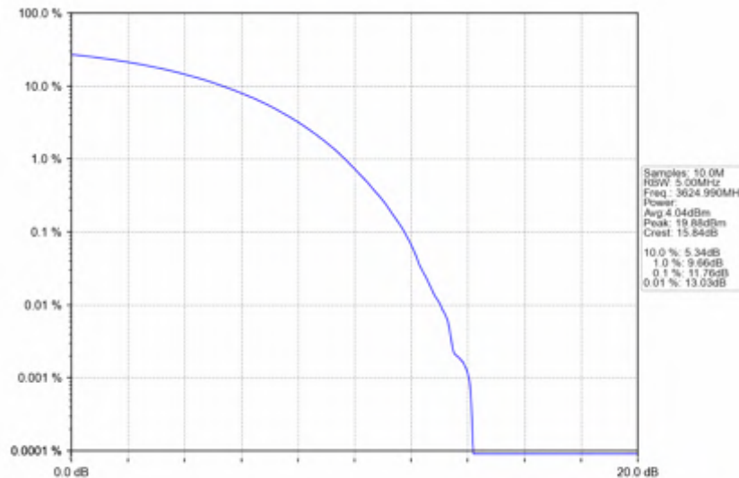
n78d_30kHz_SISO_NTNV_30MHz_CP-OFDM_256_QAM_3624.99MHz_Outer_Full
