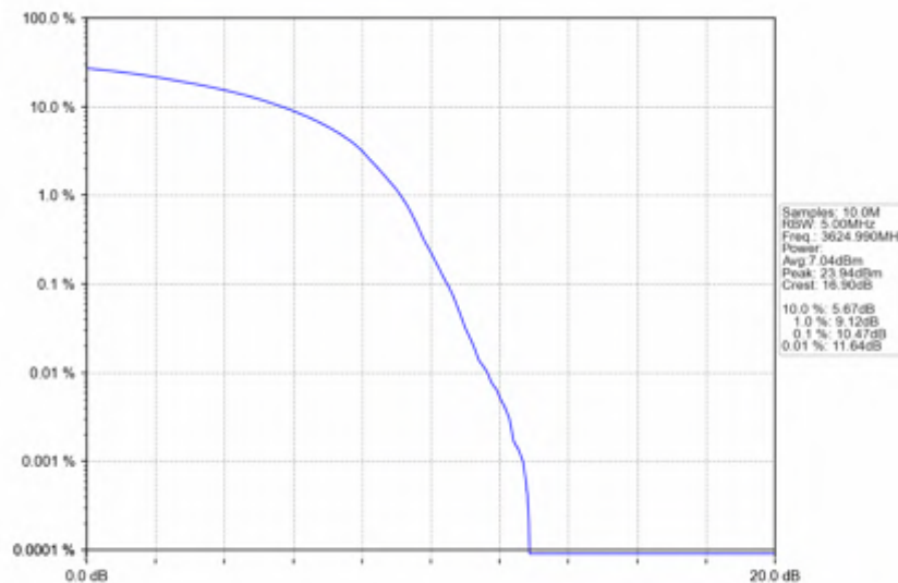
n78d_30kHz_SISO_NTV_15MHz_DFT-s-OFDM_16_QAM_3624.99MHz_Outer_Full
