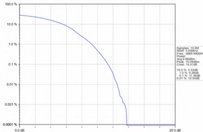
n78d_30kHz_SISO_NTNV_60MHz_DFT-s-OFDM_QPSK_3669.99MHz_Outer_Full
