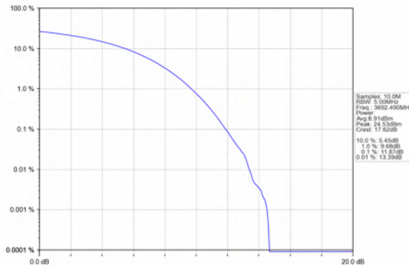
n78d_30kHz_SISO_NTNV_15MHz_CP-OFDM 64 QAM_3692.49MHz_Outer_Full
