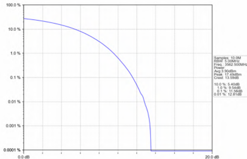
n78d_30kHz_SISO_NTNV_25MHz_CP-OFDM_256_QAM_3562.5MHz_Outer_Full
