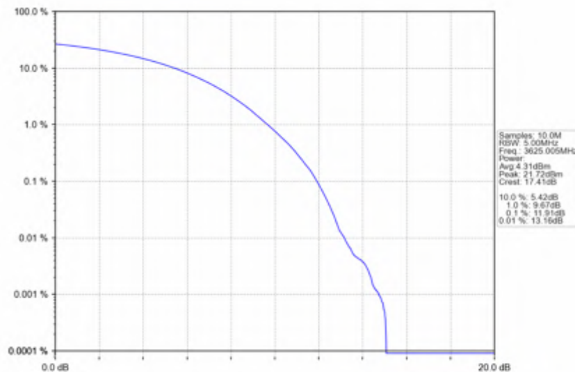
n78d_15kHz_SISO_NTNV_25MHz_CP-OFDM_16_QAM_3625.005MHz_Outer_Full
