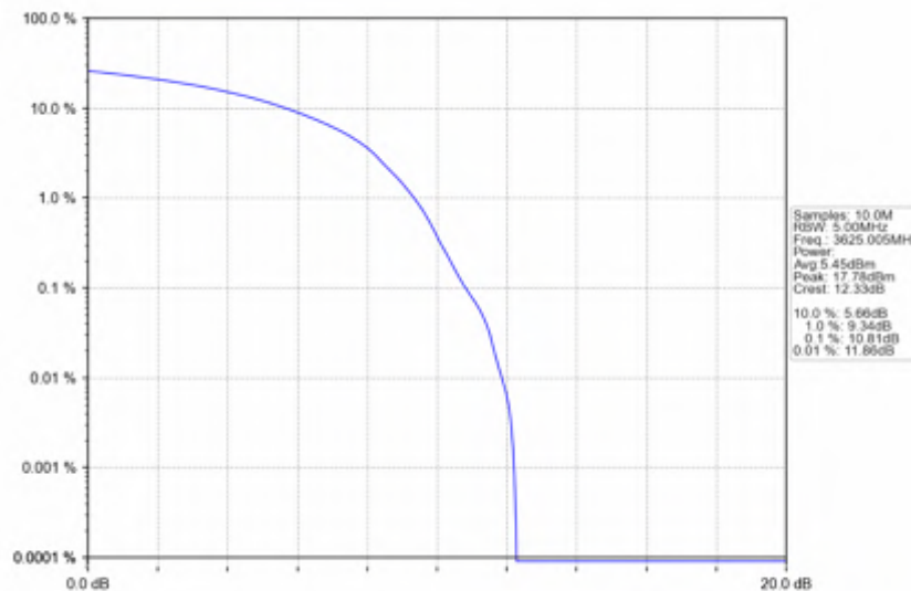
n78d_15kHz_SISO_NTV_20MHz_DFT-s-OFDM_16_QAM_3625.005MHz_Outer_Full
