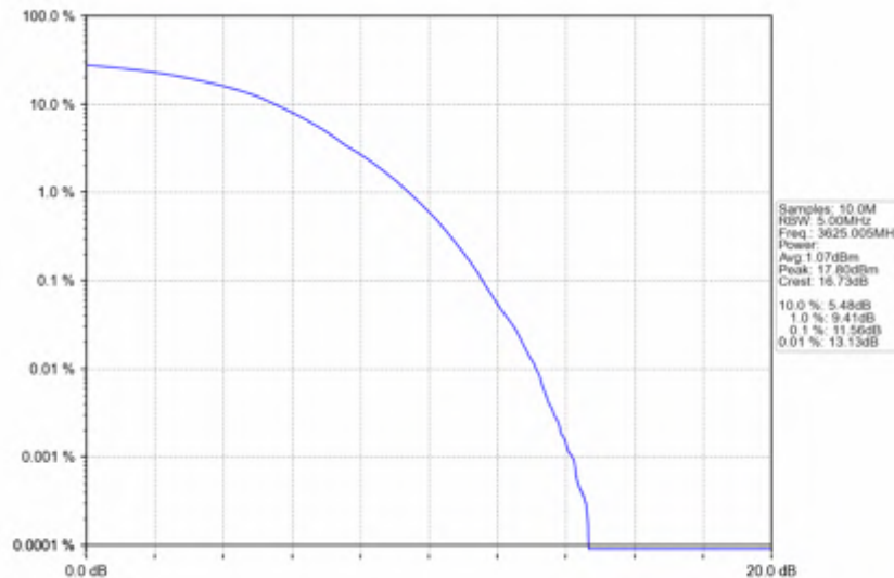
n78d_15kHz_SISO_NTNV_50MHz_DFT-s-OFDM_256_QAM_3625.005MHz_Outer_Full
