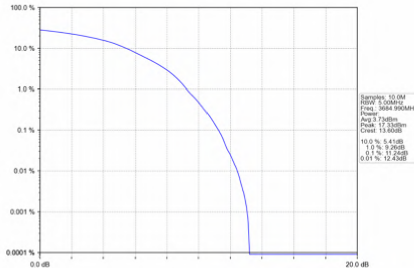
n78d_15kHz_SISO_NTNV_30MHz_DFT-s-OFDM 256 QAM_3684.99MHz_Outer_Full
