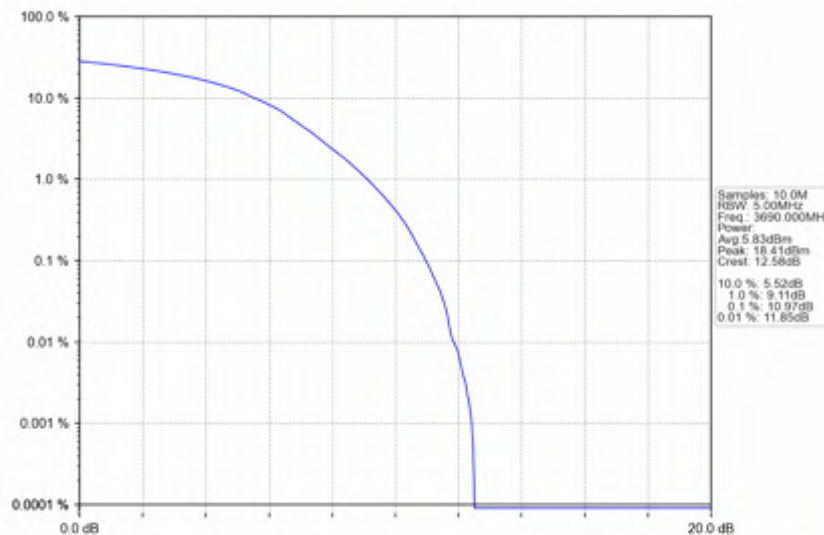
n78d_30kHz_SISO_NTNV_20MHz_DFT-s-OFDM 16 QAM_3690MHz_Outer_Full
