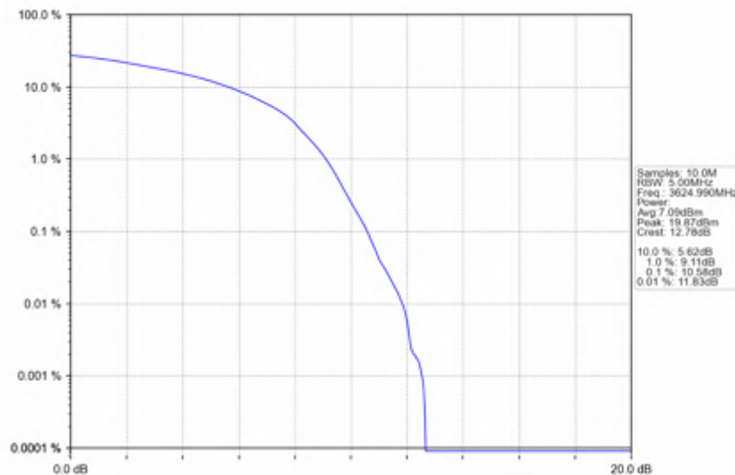
n78d_30kHz_SISO_NTV_15MHz_DFT-s-OFDM_64_QAM_3624.99MHz_Outer_Full
