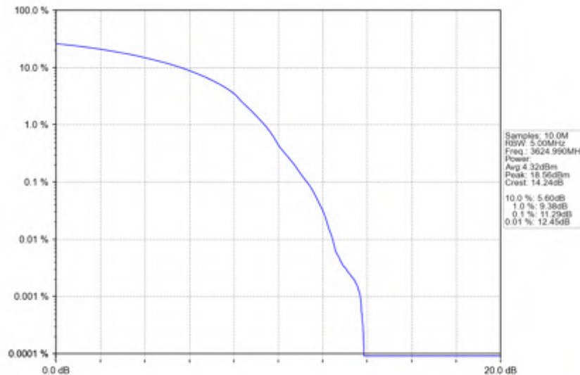
n78d_30kHz_SISO_NTNV_30MHz_DFT-s-OFDM_256_QAM_3624.99MHz_Outer_Full
