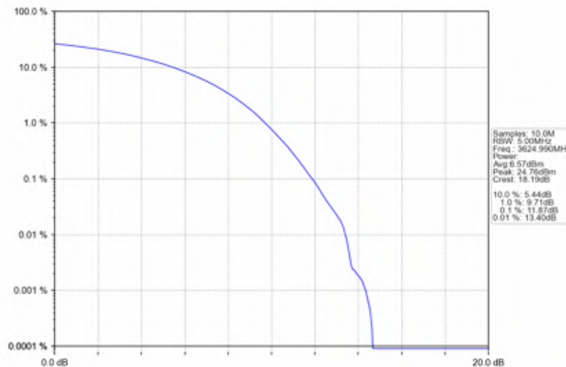
n78d_30kHz_SISO_NTNV_15MHz_CP-OFDM 64 QAM_3624.99MHz_Outer_Full
