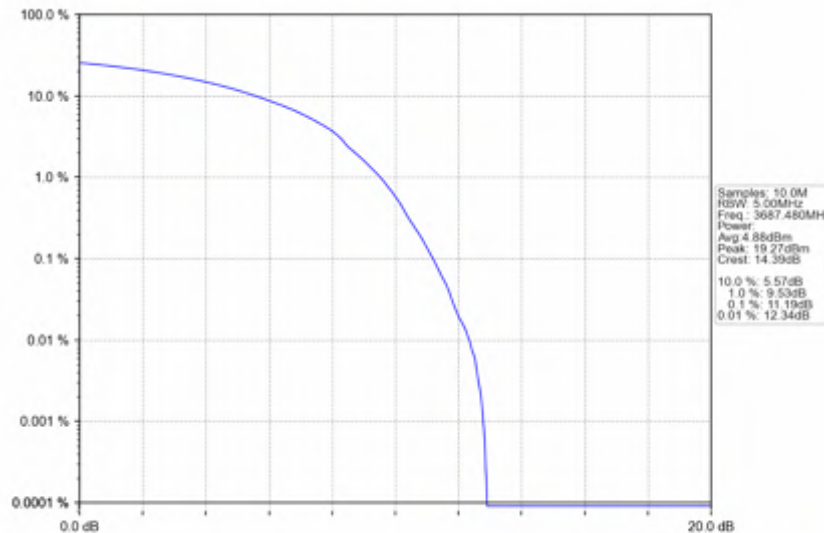
n78d_30kHz_SISO_NTNV_25MHz_DFT-s-OFDM_256_QAM_3687.48MHz_Outer_Full
