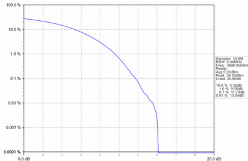
n78d_30kHz_SISO_NTNV_20MHz_CP-OFDM QPSK_3690MHz_Outer_Full
