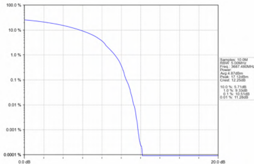
n78d_30kHz_SISO_NTNV_25MHz_DFT-s-OFDM_QPSK_3687.48MHz_Outer_Full
