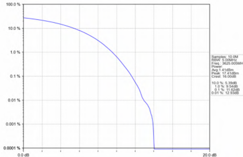
n78d_15kHz_SISO_NTNV_50MHz_CP-OFDM_256_QAM_3625.005MHz_Outer_Full
