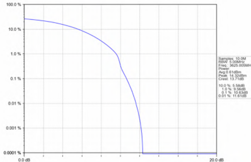
n78d_15kHz_SISO_NTNV_15MHz_DFT-s-OFDM_16_QAM_3625.005MHz_Outer_Full
