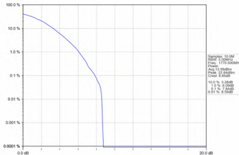
n66_30kHz_SISO_NTNV_20MHz_DFT-s-OFDM 256 QAM_1770MHz_Outer_Full
