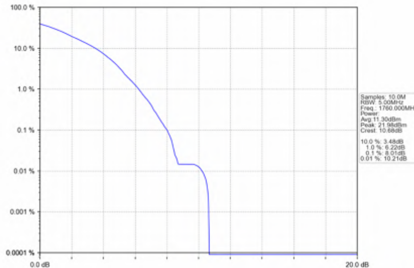
n66_15kHz_SISO_NTNV_40MHz_DFT-s-OFDM 256 QAM_1760MHz_Outer_Full
