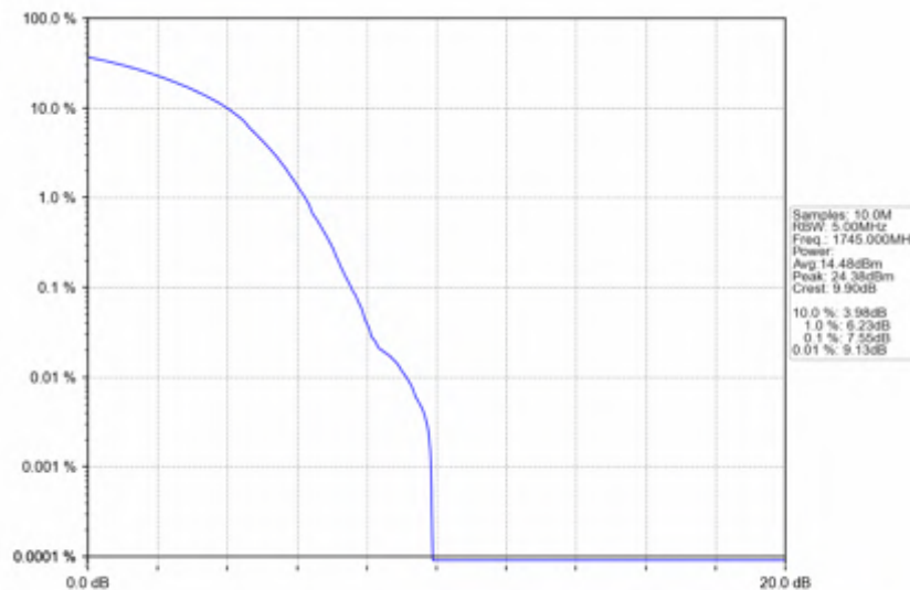
n66_30kHz_SISO_NTNV_30MHz_DFT-s-OFDM_16_QAM_1745MHz_Outer_Full
