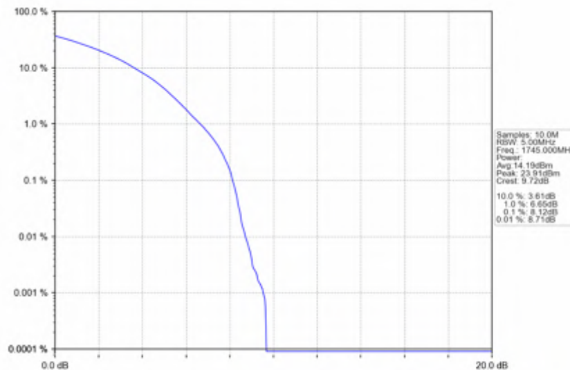
n66_30kHz_SISO_NTNV_25MHz_CP-OFDM QPSK_1745MHz_Outer_Full
