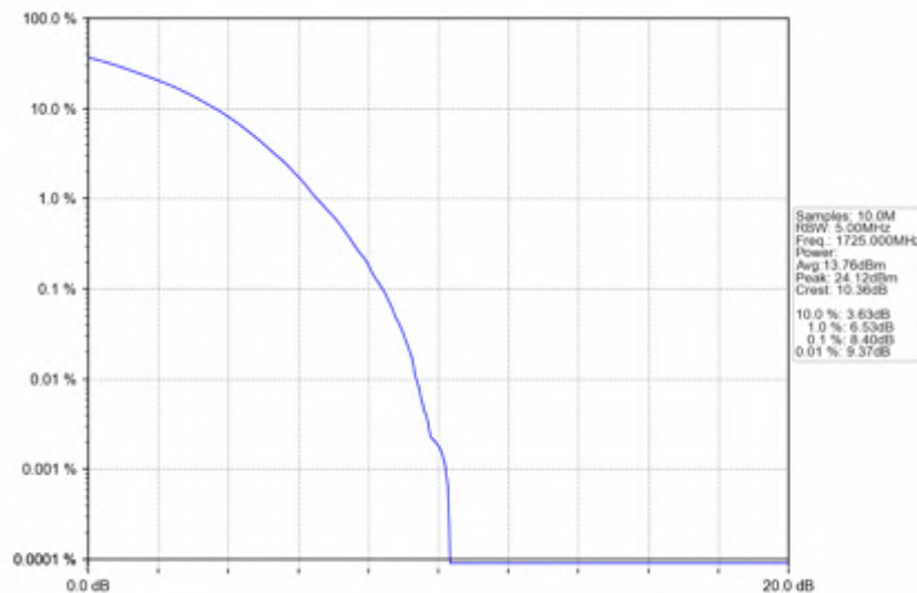
n66_30kHz_SISO_NTNV_30MHz_CP-OFDM_64_QAM_1725MHz_Outer_Full
