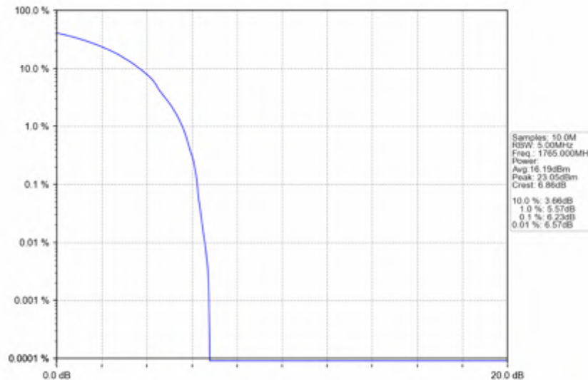
n66_30kHz_SISO_NTNV_30MHz_DFT-s-OFDM_PI/2_BPSK_1765MHz_Outer_Full
