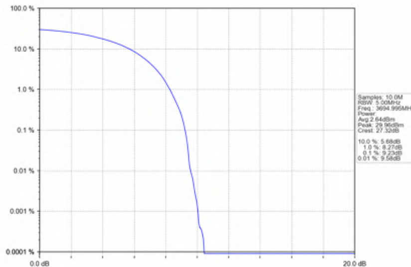
n78d_15kHz_SISO_NTNV_10MHz_DFT-s-OFDM QPSK_3694.995MHz_Outer_Full
