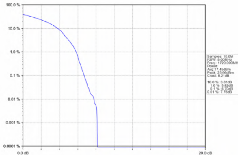
n66_15kHz_SISO_NTNV_20MHz_DFT-s-OFDM QPSK_1720MHz_Outer_Full
