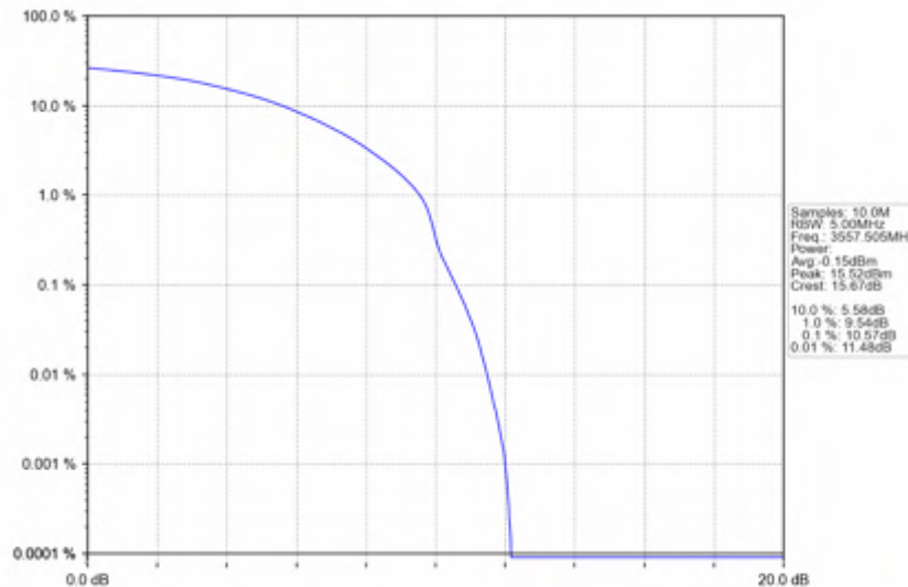
n78d_15kHz_SISO_NTNV_15MHz_DFT-s-OFDM_16_QAM_3557.505MHz_Outer_Full
