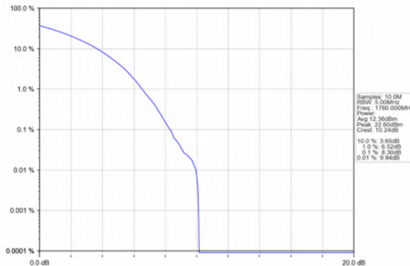
n66_15kHz_SISO_NTNV_40MHz_CP-OFDM 64 QAM_1760MHz_Outer_Full
