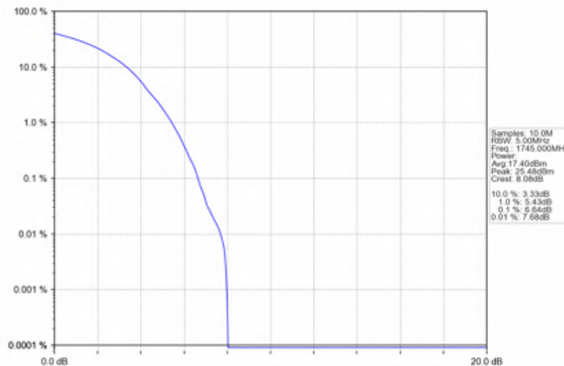
n66_30kHz_SISO_NTNV_10MHz_DFT-s-OFDM_256_QAM_1745MHz_Outer_Full
