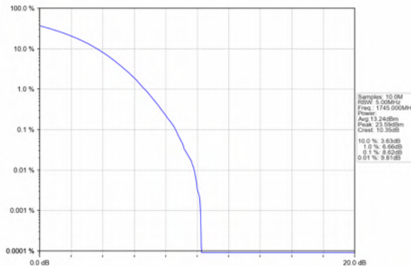
n66 15kHz SISO NTN 30MHz CP-OFDM 16 QAM 1745MHz Outer Full
