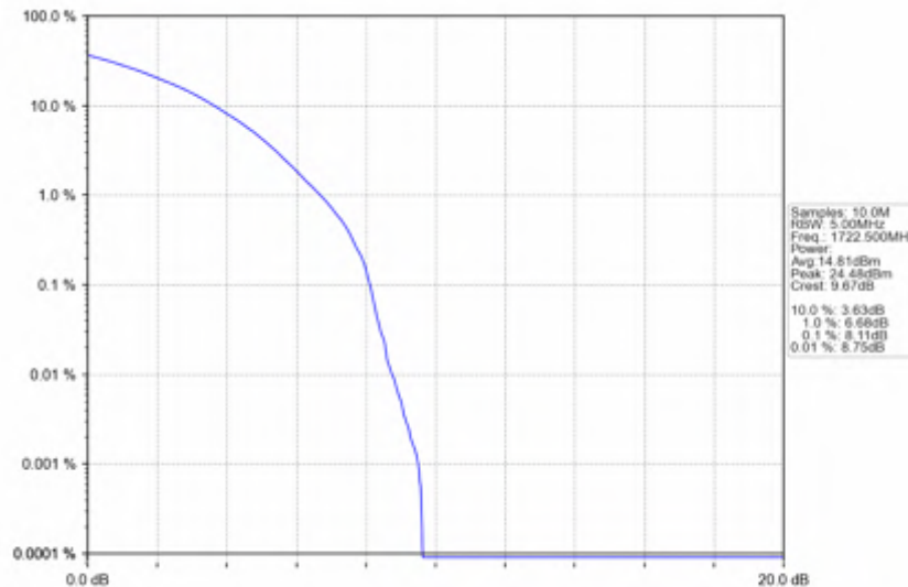
n66_30kHz_SISO_NTNV_25MHz_CP-OFDM_QPSK_1722.5MHz_Outer_Full
