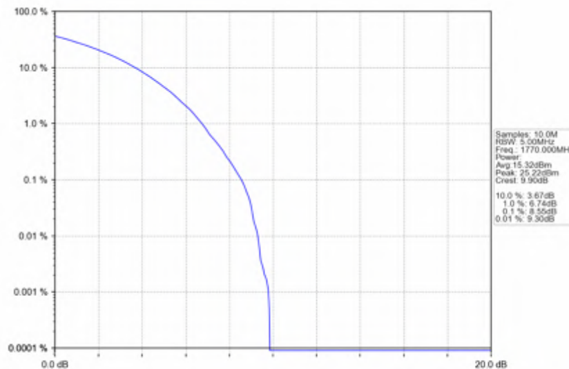
n66_15kHz_SISO_NTNV_20MHz_CP-OFDM 16 QAM_1770MHz_Outer_Full
