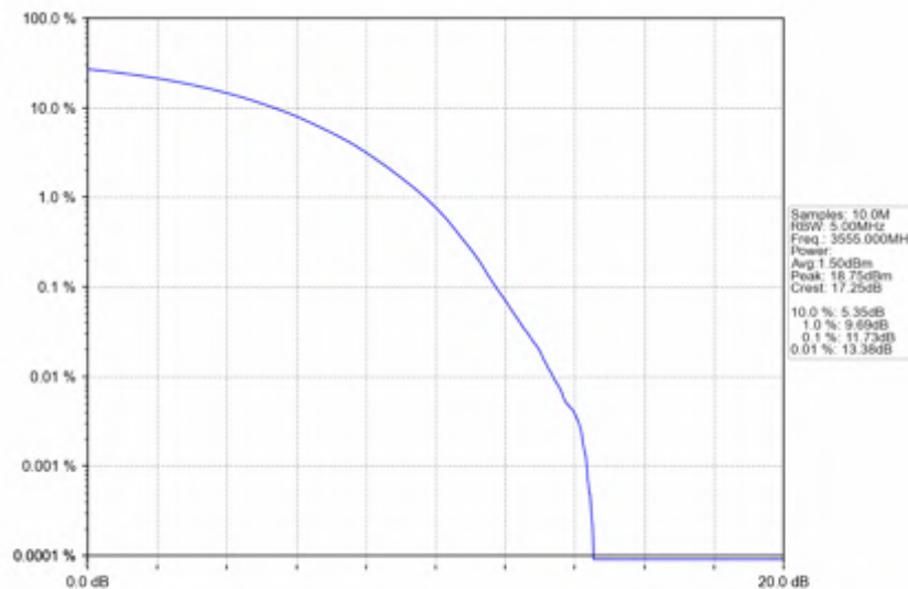
n78d_15kHz_SISO_NTNV_10MHz_CP-OFDM_256_QAM_3555MHz_Outer_Full
