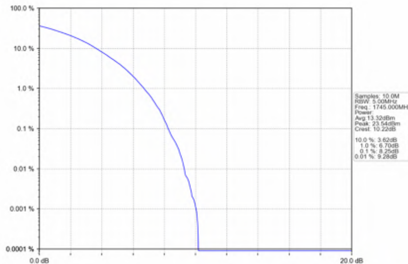
n66_30kHz_SISO_NTNV_30MHz_CP-OFDM QPSK_1745MHz_Outer_Full
