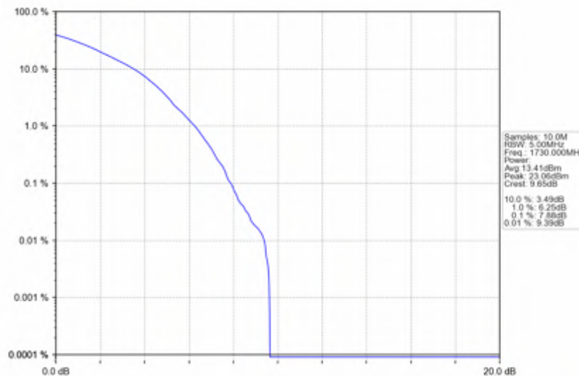
n66_15kHz_SISO_NTNV_40MHz_DFT-s-OFDM_64_QAM_1730MHz_Outer_Full
