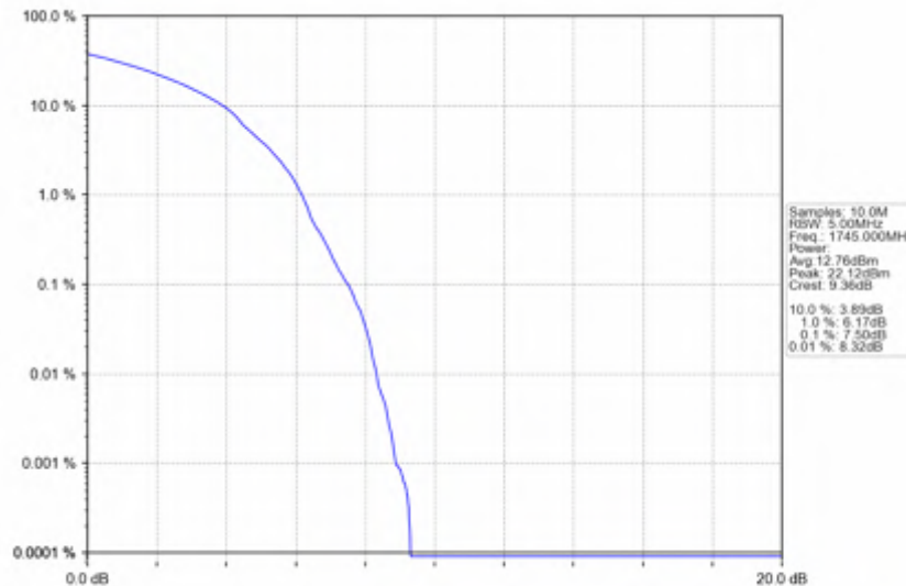
n66_30kHz_SISO_NTNV_25MHz_DFT-s-OFDM_256_QAM_1745MHz_Outer_Full
