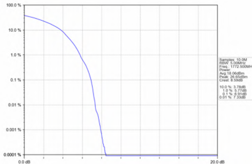
n66_30kHz_SISO_NTV_15MHz_DFT-s-OFDM 16 QAM_1772.5MHz_Outer_Full
