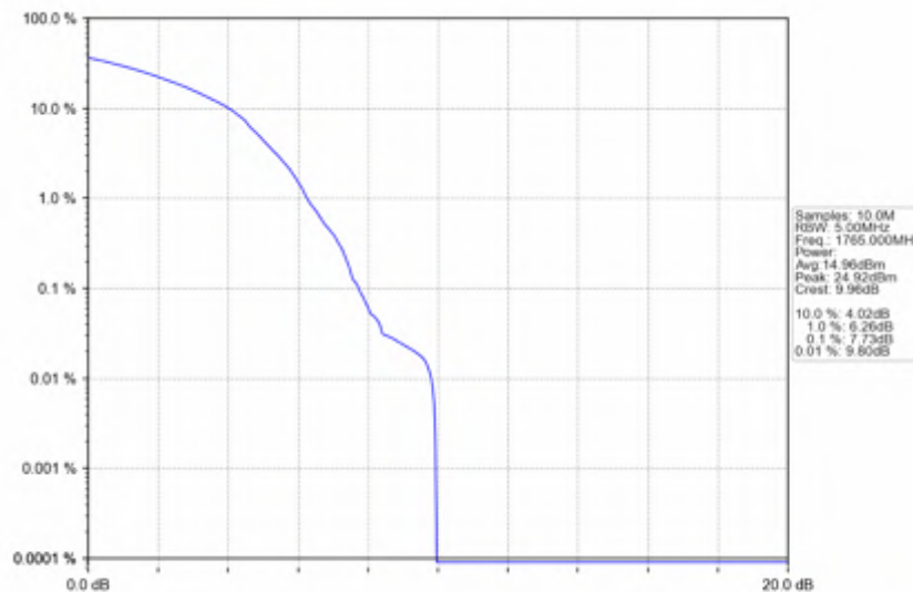
n66_30kHz_SISO_NTNV_30MHz_DFT-s-OFDM_16_QAM_1765MHz_Outer_Full
