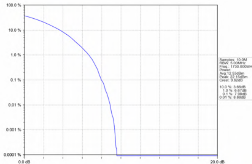
n66_30kHz_SISO_NTNV_40MHz_CP-OFDM 64 QAM_1730MHz_Outer_Full
