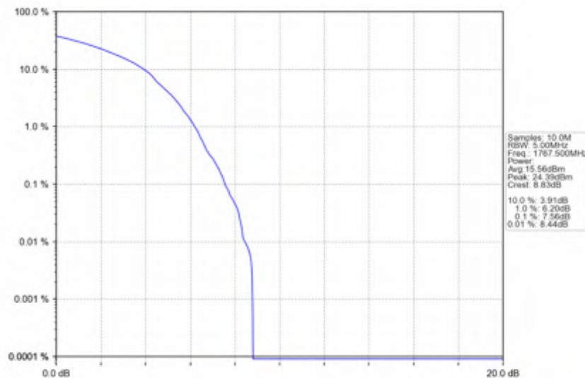
n66_30kHz_SISO_NTV_25MHz_DFT-s-OFDM_16_QAM_1767.5MHz_Outer_Full
