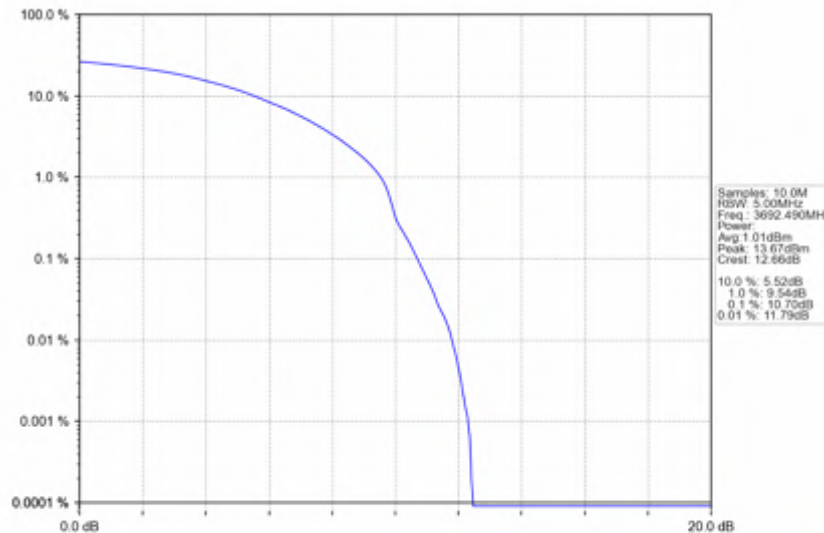
n78d_15kHz_SISO_NTNV_15MHz_DFT-s-OFDM_256_QAM_3692.49MHz_Outer_Full
