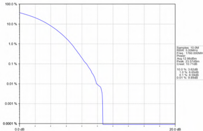
n66_15kHz_SISO_NTNV_40MHz_CP-OFDM 16 QAM_1760MHz_Outer_Full
