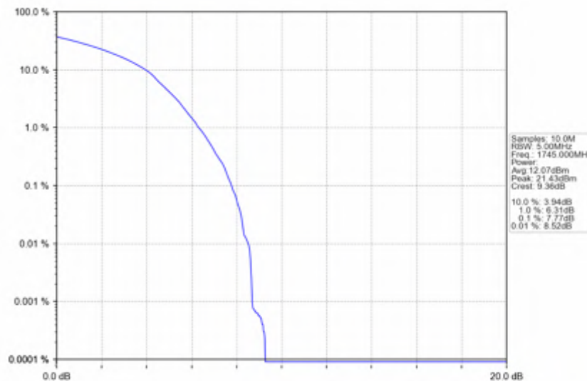
n66_30kHz_SISO_NTNV_30MHz_DFT-s-OFDM_256_QAM_1745MHz_Outer_Full
