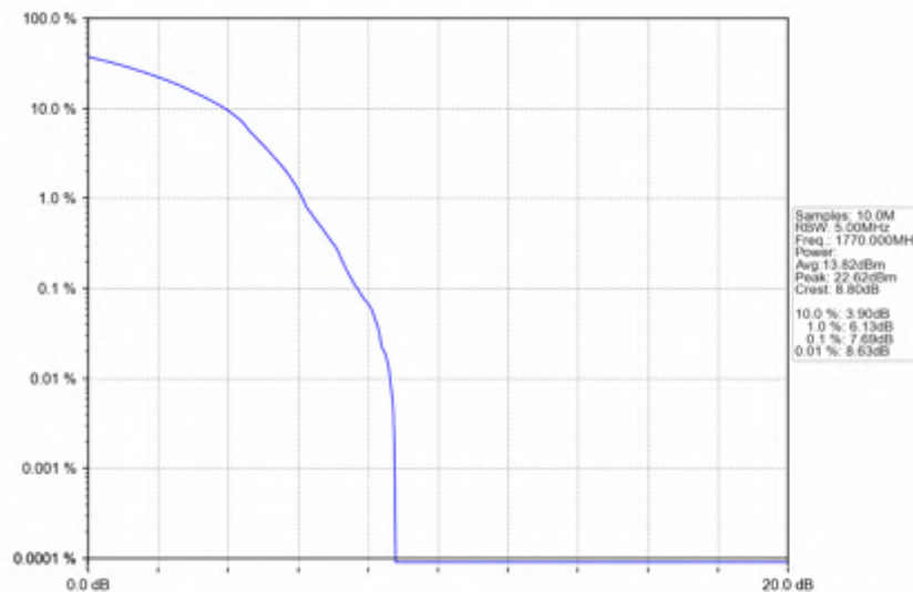
n66_15kHz_SISO_NTNV_20MHz_DFT-s-OFDM 256 QAM_1770MHz_Outer_Full
