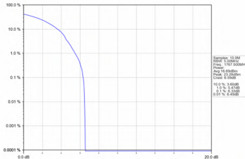
n66_30kHz_SISO_NTNV_25MHz_DFT-s-OFDM PI/2 BPSK_1767.5MHz_Outer_Full
