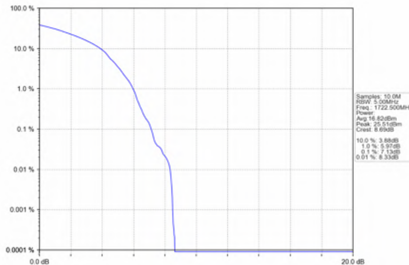
n66_30kHz_SISO_NTNV_25MHz_DFT-s-OFDM QPSK_1722.5MHz_Outer_Full
