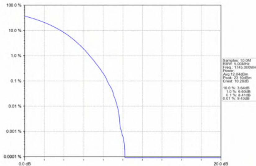
n66_30kHz_SISO_NTNV_30MHz_CP-OFDM_64_QAM_1745MHz_Outer_Full
