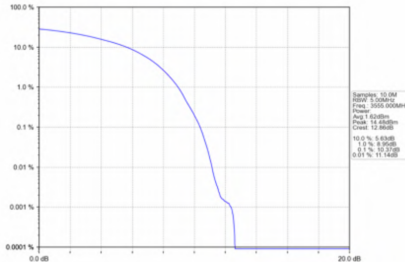
n78d_15kHz_SISO_NTNV_10MHz_DFT-s-OFDM_256_QAM_3555MHz_Outer_Full
