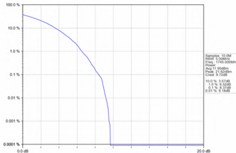
n66_30kHz_SISO_NTNV_40MHz_CP-OFDM QPSK_1745MHz_Outer_Full
