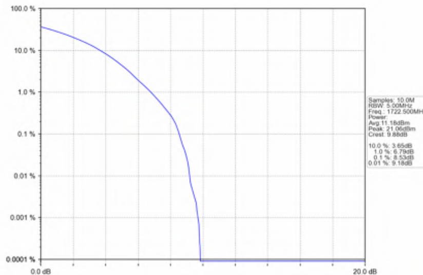
n66_30kHz_SISO_NTNV_25MHz_CP-OFDM_256_QAM_1722.5MHz_Outer_Full
