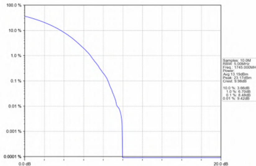
n66_15kHz_SISO_NTNV_30MHz_CP-OFDM QPSK_1745MHz_Outer_Full
