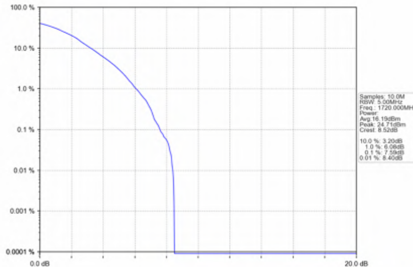
n66_30kHz_SISO_NTNV_20MHz_DFT-s-OFDM_64_QAM_1720MHz_Outer_Full
