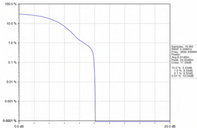
n78d_15kHz_SISO_NTNV_15MHz_DFT-s-OFDM PI/2 BPSK_3692.49MHz_Outer_Full
