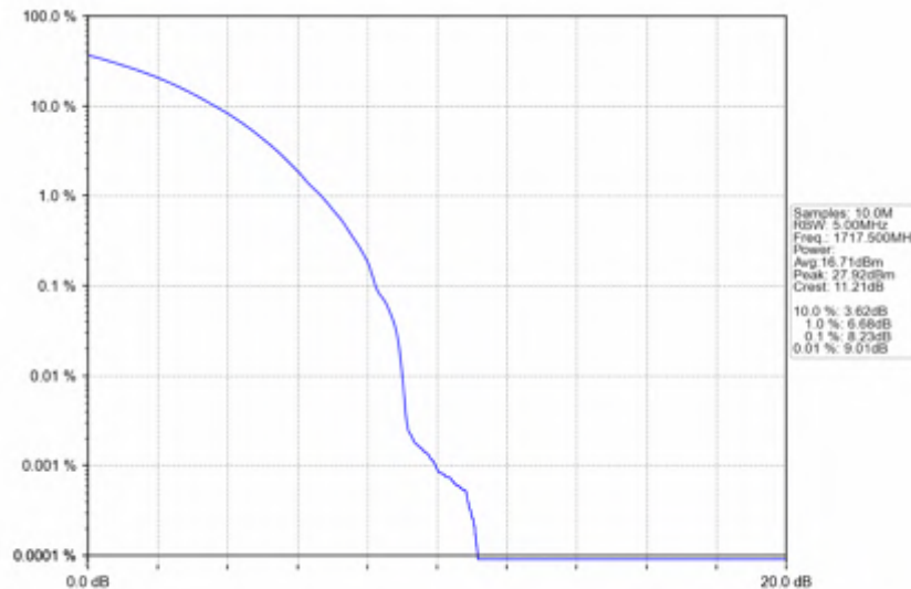
n66_30kHz_SISO_NTNV_15MHz_CP-OFDM_QPSK_1717.5MHz_Outer_Full
