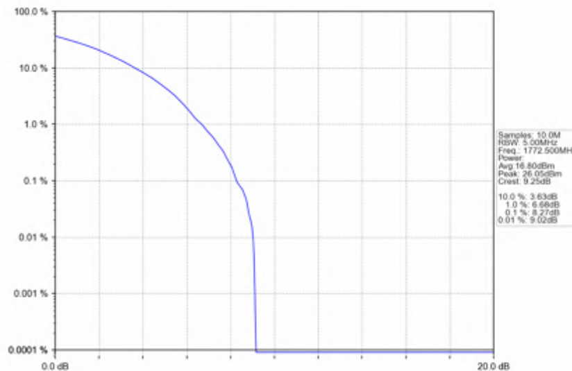
n66_30kHz_SISO_NTNV_15MHz_CP-OFDM QPSK_1772.5MHz_Outer_Full
