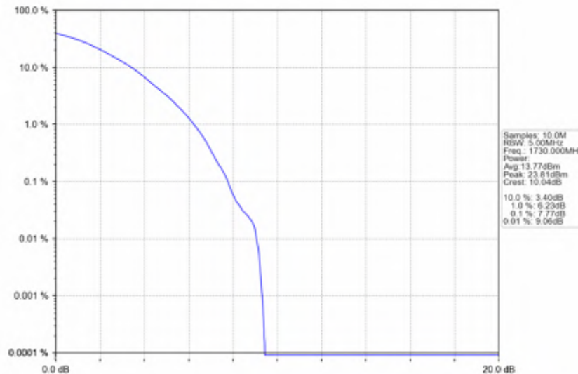
n66_30kHz_SISO_NTNV_40MHz_DFT-s-OFDM_64_QAM_1730MHz_Outer_Full
