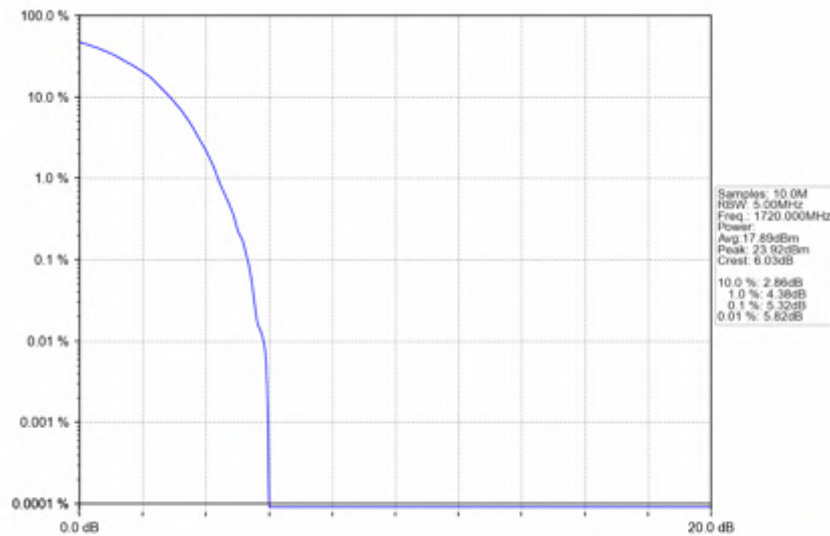
n66_30kHz_SISO_NTNV_20MHz_DFT-s-OFDM_PI/2_BPSK_1720MHz_Outer_Full
