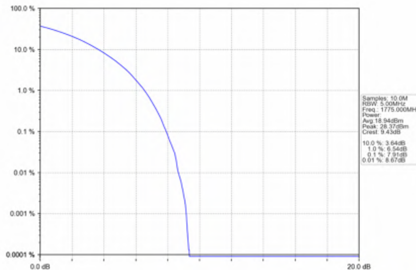
n66_30kHz_SISO_NTNV_10MHz_CP-OFDM 16 QAM_1775MHz_Outer_Full
