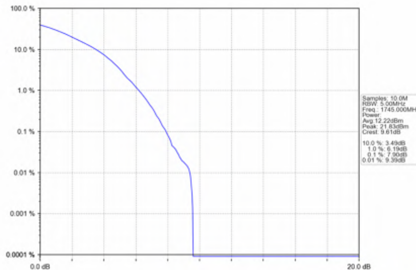
n66_15kHz_SISO_NTNV_40MHz_DFT-s-OFDM_64_QAM_1745MHz_Outer_Full
