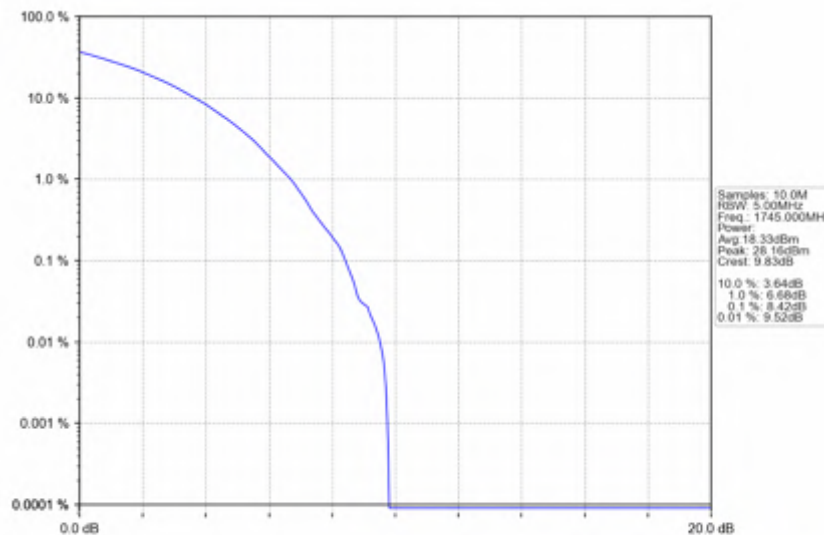
n66_30kHz_SISO_NTNV_10MHz_CP-OFDM 64 QAM_1745MHz_Outer_Full
