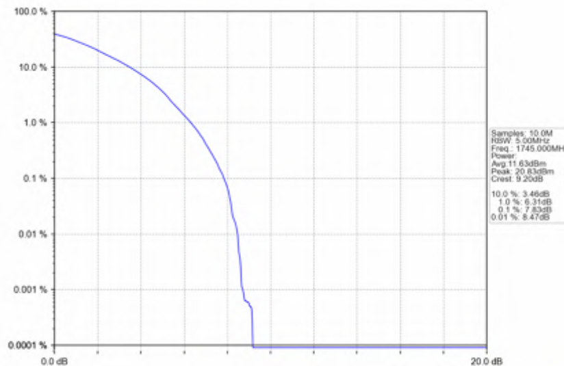
n66_15kHz_SISO_NTNV_30MHz_DFT-s-OFDM_256_QAM_1745MHz_Outer_Full
