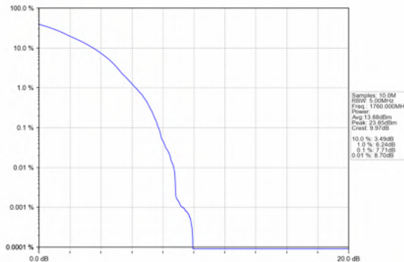
n66_15kHz_SISO_NTNV_40MHz_DFT-s-OFDM_16_QAM_1760MHz_Outer_Full
