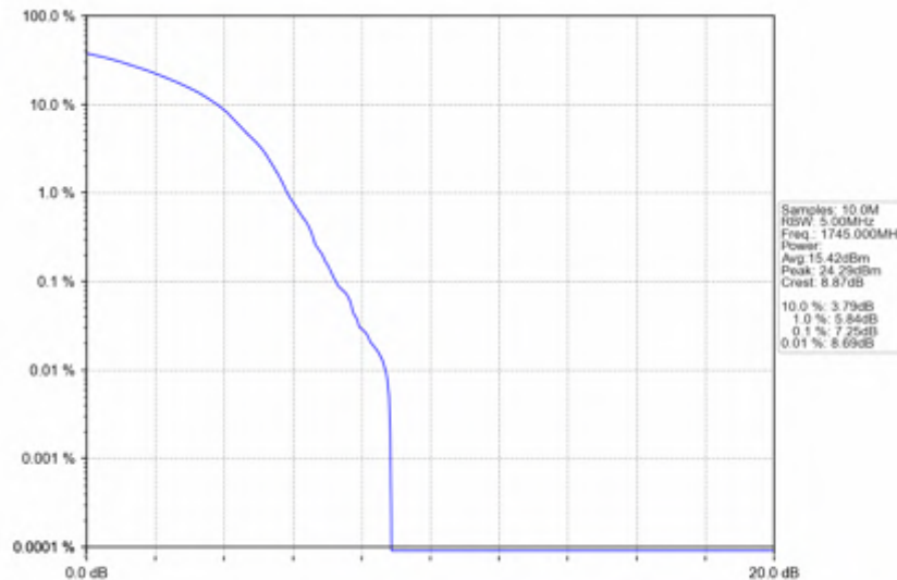
n66_30kHz_SISO_NTNV_15MHz_DFT-s-OFDM_256_QAM_1745MHz_Outer_Full
