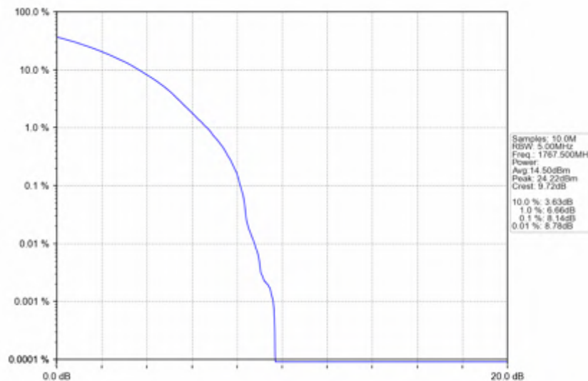
n66_30kHz_SISO_NTNV_25MHz_CP-OFDM QPSK_1767.5MHz_Outer_Full
