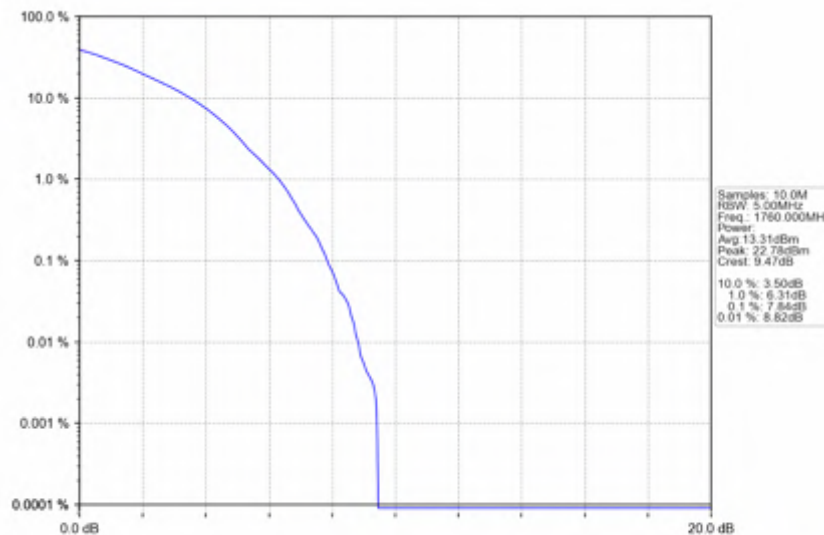
n66_15kHz_SISO_NTNV_40MHz_DFT-s-OFDM_64_QAM_1760MHz_Outer_Full
