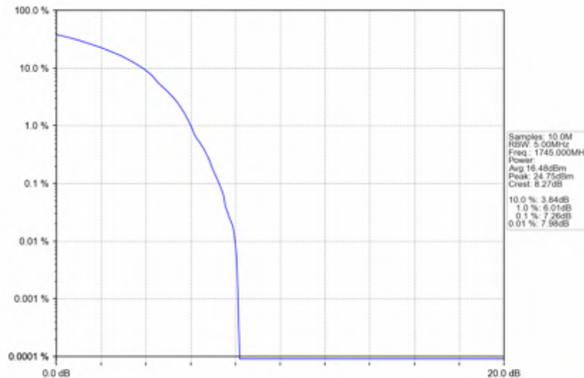
n66_15kHz_SISO_NTNV_20MHz_DFT-s-OFDM_16_QAM_1745MHz_Outer_Full
