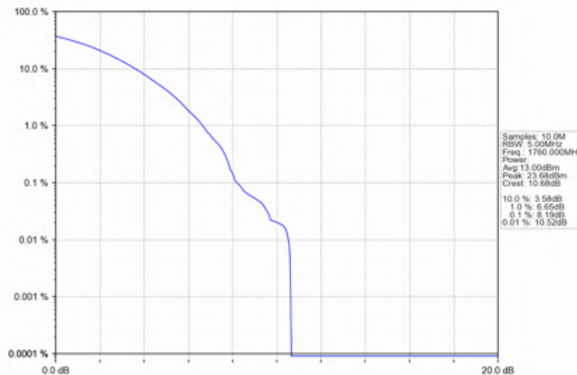
n66_30kHz_SISO_NTNV_40MHz_CP-OFDM 16 QAM_1760MHz_Outer_Full
