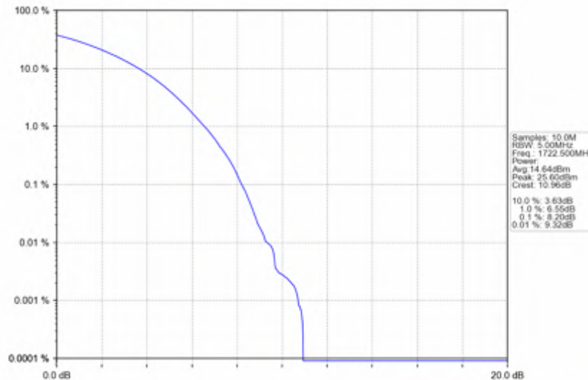
n66_15kHz_SISO_NTNV_25MHz_CP-OFDM_QPSK_1722.5MHz_Outer_Full
