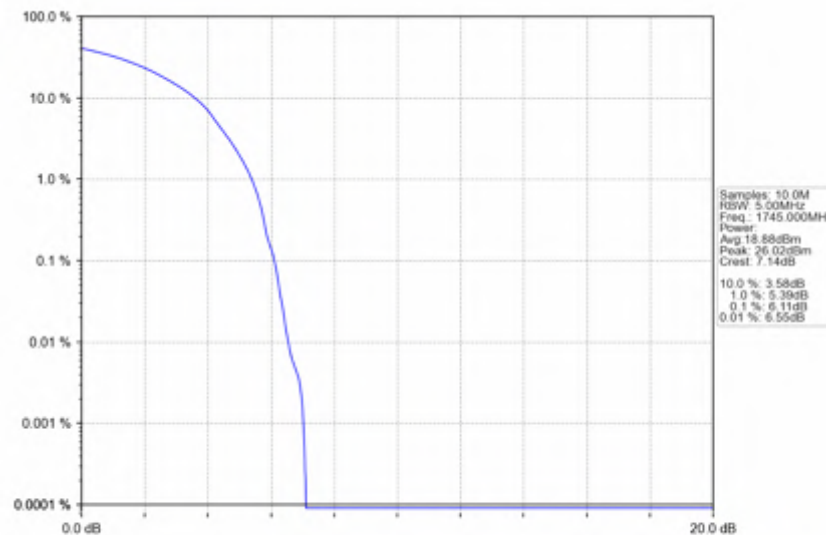
n66_30kHz_SISO_NTNV_15MHz_DFT-s-OFDM QPSK_1745MHz_Outer_Full
