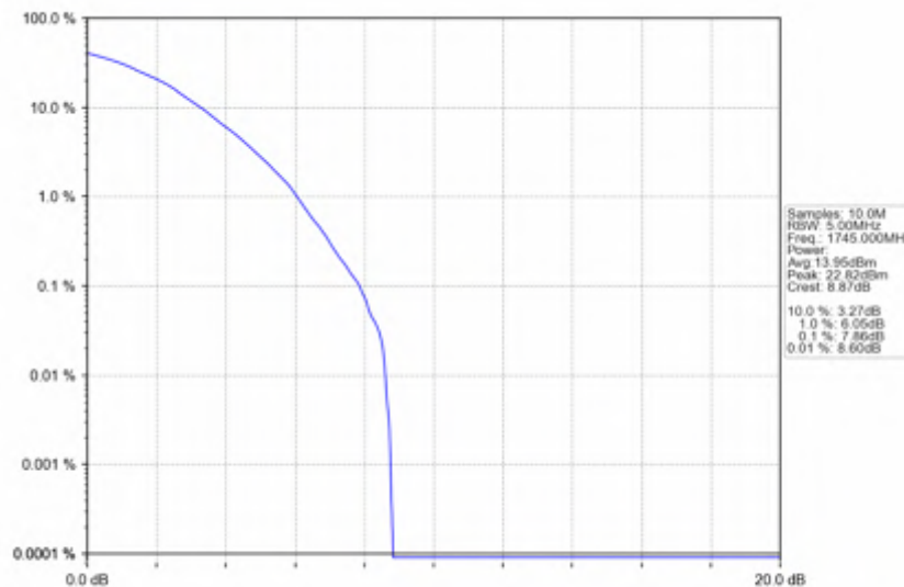
n66_30kHz_SISO_NTNV_20MHz_DFT-s-OFDM_256_QAM_1745MHz_Outer_Full
