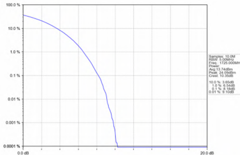
n66_15kHz_SISO_NTNV_30MHz_CP-OFDM 64 QAM_1725MHz_Outer_Full
