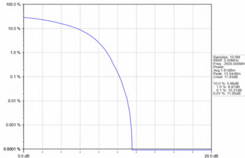
n78d_15kHz_SISO_NTNV_10MHz_DFT-s-OFDM_64_QAM_3555MHz_Outer_Full
