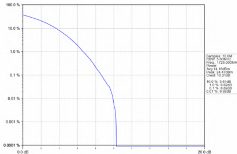
n66_15kHz_SISO_NTNV_30MHz_CP-OFDM_16_QAM_1725MHz_Outer_Full
