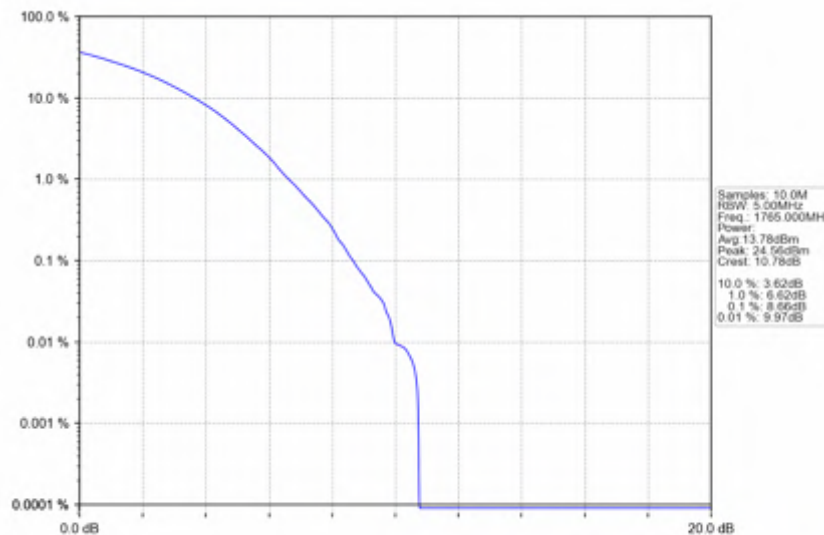
n66_15kHz_SISO_NTNV_30MHz_CP-OFDM 16 QAM_1765MHz_Outer_Full
