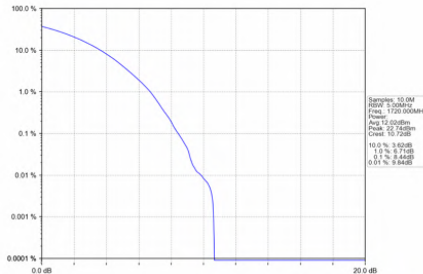
n66_30kHz_SISO_NTNV_20MHz_CP-OFDM 256 QAM_1720MHz_Outer_Full
