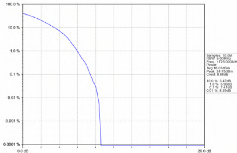
n66_15kHz_SISO_NTNV_30MHz_DFT-s-OFDM QPSK_1725MHz_Outer_Full
