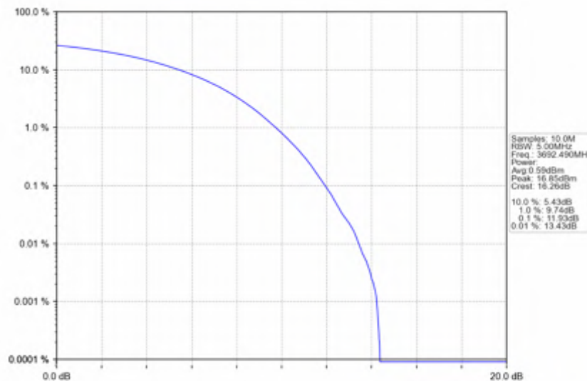
n78d_15kHz_SISO_NTNV_15MHz_CP-OFDM QPSK_3692.49MHz_Outer_Full
