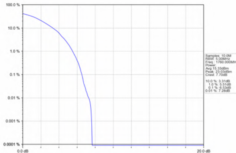
n66_30kHz_SISO_NTNV_40MHz_DFT-s-OFDM_PI/2_BPSK_1760MHz_Outer_Full
