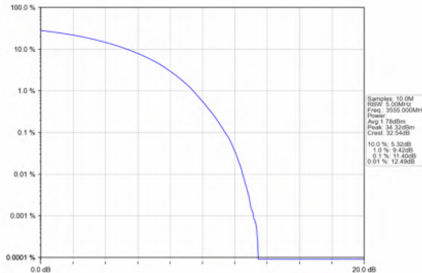
n78d_15kHz_SISO_NTNV_10MHz_CP-OFDM 64 QAM_3555MHz_Outer_Full
