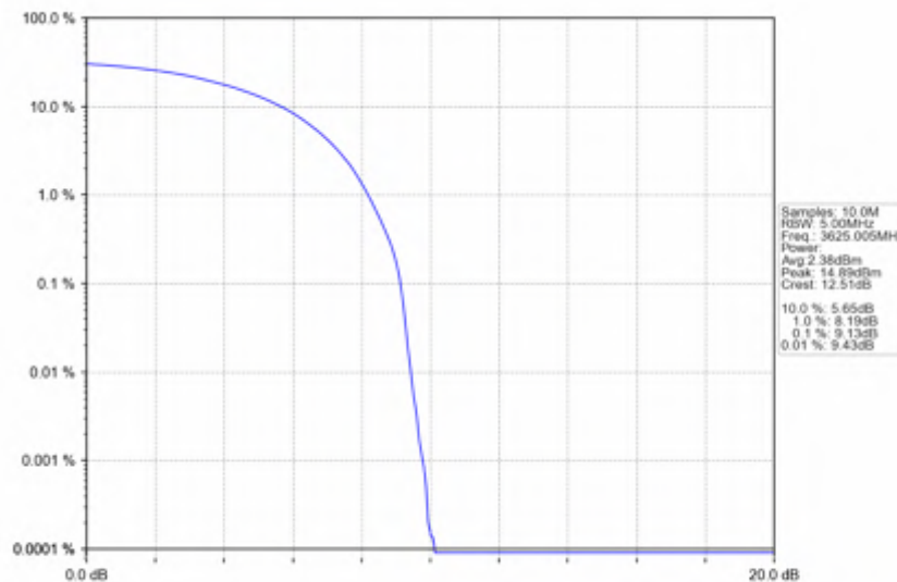
n78d_15kHz_SISO_NTNV_10MHz_DFT-s-OFDM QPSK_3625.005MHz_Outer_Full
