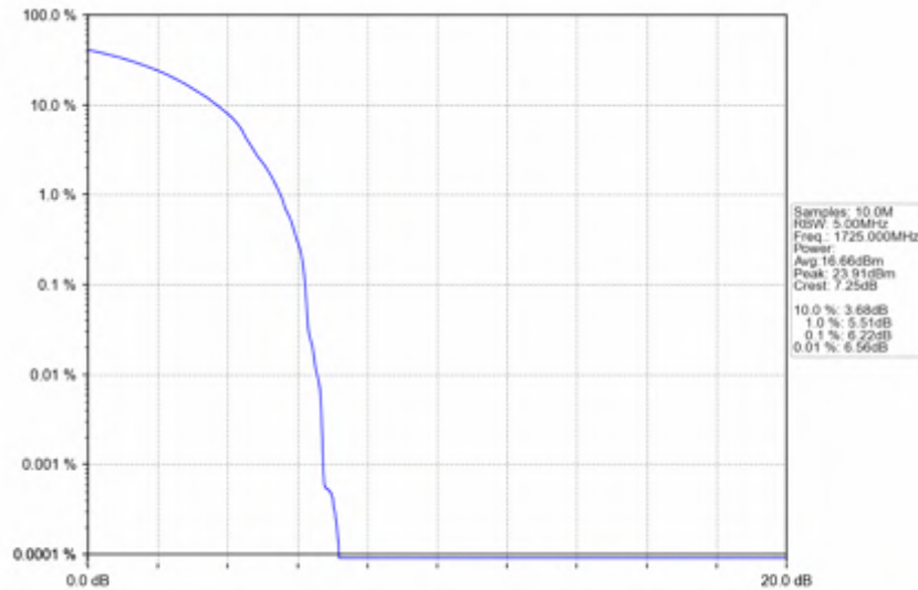
n66 30kHz SISO NTNV 30MHz DFT-s-OFDM PI/2 BPSK 1725MHz Outer Full
