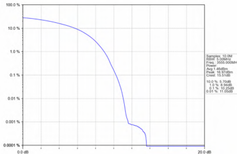
n78d_15kHz_SISO_NTNV_10MHz_DFT-s-OFDM_16_QAM_3555MHz_Outer_Full
