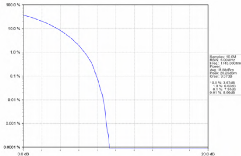
n66_30kHz_SISO_NTNV_10MHz_CP-OFDM QPSK_1745MHz_Outer_Full
