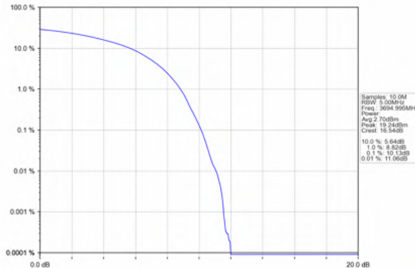
n78d_15kHz_SISO_NTNV_10MHz_DFT-s-OFDM 64 QAM_3694.995MHz_Outer_Full
