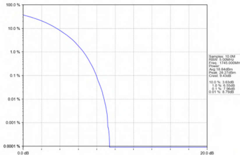
n66_30kHz_SISO_NTNV_10MHz_CP-OFDM_16_QAM_1745MHz_Outer_Full
