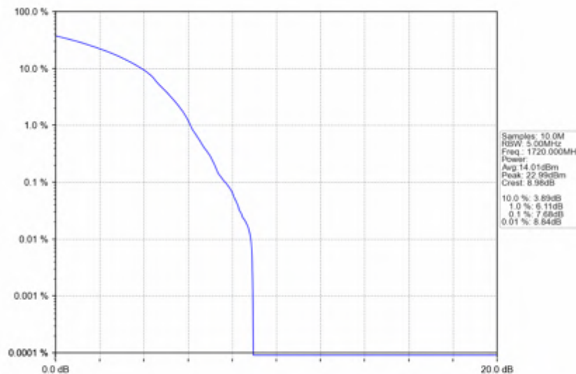
n66_15kHz_SISO_NTNV_20MHz_DFT-s-OFDM_256_QAM_1720MHz_Outer_Full
