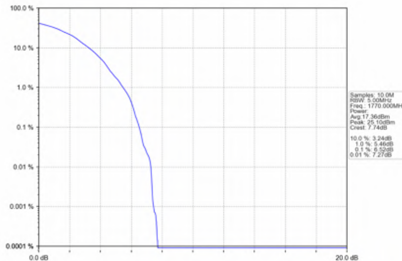
n66_30kHz_SISO_NTNV_20MHz_DFT-s-OFDM_QPSK_1770MHz_Outer_Full
