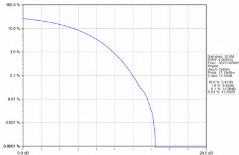
n78d_15kHz_SISO_NTNV_15MHz_CP-OFDM 64 QAM_3625.005MHz_Outer_Full
