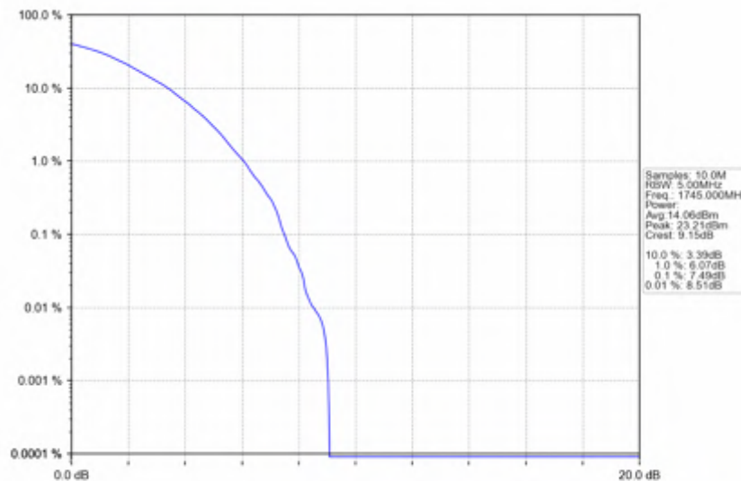
n66_30kHz_SISO_NTNV_40MHz_DFT-s-OFDM QPSK_1745MHz_Outer_Full
