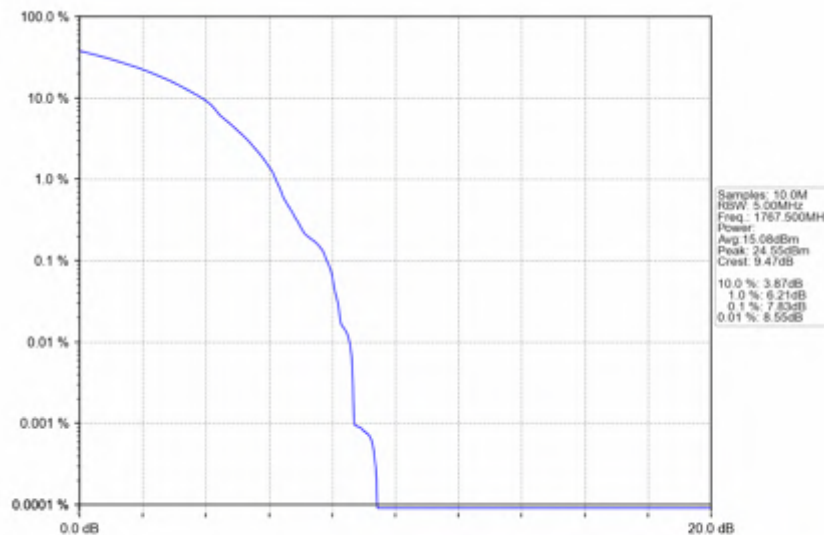
n66_30kHz_SISO_NTNV_25MHz_DFT-s-OFDM_64_QAM_1767.5MHz_Outer_Full
