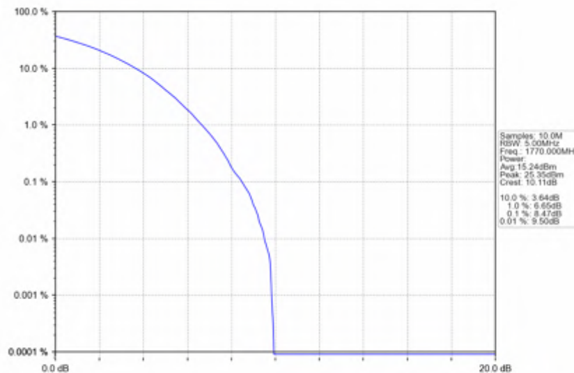
n66_15kHz_SISO_NTNV_20MHz_CP-OFDM QPSK_1770MHz_Outer_Full
