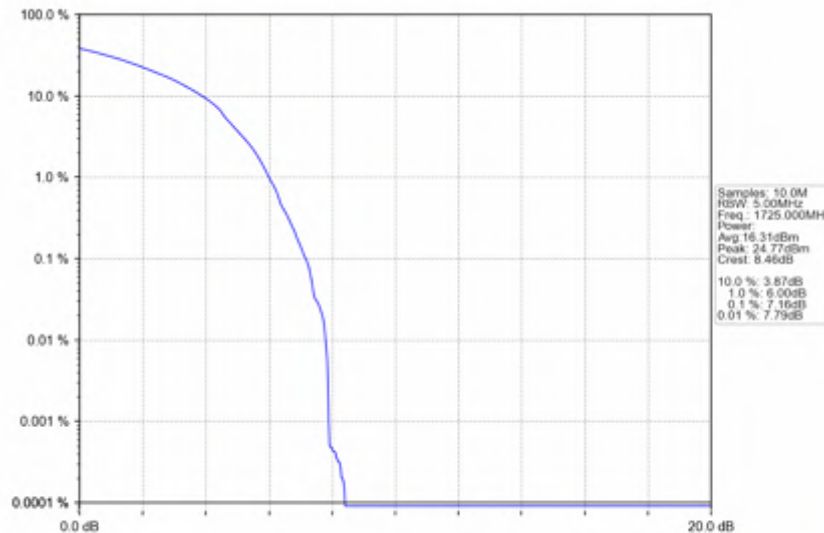
n66_30kHz_SISO_NTNV_30MHz_DFT-s-OFDM_QPSK_1725MHz_Outer_Full
