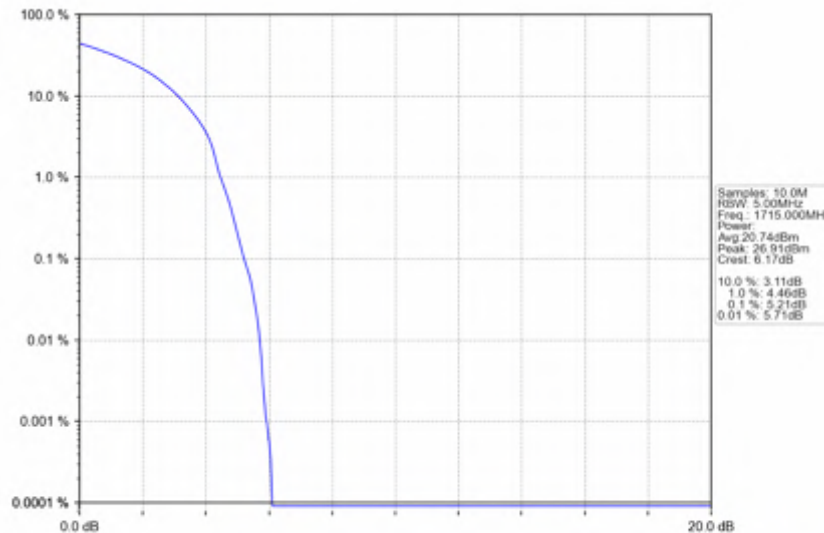
n66_30kHz_SISO_NTNV_10MHz_DFT-s-OFDM QPSK_1715MHz_Outer_Full
