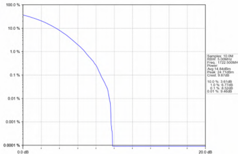
n66_30kHz_SISO_NTNV_25MHz_CP-OFDM_16_QAM_1722.5MHz_Outer_Full
