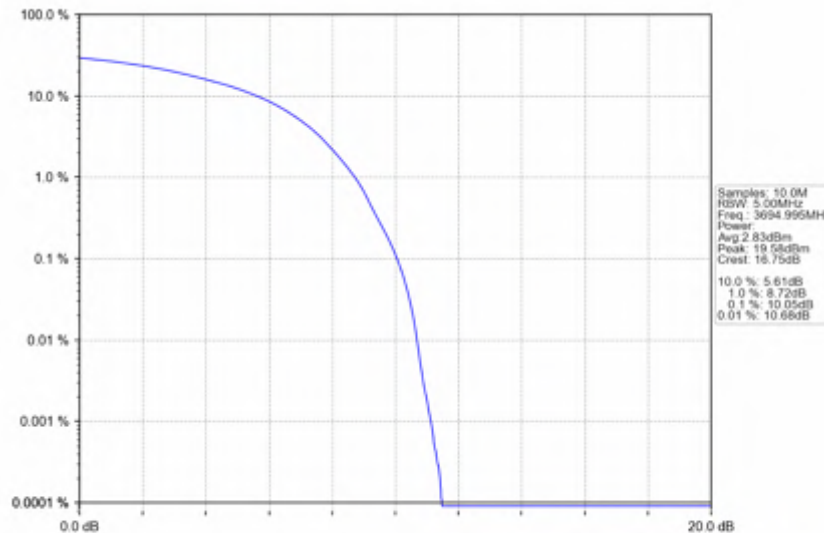
n78d_15kHz_SISO_NTNV_10MHz_DFT-s-OFDM_16_QAM_3694.995MHz_Outer_Full
