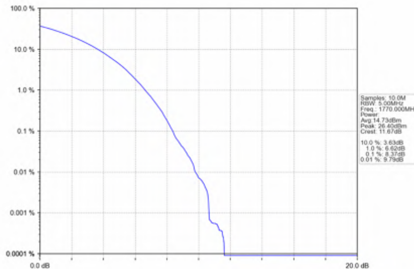
n66_15kHz_SISO_NTNV_20MHz_CP-OFDM 64 QAM_1770MHz_Outer_Full
