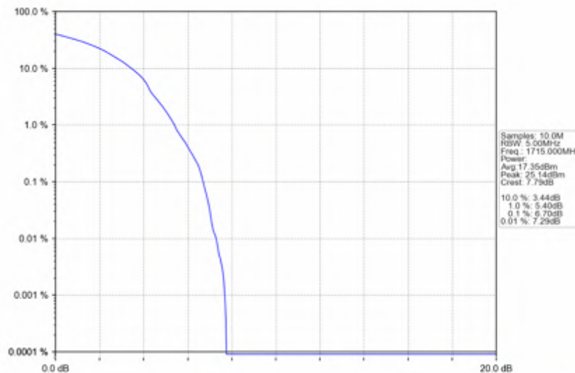
n66_30kHz_SISO_NTNV_10MHz_DFT-s-OFDM_256_QAM_1715MHz_Outer_Full
