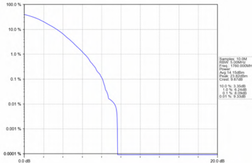
n66_30kHz_SISO_NTNV_40MHz_DFT-s-OFDM_16_QAM_1760MHz_Outer_Full
