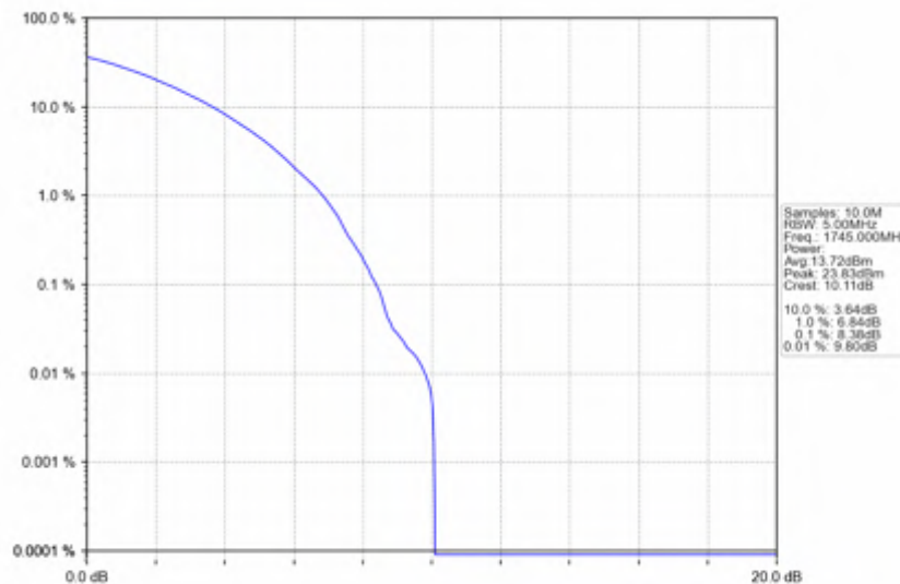
n66_30kHz_SISO_NTNV_25MHz_CP-OFDM 64 QAM_1745MHz_Outer_Full
