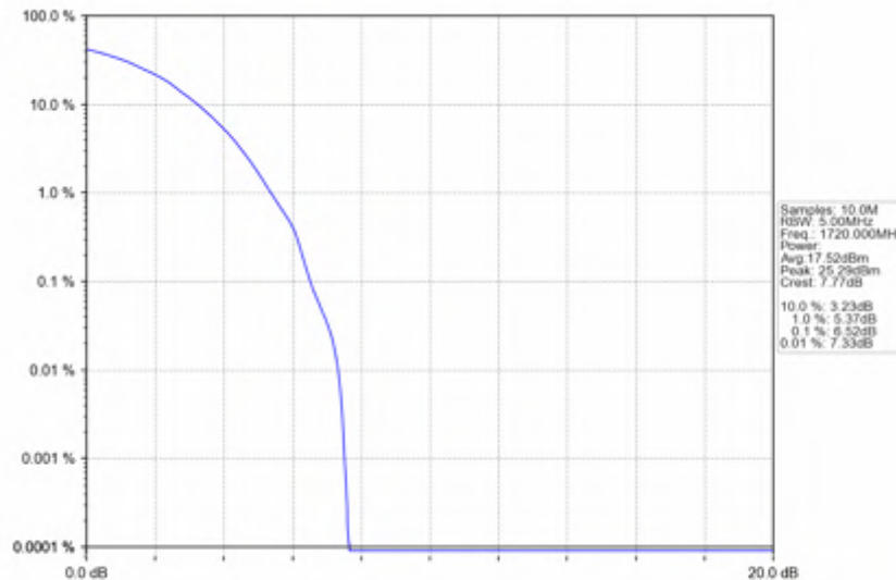
n66_30kHz_SISO_NTNV_20MHz_DFT-s-OFDM QPSK_1720MHz_Outer_Full
