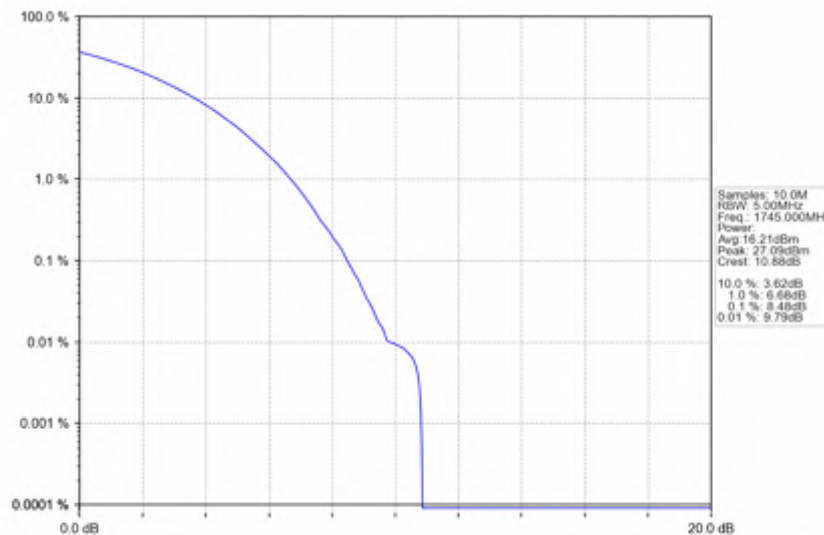
n66_30kHz_SISO_NTNV_15MHz_CP-OFDM_64_QAM_1745MHz_Outer_Full
