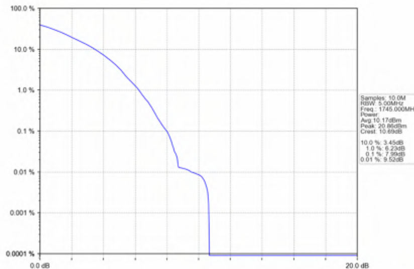
n66_15kHz_SISO_NTNV_40MHz_DFT-s-OFDM_256_QAM_1745MHz_Outer_Full
