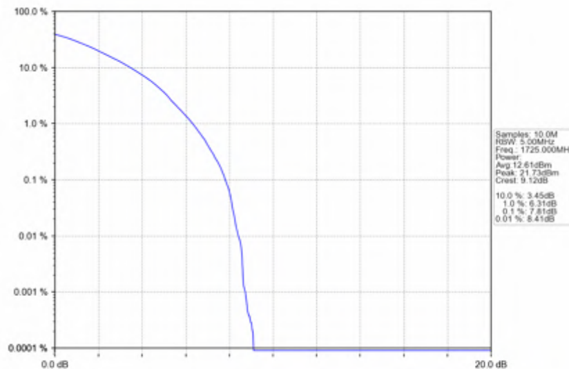
n66_15kHz_SISO_NTNV_30MHz_DFT-s-OFDM_256_QAM_1725MHz_Outer_Full
