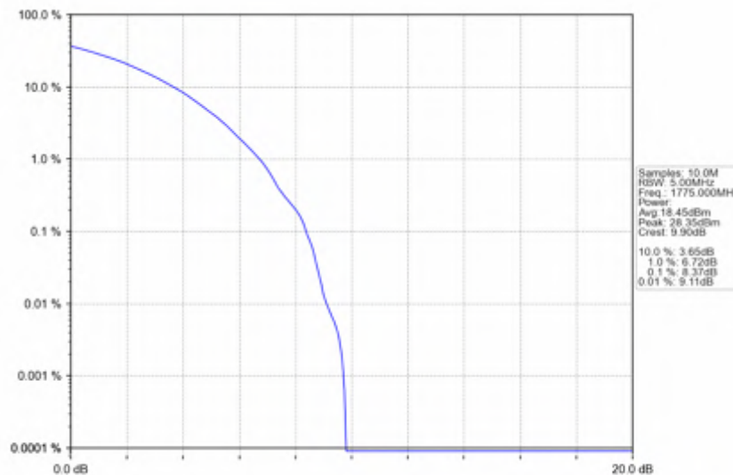
n66_30kHz_SISO_NTNV_10MHz_CP-OFDM 64 QAM_1775MHz_Outer_Full
