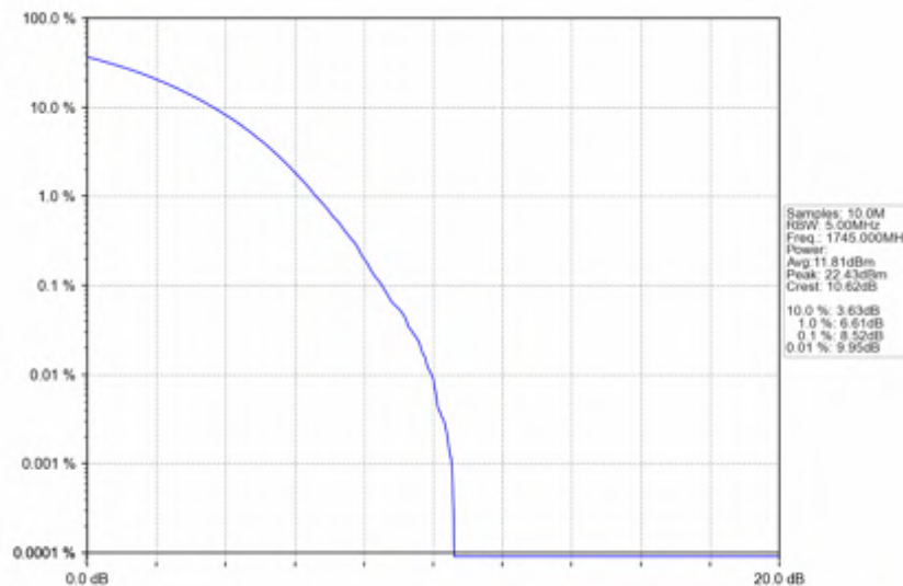
n66_15kHz_SISO_NTNV_40MHz_CP-OFDM_16_QAM_1745MHz_Outer_Full
