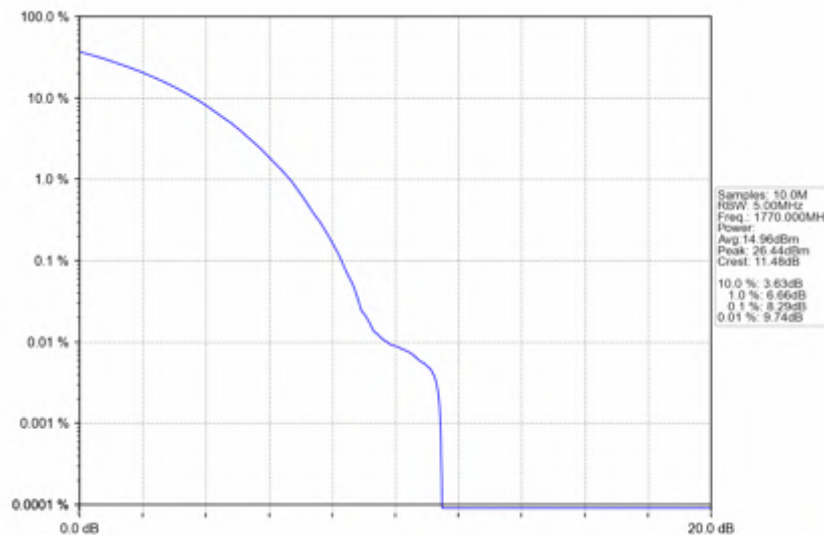
n66_30kHz_SISO_NTNV_20MHz_CP-OFDM 64 QAM_1770MHz_Outer_Full
