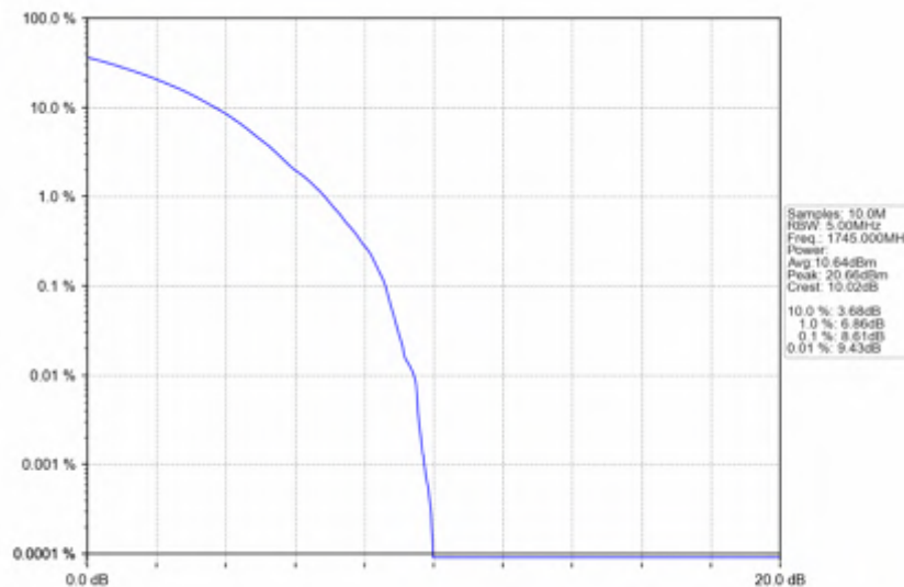
n66_30kHz_SISO_NTNV_25MHz_CP-OFDM_256_QAM_1745MHz_Outer_Full
