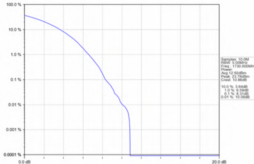
n66_15kHz_SISO_NTNV_40MHz_CP-OFDM QPSK_1730MHz_Outer_Full
