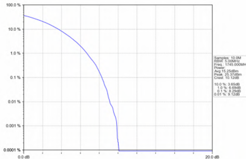
n66_15kHz_SISO_NTNV_20MHz_CP-OFDM_16_QAM_1745MHz_Outer_Full
