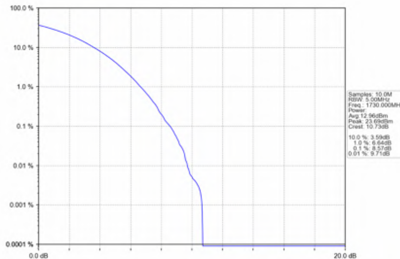
n66_15kHz_SISO_NTNV_40MHz_CP-OFDM_16_QAM_1730MHz_Outer_Full
