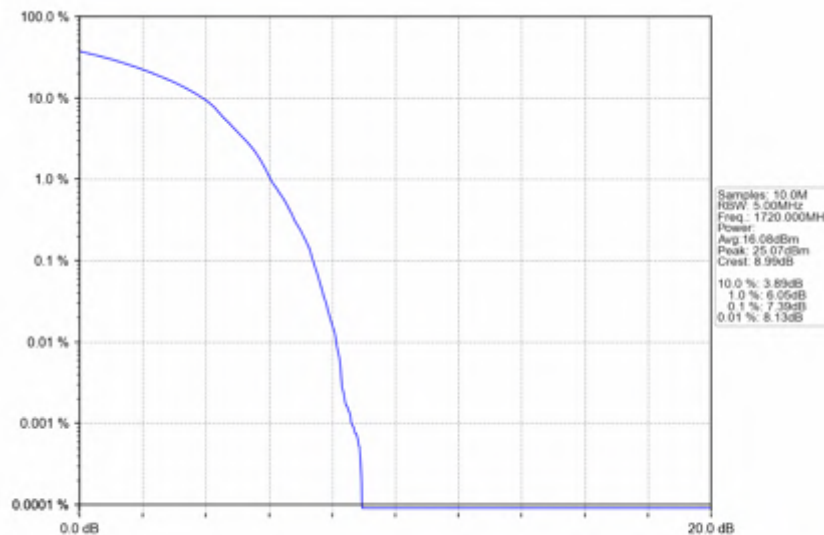
n66_15kHz_SISO_NTNV_20MHz_DFT-s-OFDM_64_QAM_1720MHz_Outer_Full
