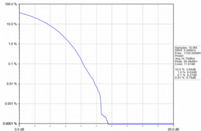
n66_15kHz_SISO_NTNV_20MHz_CP-OFDM 64 QAM_1720MHz_Outer_Full
