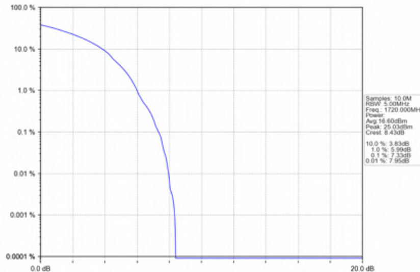
n66_15kHz_SISO_NTNV_20MHz_DFT-s-OFDM_16_QAM_1720MHz_Outer_Full
