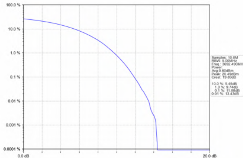
n78d_15kHz_SISO_NTNV_15MHz_CP-OFDM 64 QAM_3692.49MHz_Outer_Full
