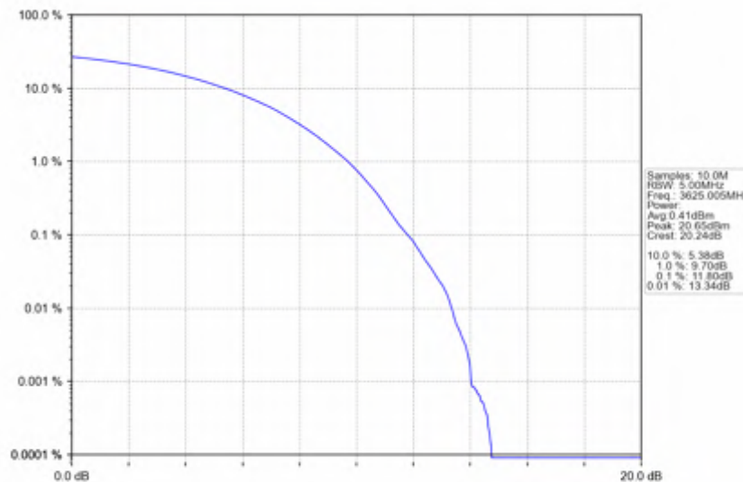
n78d_15kHz_SISO_NTNV_15MHz_CP-OFDM QPSK_3625.005MHz_Outer_Full
