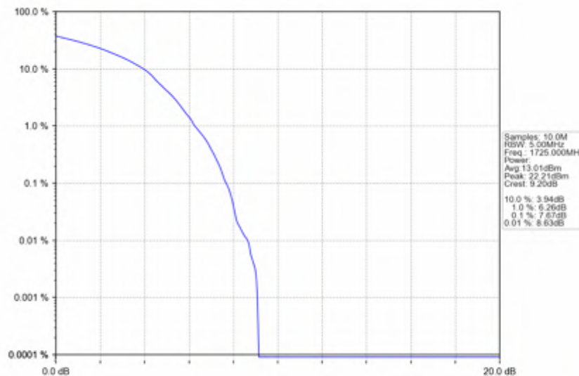
n66_30kHz_SISO_NTNV_30MHz_DFT-s-OFDM_256_QAM_1725MHz_Outer_Full
