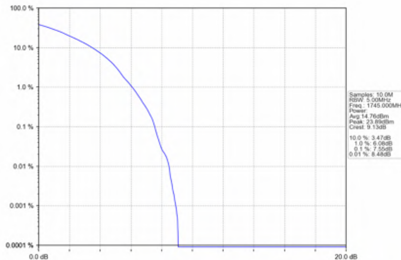
n66_15kHz_SISO_NTNV_25MHz_DFT-s-OFDM_64_QAM_1745MHz_Outer_Full
