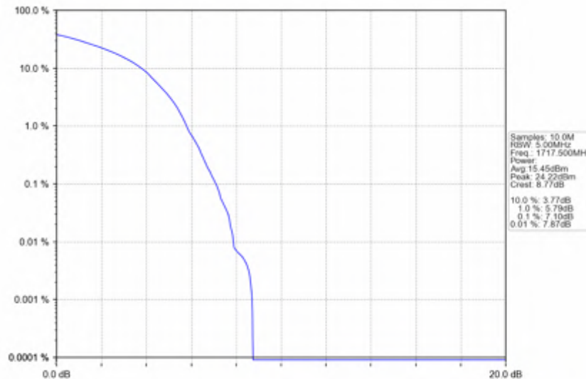
n66_30kHz_SISO_NTNV_15MHz_DFT-s-OFDM_256_QAM_1717.5MHz_Outer_Full
