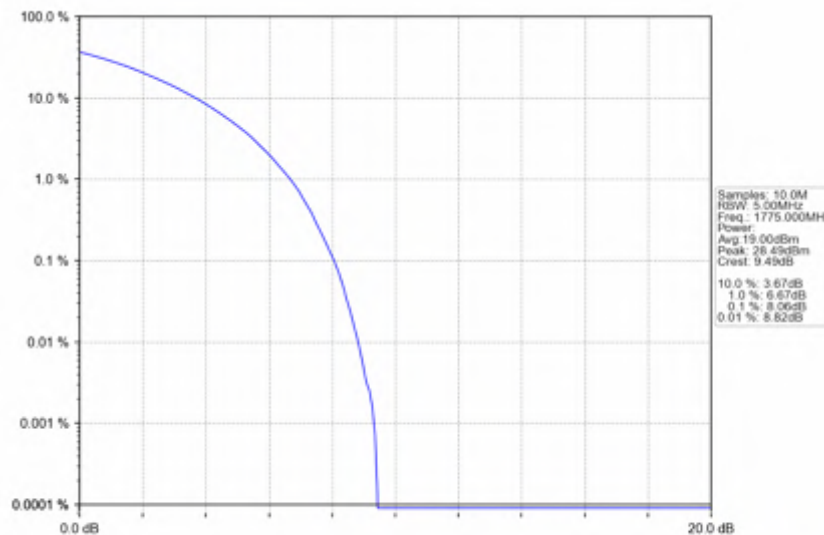
n66_30kHz_SISO_NTNV_10MHz_CP-OFDM QPSK_1775MHz_Outer_Full
