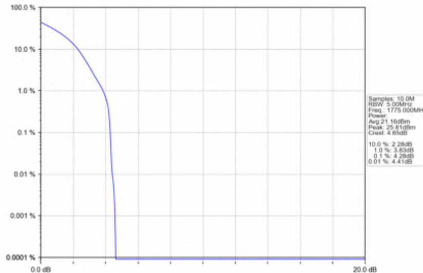
n66_30kHz_SISO_NTNV_10MHz_DFT-s-OFDM PI/2 BPSK_1775MHz_Outer_Full
