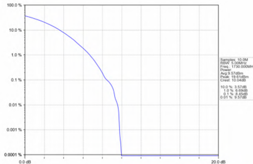
n66_30kHz_SISO_NTNV_40MHz_CP-OFDM 256 QAM_1730MHz_Outer_Full
