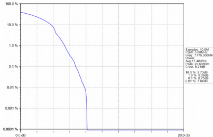
n66_30kHz_SISO_NTNV_10MHz_DFT-s-OFDM 256 QAM_1775MHz_Outer_Full
