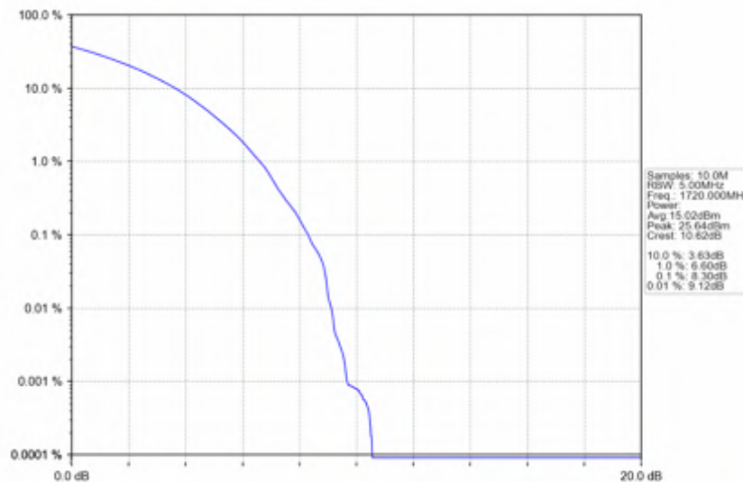
n66_30kHz_SISO_NTNV_20MHz_CP-OFDM 64 QAM_1720MHz_Outer_Full
