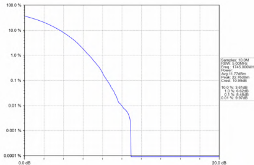
n66_15kHz_SISO_NTNV_40MHz_CP-OFDM QPSK_1745MHz_Outer_Full
