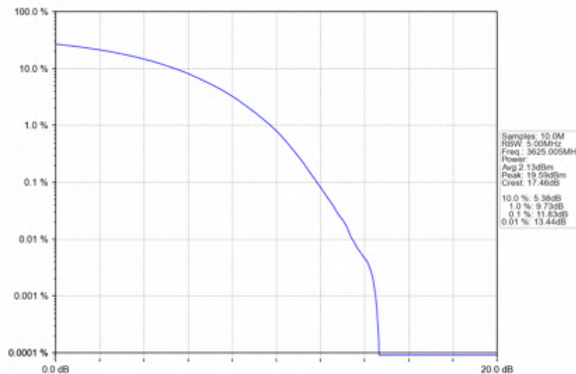
n78d_15kHz_SISO_NTNV_10MHz_CP-OFDM_256_QAM_3625.005MHz_Outer_Full
