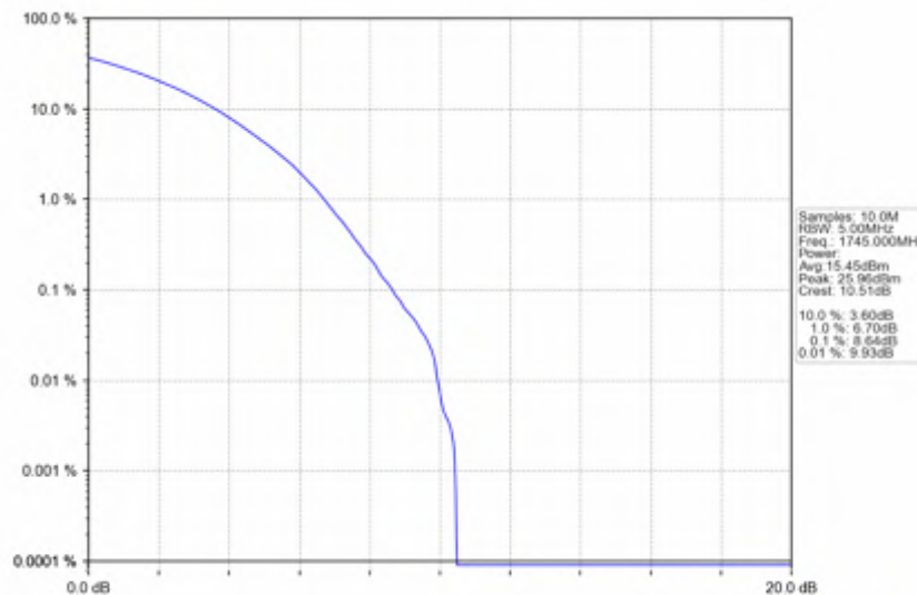
n66_30kHz_SISO_NTNV_20MHz_CP-OFDM_16_QAM_1745MHz_Outer_Full
