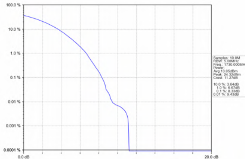
n66_30kHz_SISO_NTNV_40MHz_CP-OFDM QPSK_1730MHz_Outer_Full
