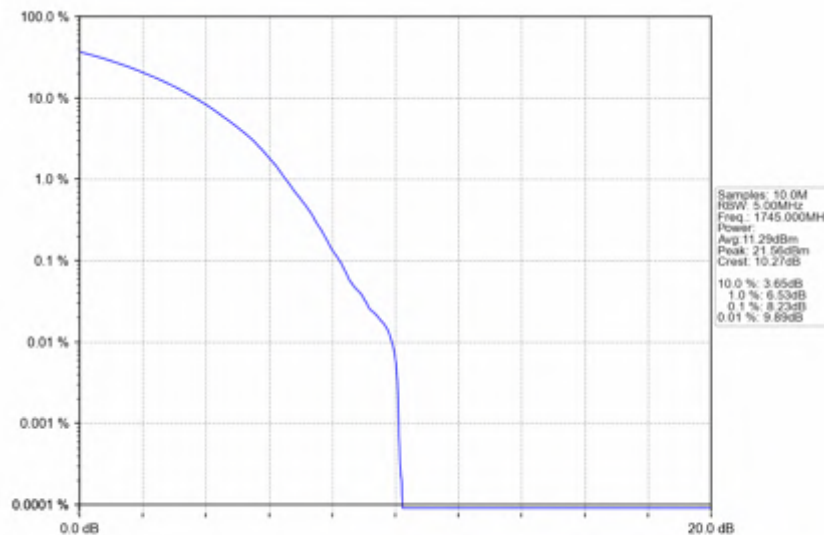
n66_15kHz_SISO_NTNV_40MHz_CP-OFDM 64 QAM_1745MHz_Outer_Full
