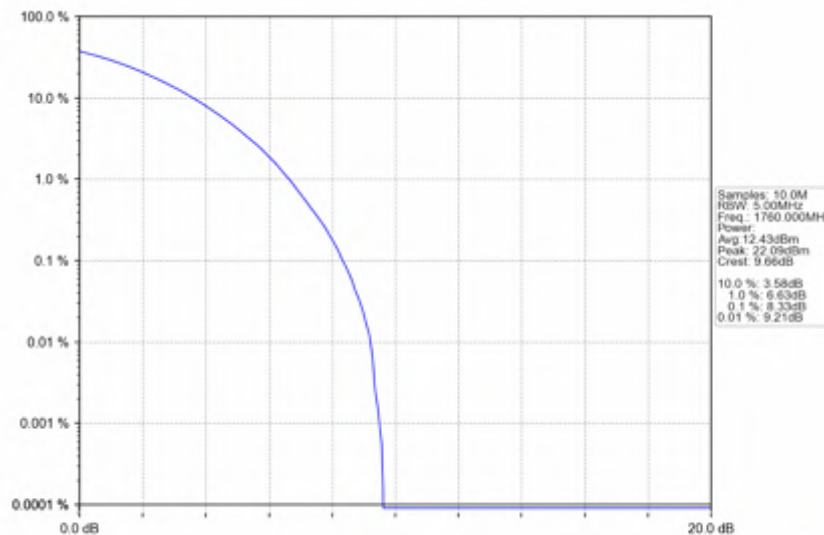
n66_30kHz_SISO_NTNV_40MHz_CP-OFDM_64_QAM_1760MHz_Outer_Full
