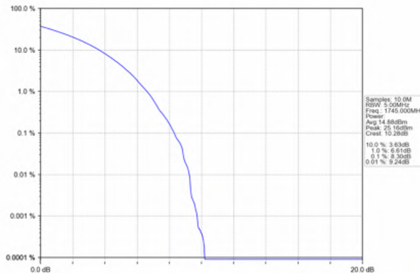
n66_30kHz_SISO_NTNV_20MHz_CP-OFDM 64 QAM_1745MHz_Outer_Full
