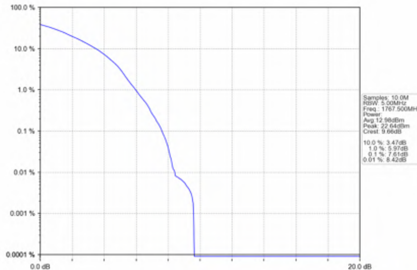
n66_15kHz_SISO_NTNV_25MHz_DFT-s-OFDM_256_QAM_1767.5MHz_Outer_Full
