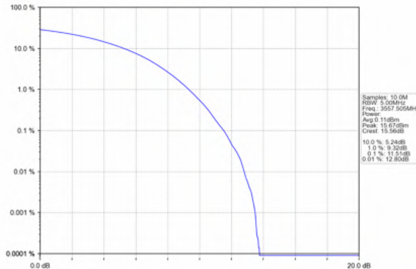
n78d_15kHz_SISO_NTNV_15MHz_CP-OFDM_QPSK_3557.505MHz_Outer_Full
