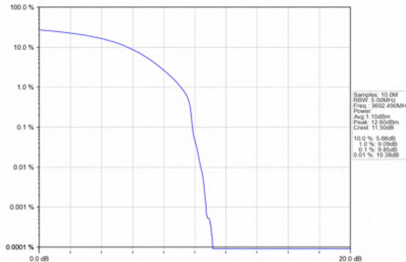
n78d_15kHz_SISO_NTNV_15MHz_DFT-s-OFDM QPSK_3692.49MHz_Outer_Full
