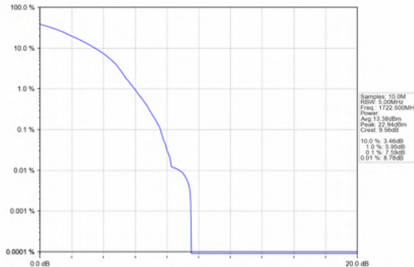
n66_15kHz_SISO_NTNV_25MHz_DFT-s-OFDM_256_QAM_1722.5MHz_Outer_Full
