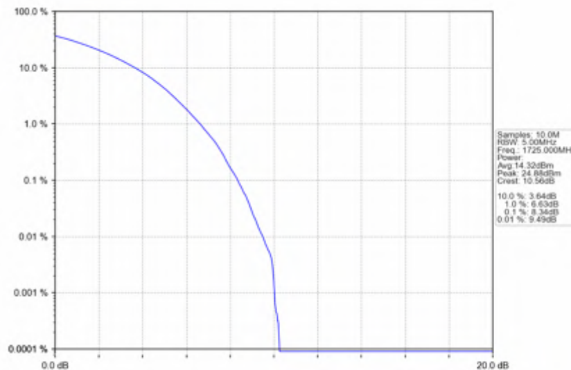
n66_30kHz_SISO_NTNV_30MHz_CP-OFDM_16_QAM_1725MHz_Outer_Full
