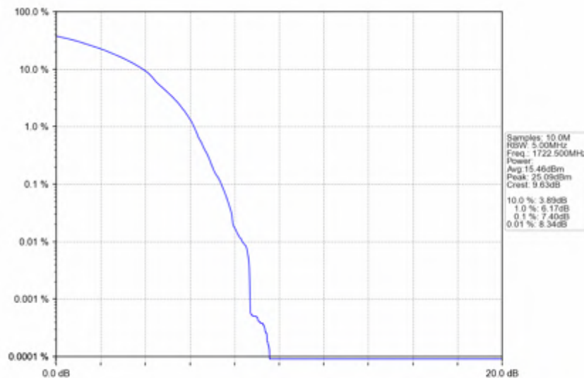
n66_30kHz_SISO_NTV_25MHz_DFT-s-OFDM_64_QAM_1722.5MHz_Outer_Full
