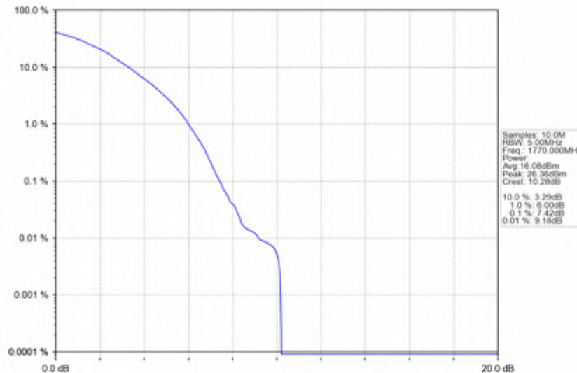
n66_30kHz_SISO_NTNV_20MHz_DFT-s-OFDM_64_QAM_1770MHz_Outer_Full
