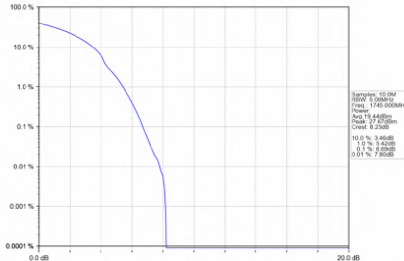
n66_30kHz_SISO_NTNV_10MHz_DFT-s-OFDM_64_QAM_1745MHz_Outer_Full
