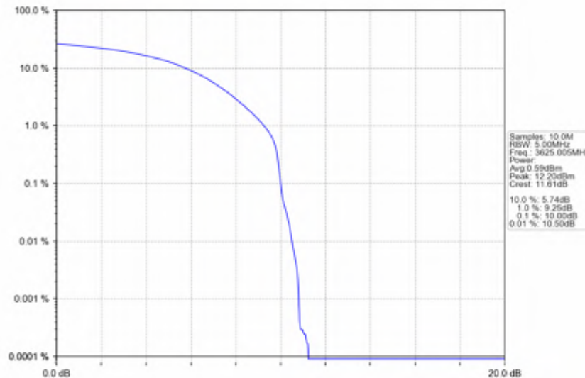
n78d_15kHz_SISO_NTNV_15MHz_DFT-s-OFDM QPSK_3625.005MHz_Outer_Full
