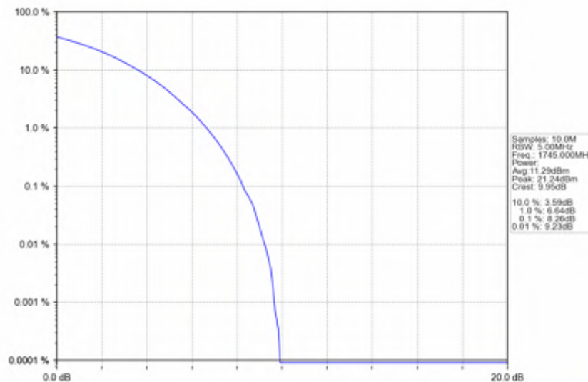
n66_30kHz_SISO_NTNV_40MHz_CP-OFDM_64_QAM_1745MHz_Outer_Full
