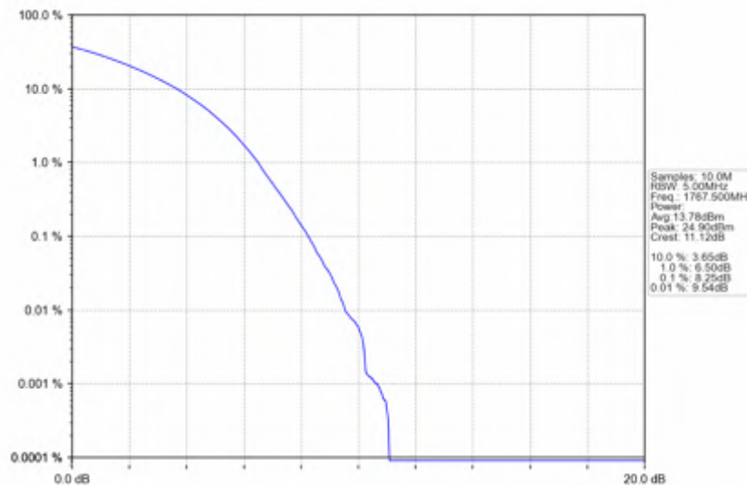
n66_15kHz_SISO_NTNV_25MHz_CP-OFDM 64 QAM_1767.5MHz_Outer_Full
