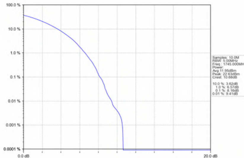
n66_30kHz_SISO_NTNV_40MHz_CP-OFDM_16_QAM_1745MHz_Outer_Full
