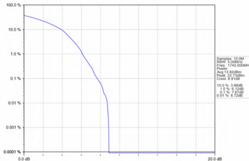
n66_15kHz_SISO_NTNV_20MHz_DFT-s-OFDM_256_QAM_1745MHz_Outer_Full
