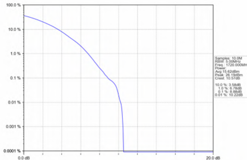
n66_30kHz_SISO_NTNV_20MHz_CP-OFDM_16_QAM_1720MHz_Outer_Full
