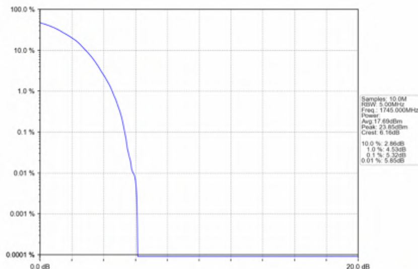
n66 30kHz SISO NTV 20MHz DFT-s-OFDM PI/2 BPSK 1745MHz Outer Full
