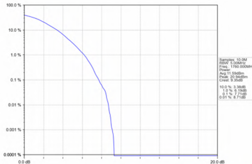
n66_30kHz_SISO_NTNV_40MHz_DFT-s-OFDM 256 QAM_1760MHz_Outer_Full
