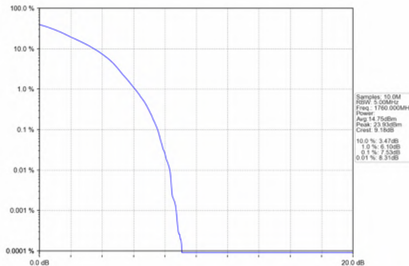
n66_15kHz_SISO_NTNV_40MHz_DFT-s-OFDM QPSK_1760MHz_Outer_Full
