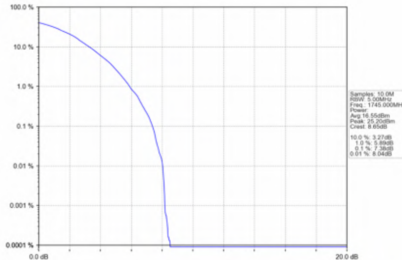
n66_30kHz_SISO_NTNV_20MHz_DFT-s-OFDM_16_QAM_1745MHz_Outer_Full
