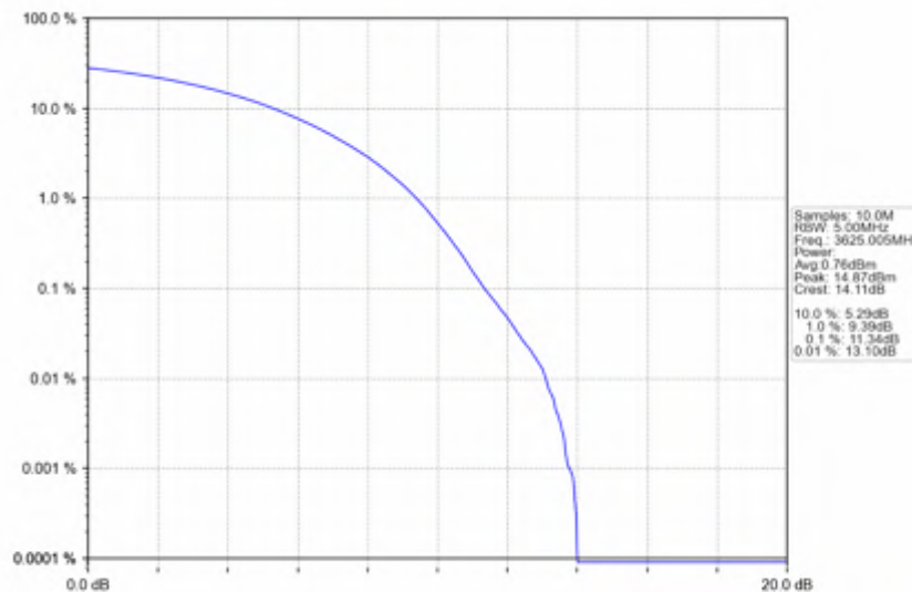
n78d_15kHz_SISO_NTNV_15MHz_CP-OFDM_256_QAM_3625.005MHz_Outer_Full
