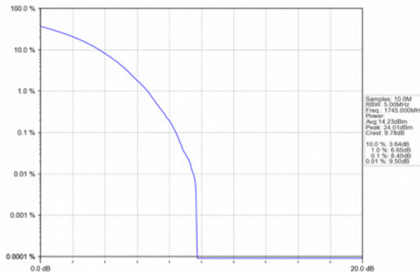
n66_30kHz_SISO_NTNV_25MHz_CP-OFDM_16_QAM_1745MHz_Outer_Full
