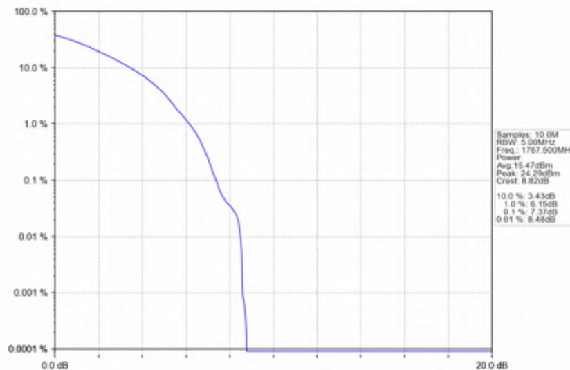
n66_15kHz_SISO_NTV_25MHz_DFT-s-OFDM 16 QAM_1767.5MHz_Outer_Full
