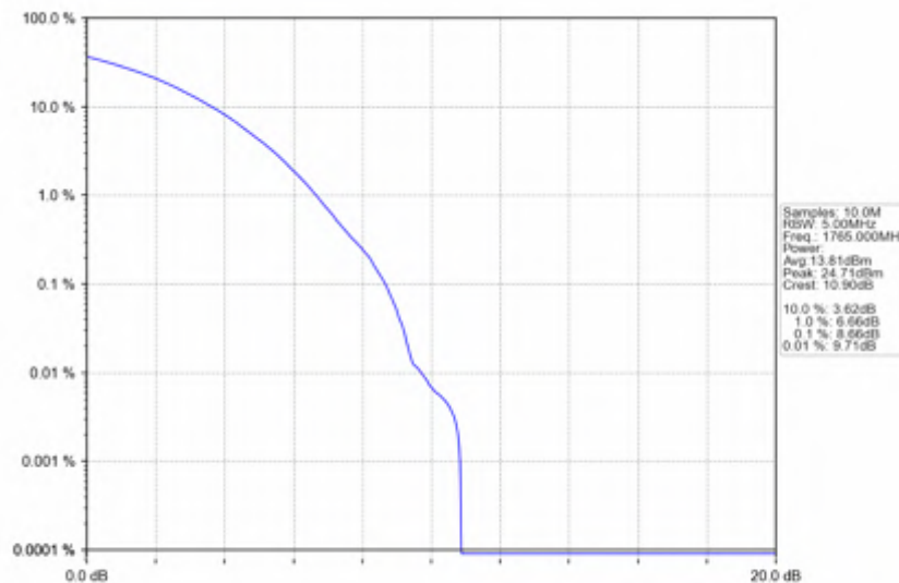
n66_15kHz_SISO_NTNV_30MHz_CP-OFDM QPSK_1765MHz_Outer_Full
