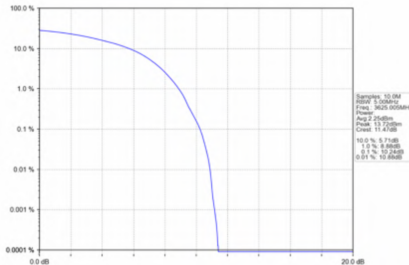
n78d_15kHz_SISO_NTNV_10MHz_DFT-s-OFDM_16_QAM_3625.005MHz_Outer_Full
