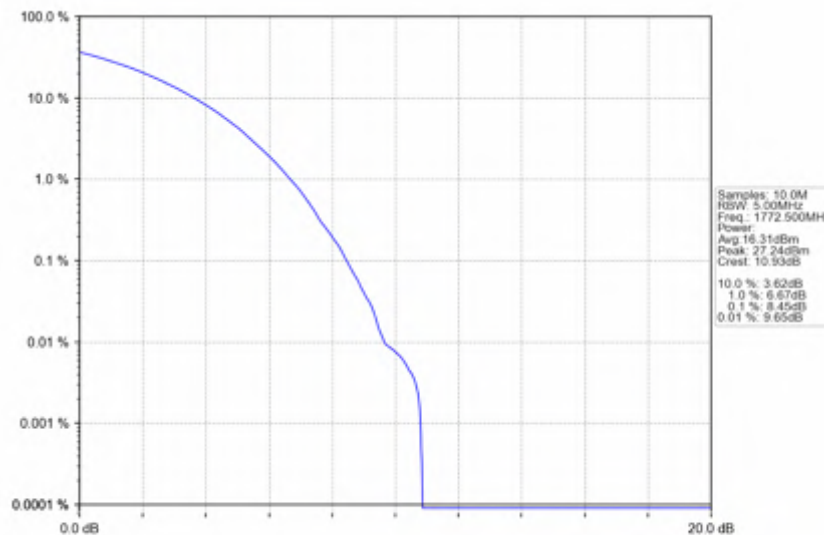
n66_30kHz_SISO_NTNV_15MHz_CP-OFDM_64_QAM_1772.5MHz_Outer_Full
