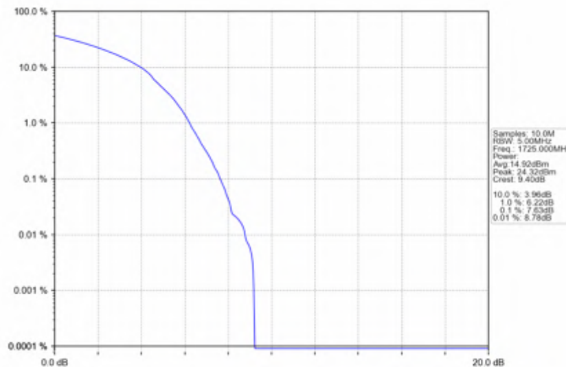
n66_30kHz_SISO_NTNV_30MHz_DFT-s-OFDM_64_QAM_1725MHz_Outer_Full
