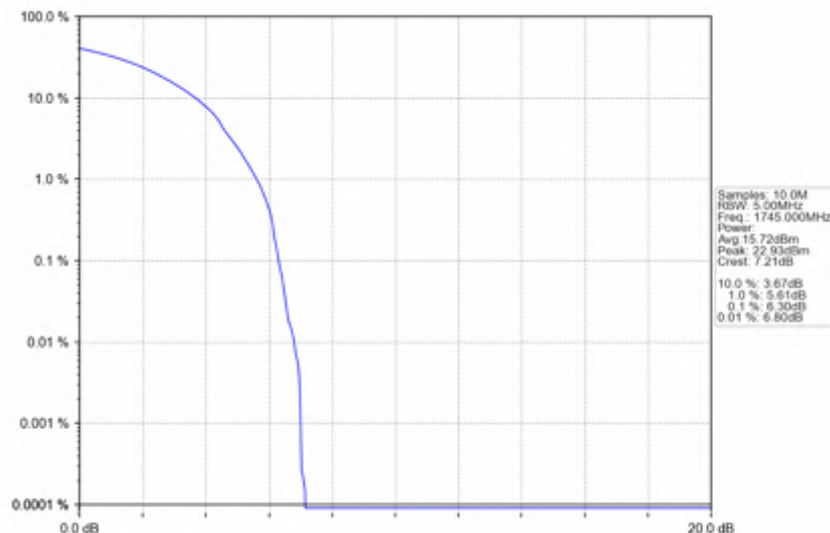
n66 30kHz SISO NTNV 30MHz DFT-s-OFDM PI/2 BPSK 1745MHz Outer Full
