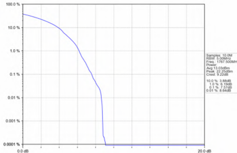
n66_30kHz_SISO_NTNV_25MHz_DFT-s-OFDM_256_QAM_1767.5MHz_Outer_Full
