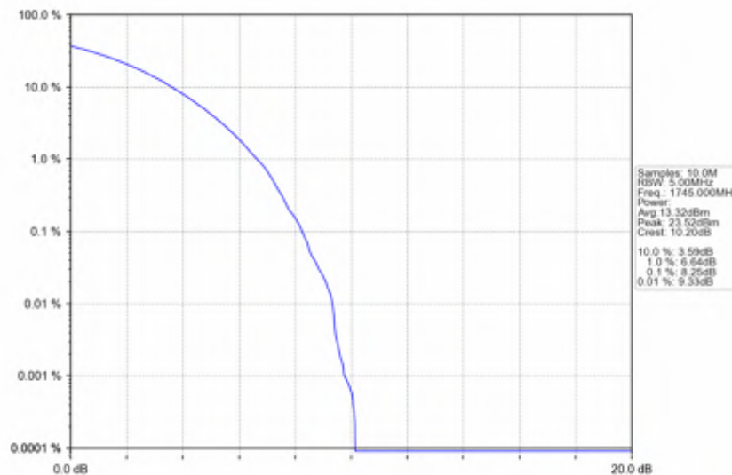
n66_30kHz_SISO_NTNV_30MHz_CP-OFDM_16_QAM_1745MHz_Outer_Full
