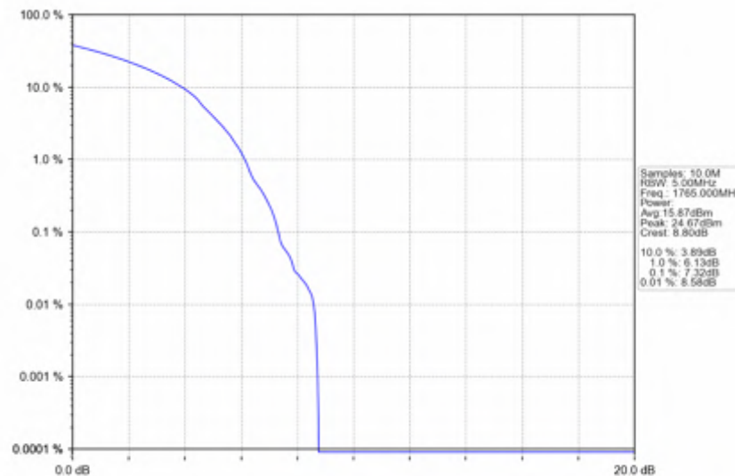
n66_30kHz_SISO_NTNV_30MHz_DFT-s-OFDM QPSK_1765MHz_Outer_Full
