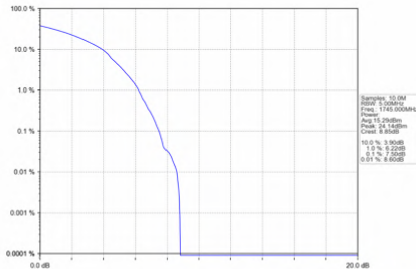
n66 30kHz SISO NTN 25MHz DFT-s-OFDM 16 QAM 1745MHz Outer Full
