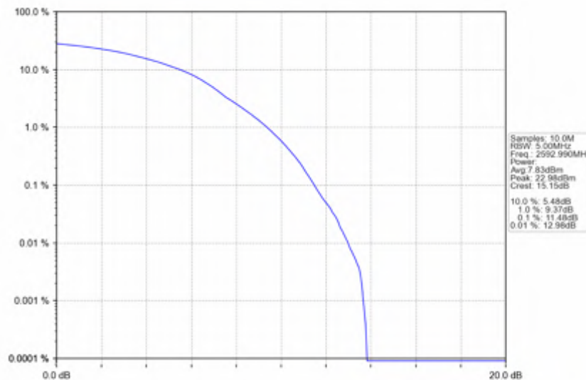
n41_30kHz_SISO_NTNV_60MHz_DFT-s-OFDM_16_QAM_2592.99MHz_Outer_Full
