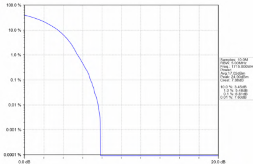
n66_15kHz_SISO_NTNV_10MHz_DFT-s-OFDM_256_QAM_1715MHz_Outer_Full
