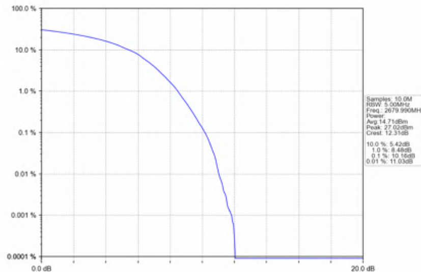
n41_30kHz_SISO_NTNV_20MHz_DFT-s-OFDM QPSK_2679.99MHz_Outer_Full
