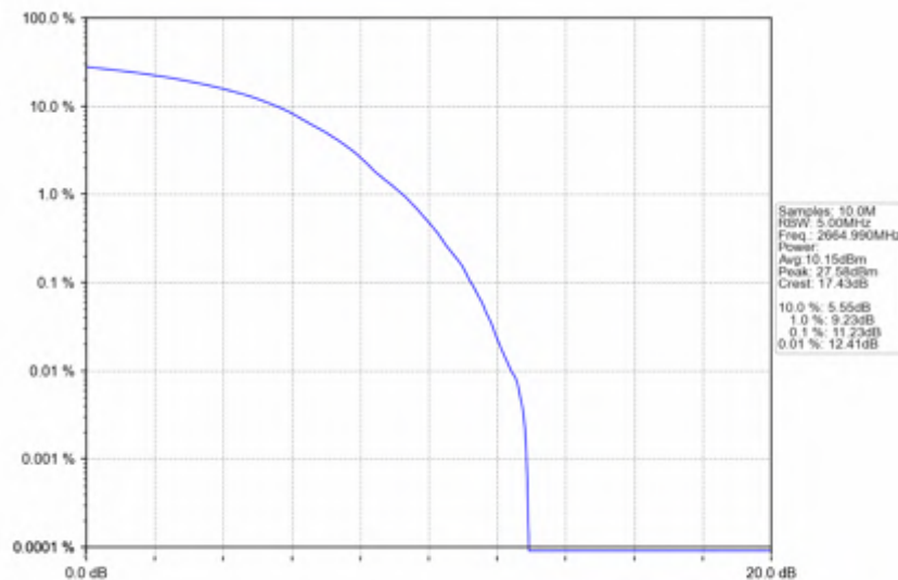
n41_30kHz_SISO_NTNV_50MHz_DFT-s-OFDM QPSK_2664.99MHz_Outer_Full
