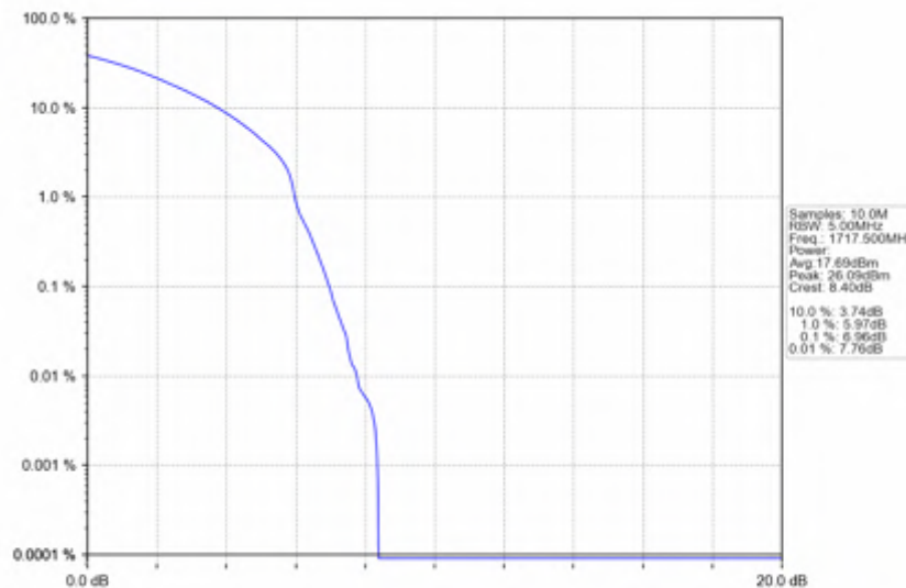
n66_15kHz_SISO_NTNV_15MHz_DFT-s-OFDM_16_QAM_1717.5MHz_Outer_Full
