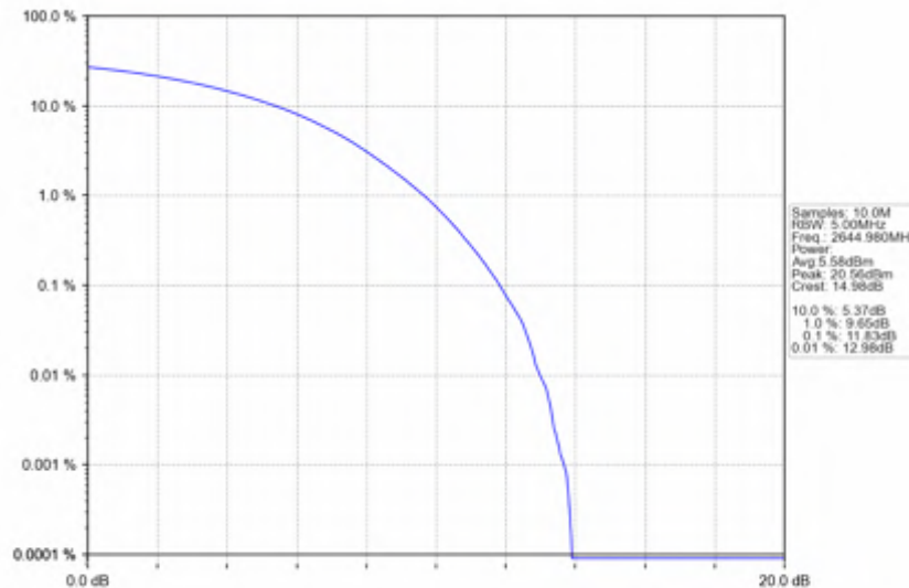
n41_30kHz_SISO_NTNV_90MHz_CP-OFDM_16_QAM_2644.98MHz_Outer_Full
