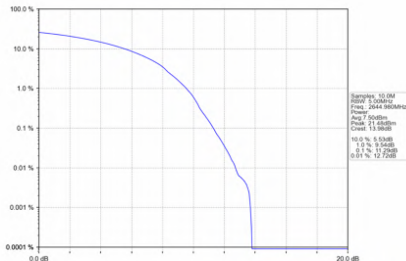
n41 30kHz SISO NTNV 90MHz DFT-s-OFDM QPSK 2644.98MHz Outer Full
