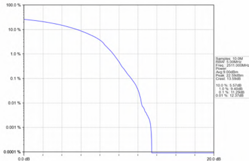
n41_30kHz_SISO_NTNV_30MHz_DFT-s-OFDM_256_QAM_2511MHz_Outer_Full
