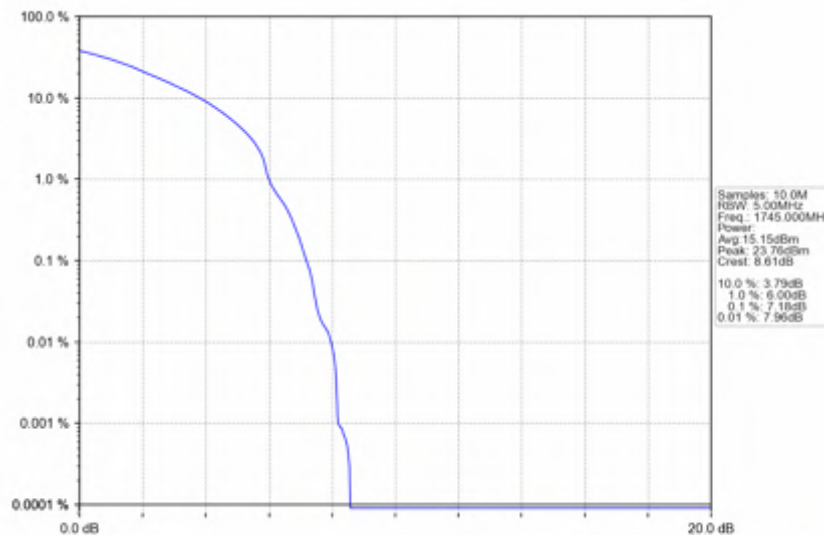
n66_15kHz_SISO_NTNV_15MHz_DFT-s-OFDM_256_QAM_1745MHz_Outer_Full
