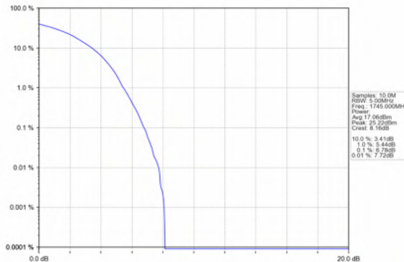
n66_15kHz_SISO_NTNV_10MHz_DFT-s-OFDM_256_QAM_1745MHz_Outer_Full
