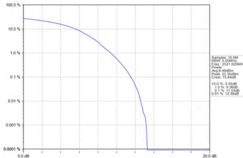
n41_30kHz_SISO_NTNV_50MHz_DFT-s-OFDM_256_QAM_2521.02MHz_Outer_Full
