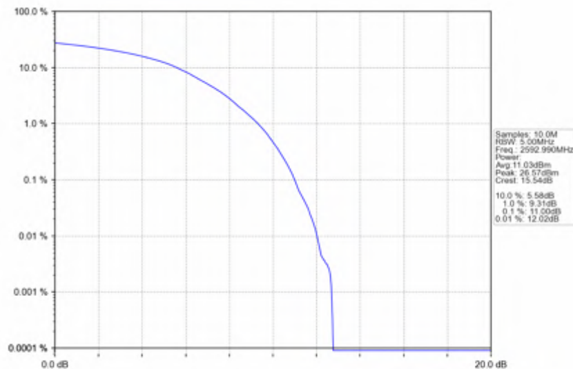
n41_30kHz_SISO_NTNV_40MHz_DFT-s-OFDM QPSK_2592.99MHz_Outer_Full
