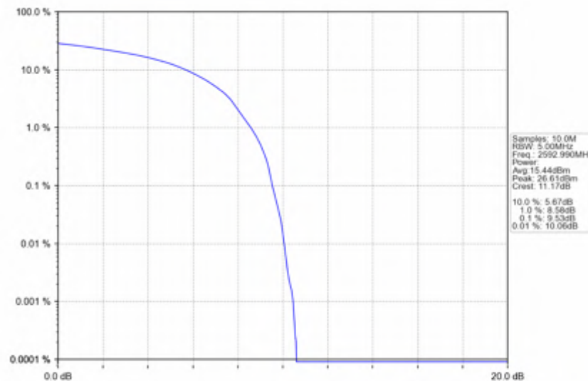
n41_30kHz_SISO_NTNV_15MHz_DFT-s-OFDM QPSK_2592.99MHz_Outer_Full
