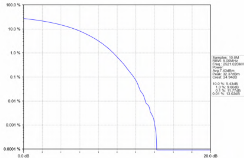
n41_30kHz_SISO_NTNV_50MHz_CP-OFDM_64_QAM_2521.02MHz_Outer_Full
