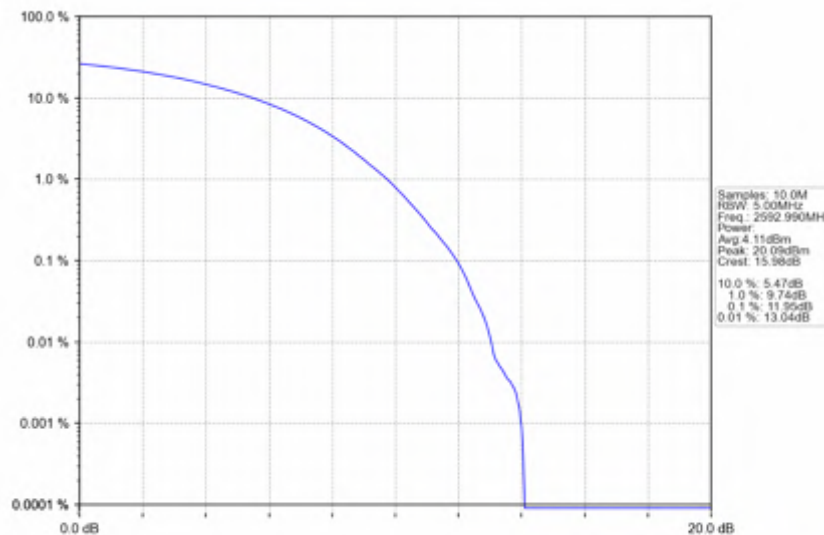
n41_30kHz_SISO_NTNV_100MHz_CP-OFDM QPSK_2592.99MHz_Outer_Full
