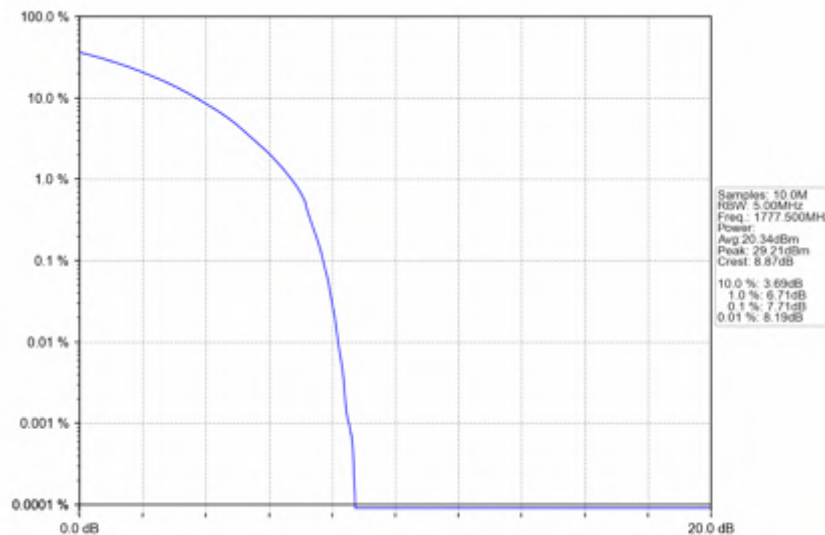
n66_15kHz_SISO_NTNV_5MHz_CP-OFDM QPSK_1777.5MHz_Outer_Full
