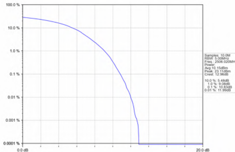
n41_30kHz_SISO_NTNV_20MHz_DFT-s-OFDM_256_QAM_2506.02MHz_Outer_Full
