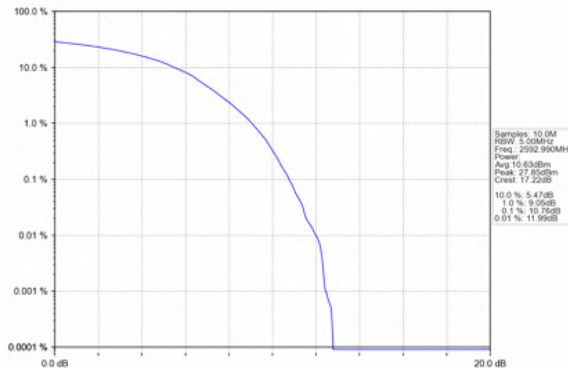
n41_30kHz_SISO_NTNV_20MHz_DFT-s-OFDM_256_QAM_2592.99MHz_Outer_Full
