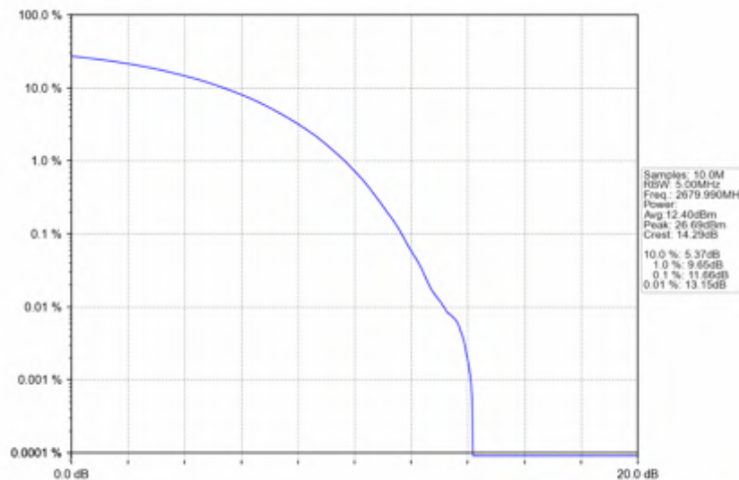
n41_30kHz_SISO_NTNV_20MHz_CP-OFDM_16_QAM_2679.99MHz_Outer_Full
