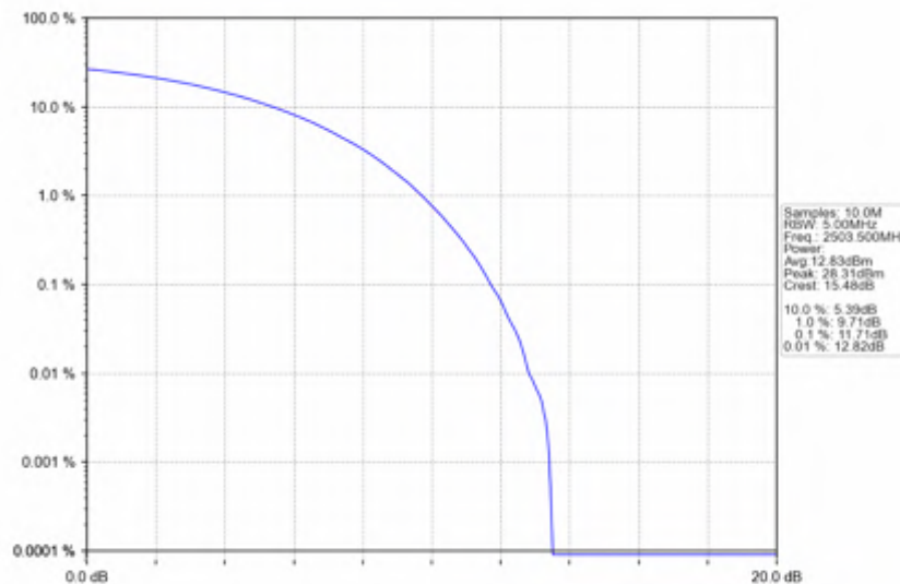
n41_30kHz_SISO_NTNV_15MHz_CP-OFDM QPSK_2503.5MHz_Outer_Full
