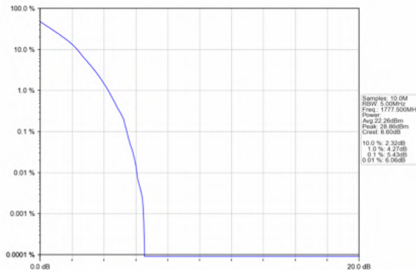
n66_15kHz_SISO_NTNV_5MHz_DFT-s-OFDM_QPSK_1777.5MHz_Outer_Full
