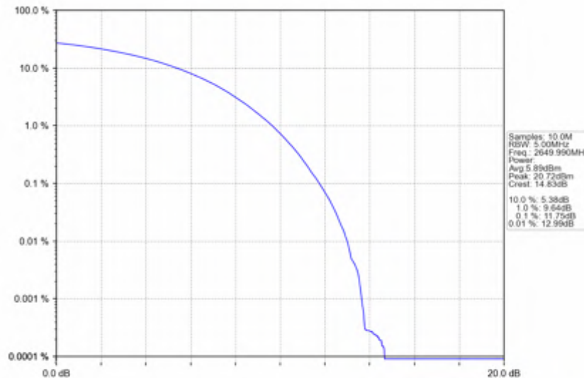
n41_30kHz_SISO_NTNV_80MHz_CP-OFDM_16_QAM_2649.99MHz_Outer_Full
