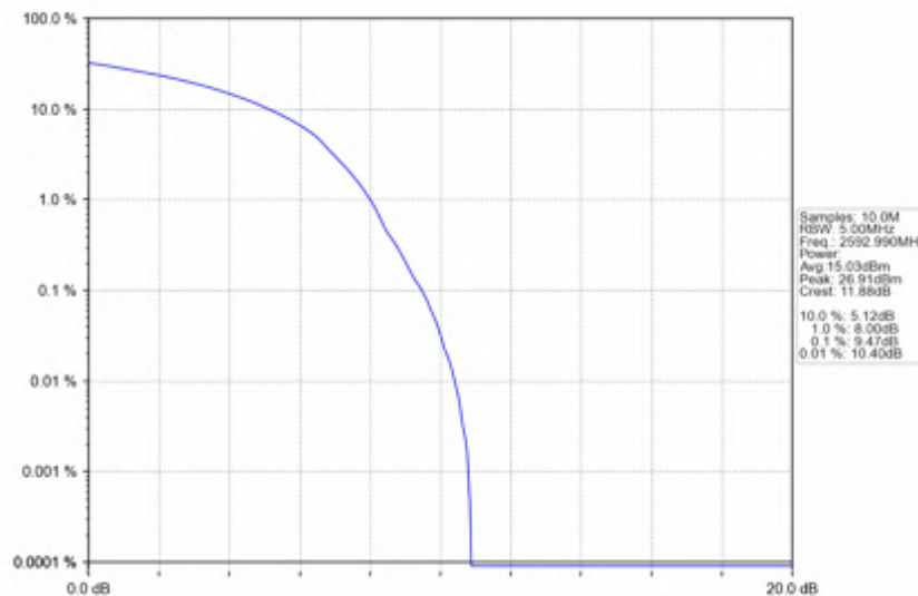
n41_30kHz_SISO_NTNV_15MHz_DFT-s-OFDM_64_QAM_2592.99MHz_Outer_Full
