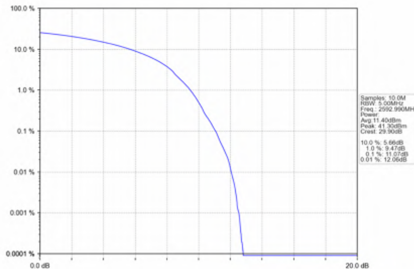
n41_30kHz_SISO_NTNV_30MHz_DFT-s-OFDM_16_QAM_2592.99MHz_Outer_Full
