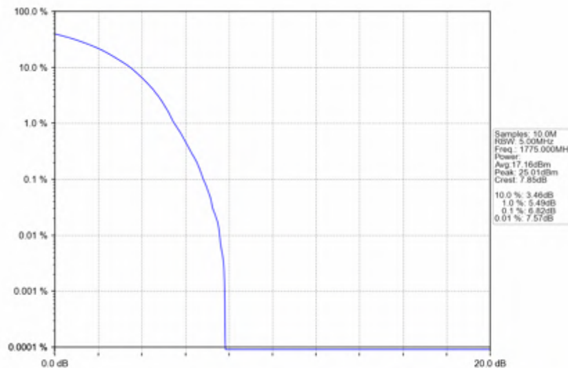
n66_15kHz_SISO_NTNV_10MHz_DFT-s-OFDM 256 QAM_1775MHz_Outer_Full
