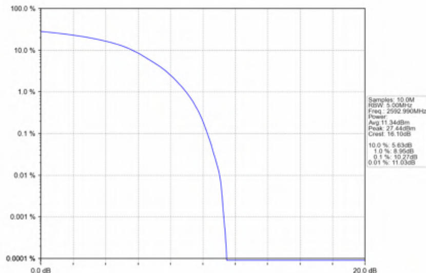
n41 30kHz SISO NTNV 40MHz DFT-s-OFDM PI/2 BPSK 2592.99MHz Outer Full
