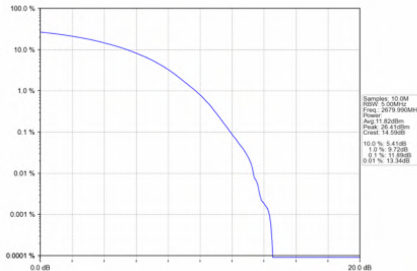
n41_30kHz_SISO_NTNV_20MHz_CP-OFDM 64 QAM_2679.99MHz_Outer_Full
