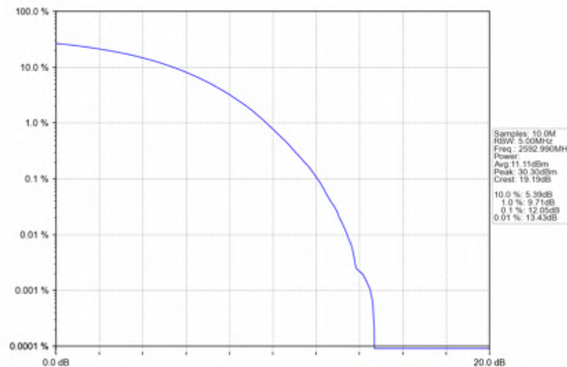
n41_30kHz_SISO_NTNV_10MHz_CP-OFDM 256 QAM_2592.99MHz_Outer_Full
