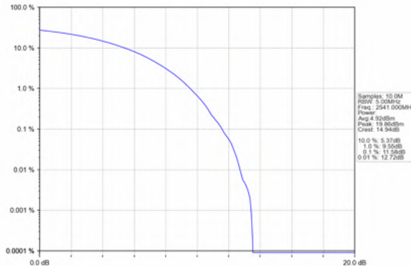
n41_30kHz_SISO_NTNV_90MHz_CP-OFDM_64_QAM_2541MHz_Outer_Full
