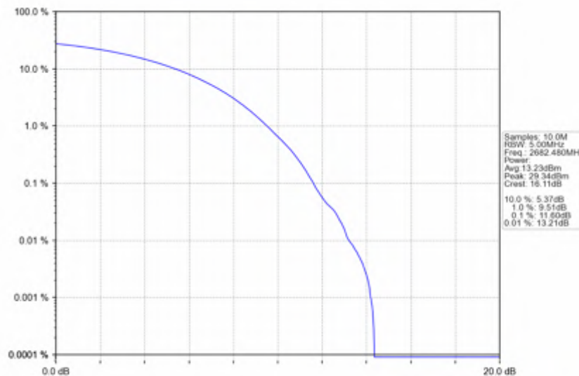
n41_30kHz_SISO_NTNV_15MHz_CP-OFDM_16_QAM_2682.48MHz_Outer_Full
