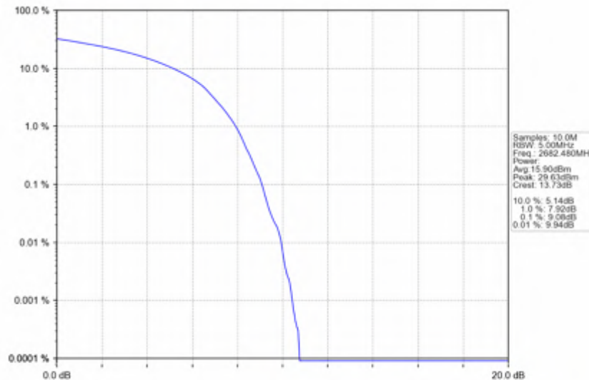
n41_30kHz_SISO_NTNV_15MHz_DFT-s-OFDM_16_QAM_2682.48MHz_Outer_Full
