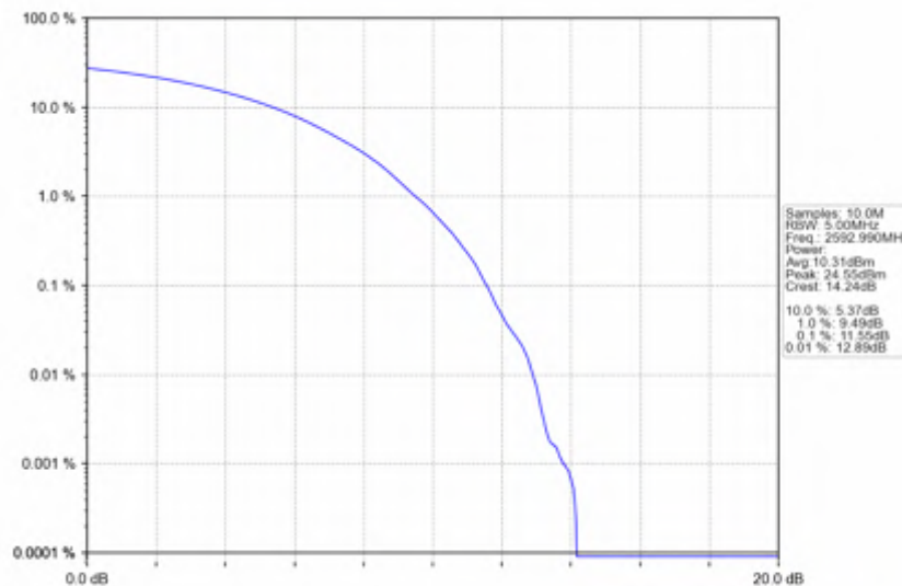
n41_30kHz_SISO_NTNV_30MHz_CP-OFDM_16_QAM_2592.99MHz_Outer_Full
