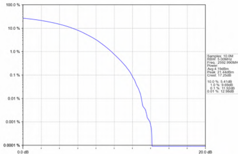
n41_30kHz_SISO_NTNV_100MHz_CP-OFDM_16_QAM_2592.99MHz_Outer_Full
