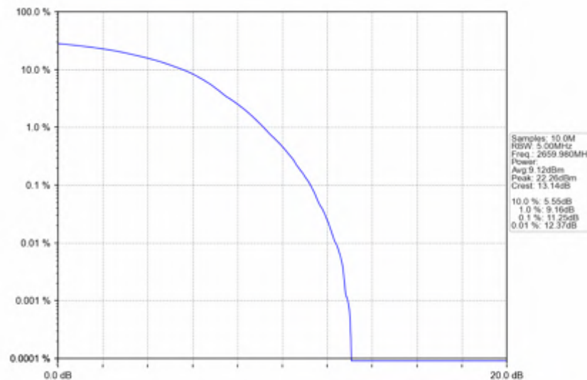
n41_30kHz_SISO_NTNV_60MHz_DFT-s-OFDM QPSK_2659.98MHz_Outer_Full
