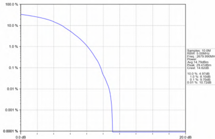
n41_30kHz_SISO_NTNV_20MHz_DFT-s-OFDM 16 QAM_2679.99MHz_Outer_Full
