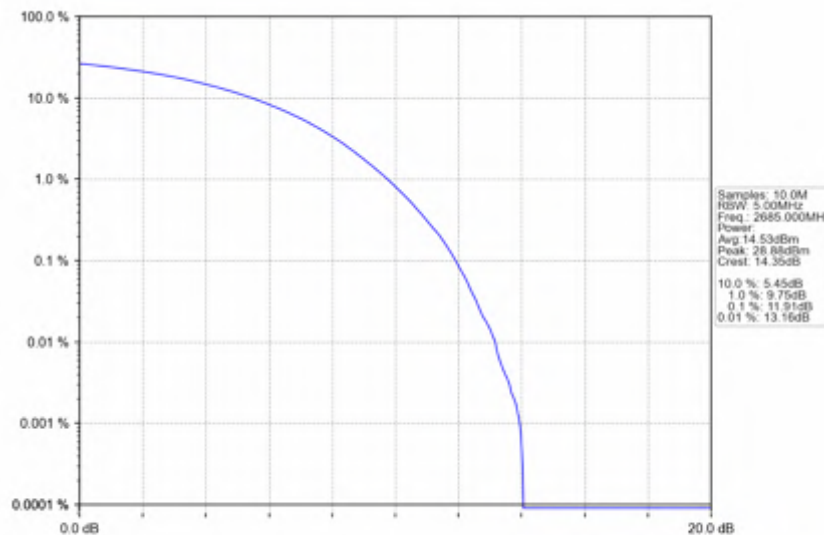
n41_30kHz_SISO_NTNV_10MHz_CP-OFDM 64 QAM_2685MHz_Outer_Full
