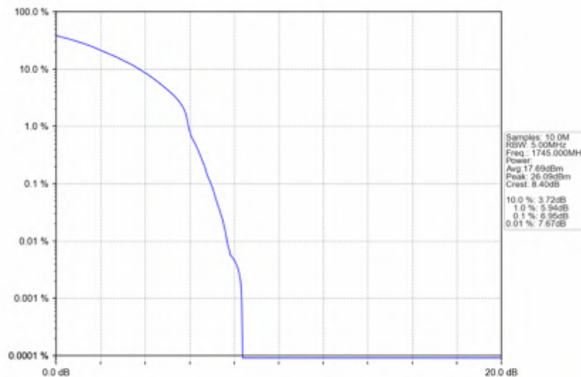
n66_15kHz_SISO_NTNV_15MHz_DFT-s-OFDM_16_QAM_1745MHz_Outer_Full
