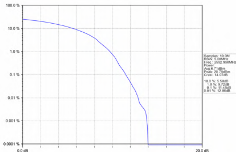
n41 30kHz SISO NTNV 90MHz DFT-s-OFDM QPSK 2592.99MHz Outer Full
