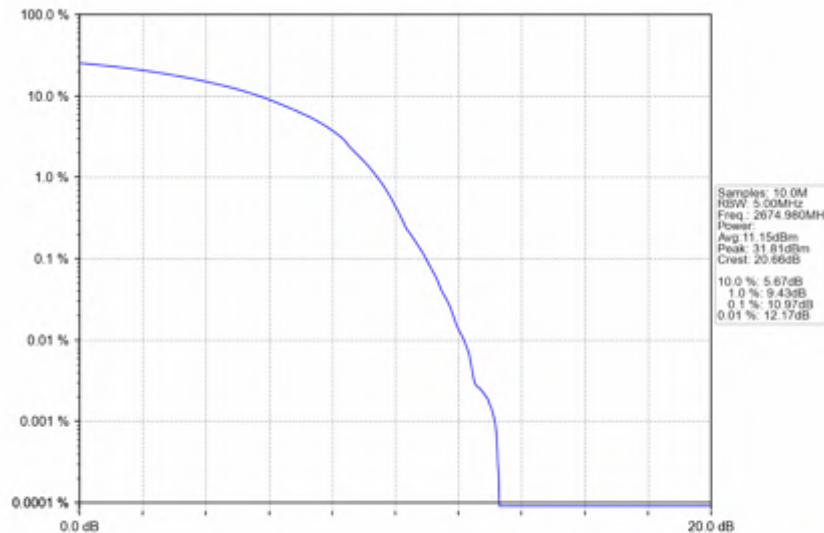
n41_30kHz_SISO_NTNV_30MHz_DFT-s-OFDM_64_QAM_2674.98MHz_Outer_Full
