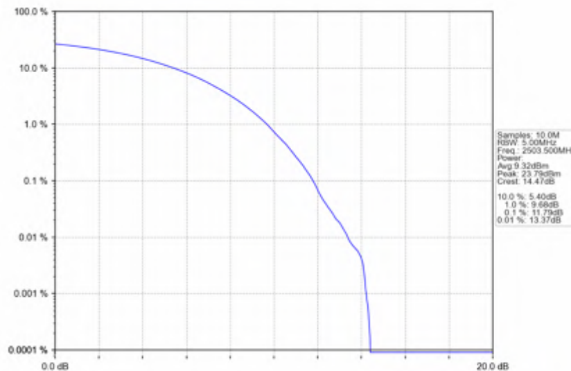
n41_30kHz_SISO_NTNV_15MHz_CP-OFDM_256_QAM_2503.5MHz_Outer_Full
