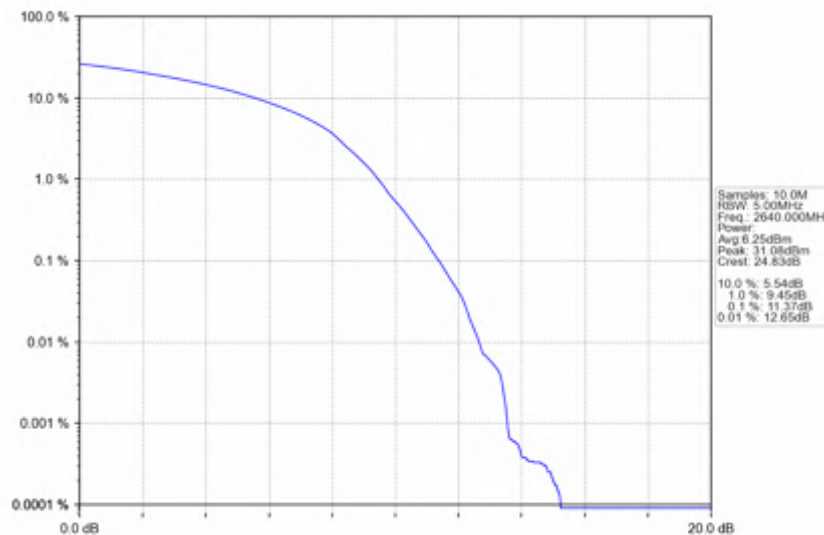
n41_30kHz_SISO_NTNV_100MHz_DFT-s-OFDM 16 QAM 2640MHz_Outer_Full
