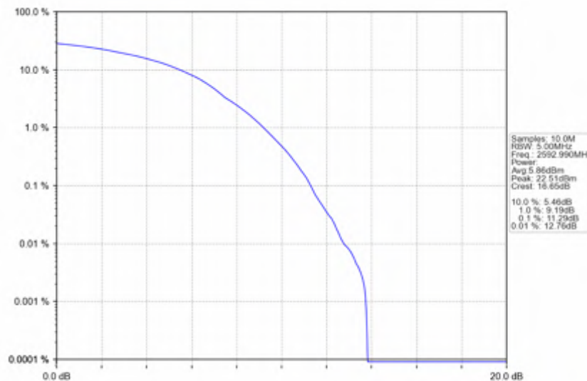
n41_30kHz_SISO_NTNV_80MHz_DFT-s-OFDM_64_QAM_2592.99MHz_Outer_Full
