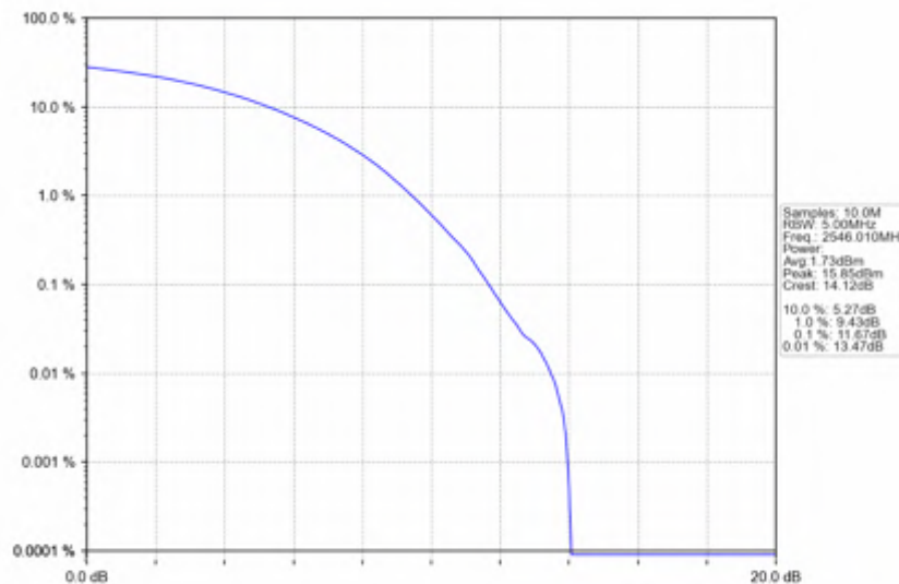
n41_30kHz_SISO_NTNV_100MHz_CP-OFDM_256_QAM_2546.01MHz_Outer_Full
