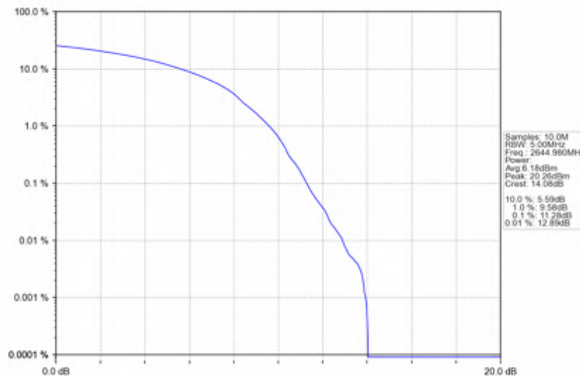
n41_30kHz_SISO_NTNV_90MHz_DFT-s-OFDM_64_QAM_2644.98MHz_Outer_Full
