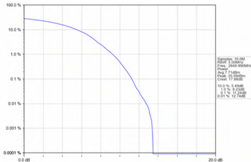
n41_30kHz_SISO_NTNV_80MHz_DFT-s-OFDM QPSK_2649.99MHz_Outer_Full
