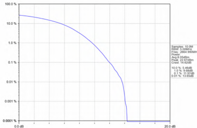
n41_30kHz_SISO_NTNV_50MHz_CP-OFDM_16_QAM_2664.99MHz_Outer_Full
