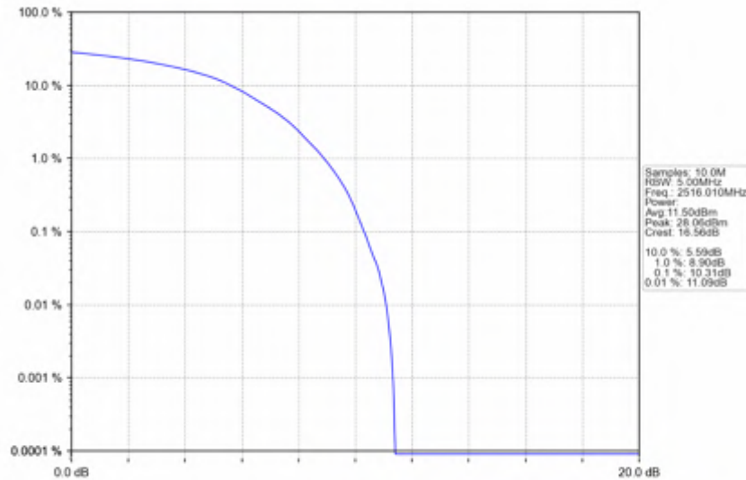
n41 30kHz SISO NTNV 40MHz DFT-s-OFDM PI/2 BPSK 2516.01MHz Outer Full
