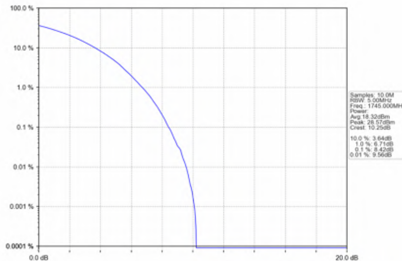
n66_15kHz_SISO_NTNV_10MHz_CP-OFDM QPSK_1745MHz_Outer_Full
