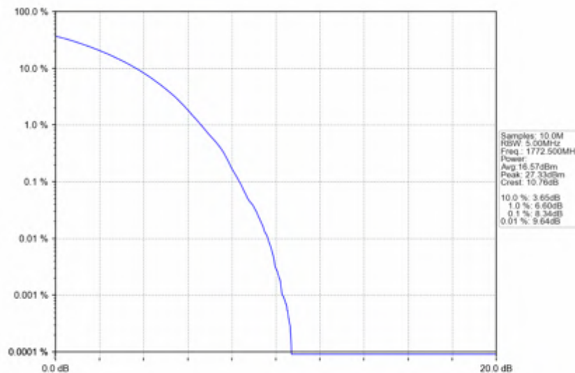
n66_15kHz_SISO_NTNV_15MHz_CP-OFDM QPSK_1772.5MHz_Outer_Full
