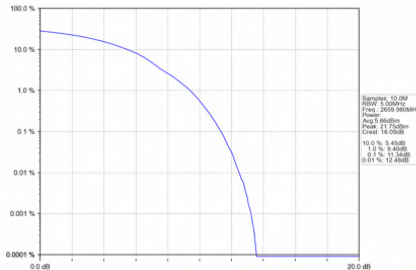
n41_30kHz_SISO_NTNV_60MHz_DFT-s-OFDM 256 QAM_2659.98MHz_Outer_Full
