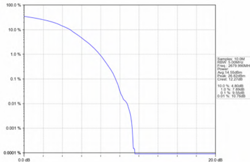
n41_30kHz_SISO_NTNV_20MHz_DFT-s-OFDM 64 QAM_2679.99MHz_Outer_Full
