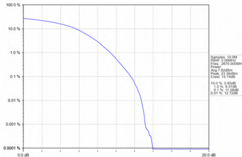
n41_30kHz_SISO_NTNV_40MHz_DFT-s-OFDM 256 QAM_2670MHz_Outer_Full
