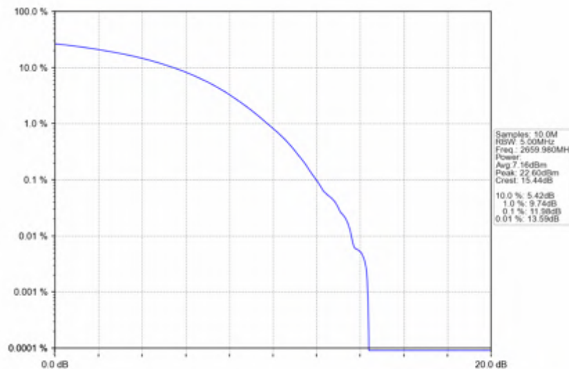
n41_30kHz_SISO_NTNV_60MHz_CP-OFDM QPSK_2659.98MHz_Outer_Full
