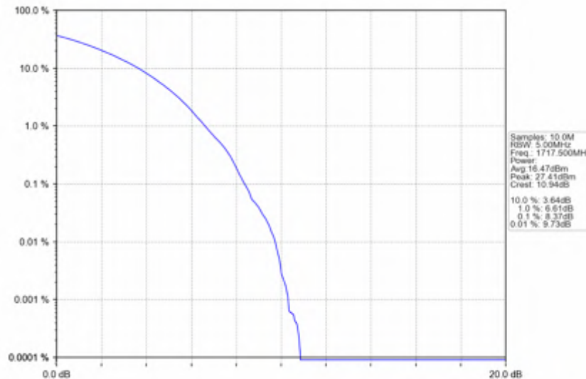
n66_15kHz_SISO_NTNV_15MHz_CP-OFDM_QPSK_1717.5MHz_Outer_Full
