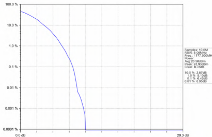
n66_15kHz_SISO_NTNV_5MHz_DFT-s-OFDM_64_QAM_1777.5MHz_Outer_Full
