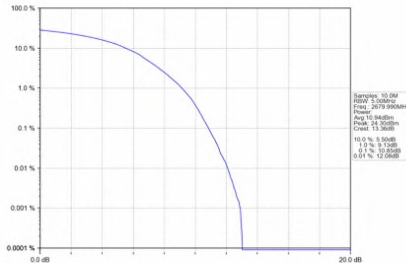
n41_30kHz_SISO_NTNV_20MHz_DFT-s-OFDM 256 QAM_2679.99MHz_Outer_Full
