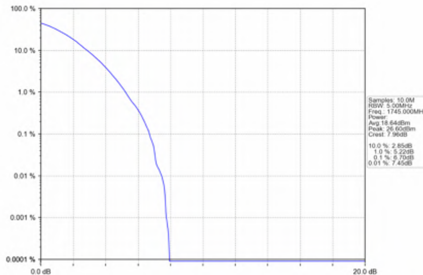
n66_15kHz_SISO_NTNV_5MHz_DFT-s-OFDM_256_QAM_1745MHz_Outer_Full
