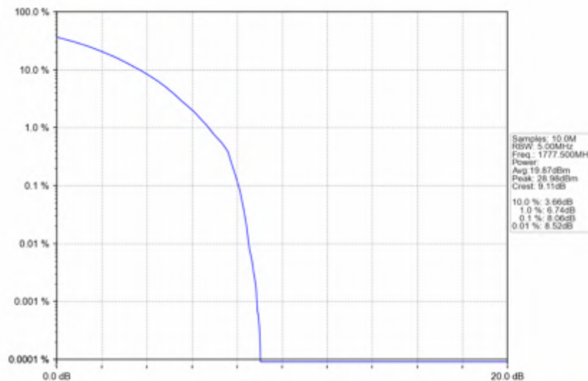
n66_15kHz_SISO_NTNV_5MHz_CP-OFDM 64 QAM_1777.5MHz_Outer_Full
