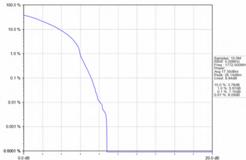
n66_15kHz_SISO_NTNV_15MHz_DFT-s-OFDM_64_QAM_1772.5MHz_Outer_Full
