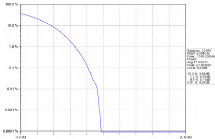
n66_15kHz_SISO_NTNV_10MHz_CP-OFDM 64 QAM_1745MHz_Outer_Full
