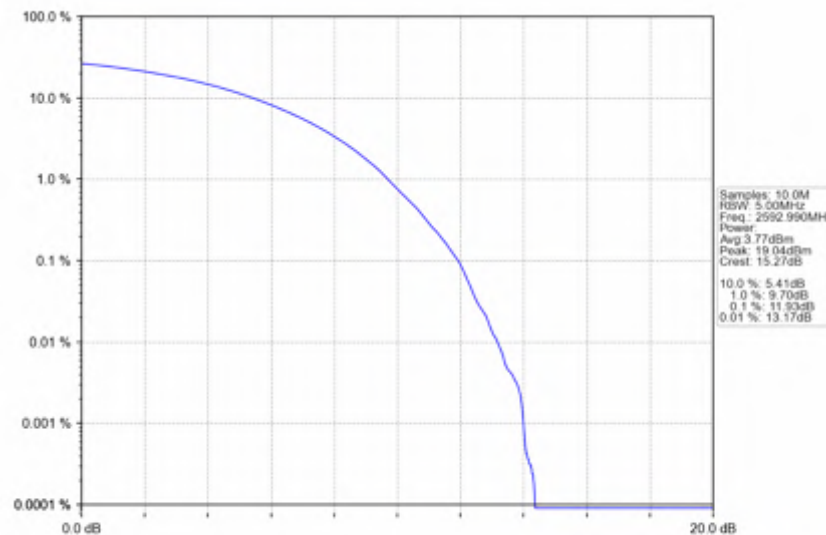
n41_30kHz_SISO_NTNV_100MHz_CP-OFDM 64 QAM_2592.99MHz_Outer_Full
