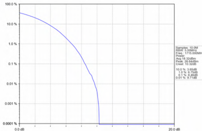
n66_15kHz_SISO_NTNV_10MHz_CP-OFDM QPSK_1715MHz_Outer_Full
