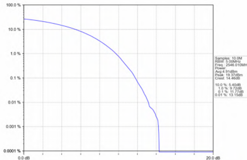
n41_30kHz_SISO_NTNV_100MHz_CP-OFDM_QPSK_2546.01MHz_Outer_Full
