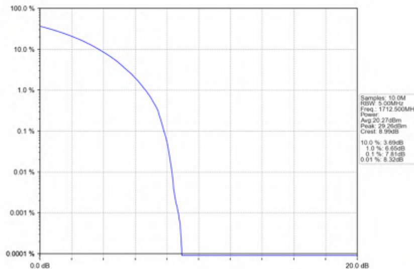
n66_15kHz_SISO_NTNV_5MHz_CP-OFDM_16_QAM_1712.5MHz_Outer_Full
