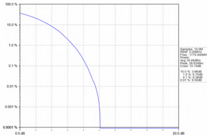
n66_15kHz_SISO_NTNV_10MHz_CP-OFDM QPSK_1775MHz_Outer_Full
