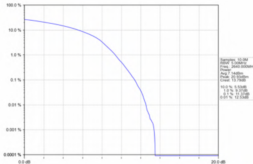
n41_30kHz_SISO_NTNV_100MHz_DFT-s-OFDM QPSK_2640MHz_Outer_Full
