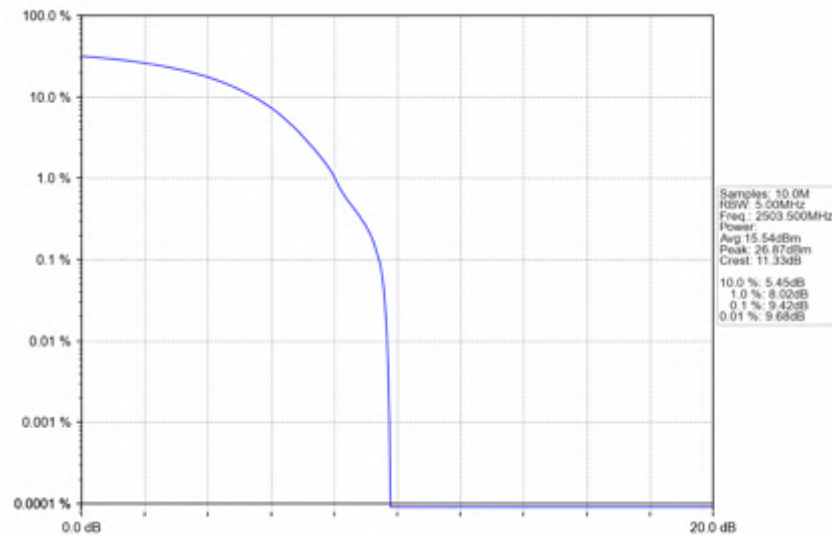
n41_30kHz_SISO_NTNV_15MHz_DFT-s-OFDM PI/2 BPSK_2503.5MHz_Outer_Full
