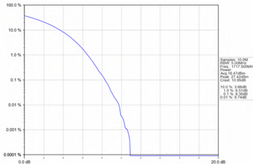
n66_15kHz_SISO_NTNV_15MHz_CP-OFDM_16_QAM_1717.5MHz_Outer_Full
