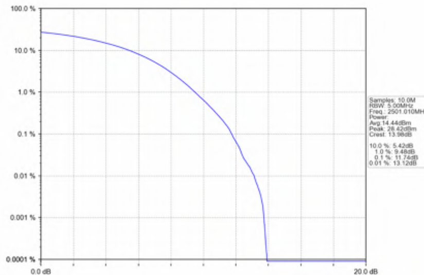
n41_30kHz_SISO_NTNV_10MHz_CP-OFDM 64 QAM_2501.01MHz_Outer_Full
