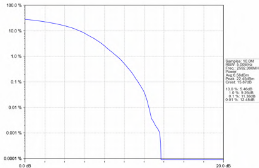
n41_30kHz_SISO_NTNV_50MHz_DFT-s-OFDM_256_QAM_2592.99MHz_Outer_Full
