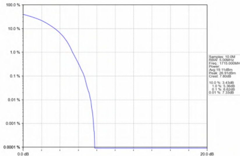
n66_15kHz_SISO_NTNV_10MHz_DFT-s-OFDM_64_QAM_1715MHz_Outer_Full
