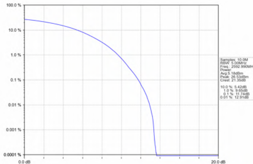
n41_30kHz_SISO_NTNV_40MHz_CP-OFDM_256_QAM_2592.99MHz_Outer_Full
