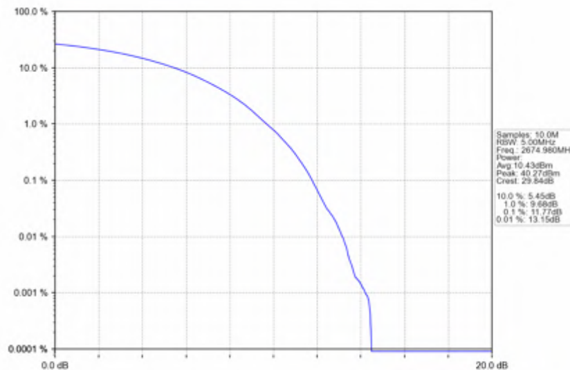
n41_30kHz_SISO_NTNV_30MHz_CP-OFDM 16 QAM_2674.98MHz_Outer_Full
