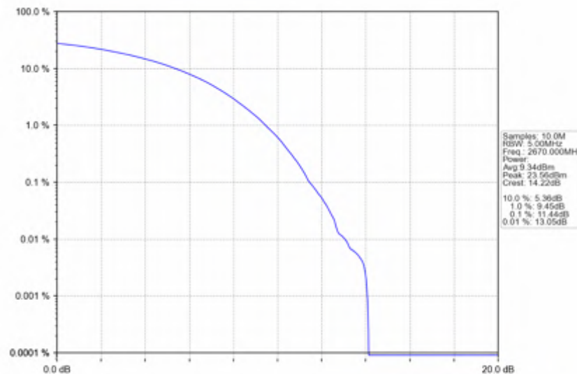
n41_30kHz_SISO_NTNV_40MHz_CP-OFDM QPSK_2670MHz_Outer_Full
