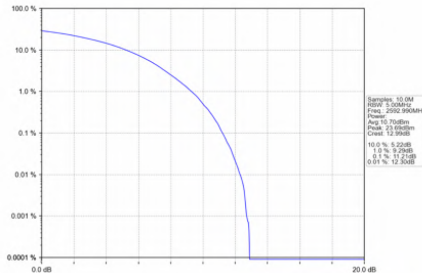
n41_30kHz_SISO_NTNV_30MHz_CP-OFDM QPSK_2592.99MHz_Outer_Full
