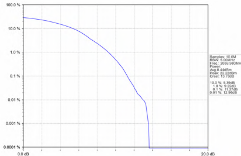
n41_30kHz_SISO_NTNV_60MHz_DFT-s-OFDM_16_QAM_2659.98MHz_Outer_Full
