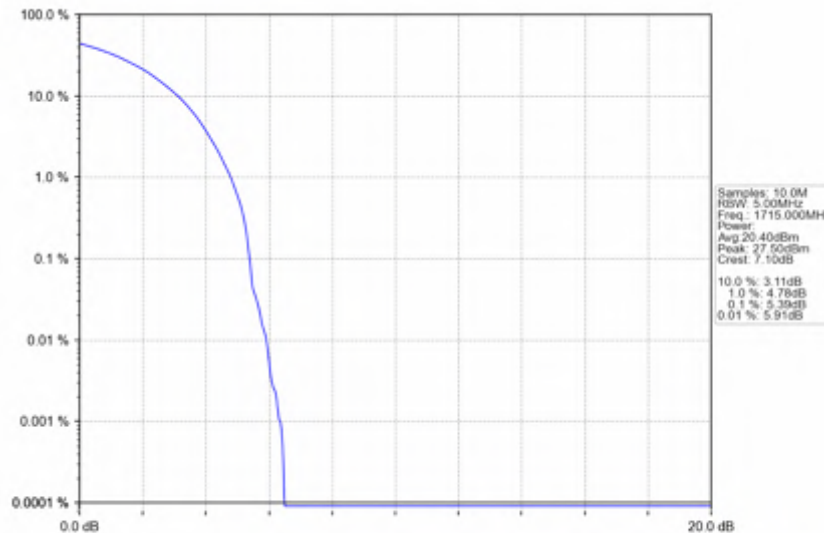
n66_15kHz_SISO_NTNV_10MHz_DFT-s-OFDM QPSK_1715MHz_Outer_Full
