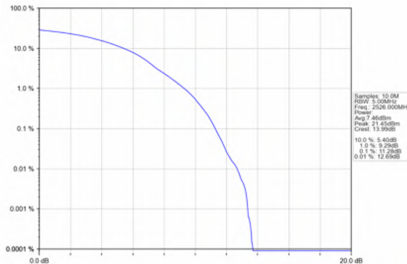
n41_30kHz_SISO_NTNV_60MHz_DFT-s-OFDM_64_QAM_2526MHz_Outer_Full
