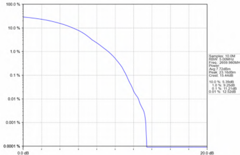
n41_30kHz_SISO_NTNV_60MHz_DFT-s-OFDM_64_QAM_2659.98MHz_Outer_Full
