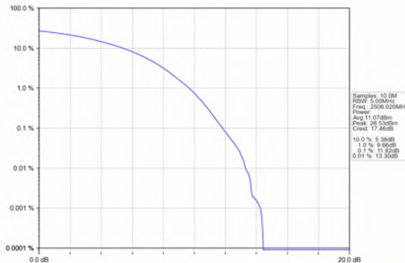
n41_30kHz_SISO_NTNV_20MHz_CP-OFDM_64_QAM_2506.02MHz_Outer_Full
