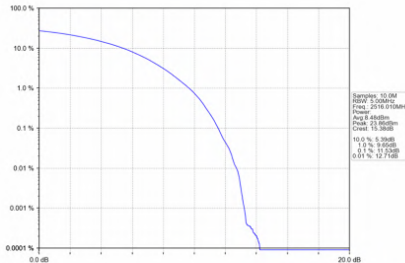
n41_30kHz_SISO_NTNV_40MHz_CP-OFDM 64 QAM_2516.01MHz_Outer_Full
