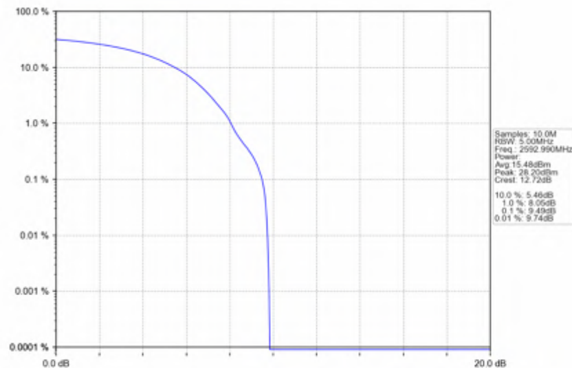
n41_30kHz_SISO_NTNV_15MHz_DFT-s-OFDM PI/2 BPSK_2592.99MHz_Outer_Full
