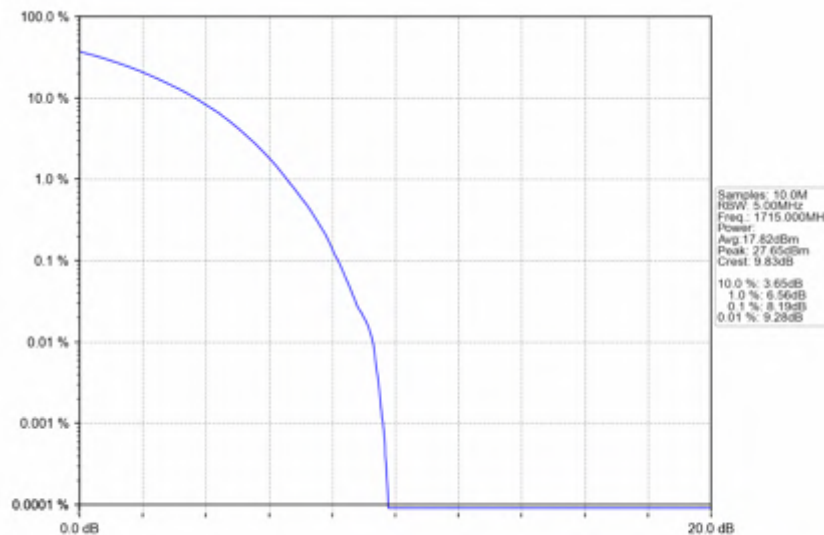
n66_15kHz_SISO_NTNV_10MHz_CP-OFDM 64 QAM_1715MHz_Outer_Full
