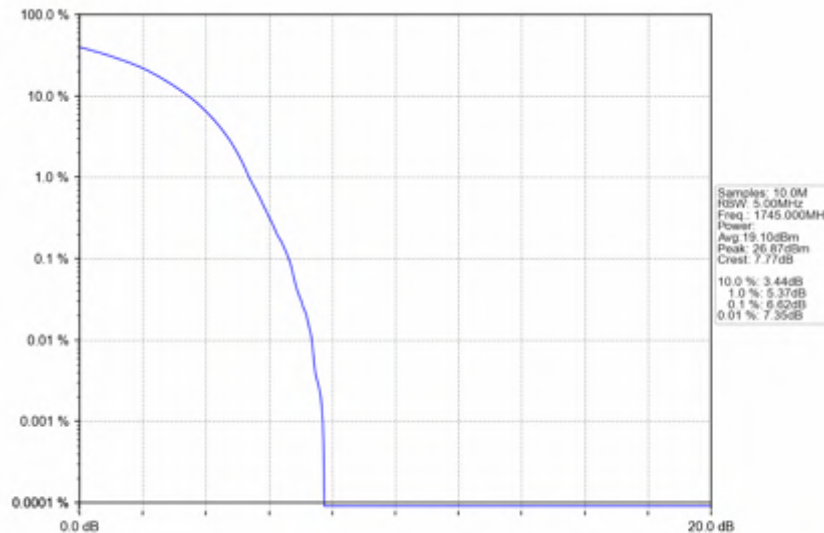
n66_15kHz_SISO_NTNV_10MHz_DFT-s-OFDM_64_QAM_1745MHz_Outer_Full
