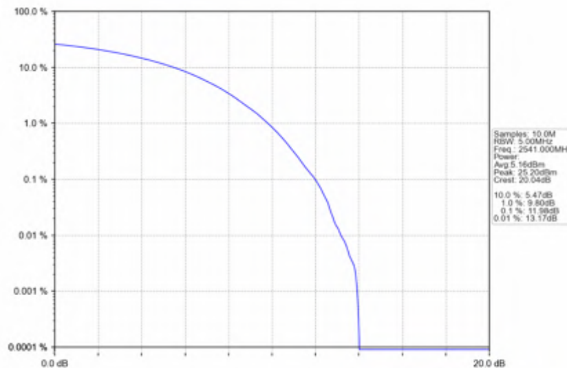
n41_30kHz_SISO_NTNV_90MHz_CP-OFDM_16_QAM_2541MHz_Outer_Full
