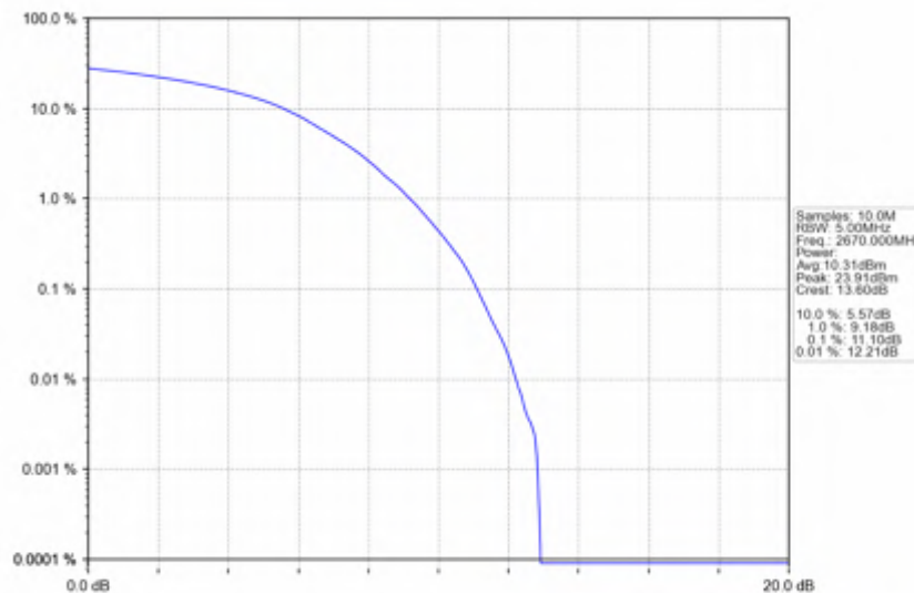
n41_30kHz_SISO_NTNV_40MHz_DFT-s-OFDM_16_QAM_2670MHz_Outer_Full
