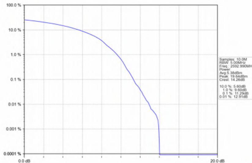
n41_30kHz_SISO_NTNV_90MHz_DFT-s-OFDM_64_QAM_2592.99MHz_Outer_Full
