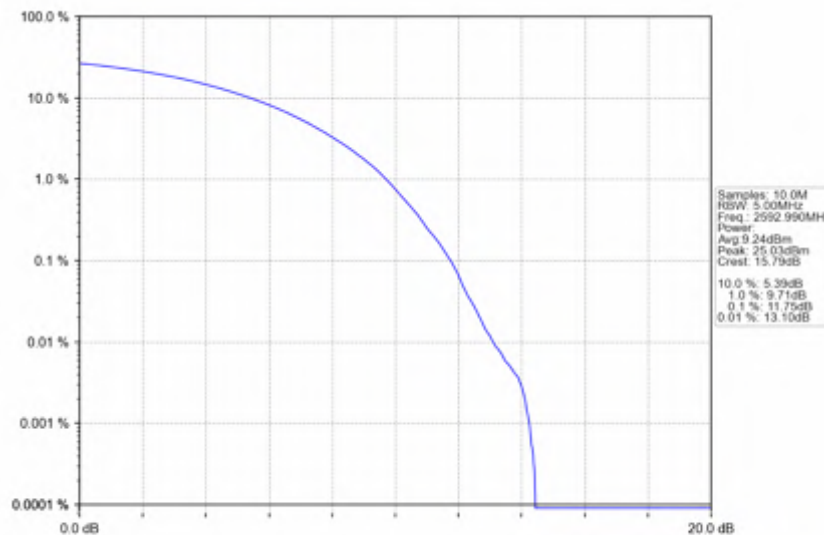
n41_30kHz_SISO_NTNV_15MHz_CP-OFDM_256_QAM_2592.99MHz_Outer_Full
