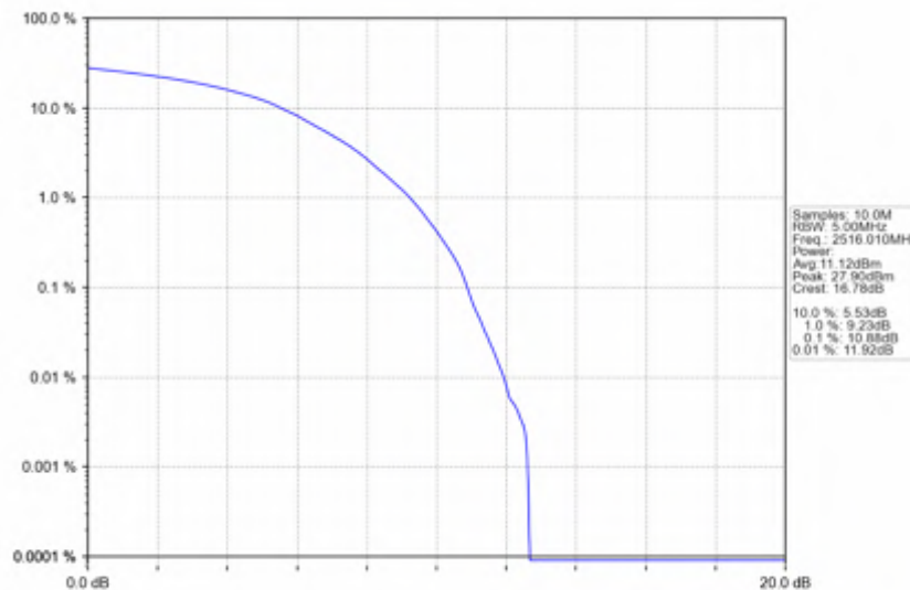
n41_30kHz_SISO_NTNV_40MHz_DFT-s-OFDM QPSK_2516.01MHz_Outer_Full
