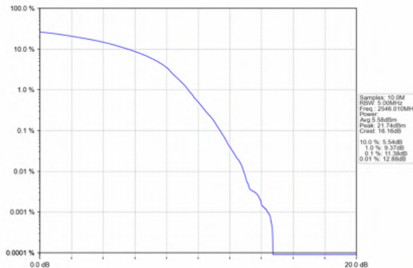
n41_30kHz_SISO_NTNV_100MHz_DFT-s-OFDM 64 QAM 2546.01MHz_Outer_Full
