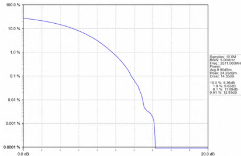
n41_30kHz_SISO_NTNV_30MHz_CP-OFDM 64 QAM_2511MHz_Outer_Full
