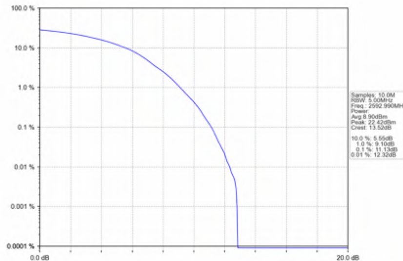
n41_30kHz_SISO_NTNV_60MHz_DFT-s-OFDM QPSK_2592.99MHz_Outer_Full
