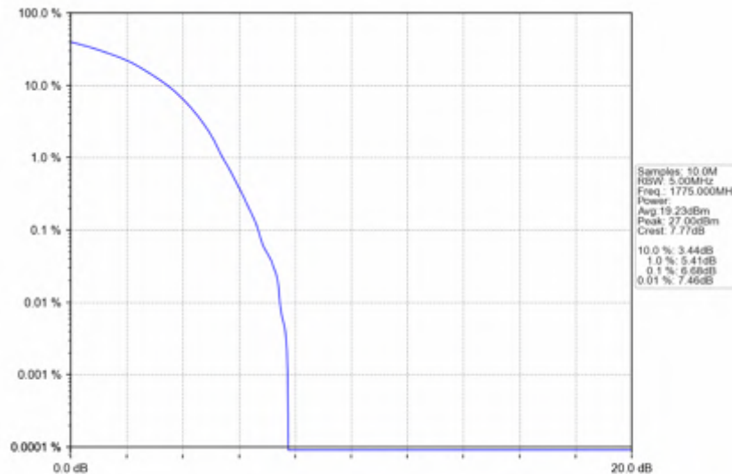
n66_15kHz_SISO_NTNV_10MHz_DFT-s-OFDM_64_QAM_1775MHz_Outer_Full
