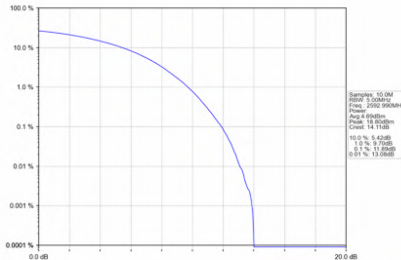
n41_30kHz_SISO_NTNV_90MHz_CP-OFDM_16_QAM_2592.99MHz_Outer_Full
